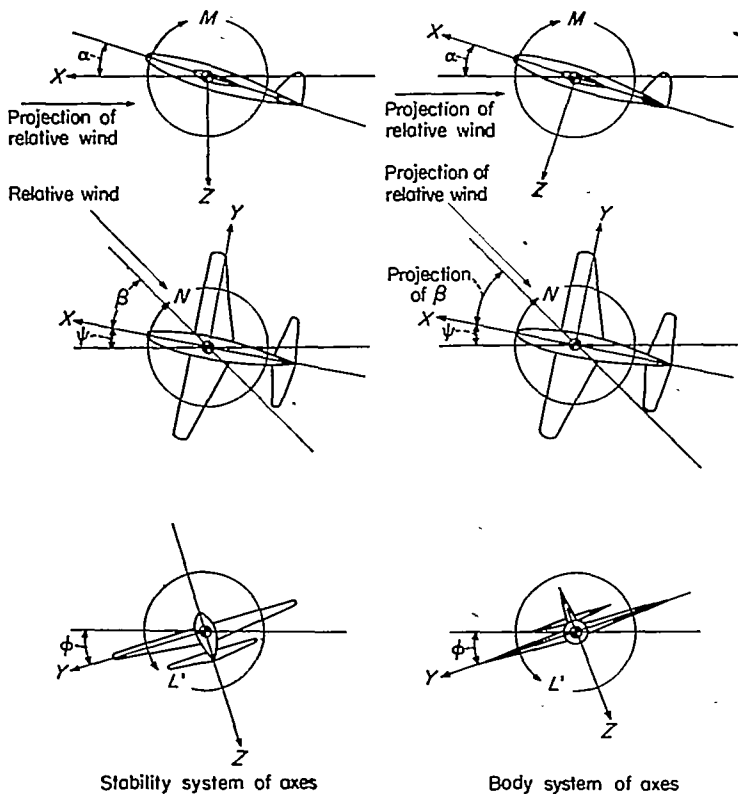
FIGURE 1. —Sketch depicting the stability and body systems of axes. Each view presents a plane of the axes system as viewed along the third axis.
