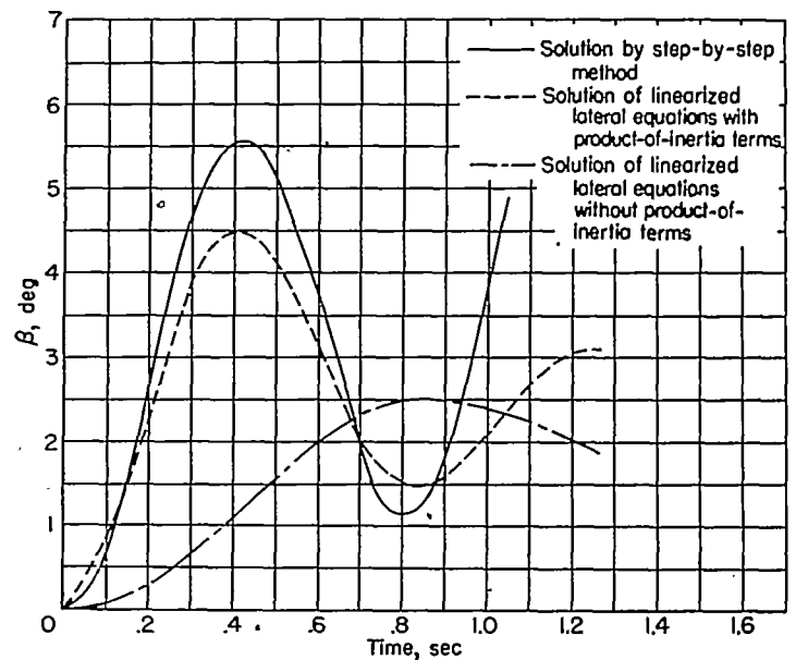
FIGURE 9.—Comparison of a solution by step-by-step method and a solution of linearized lateral equations of the variation of angle of sideslip with time for airplane A, loading 1, when rolled in a 0g pullout.
