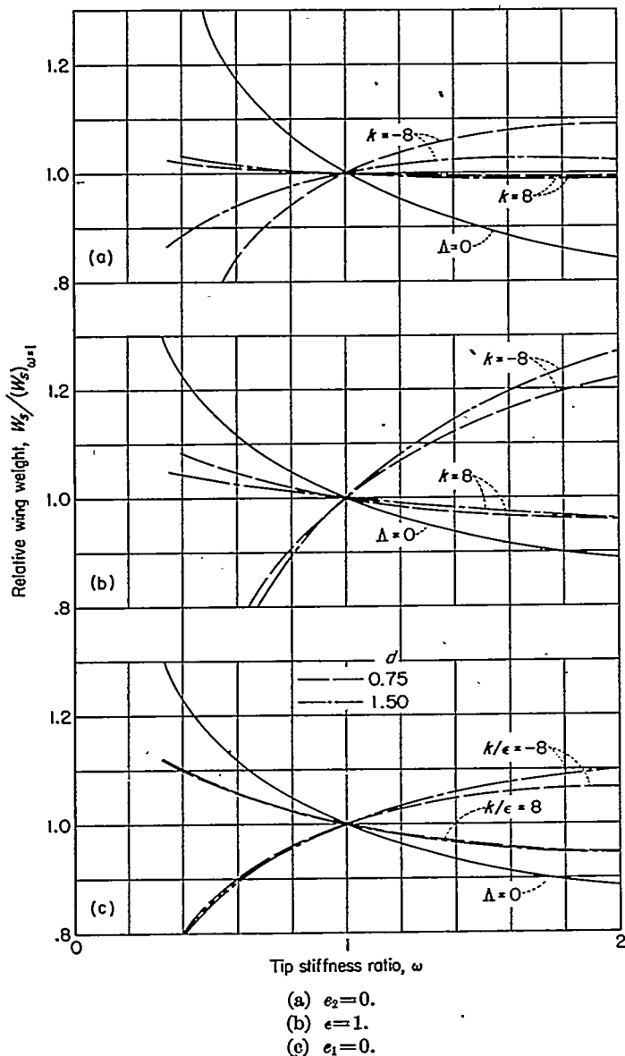
FIGURE 10.—The effect of tip stiffness ratio on the structural weight required to maintain a constant level of lateral-control effectiveness ( C_{l_3}=0.8C_{l_{30}} ) at a given dynamic pressure for wings with a taper ratio of 0.5.
