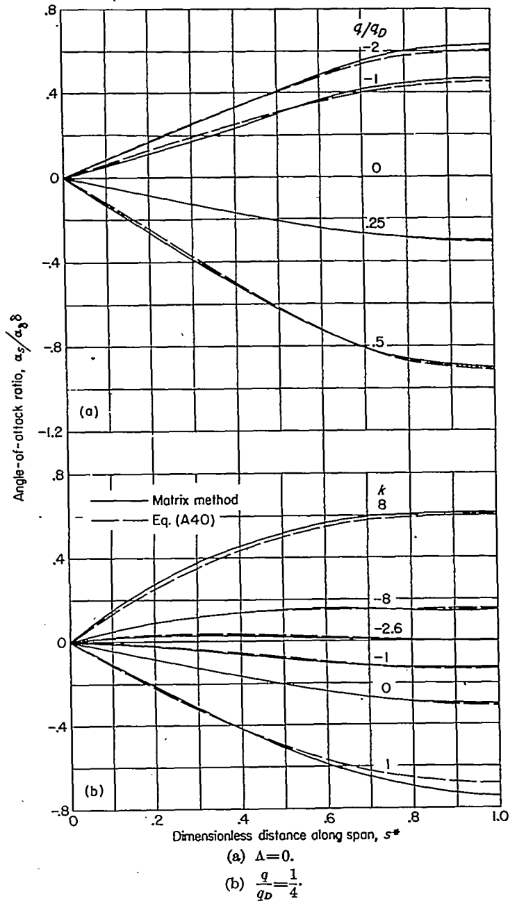
FIGURE 14.—Comparison of angle-of-attack ratios calculated by the matrix method of the appendix with those calculated by equation (A40) for uniform wings. s_r^* = 0.5 ; \epsilon = 1.0 .
