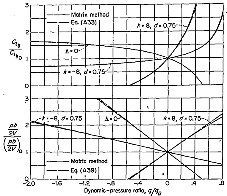
FIGURE 13.—Comparison of rolling power and rolling maneuverability calculated by the matrix method of the appendix with those calculated by equations (A33) and (A39) for uniform wings. s_1^* = 0.5 ; \epsilon = 1.0 .
