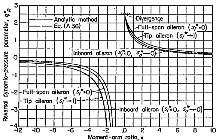
FIGURE 6.—Comparison of dynamic pressures at aileron reversal calculated by the analytic integration method of the appendix with those calculated from equation (A36) for unswept uniform wings.
