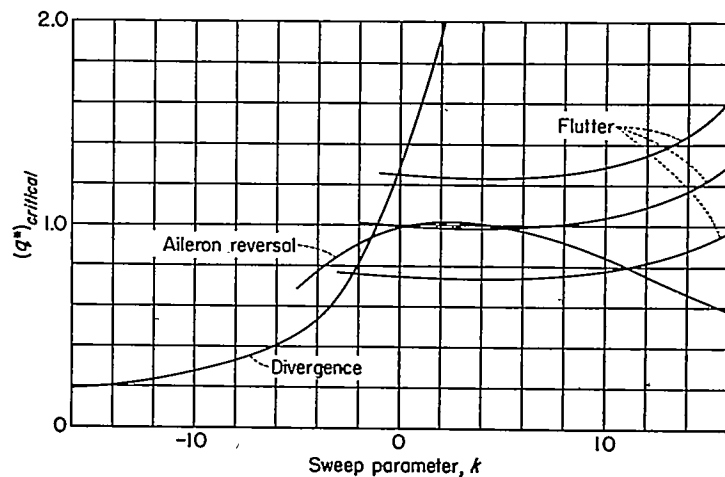
FIGURE 11.—Variation of critical dynamic pressures with the sweep parameter k .
