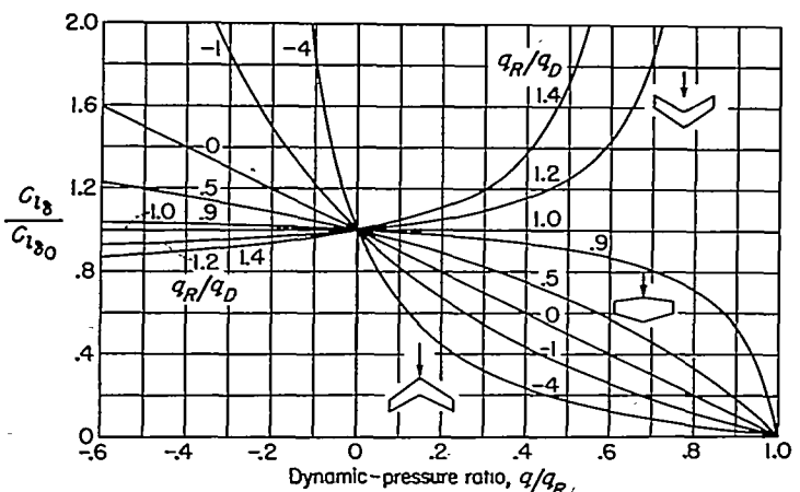
FIGURE 8.—Variation of aileron rolling effectiveness with dynamic-pressure ratio and the parameter q_R/q_D .
