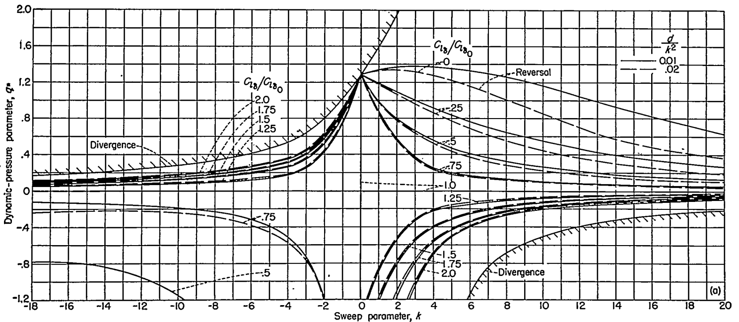
(a) Wings with moment arm \epsilon_2=0 . FIGURE 4.—Charts for a preliminary survey of lateral control for flexible wings of taper ratio 0.5.
