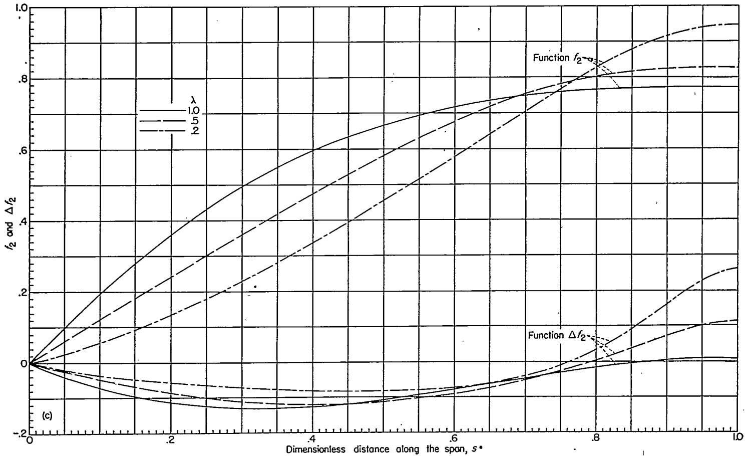
(e) Stiffnesses proportional to c^4 .
