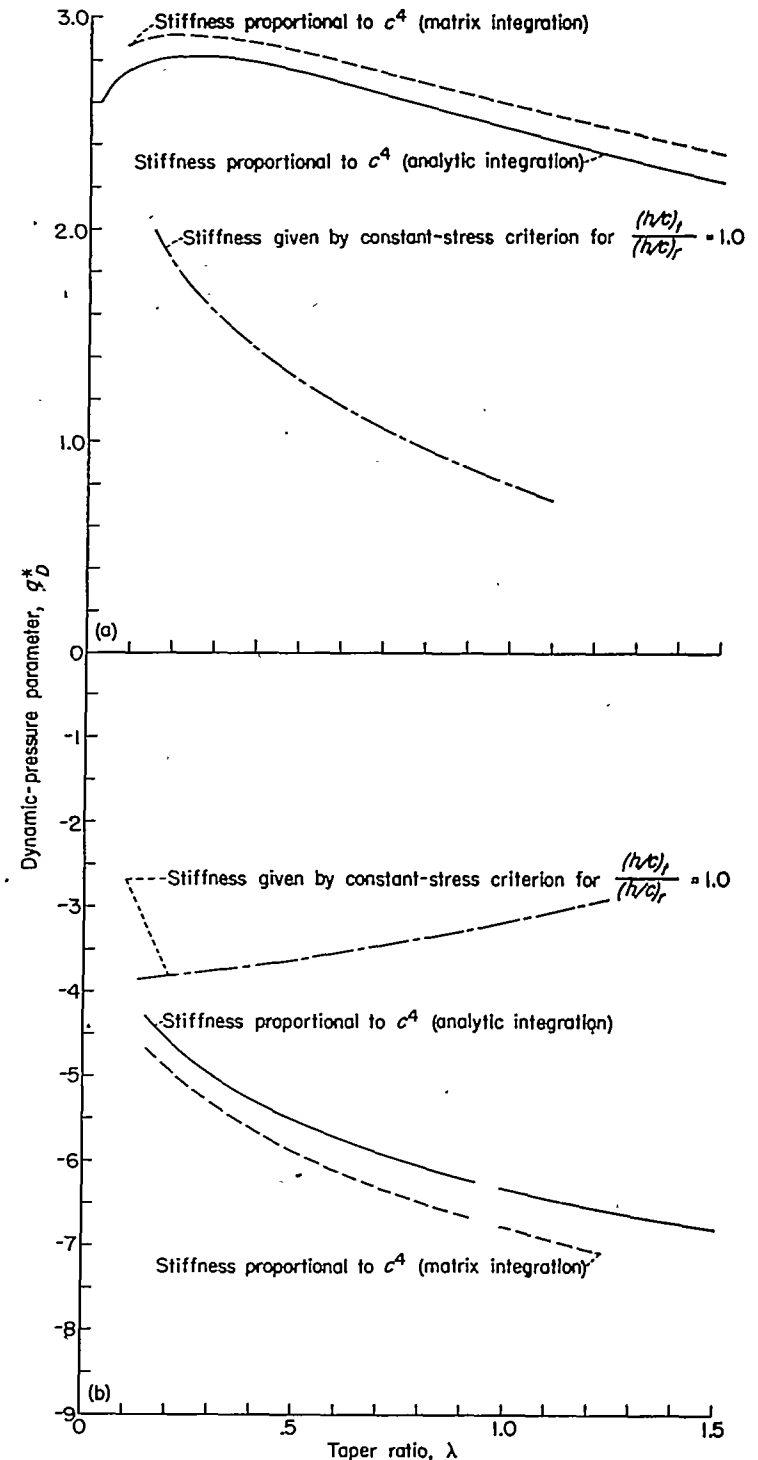
(a) Effect of taper ratio on q^*_D for unswept wings. ( q^*_D = K_1 in this case.)
