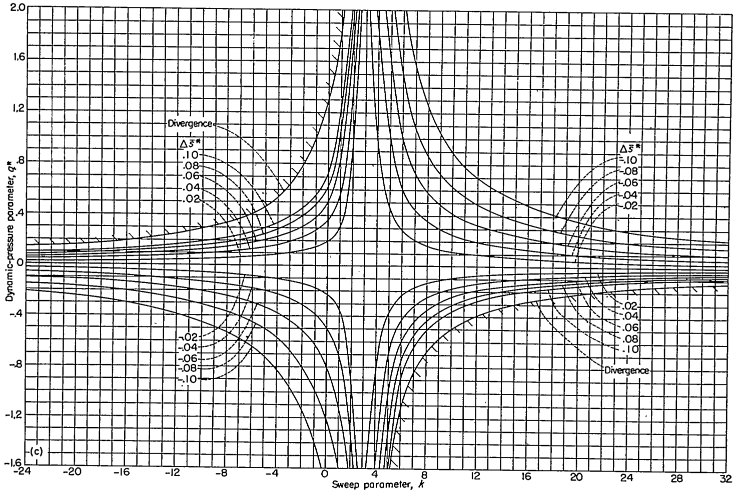
(c) Wings of taper ratio 0.5. FIGURE 2.—Continued.
