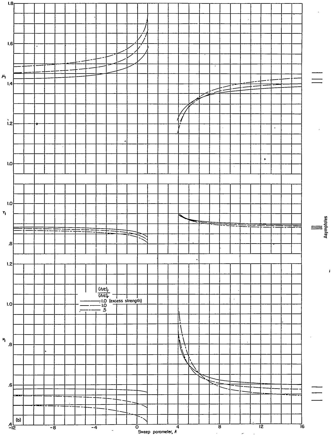
(b) Stiffnesses related to those given by constant-stress criterion for wings with taper ratio 0.5.
