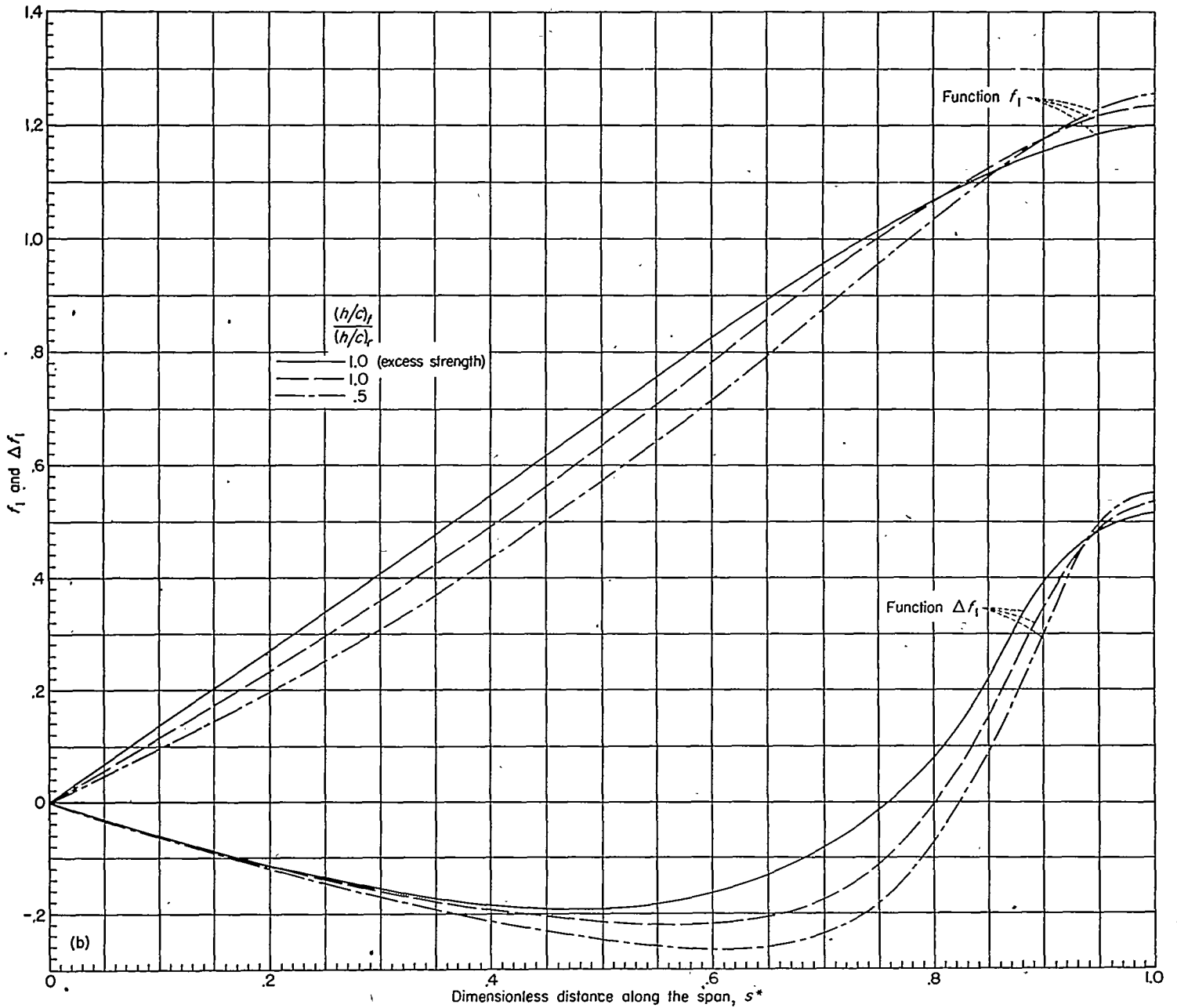
(b) Stiffnesses related to those given by constant-stress criterion for wings with taper ratio 0.5. FIGURE 5.—Continued.
