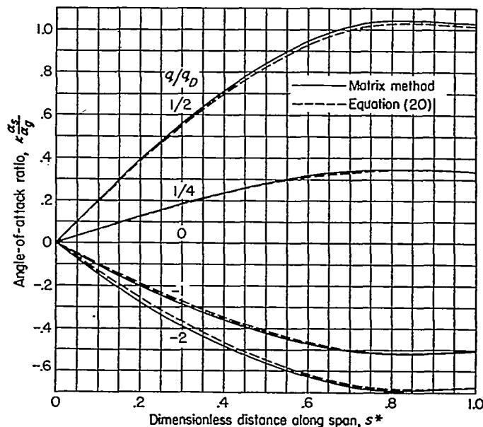
FIGURE 16.—Comparison of angle-of-attack ratios calculated by the matrix method of appendix A with those calculated from equation (20) for constant geometric angles of attack at various dynamic-pressure ratios. \lambda=0.5; k=8 ; stiffnesses proportional to c^4 .
