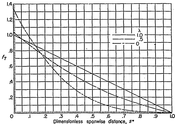
FIGURE 20.—The twisting-moment function f_7 .
