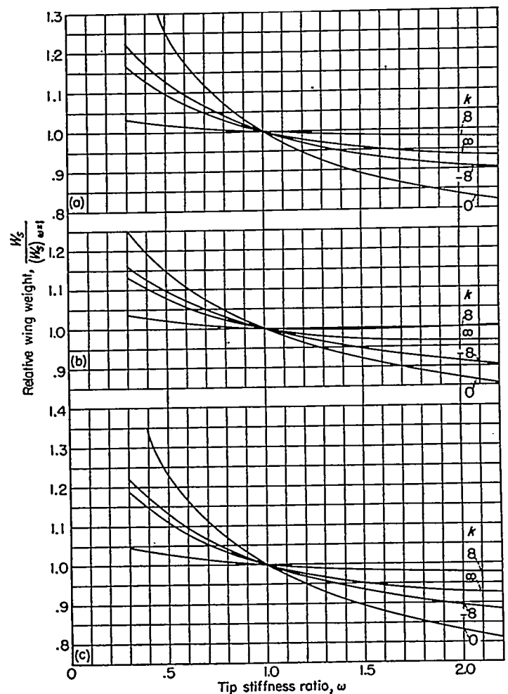
(a) Relative weight required for a given dynamic pressure at divergence. (b) Relative weight required for \frac{\bar{s}}{\bar{s}_0} = 0.9 at a given dynamic pressure. (c) Relative weight required for \frac{\bar{s}}{\bar{s}_0} = 1.1 at a given dynamic pressure.
