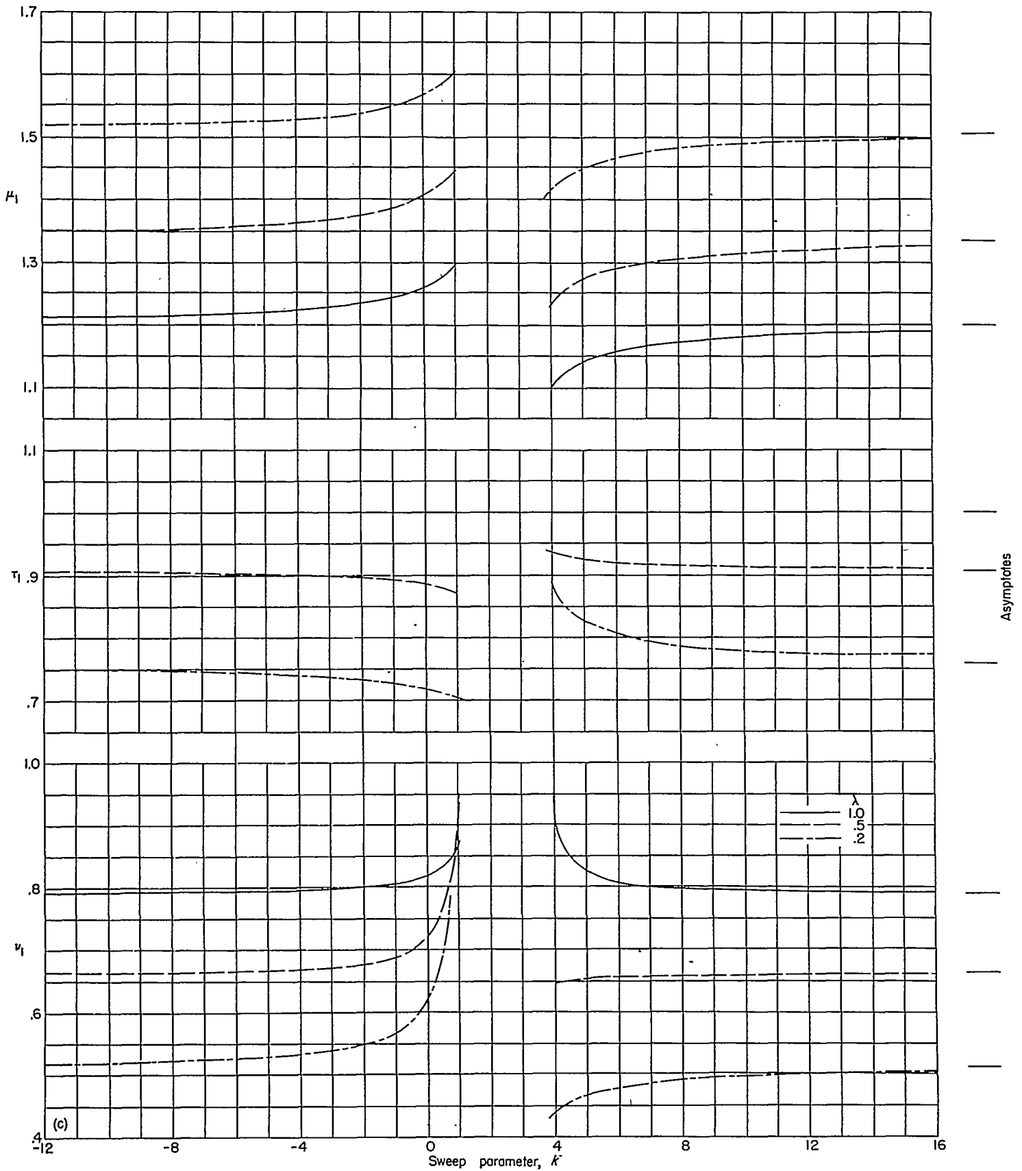
(e) Stiffnesses proportional to c^4 .
