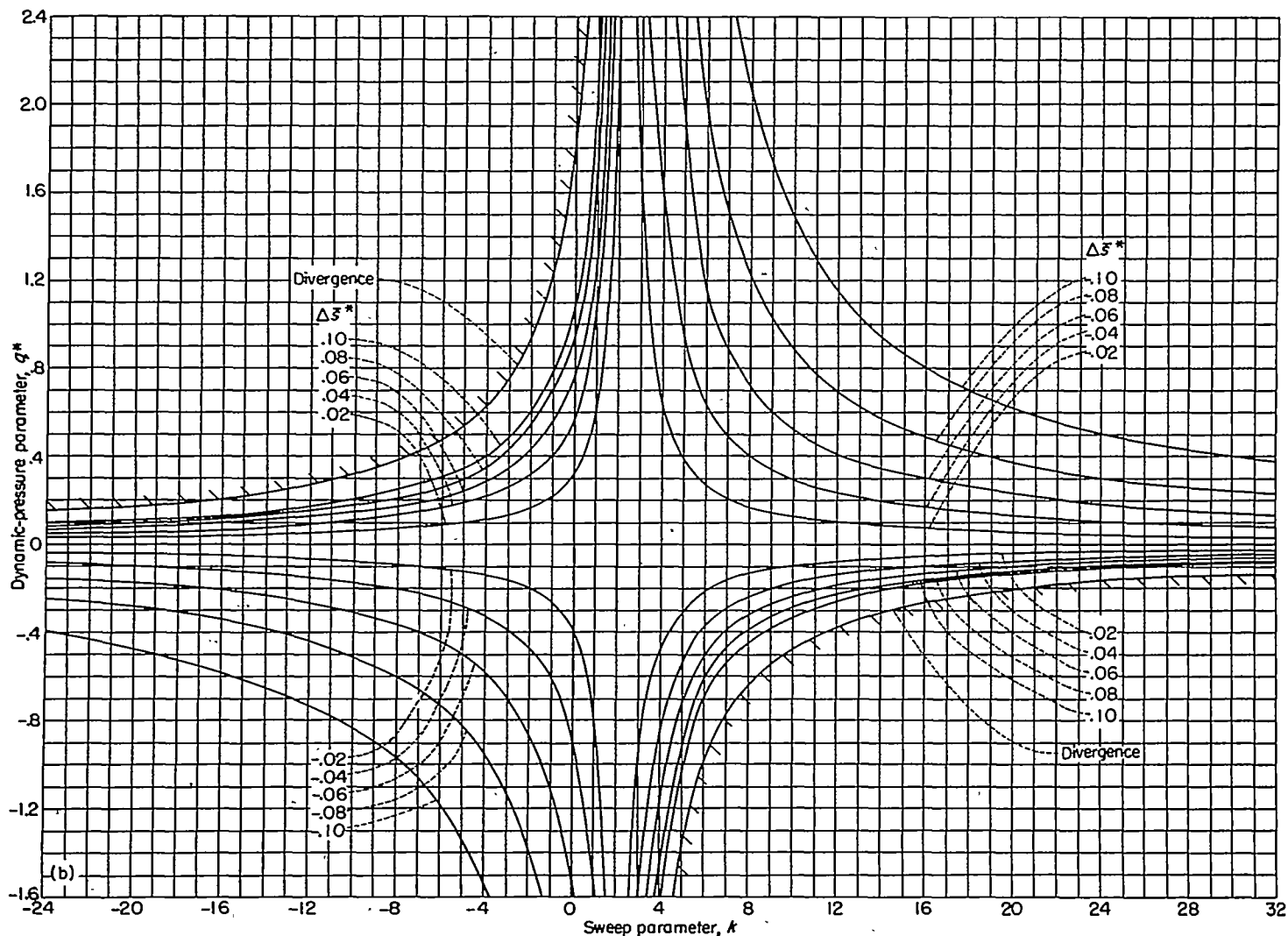
(b) Wings of taper ratio 0.2. FIGURE 2.—Continued.
