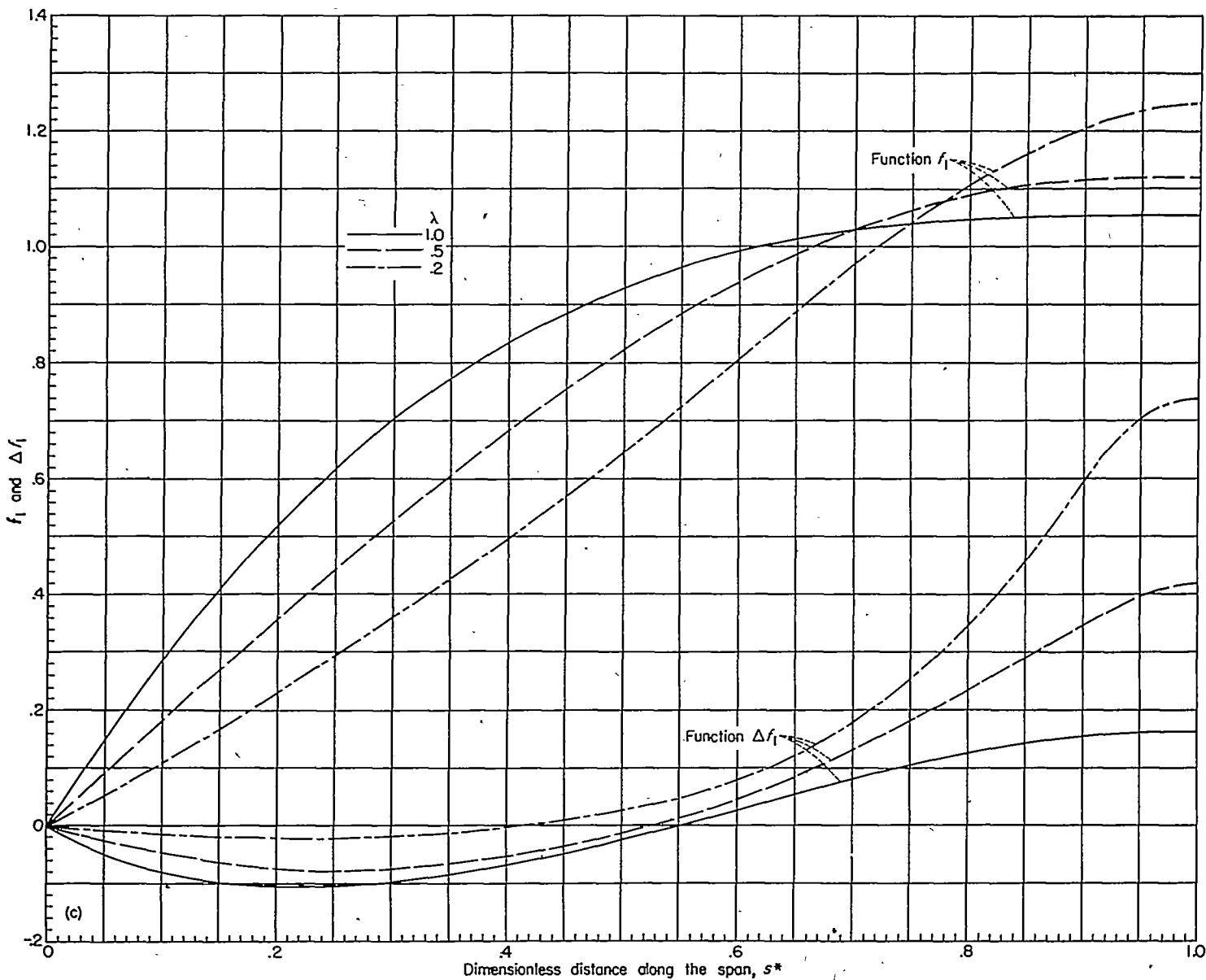
(c) Stiffnesses proportional to c^4 .
