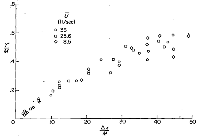
FIGURE 4.—Spread of heat from a line source. \frac{x_0}{M}=43.4 , M=1 inch.
