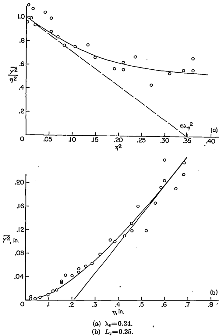
FIGURE 19.—Determination of \lambda_\eta and L_\eta ; \frac{x_0}{M} = 86.1 , M = \frac{1}{2} inch, and \bar{U} = 25.6 feet per second.
