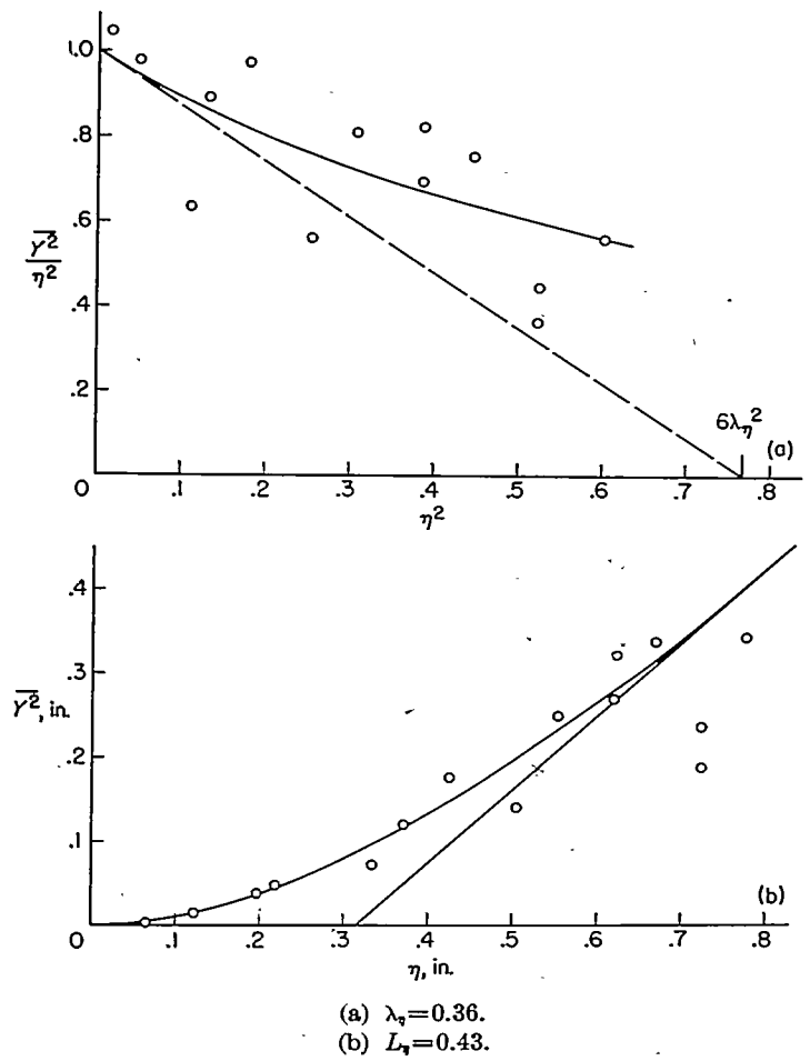
FIGURE 13.—Determination of \lambda_\eta and L_\eta ; \frac{x_0}{M} = 43.4 , M = 1 inch, and \bar{U} = 8.5 feet per second.
