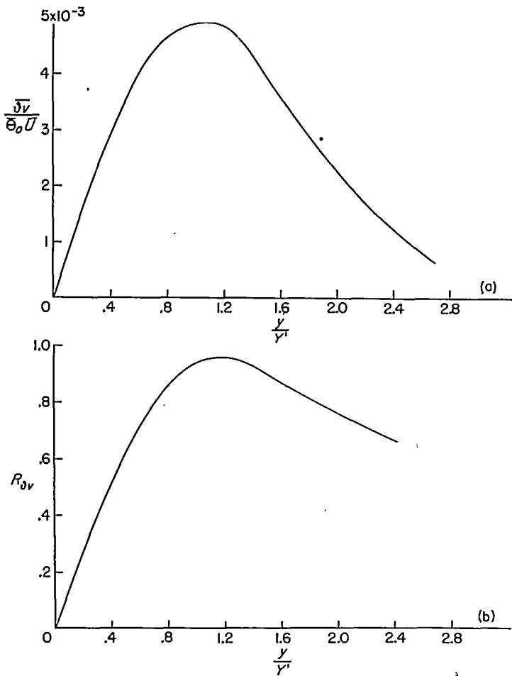
(a) \frac{\delta v}{\theta_0 U} against \frac{y}{Y'} . (b) R_{\theta v} against y/Y' .
