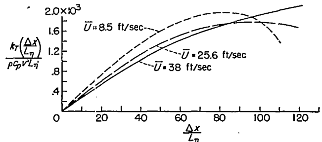
FIGURE 39.—Dimensionless turbulent-heat-transfer coefficient. \frac{x_0}{M}=43.4 and M=1 inch.
