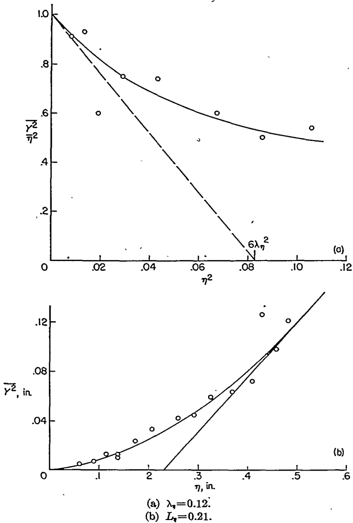
FIGURE 17.—Determination of \lambda_\eta and L_\eta ; \frac{x_0}{M} = 43.4 , M = \frac{1}{4} inch, and \bar{U} = 25.6 feet per second.
