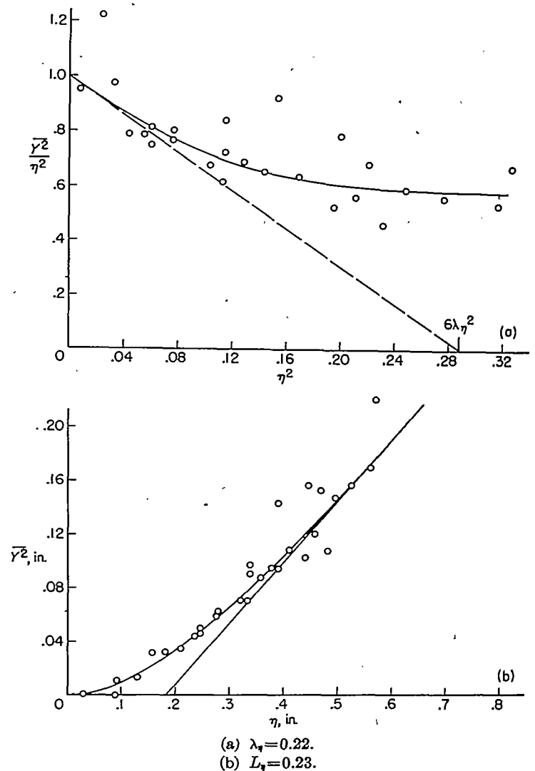
FIGURE 18.—Determination of \lambda_\eta and L_\eta ; \frac{x_0}{M} = 86.1 , M = 1 inch, and \bar{U} = 25.6 feet per second.
