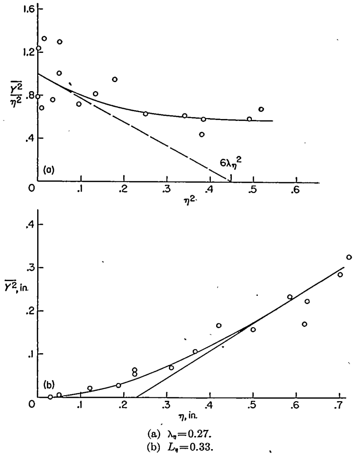
FIGURE 15.—Determination of \lambda_v and L_v ; \frac{x_0}{M} = 43.4 , M = 1 inch, and \bar{U} = 38 feet per second.
