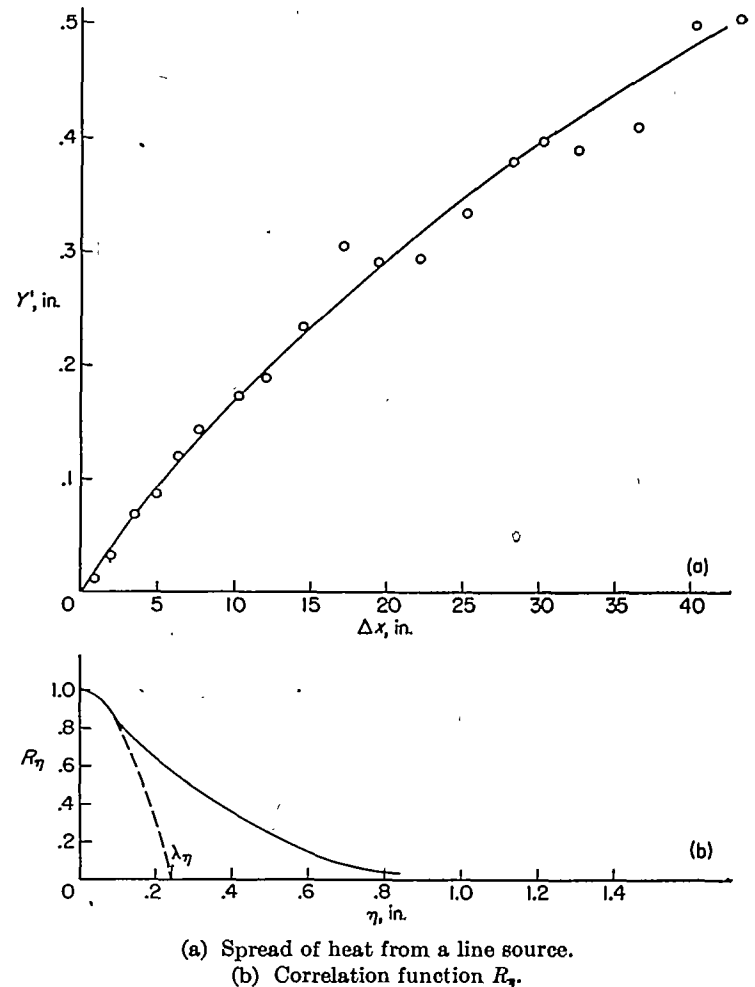
FIGURE 26.—Spread of heat from a line source and correlation function R_\eta for M=\frac{1}{2} inch, \bar{U}=25.6 feet per second, and \frac{x_o}{M}=43.4 .
