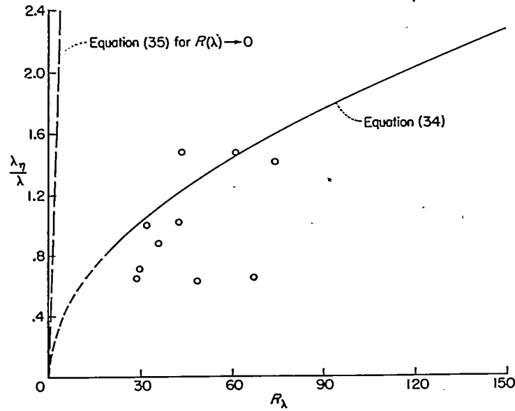
FIGURE 33.—Ratio of Lagrangian and Eulerian microscales.
