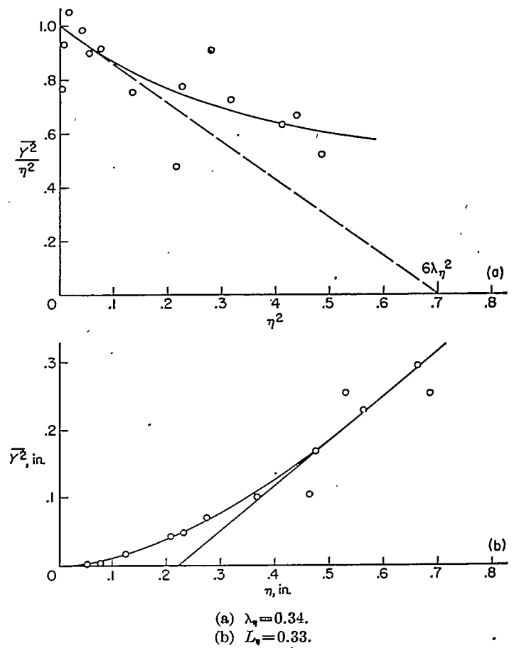
FIGURE 14.—Determination of \lambda_\eta and L_\eta ; \frac{x_0}{M} = 43.4 , M = 1 inch, and \bar{U} = 25.6 feet per second.
