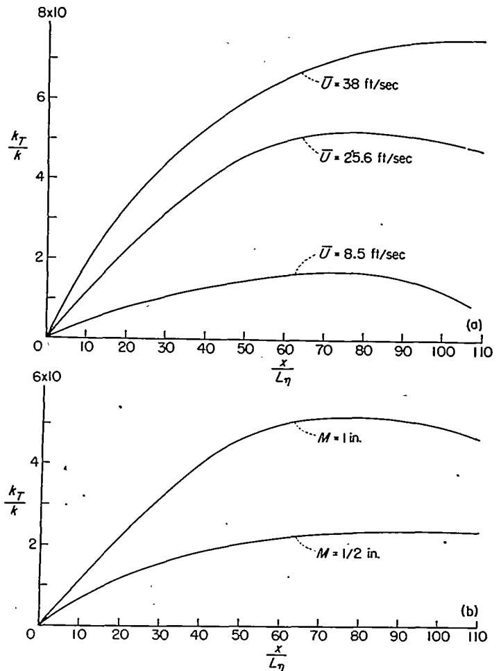
(a) Turbulent-heat-transfer coefficient at three airspeeds. M=1 inch and \frac{x_0}{M}=43.4 . (b) Turbulent-heat-transfer coefficient for two different grids. \bar{U}=25.6 feet per second and \frac{x_0}{M}=43.4 .
