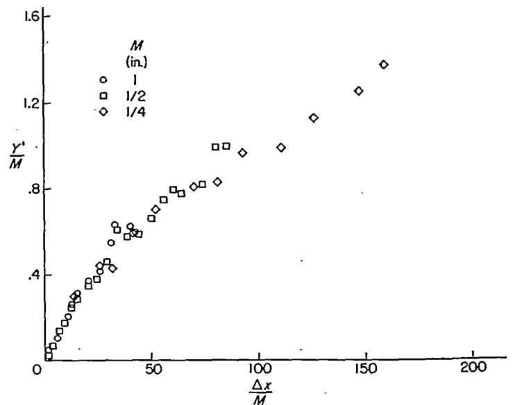
FIGURE 5.—Spread of heat from a line source. \frac{x_0}{M}=43.4 , \bar{U}=25.6 feet per second.
