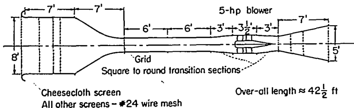
FIGURE 1.—Sketch of open-return wind tunnel.
