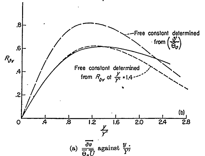
(a) \frac{\partial v}{\partial \theta} / \bar{U} against \frac{y}{Y'} . (b) R_{\partial_o} against y/Y' . Dashed curves are result of analysis based on rectangular temperature pulses.
