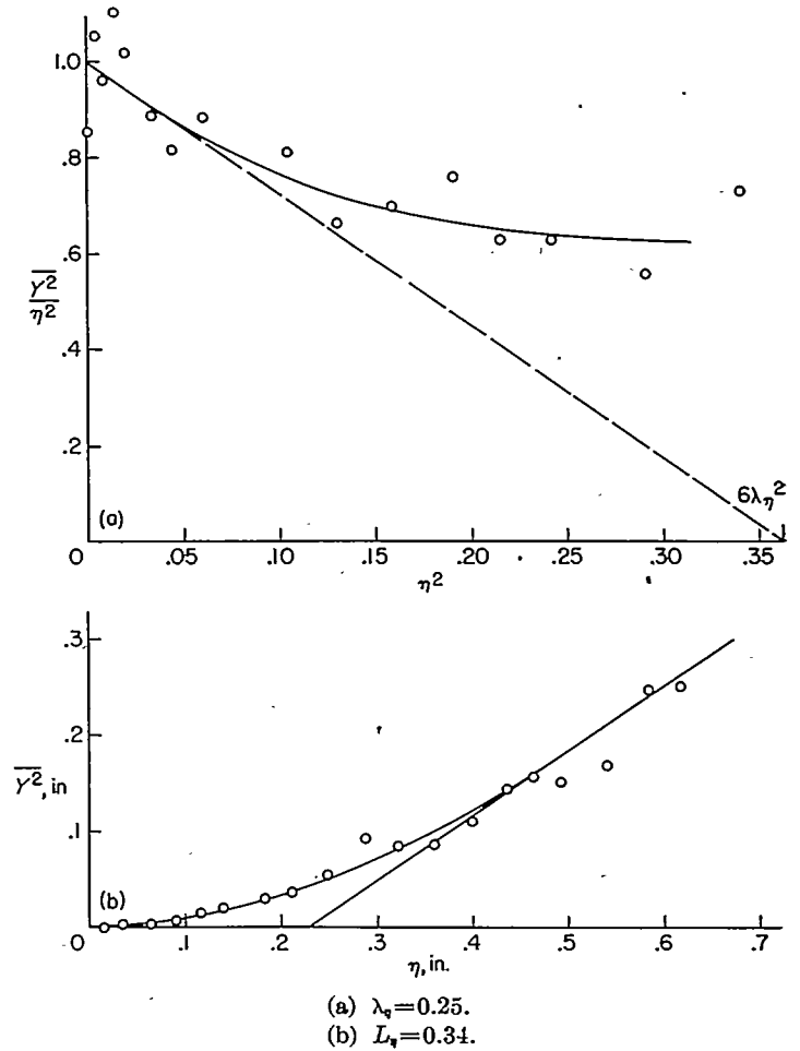
FIGURE 16.—Determination of \lambda_v and L_v ; \frac{x_0}{M} = 43.4 , M = \frac{1}{2} inch, and \bar{U} = 25.6 feet per second.
