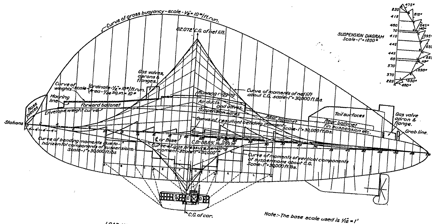
LOAD AND BENDING MOMENT DIAGRAM FOR A NON-RIGID AIRSHIP
