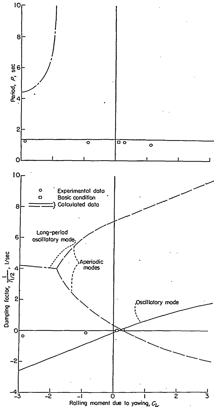
FIGURE 13.—Calculated effect of C_{l_r} on stability and comparison with experimental data.
