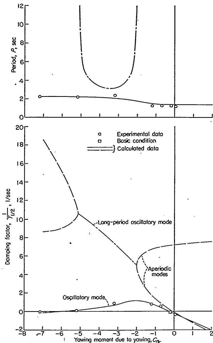
FIGURE 7.—Calculated effect of C_{nr} on stability and comparison with experimental data.
