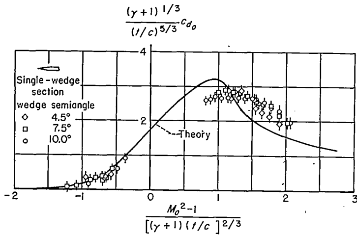
FIGURE 6.—Drag correlation of single-wedge section, k=(\gamma+1)/U_0 .
