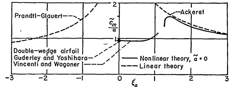
FIGURE 13.—Theoretical pitching-moment curve slope of double-wedge airfoils.
