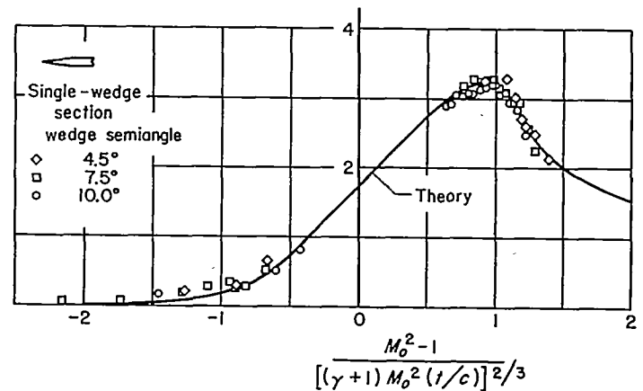
FIGURE 7.—Drag correlation of single-wedge section, k=M_0^2(\gamma+1)/U_0 .
