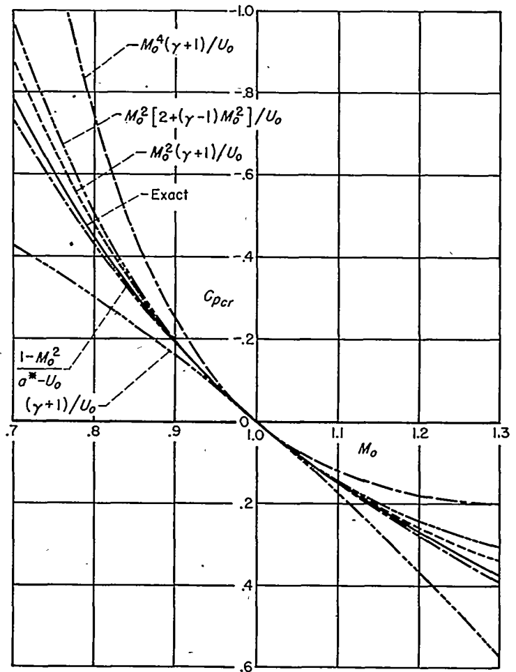
FIGURE 2.—Variation of critical pressure coefficient with Mach number. of \varphi_{xx} in equation (7) corresponds, in the present approximation, to 1 - M^2 , thus
