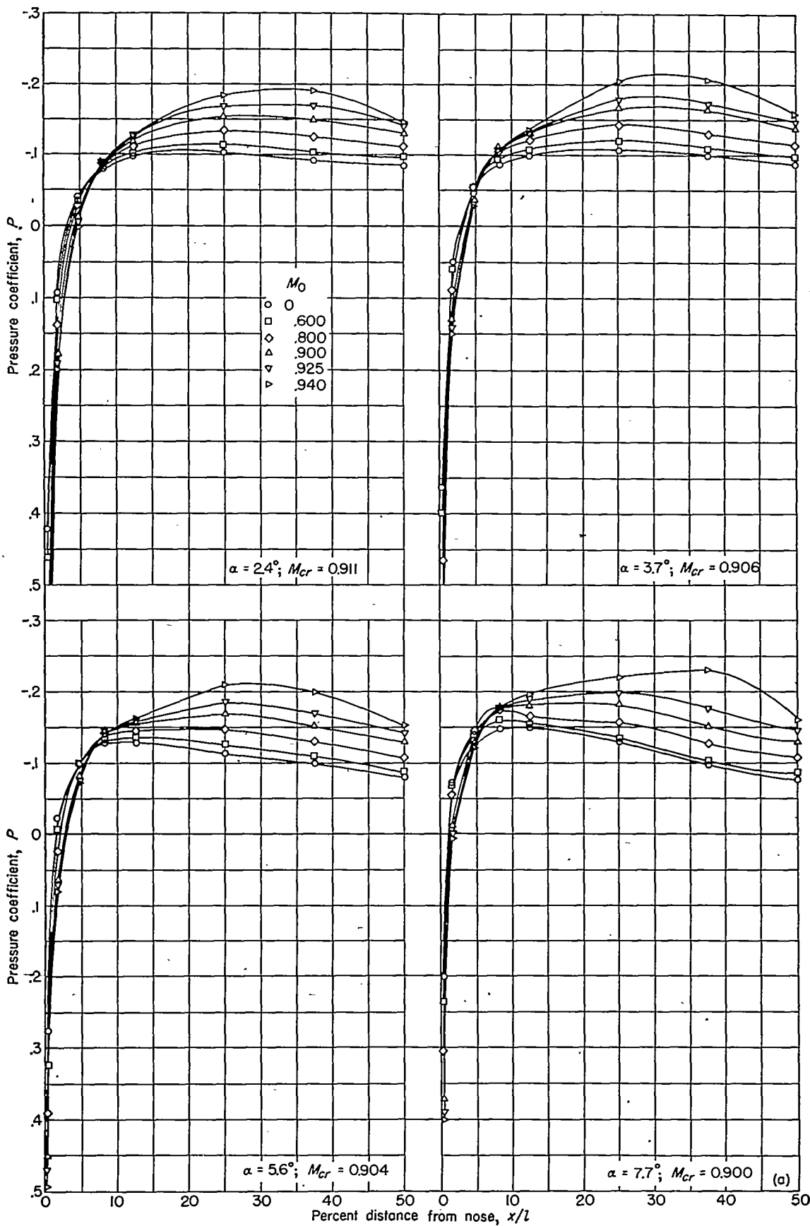
FIGURE 3.—Experimental pressure distributions over a prolate spheroid of fineness ratio 6 at several angles of attack.
