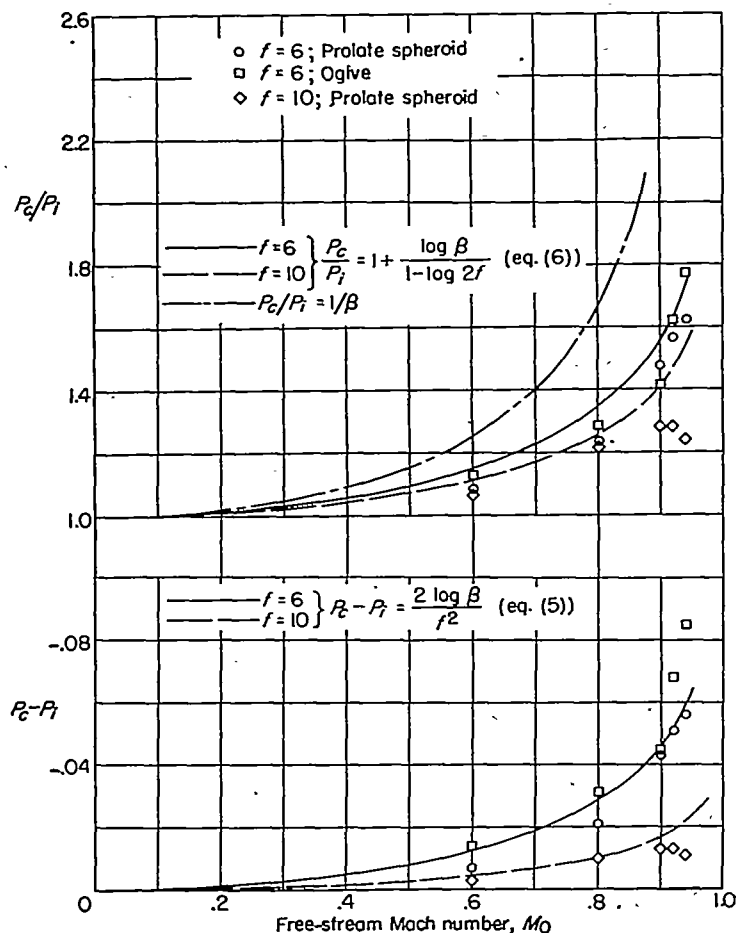
FIGURE 13.—Theoretical compressibility correction functions compared with experimental results. \alpha=0^\circ ; \tau_i=50 percent.
