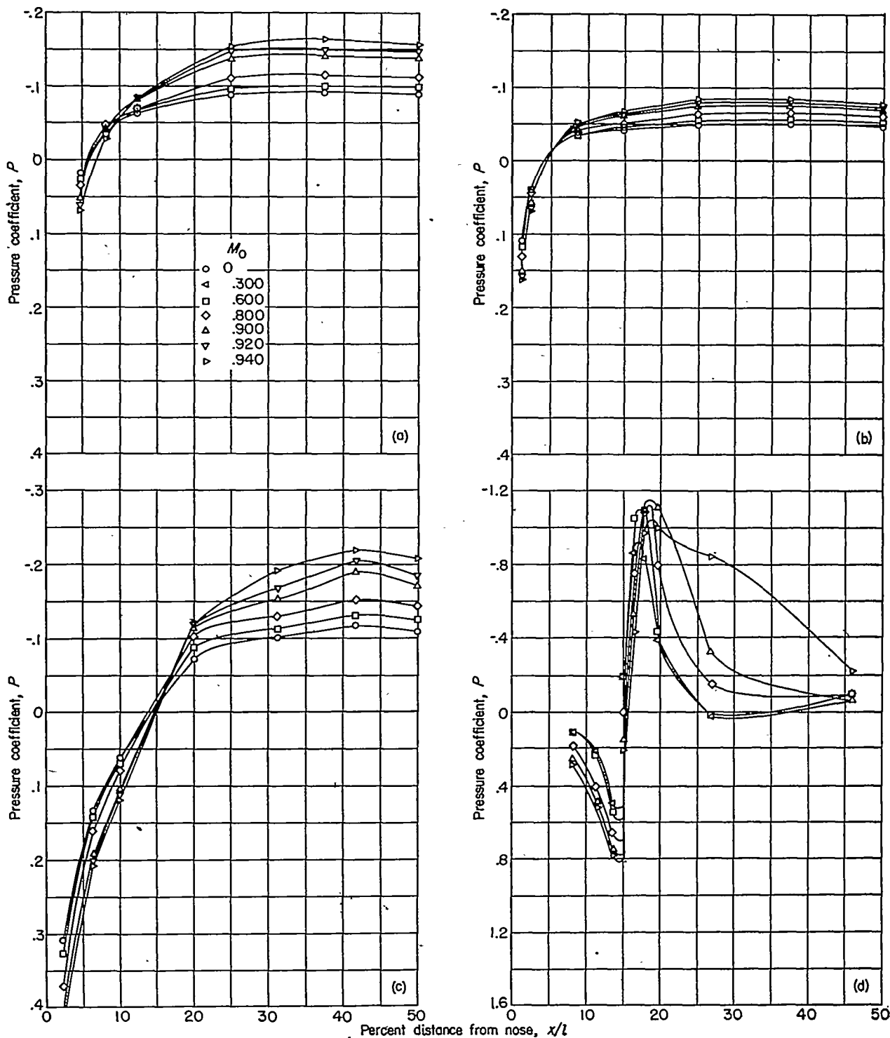
(a) Prolate spheroid; f=6 ; M_{cr}=0.916 . (b) Prolate spheroid; f=10 ; M_{cr}=0.947 . (c) Typical transonic body; M_{cr}=0.898 . (d) Prolate spheroid with annular bump; M_{cr}=0.634 . FIGURE 2.—Experimental pressure distributions over several bodies of revolution at zero angle of attack.
