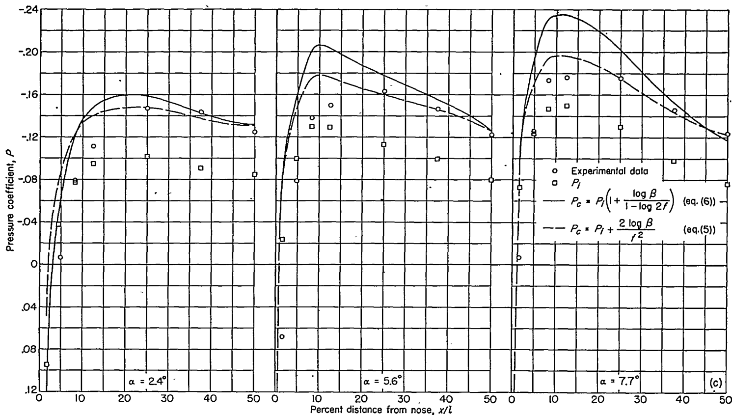
(c) f=6 ; prolate spheroid; M_0=0.900 . FIGURE 14.—Concluded.
