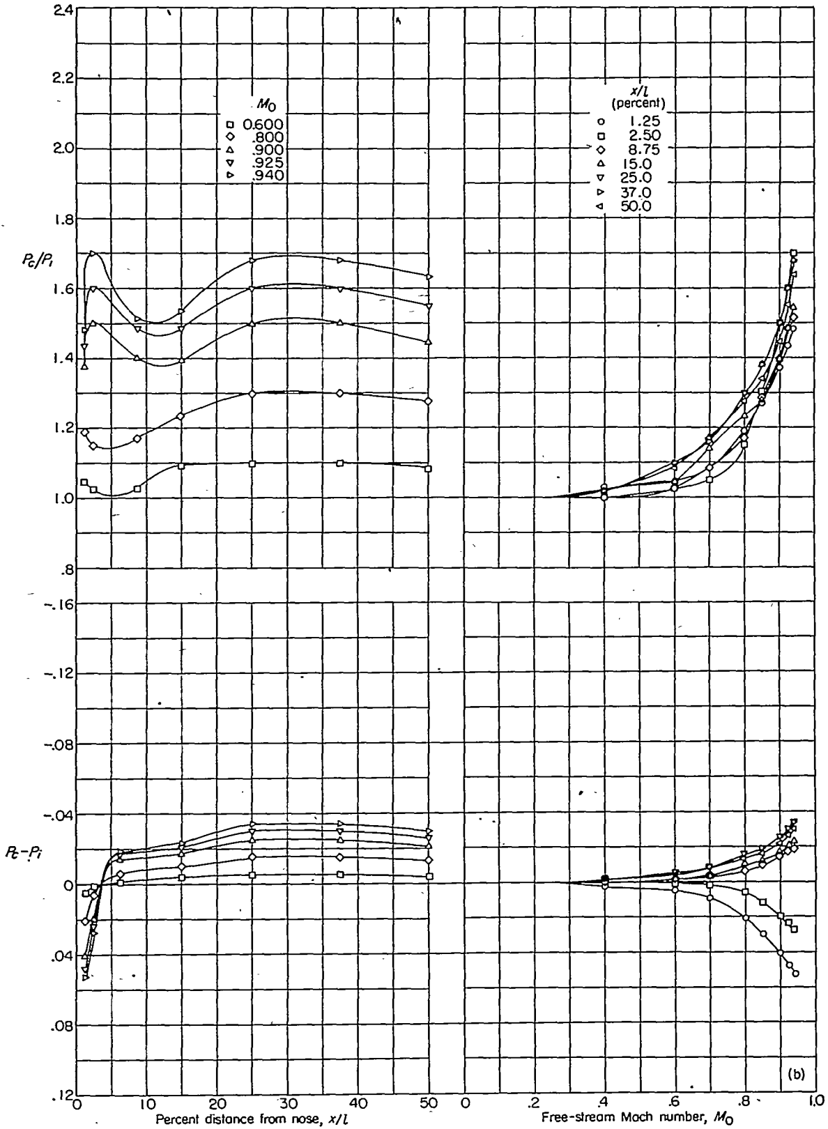
(b) Prolate spheroid; f=10 .
