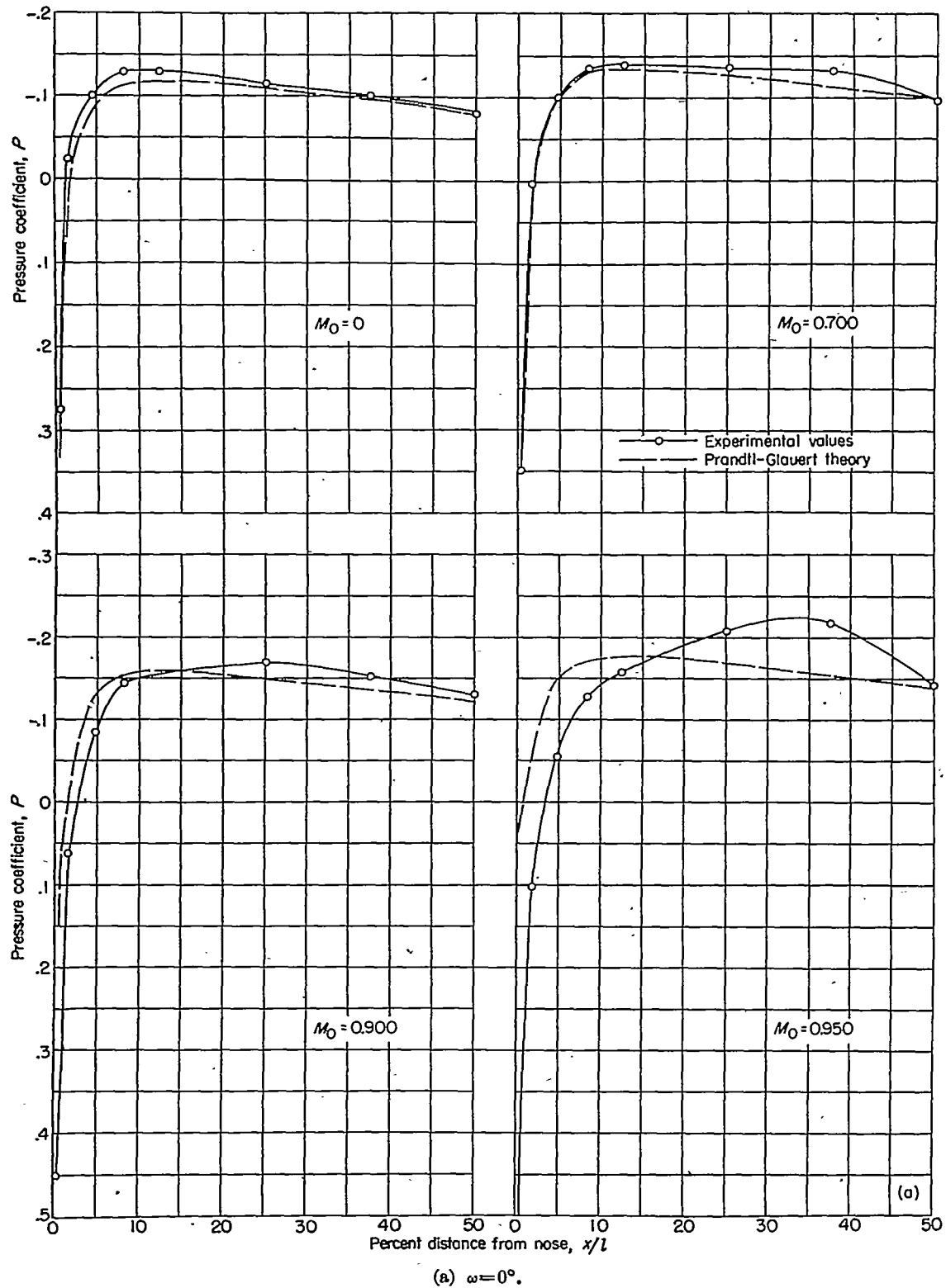
FIGURE 8.—Comparison of experimental and theoretical pressures over a prolate spheroid of fineness ratio 6 at 5.6° angle of attack.
