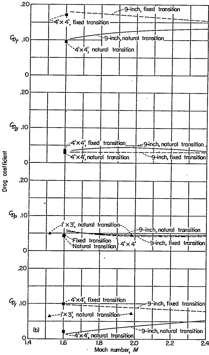
(b) R=8.6 \times 10^6 . FIGURE 12.—Continued.
