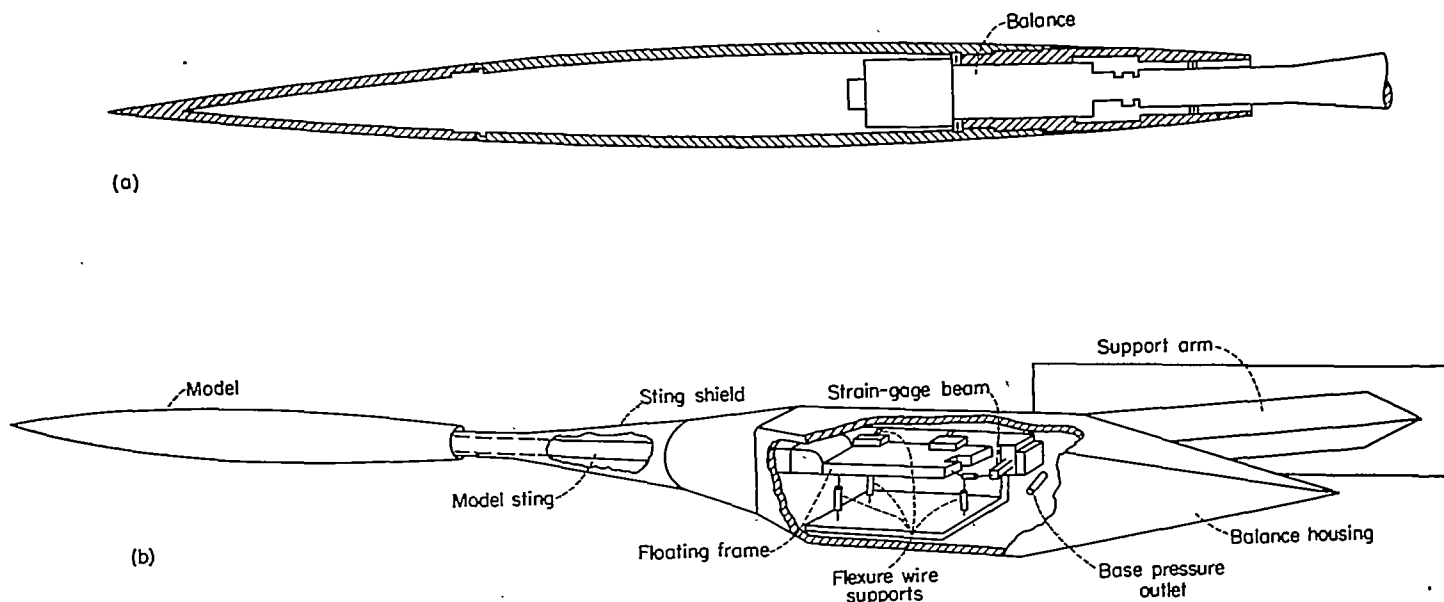
(a) Internal strain-gage balance; 4- by 4-foot tunnel (representative of arrangement in 8- by 6-foot tunnel). (b) Strain-gage balance external to model; 9-inch tunnel (representative of arrangement in 1- by 3-foot tunnel). FIGURE 4.—Sketch of model mounting and internal and external balance systems.
