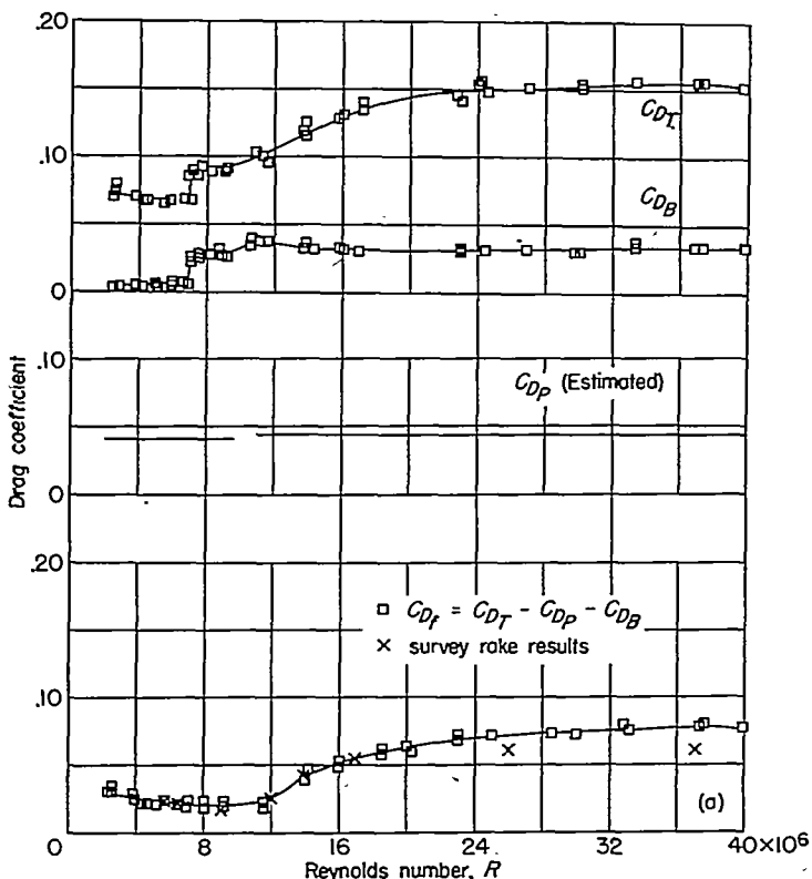
(a) Natural transition.
