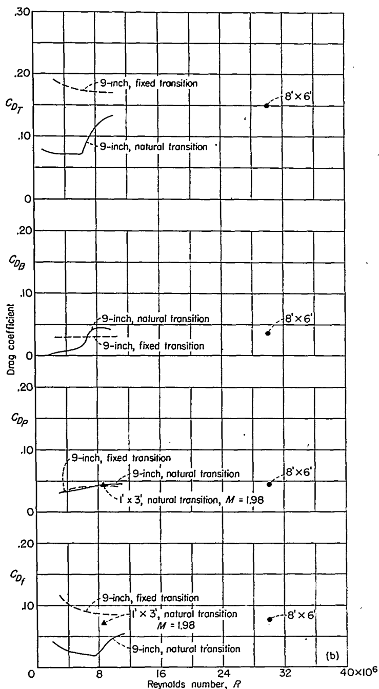
(b) M=1.93 . FIGURE 11.—Concluded.
