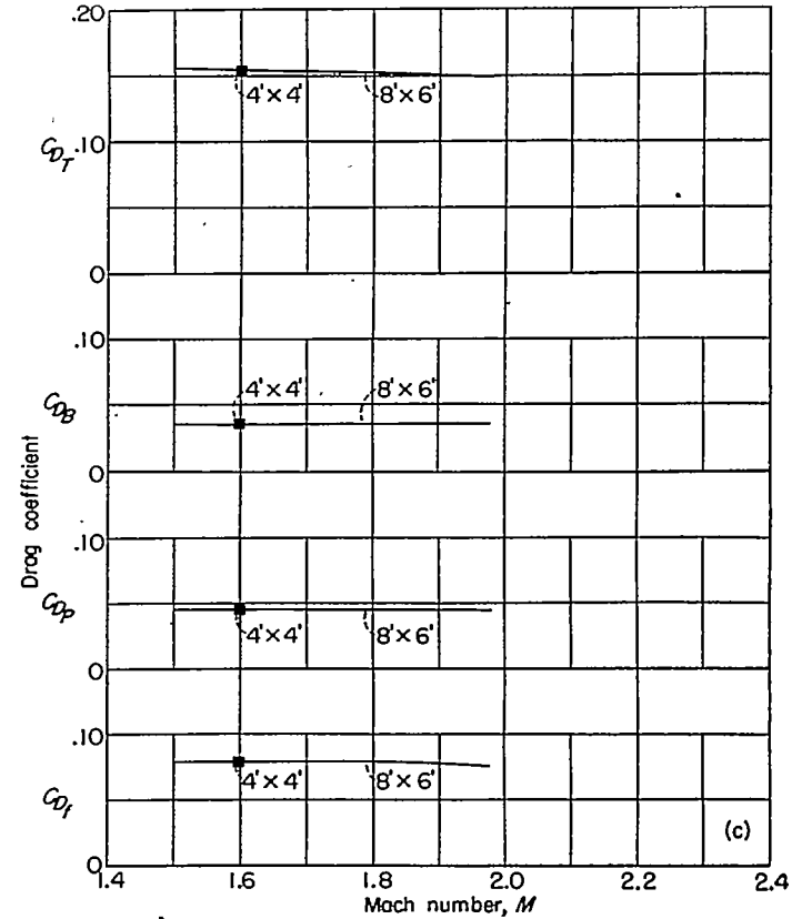
(c) R=30 \times 10^6 . FIGURE 12.—Concluded.
