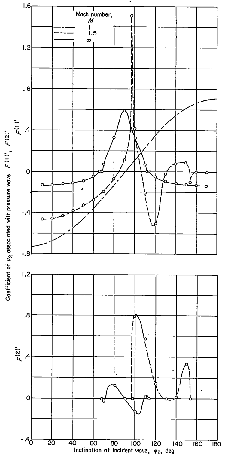
FIGURE 11.—Problem A: coefficient for part of u_2 associated with pressure wave (shock overtaking sound wave).
