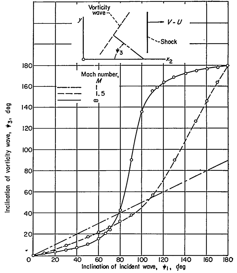
FIGURE 13.—Problem A: inclination of vorticity wave behind shock (shock overtaking sound wave).
