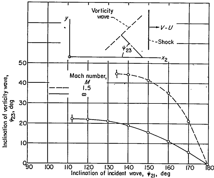
FIGURE 22.—Problem B: inclination of vorticity wave produced behind shock (sound wave overtaking shock).
