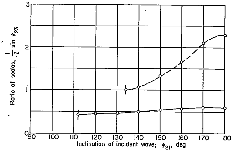
FIGURE 23.—Problem B: ratio of scales of vorticity wave behind shock and incident sound wave (sound wave overtaking shock).
