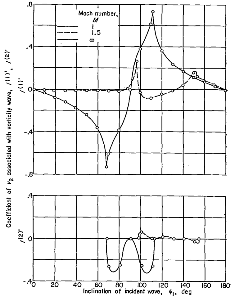
FIGURE 17.—Problem A: coefficients for part of v_2 associated with vorticity wave (shock overtaking sound wave).
