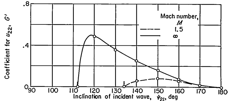
FIGURE 24.—Problem B: coefficient for part of u_{22} associated with vorticity wave (sound wave overtaking shock).
