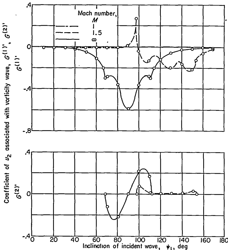
FIGURE 16.—Problem A: coefficient for part of u_2 associated with vorticity wave (shock overtaking sound wave).
