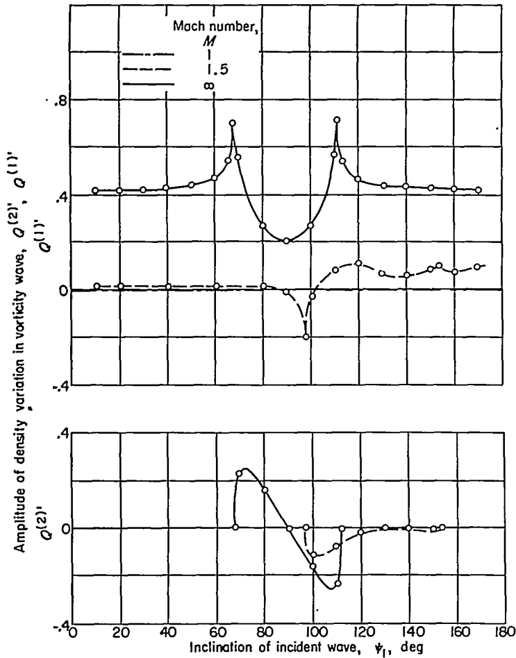
FIGURE 15.—Problem A: amplitude of density variation in vorticity wave behind shock (shock overtaking sound wave).
