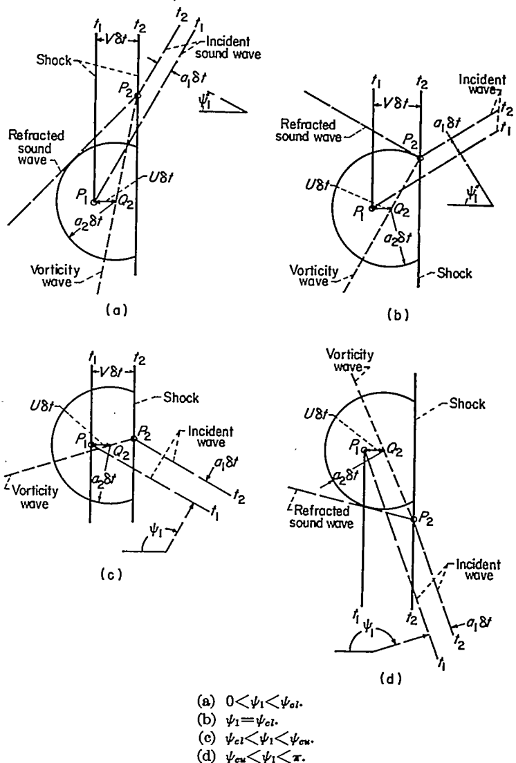
FIGURE 3.—Formation of waves behind shock, because of interaction with sound wave (problem A).
