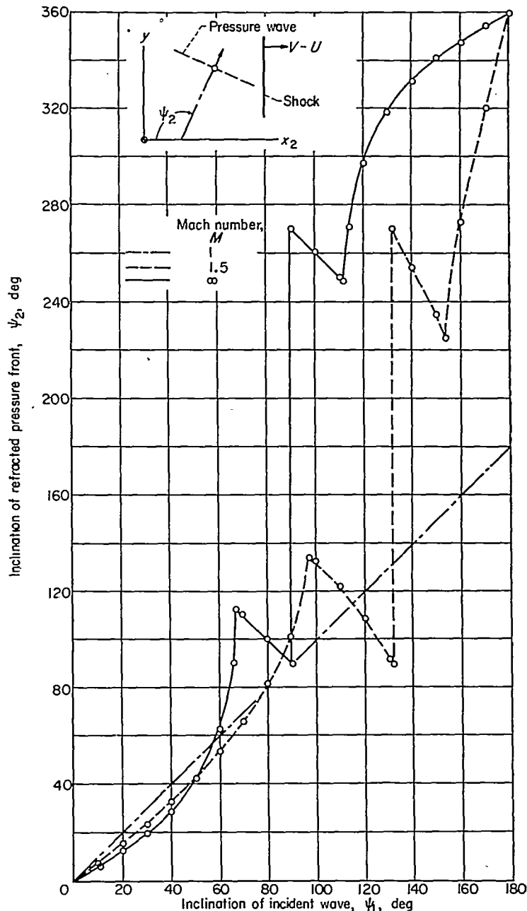
FIGURE 6.—Problem A: inclination of refracted pressure front (shock overtaking sound wave).
