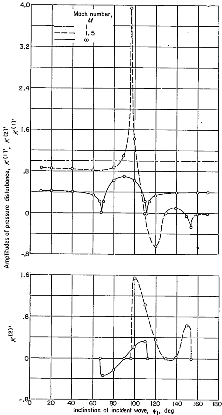
FIGURE 10.—Problem A: amplitudes of pressure disturbance behind shock (shock overtaking sound wave).
