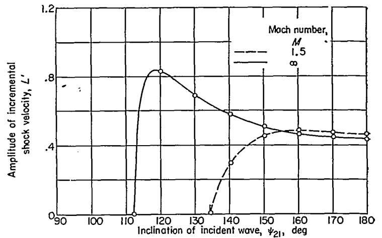
FIGURE 18.—Problem B: shock-front disturbance (sound wave overtaking shock).
