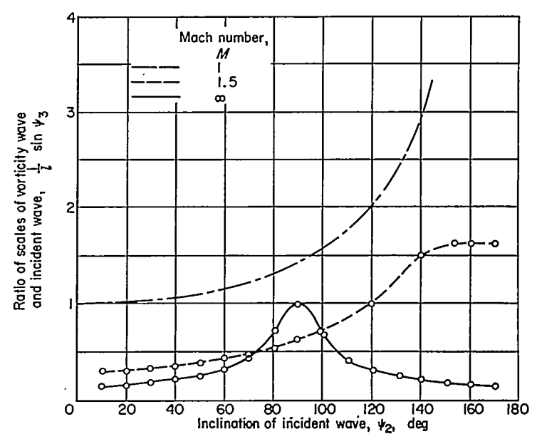
FIGURE 14.—Problem A: ratio of scales of vorticity wave behind shock to that of incident sound wave (shock overtaking sound wave).
