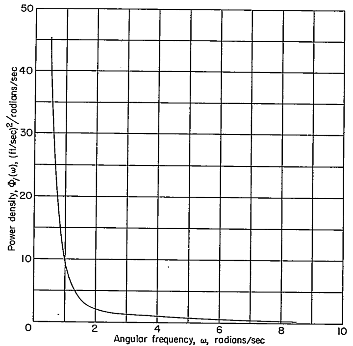
FIGURE 1.—Normalized power-spectral-density function for atmospheric vertical gust velocity \Phi_v(\omega) for airspeed of 300 feet per second.
