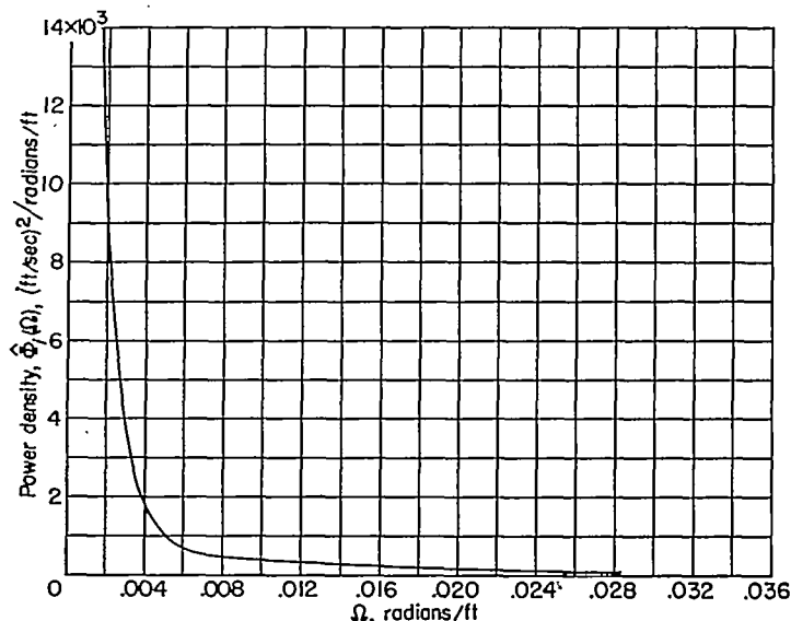
FIGURE 2.—Normalized power-spectral-density function for atmospheric vertical gust velocity \hat{\Phi}_i(\Omega) .
