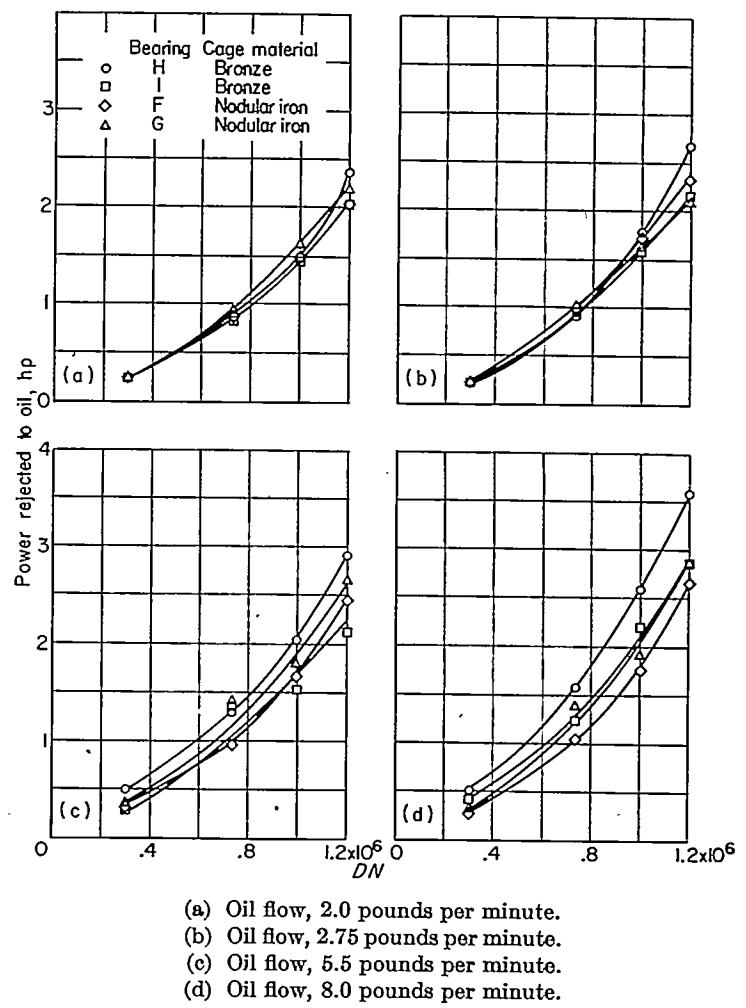
FIGURE 12.—Effect of DN on power rejected to oil in bearings F to I at four oil flows. Load, 368 pounds; oil inlet temperature, 100° F.
