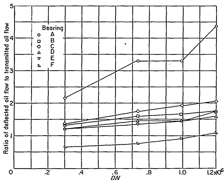
FIGURE 5.—Effect of DN on ratio of deflected to transmitted oil flows for bearings A to F. Load, 368 pounds; oil flow, 2.75 pounds per minute; oil inlet temperature, 100° F.
