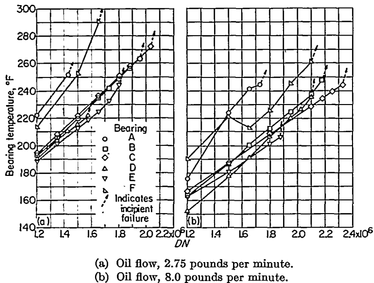
FIGURE 9.—Bearing outer-race maximum temperature as function of DN at very high speeds at two oil flows for bearings A to F. Load, 368 pounds; oil inlet temperature, 100^{\circ} F.
