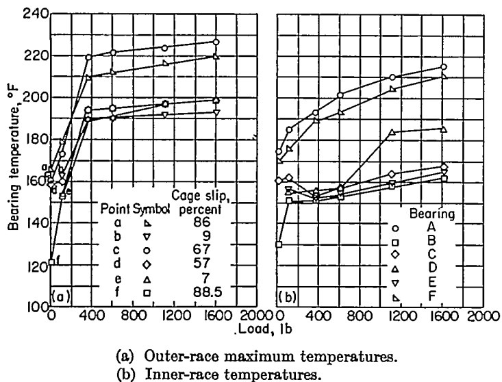
FIGURE 7.—Effect of load on bearing outer-race maximum and inner-race temperatures for bearings A to F. DN , 1.2 \times 10^6 ; oil flow, 2.75 pounds per minute; oil inlet temperature, 100^\circ F.
