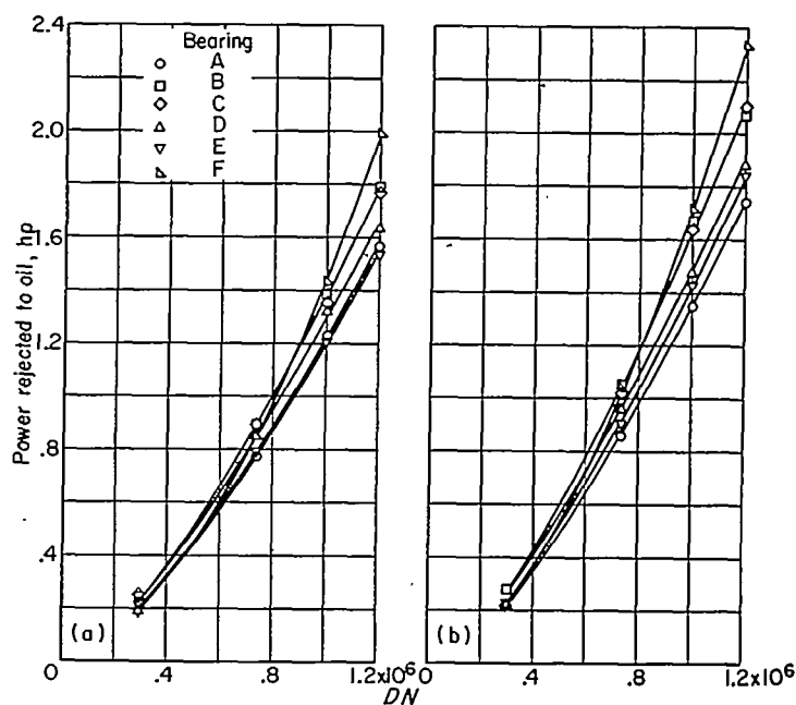
(a) Oil flow, 2.0 pounds per minute. (b) Oil flow, 2.75 pounds per minute.
