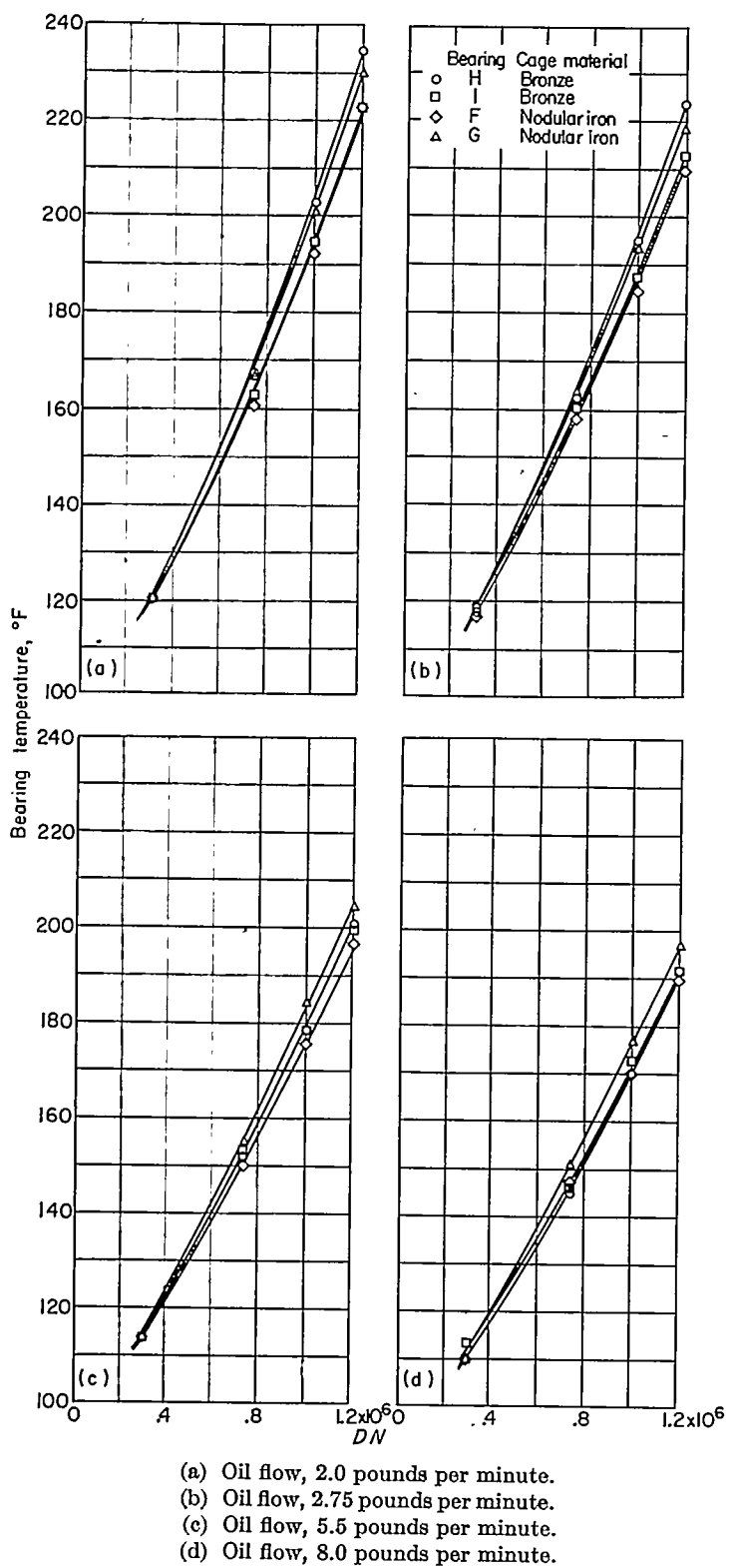
FIGURE 11.—Effect of DN on outer-race maximum temperatures of bearings F to I at four oil flows. Load, 368 pounds; oil inlet temperature, 100° F.
