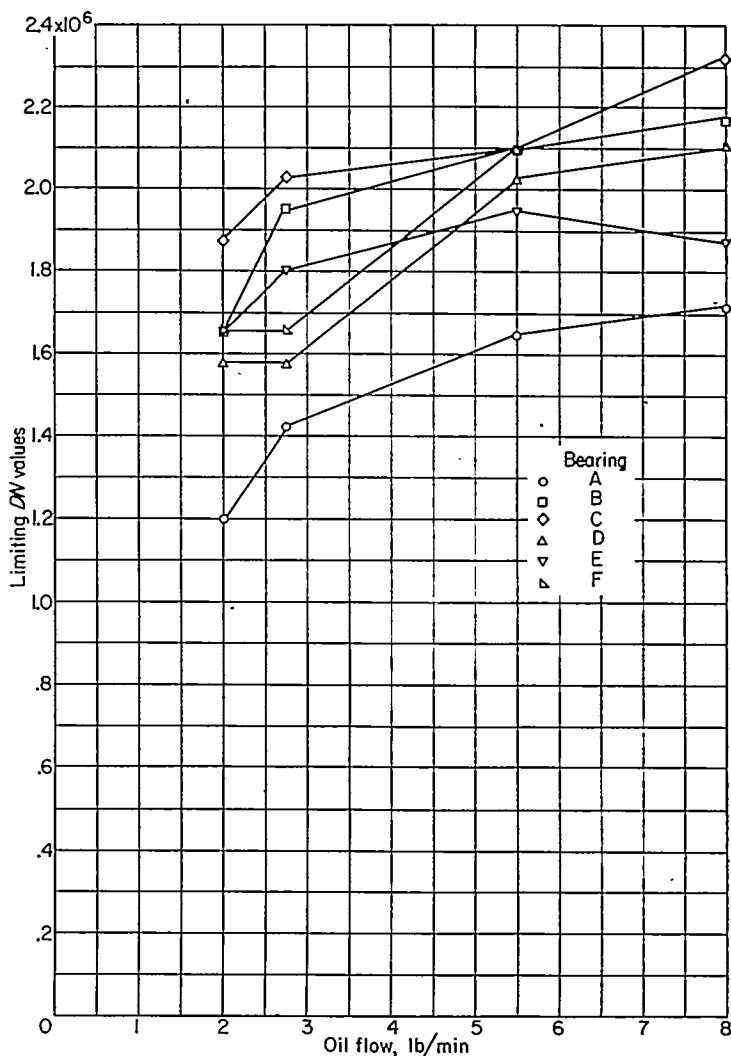
FIGURE 8.—Effect of oil flow on limiting DN value for bearings A to F. Load, 368 pounds; oil inlet temperature, 100^\circ F.
