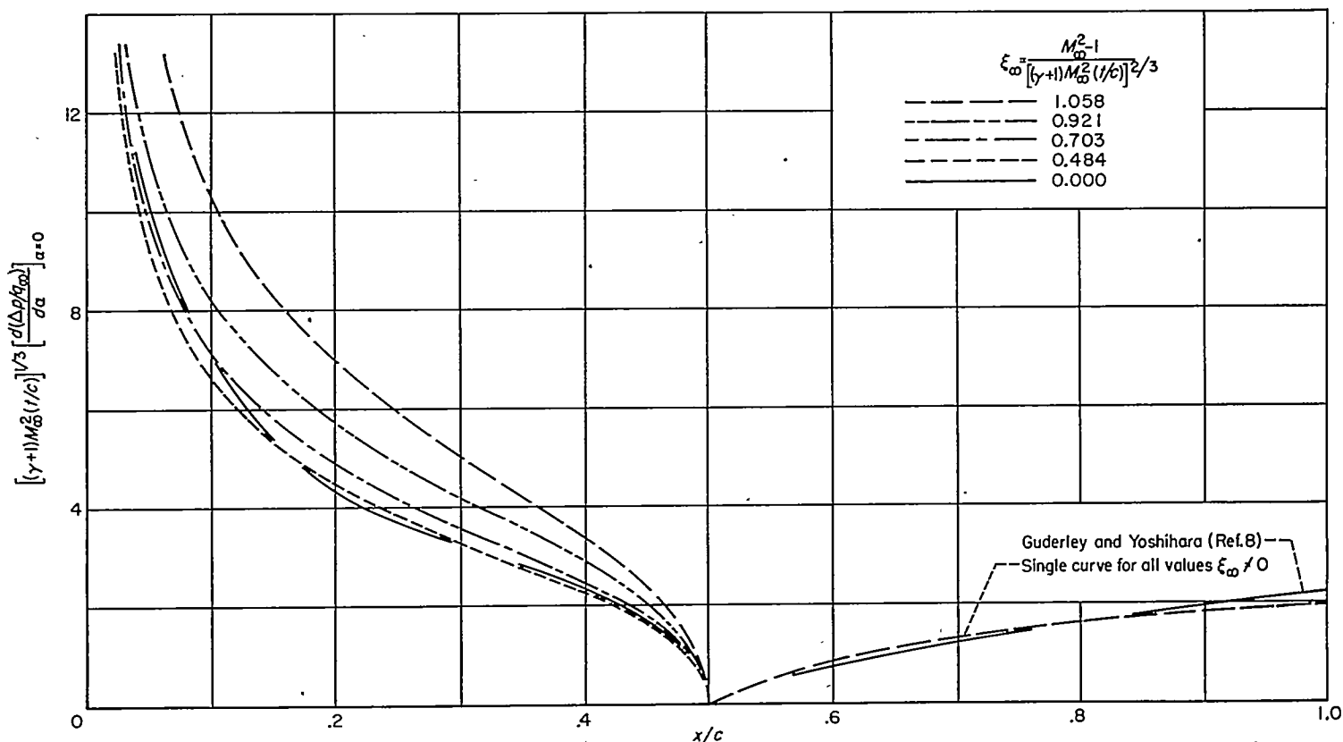
FIGURE 10.—Chordwise distribution of lift.
