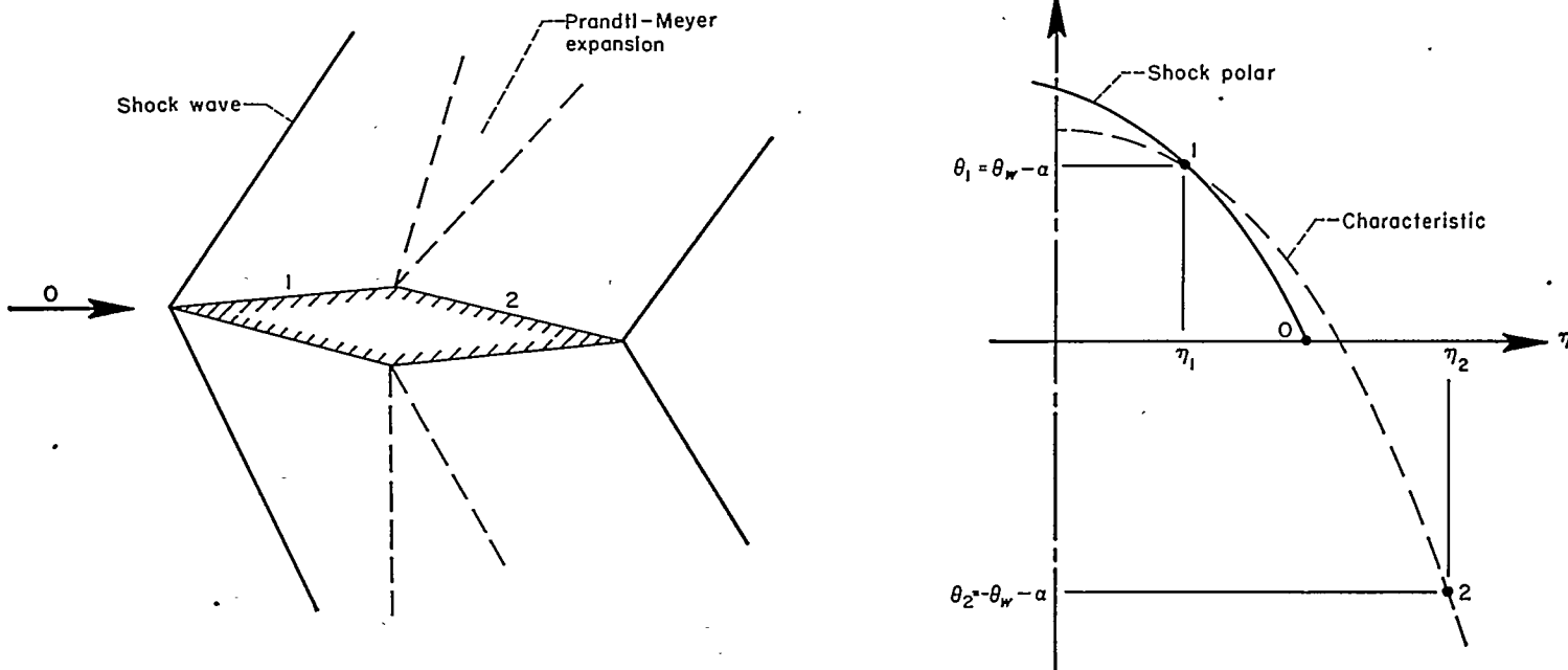
FIGURE 20.—Conditions on airfoil in completely supersonic flow.
