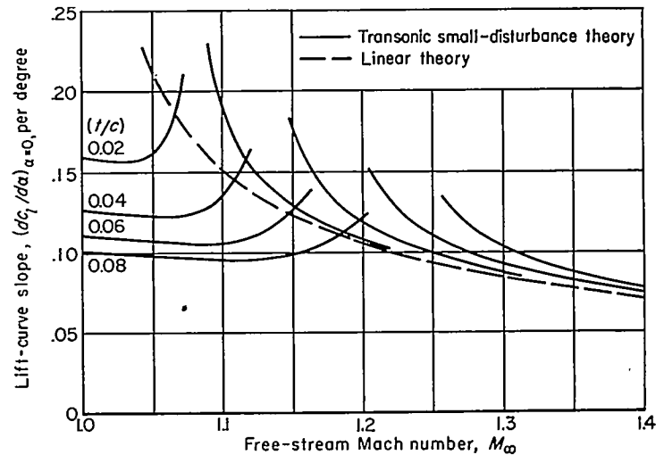
FIGURE 12.—Lift-curve slope as a function of Mach number for several thickness ratios ( \gamma=1.4 )
