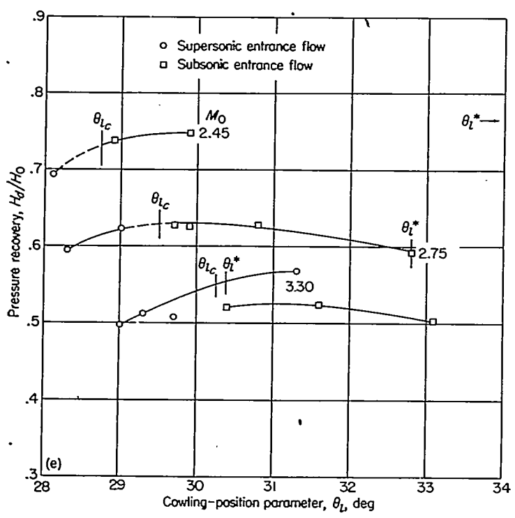
(e) 7°, 10° cowling; D_b/D_l = 0.850 ; \theta_c = 22^\circ . FIGURE 16.—Concluded.
