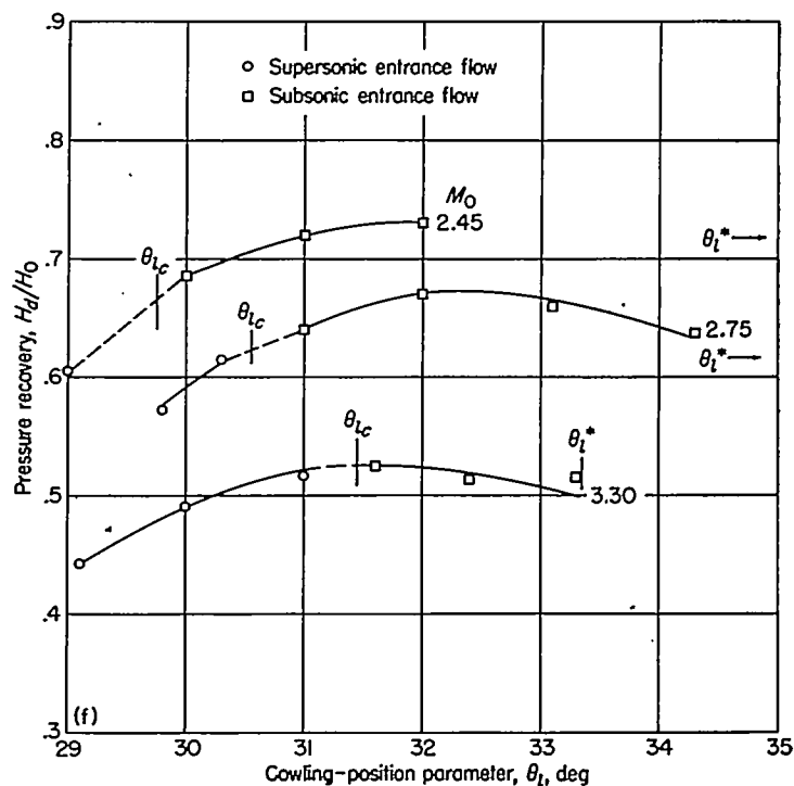
(f) 4^\circ, 7^\circ cowling; D_b/D_t=0.867 ; \theta_c=25^\circ . FIGURE 18.—Concluded.
