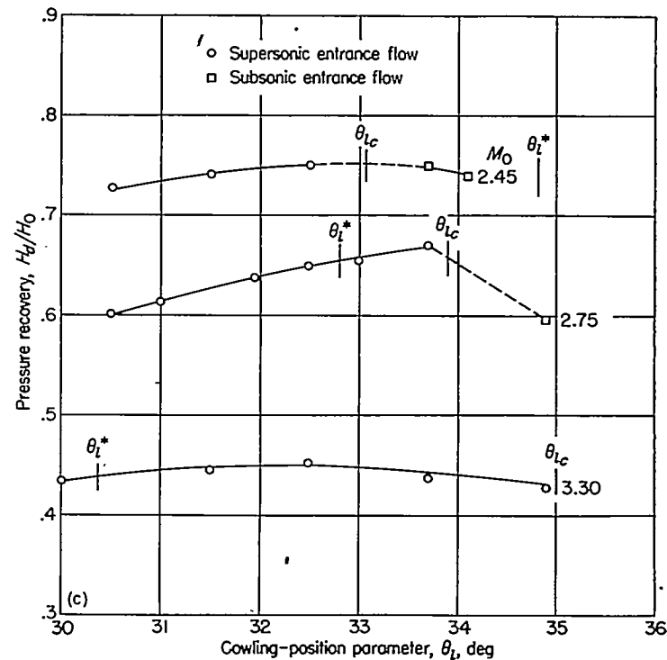
(c) 7°, 10° cowling; D_b/D_i=0.784 ; \theta_c=22^\circ . FIGURE 16.—Continued.
