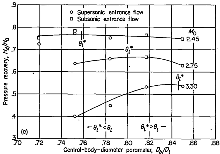
(a) \theta_c=22^\circ ; 7^\circ, 10^\circ cowling.
