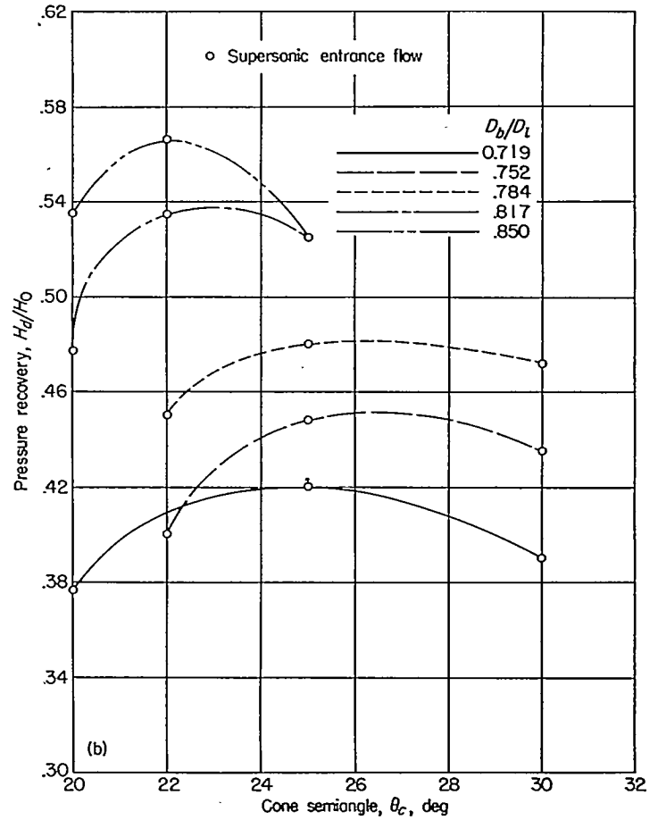
(b) 7°,10° cowling.
