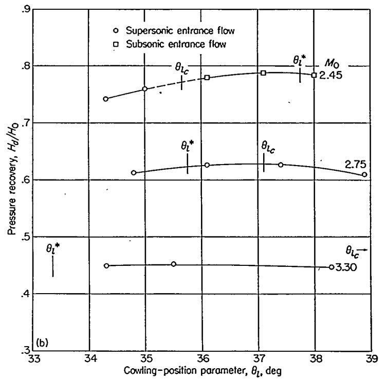
(b) 4^\circ, 7^\circ cowling; D_b/D_i=0.767 ; \theta_c=25^\circ . FIGURE 18.—Continued.
