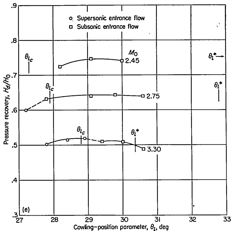
(e) 4°, 7° cowling; D_b/D_i=0.867 ; \theta_c=22^\circ . FIGURE 15.—Concluded.
