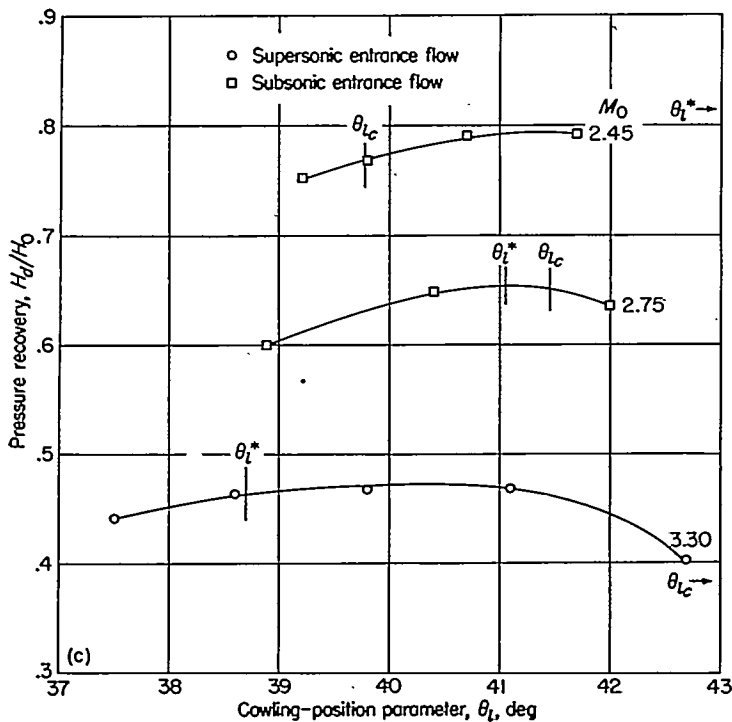
(c) 7°, 10° cowling; D_b/D_i=0.784 ; \theta_c=30^\circ . FIGURE 22.—Concluded.
