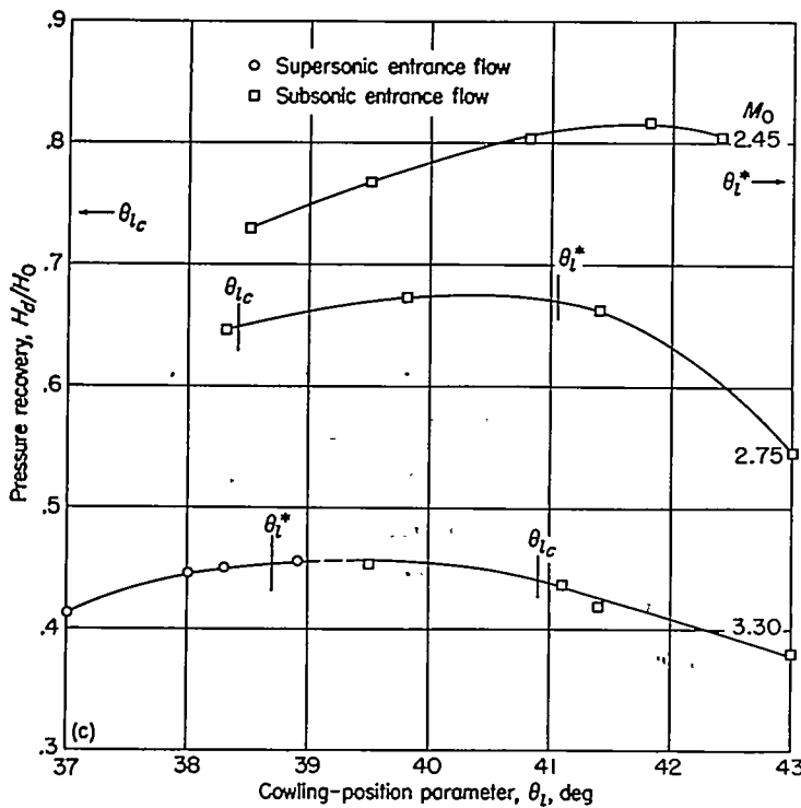
(c) 4°, 7° cowling; D_b/D_t = 0.800 ; \theta_c = 30^\circ . FIGURE 21.—Concluded.
