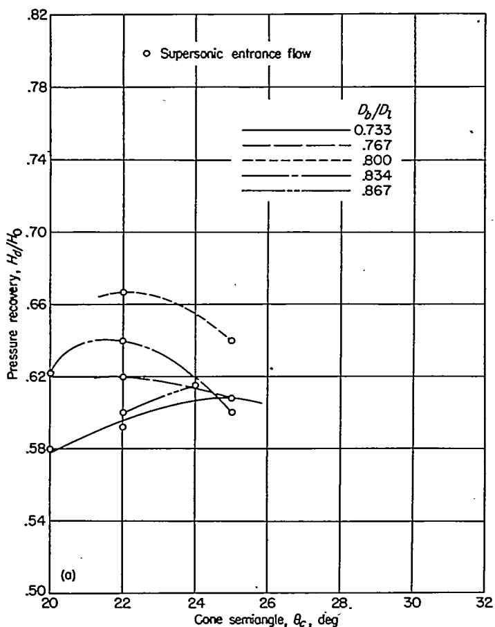
(a) 4°, 7° cowling.
