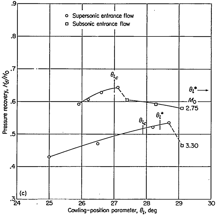
(c) 7°, 10° cowling; D_b/D_t = 0.850 ; \theta_c = 20^\circ . FIGURE 13.—Concluded.
