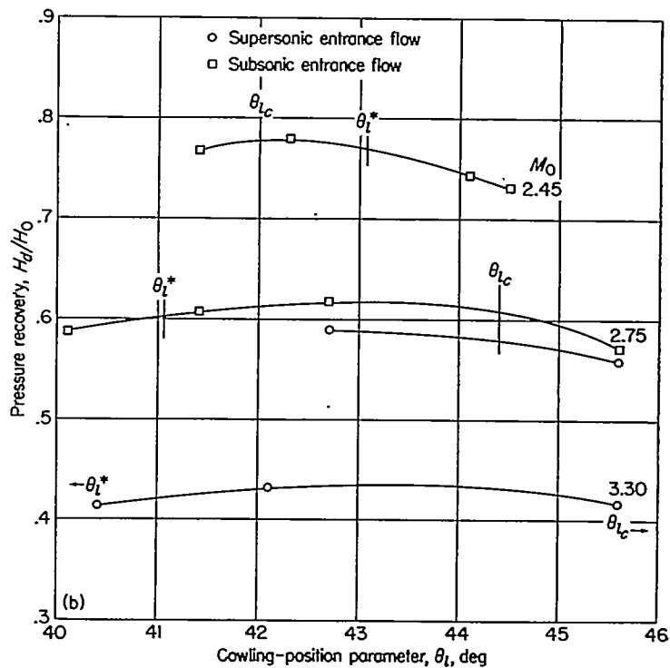
(b) 7°, 10° cowling; D_b/D_t = 0.752 ; \theta_c = 30^\circ . FIGURE 22.—Continued.
