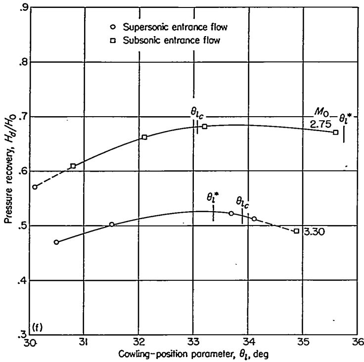
(f) 7^\circ, 10^\circ cowling; D_b/D_i=0.850 ; \theta_c=25^\circ . FIGURE 19.—Concluded.
