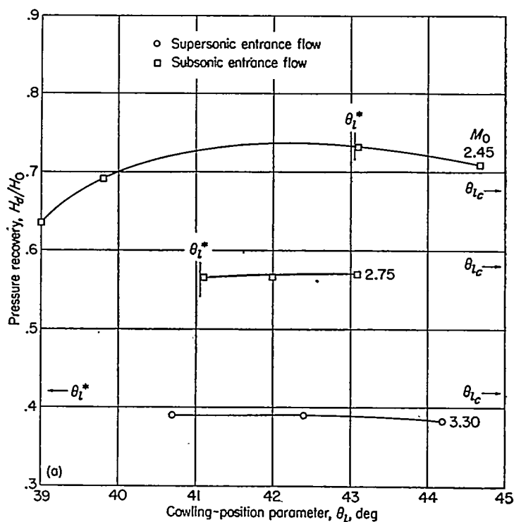
(a) 7°, 10° cowling; D_b/D_t = 0.719 ; \theta_c = 30^\circ .
