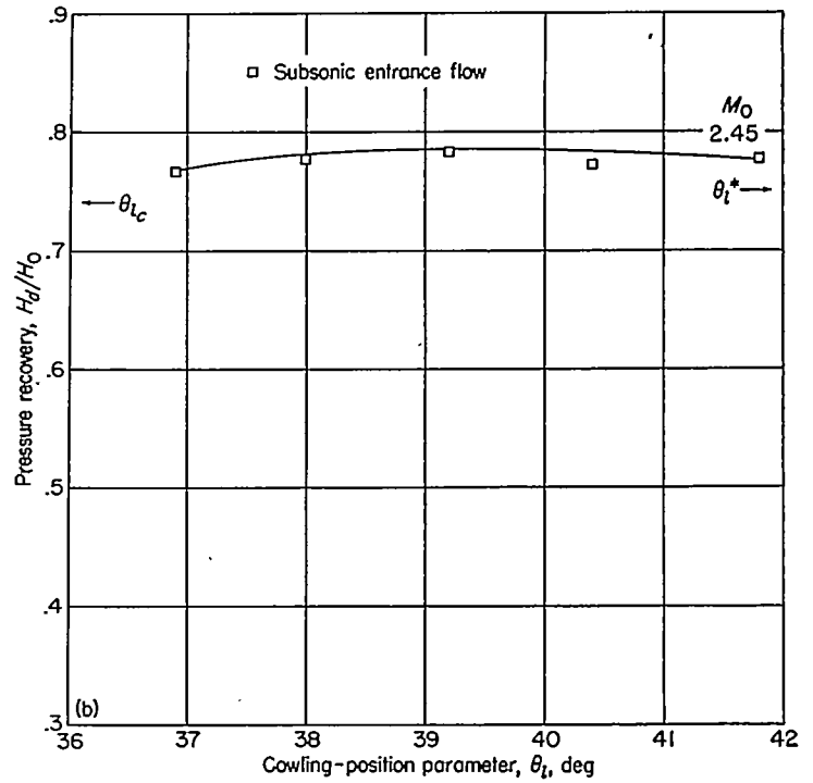
(b) 0^\circ, 2^\circ cowling; D_b/D_i=0.800 ; \theta_c=30^\circ . FIGURE 20.—Concluded.
