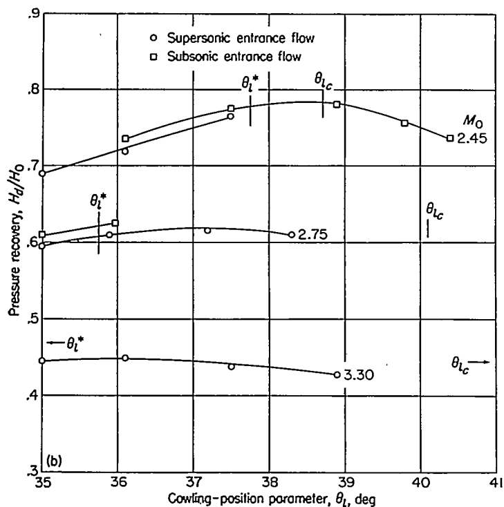
(b) 7^\circ, 10^\circ cowling; D_b/D_i=0.752 ; \theta_c=25^\circ . FIGURE 19.—Continued.
