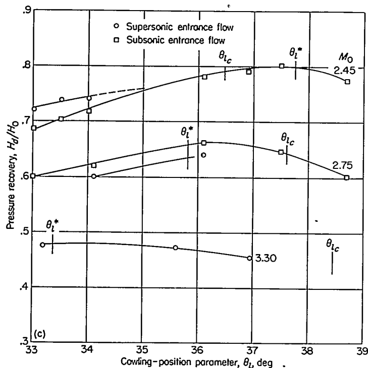
(c) 7^\circ, 10^\circ cowling; D_b/D_i=0.784 ; \theta_c=25^\circ . FIGURE 19.—Continued.
