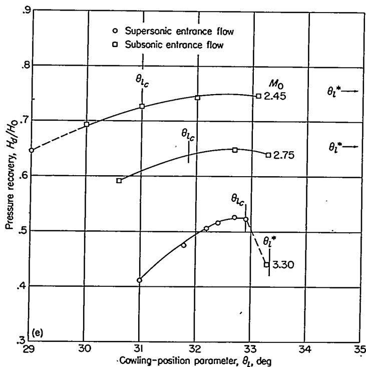
(e) 4^\circ, 7^\circ cowling; D_b/D_t=0.847 ; \theta_c=25^\circ . FIGURE 18.—Continued.
