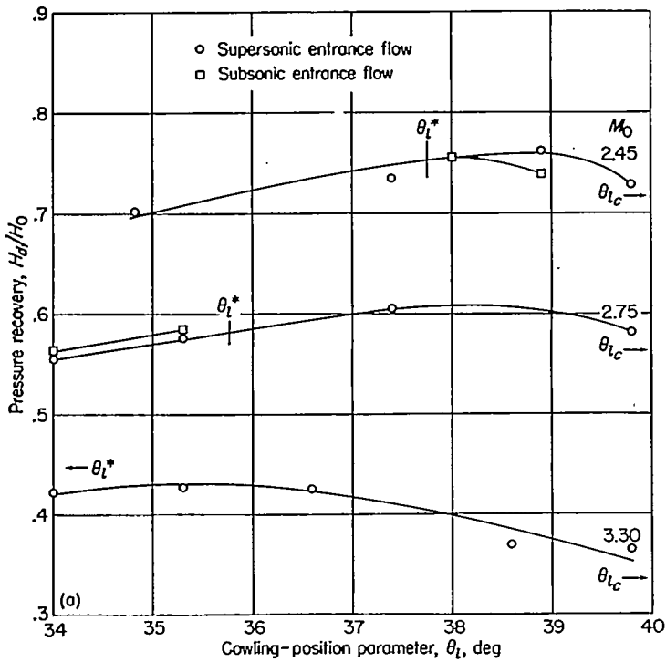
(a) 4^\circ, 7^\circ cowling; D_b/D_i=0.733 ; \theta_c=25^\circ . FIGURE 18.—Pressure recovery as a function of cowling-position parameter for \theta_c=25^\circ and 4^\circ, 7^\circ cowling.
