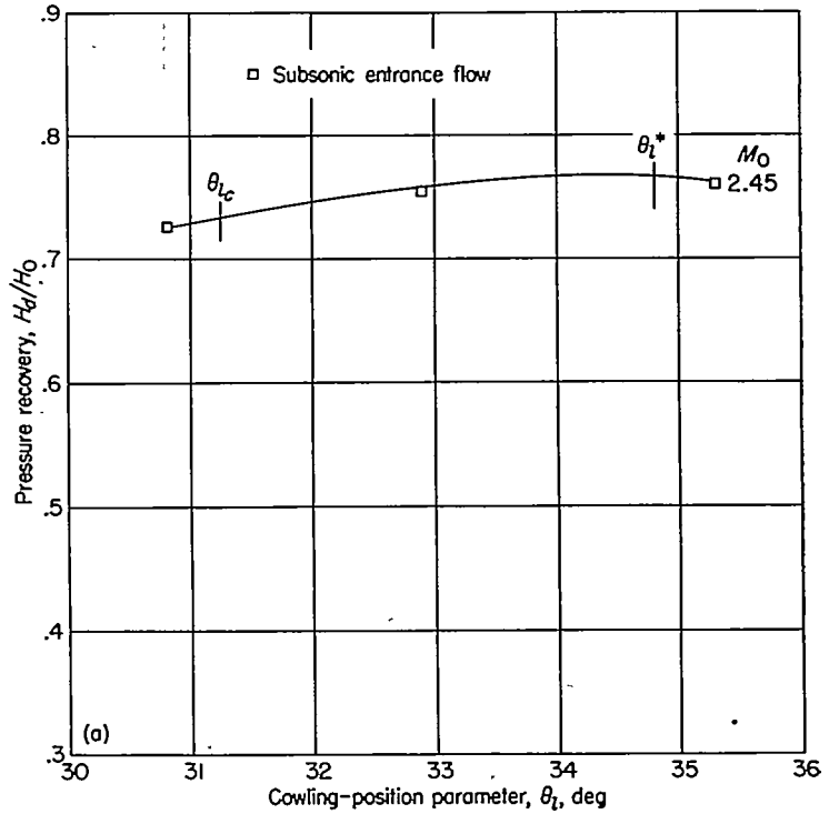
(a) 0°, 2° cowling; D_b/D_t = 0.733 ; \theta_c = 22^\circ . FIGURE 14.—Pressure recovery as a function of cowling-position parameter for \theta_c = 22^\circ and 0°, 2° cowling at M_0 = 2.45 .
