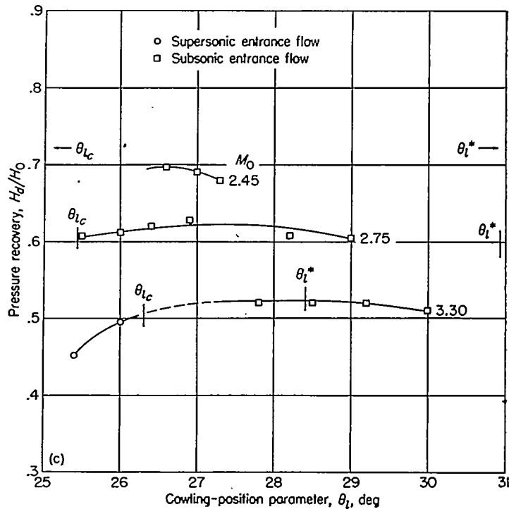
(c) 4°, 7° cowling; D_b/D_t=0.867 ; \theta_o=20^\circ .
