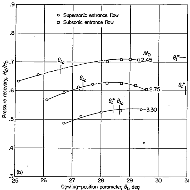
(b) 4°, 7° cowling; D_b/D_t=0.834 ; \theta_o=20^\circ .
