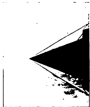
(f) \theta_L = 31.4^\circ ; M = 3.30 ; \theta_c = 20^\circ ; 4^\circ, 7^\circ cowling.
