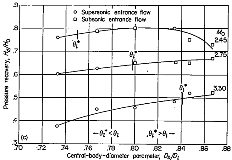
(c) \theta_c=25^\circ; 4^\circ, 7^\circ cowling. FIGURE 31.—Continued.
