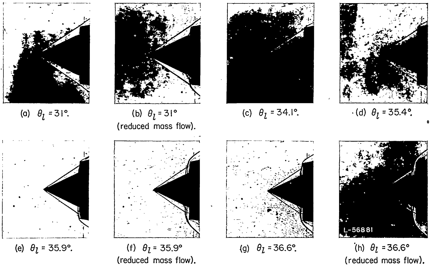
FIGURE 36.—Shadowgraphs of inlet configuration for \theta_c=25^\circ , the 7^\circ, 10^\circ cowling, and D_b/D_1=0.817 for different values of \theta_i for M_0=3.30 . (The corresponding values of pressure recovery are give in ing. 19 (d).)
