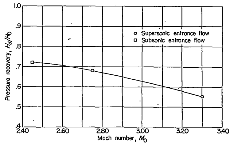
FIGURE 33.—Typical variation of pressure recovery with Mach number. \theta_c=22^\circ ; 4^\circ, 7^\circ cowling; \theta_t=32.2^\circ ; and D_b/D_t=0.834 .
