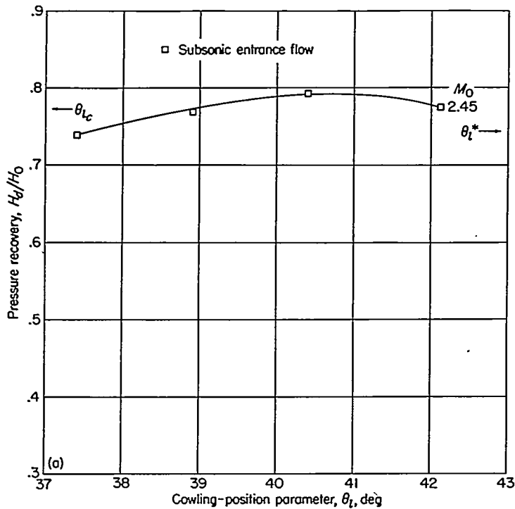
(a) 0^\circ, 2^\circ cowling; D_b/D_i=0.767 ; \theta_c=30^\circ .
