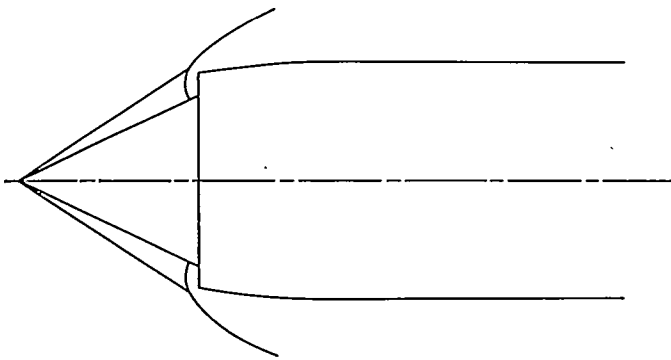
FIGURE 5.—Flow configuration of an inlet operating below the design Mach number.
