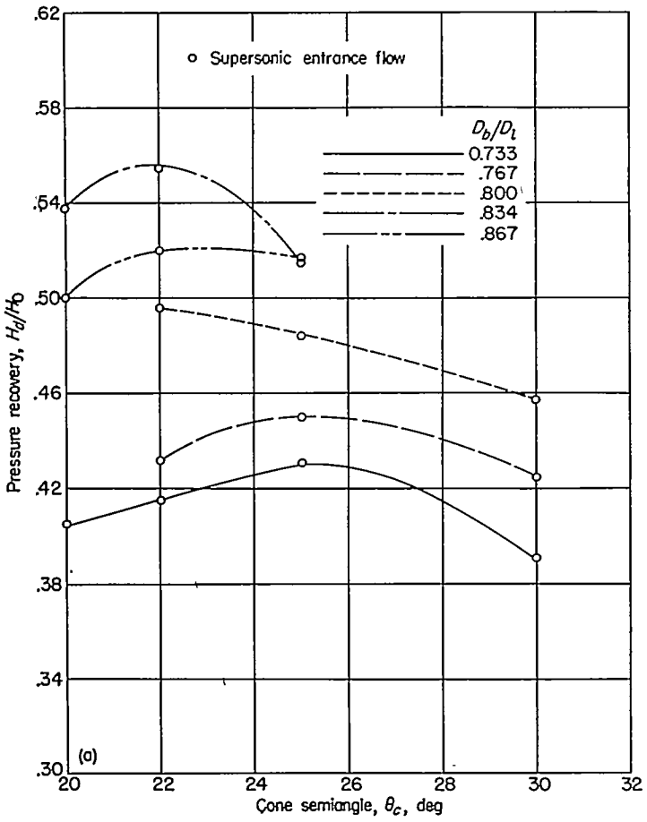
(a) 4°,7° cowling.
