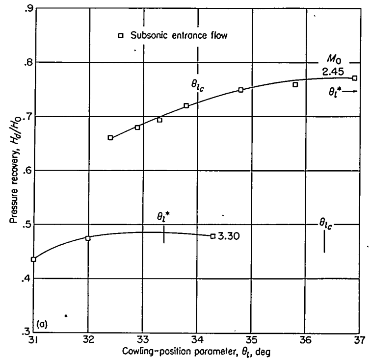
(a) 0°, 2° cowling; D_b/D_l = 0.733 ; \theta_c = 25^\circ . FIGURE 17.—Pressure recovery as a function of cowling-position parameter for \theta_c = 25^\circ and 0°, 2° cowling.
