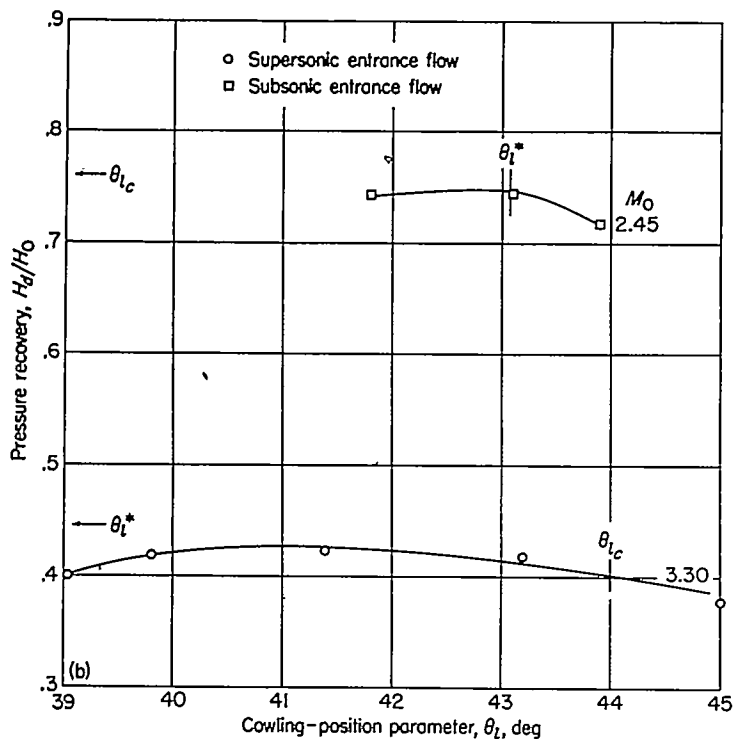
(b) 4°, 7° cowling; D_b/D_t = 0.767 ; \theta_c = 30^\circ . FIGURE 21.—Continued.
