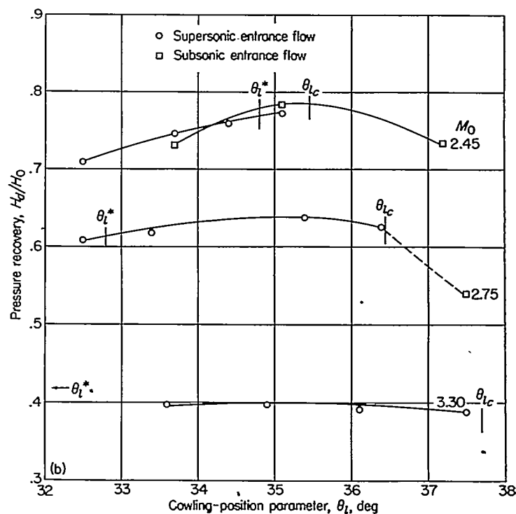
(b) 7°, 10° cowling; D_b/D_i=0.752 ; \theta_c=22^\circ . FIGURE 16.—Continued.
