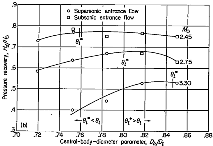
(b) \theta_c=22^\circ; 7^\circ, 10^\circ cowling. FIGURE 30.—Continued.
