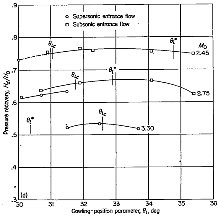
(d) 7°, 10° cowling; D_b/D_l = 0.817 ; \theta_c = 22^\circ . FIGURE 16.—Continued.
