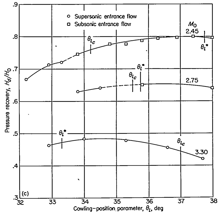
(c) 4^\circ, 7^\circ cowling; D_b/D_i=0.800 ; \theta_c=25^\circ . FIGURE 18.—Continued.
