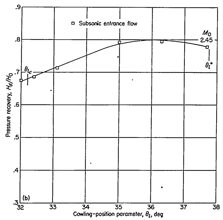
(b) 0°, 2° cowling; D_b/D_l = 0.767 ; \theta_c = 25^\circ . FIGURE 17.—Continued.
