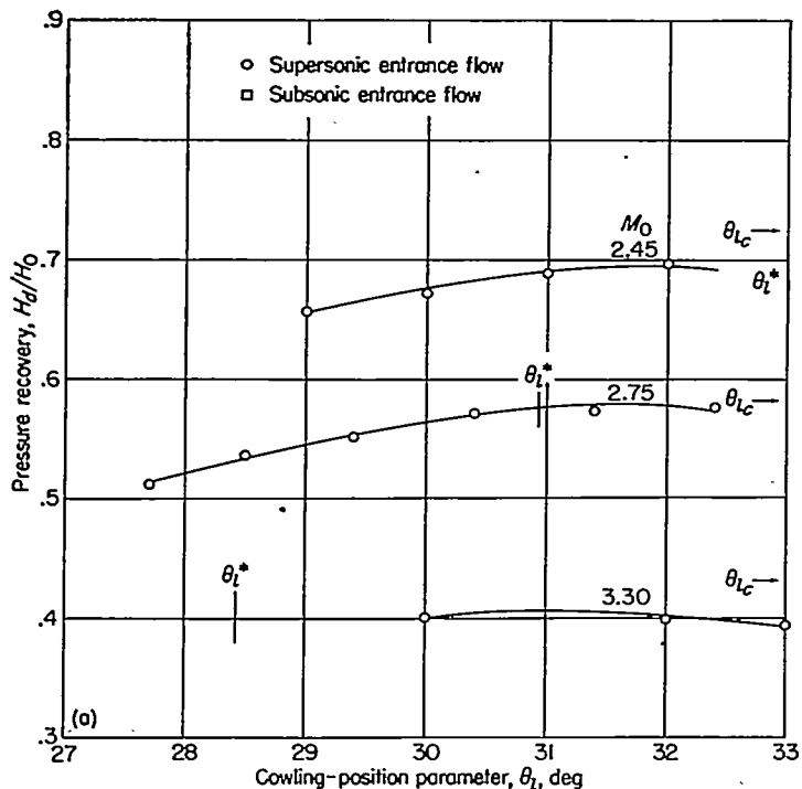
(a) 4°, 7° cowling; D_b/D_t=0.733 ; \theta_o=20^\circ .
