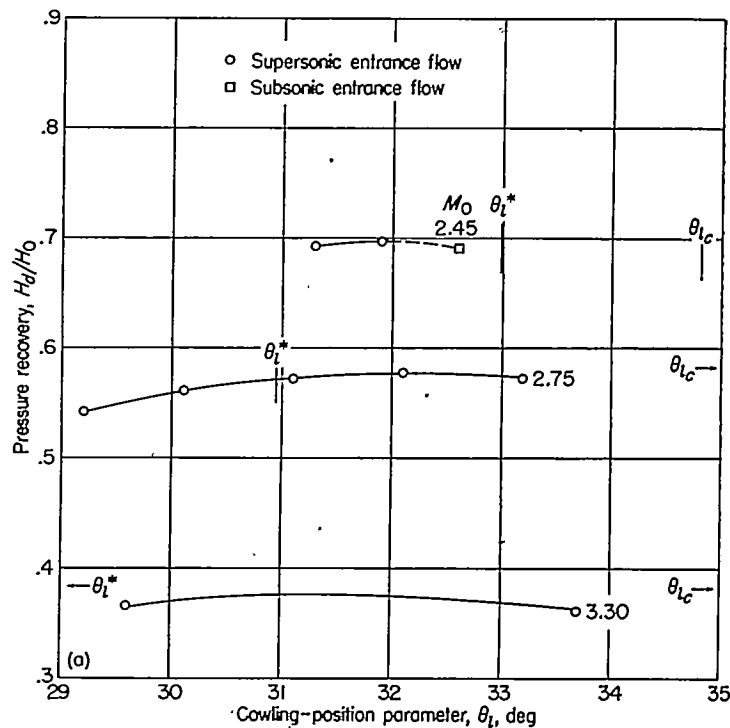
(a) 7°, 10° cowling; D_b/D_t=0.719 ; \theta_o=20^\circ .
