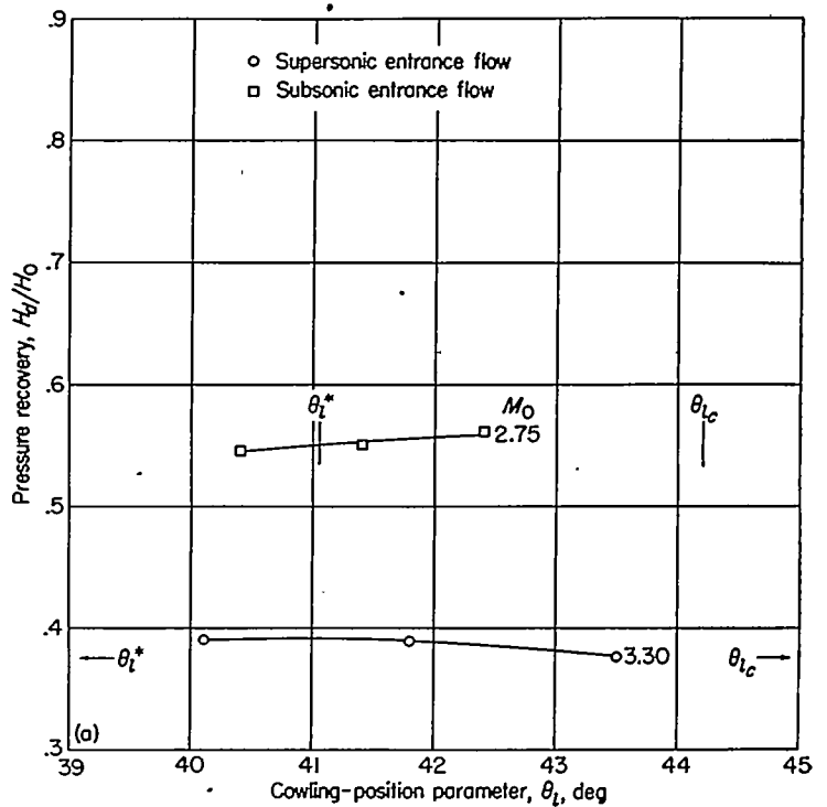
(a) 4^\circ, 7^\circ cowling; D_b/D_i=0.733 ; \theta_c=30^\circ .
