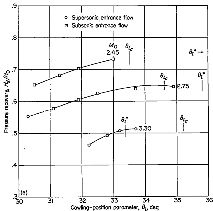
(e) 7^\circ, 10^\circ cowling; D_b/D_i=0.830 ; \theta_c=25^\circ . FIGURE 19.—Continued.
