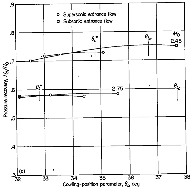
(a) 7°, 10° cowling; D_b/D_i=0.719 ; \theta_c=22^\circ .
