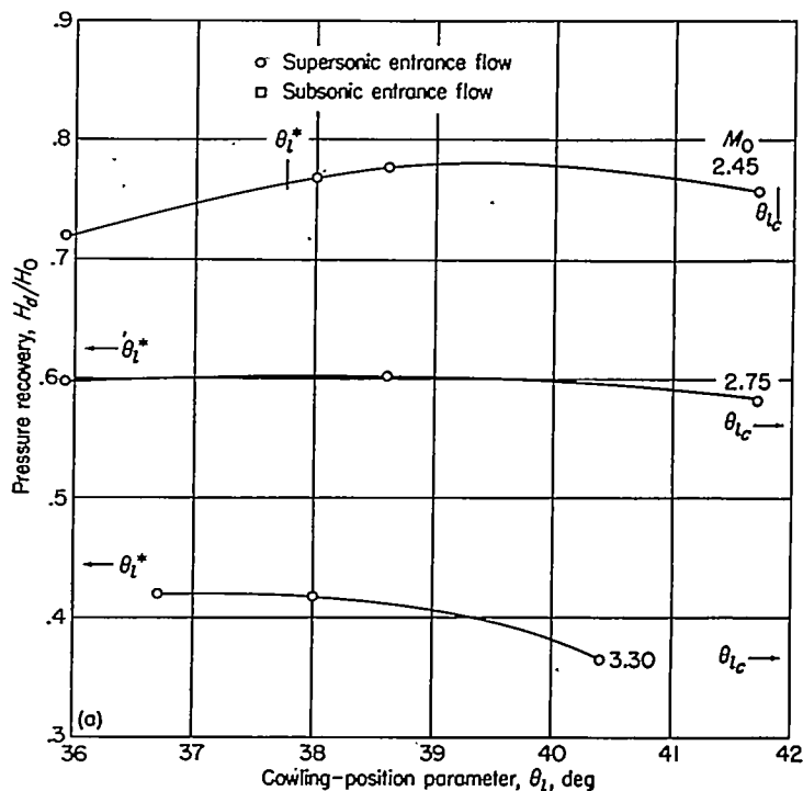
(a) 7^\circ, 10^\circ cowling; D_b/D_t=0.719 ; \theta_c=25^\circ . FIGURE 19.—Pressure recovery as a function of cowling-position parameter for \theta_c=25^\circ and 7^\circ, 10^\circ cowling at different Mach numbers.
