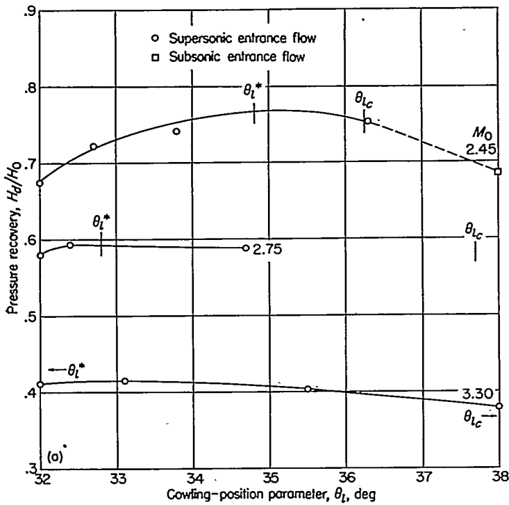
FIGURE 15.—Pressure recovery as a function of cowling-position parameter for \theta_c=22^\circ and 4^\circ, 7^\circ cowling at different Mach numbers.
