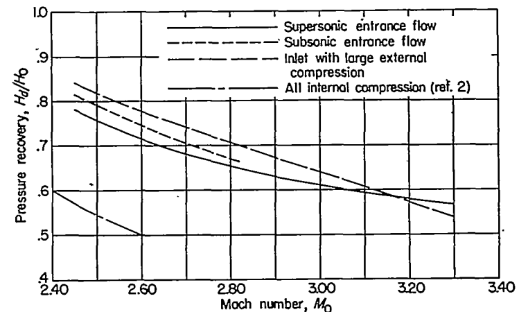
FIGURE 34.—Optimum pressure recovery obtained from all configurations tested.
