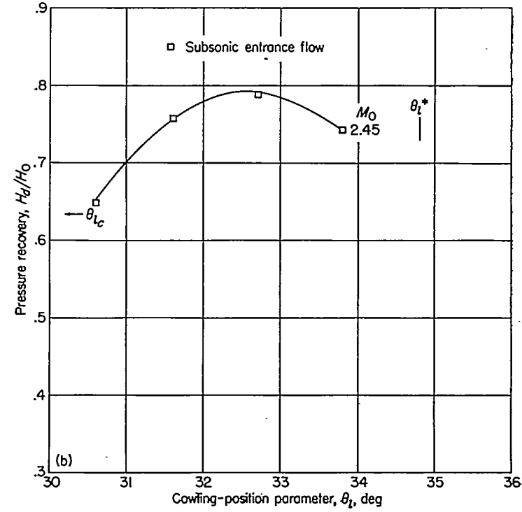
(b) 0°, 2° cowling; D_b/D_t = 0.767 ; \theta_c = 22^\circ . FIGURE 14.—Concluded.
