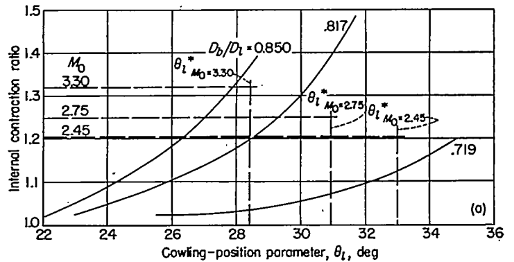
(a) \theta_c = 20^\circ .
