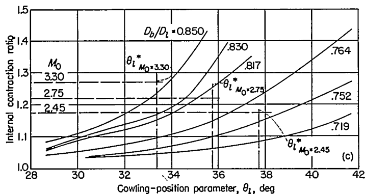
(c) \theta_c = 25^\circ .
