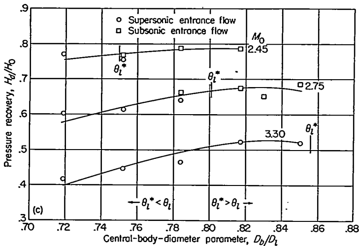
(c) \theta_c=25^\circ; 7^\circ, 10^\circ cowling. FIGURE 30.—Continued.
