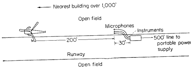
FIGURE 28.—Engine-test arrangement.
