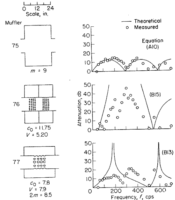
FIGURE 17.—Mufflers for large-diameter (12 in.) exhaust pipes.
