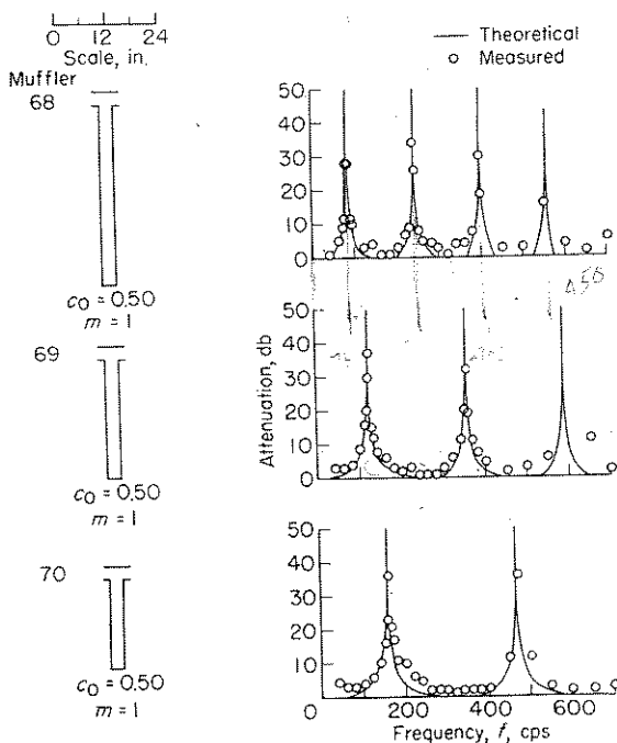
FIGURE 15.—Sid-branch tubes with same diameter as exhaust pipe. Equation (B13).
