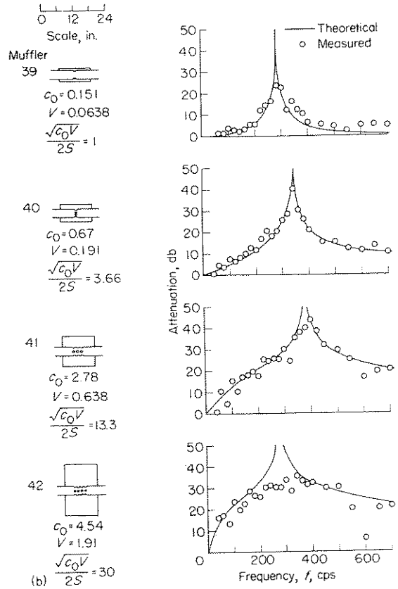
(b) Effect of varying \frac{\sqrt{c_0 l}}{2S} . Equation (B10).
