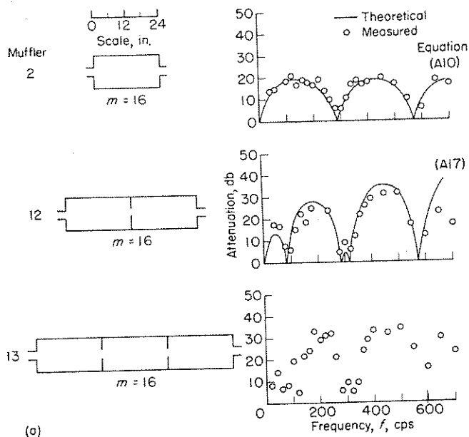
(a) Effect of number of chambers.
