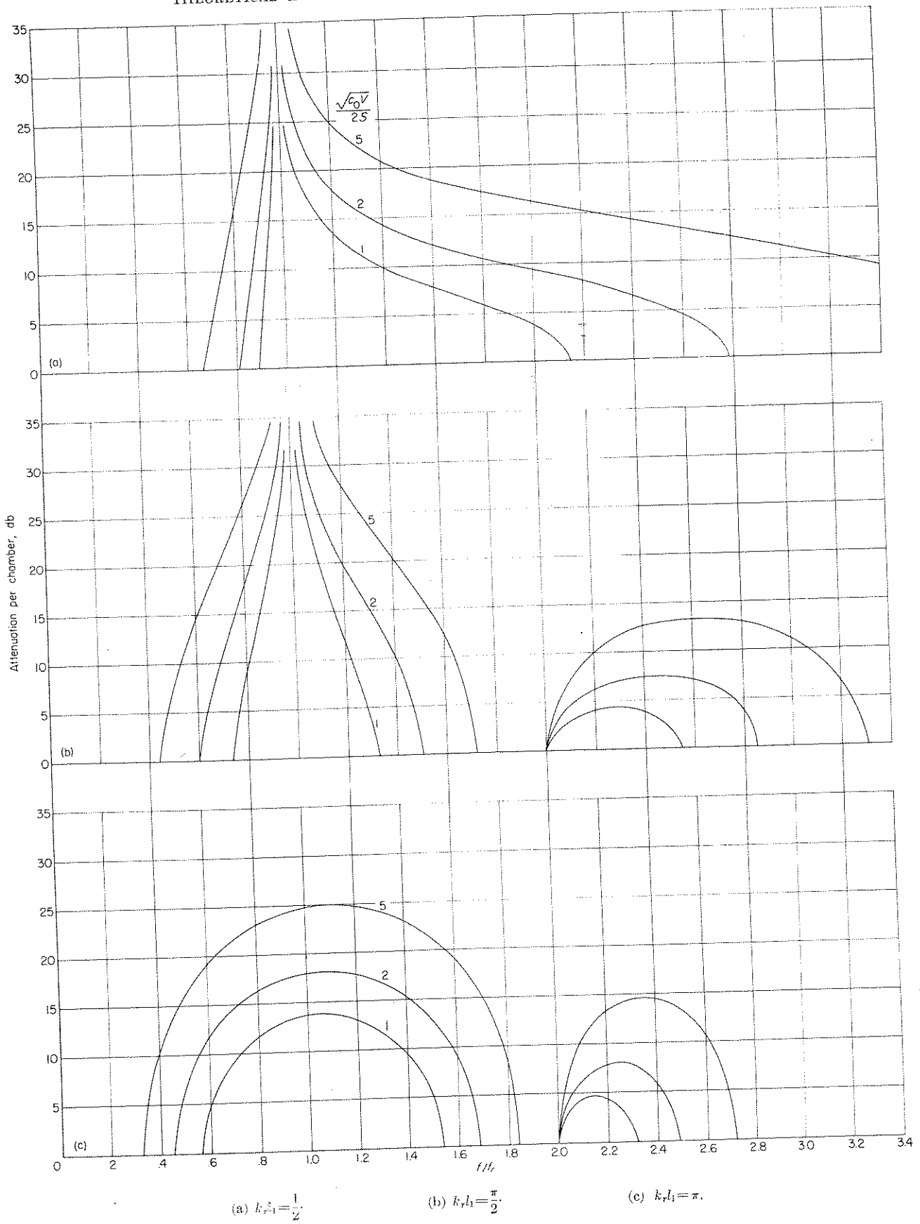
FIGURE 24.—Multiple-chamber-resonator design curves.
