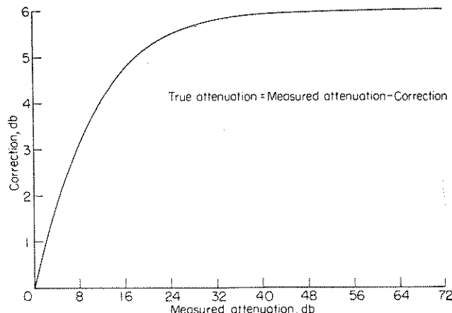
FIGURE 7.—Corrections to measured attenuation (Part I).
