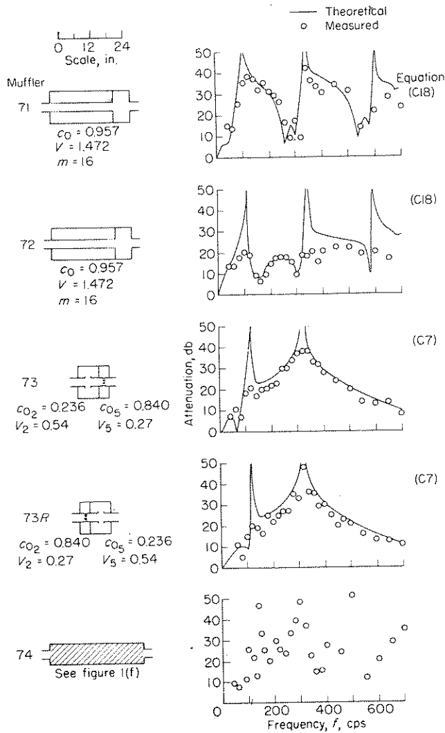
FIGURE 16.—Combination mufflers.
