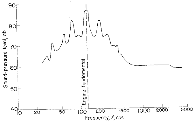
FIGURE 25.—Unmuffled-helicopter-noise frequency analysis.
