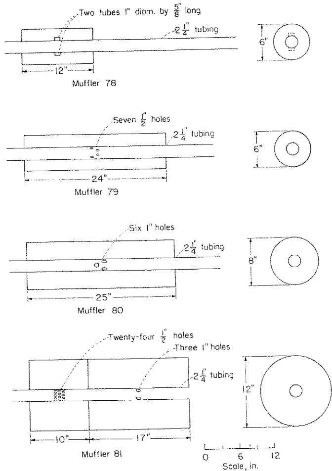
FIGURE 19.—Sketches of muffler-tailpipe combinations tested.
