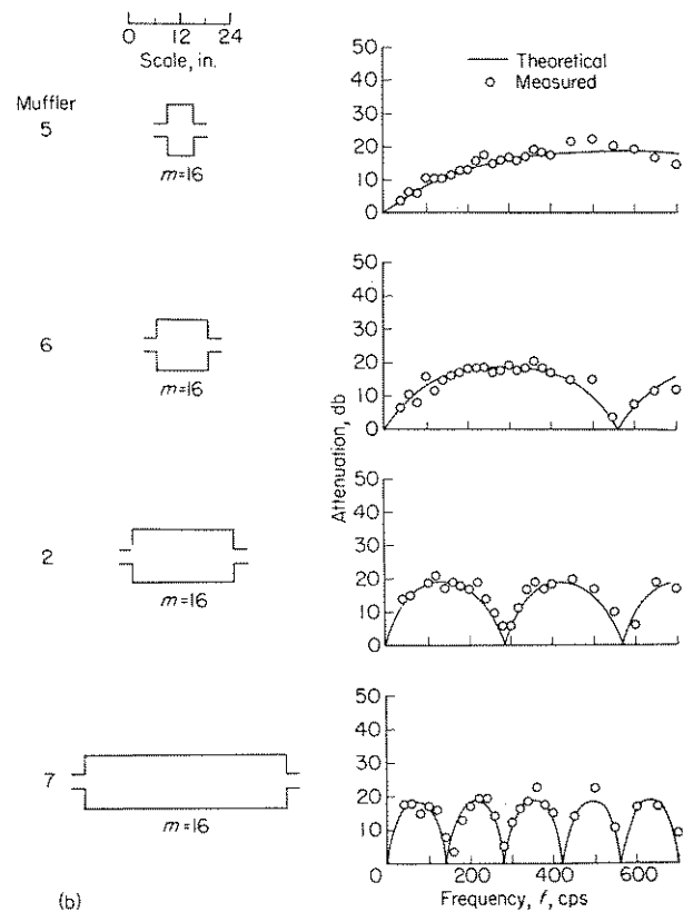
(b) Effect of length.
