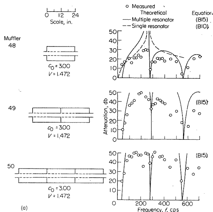
(a) Effect of number of chambers.
