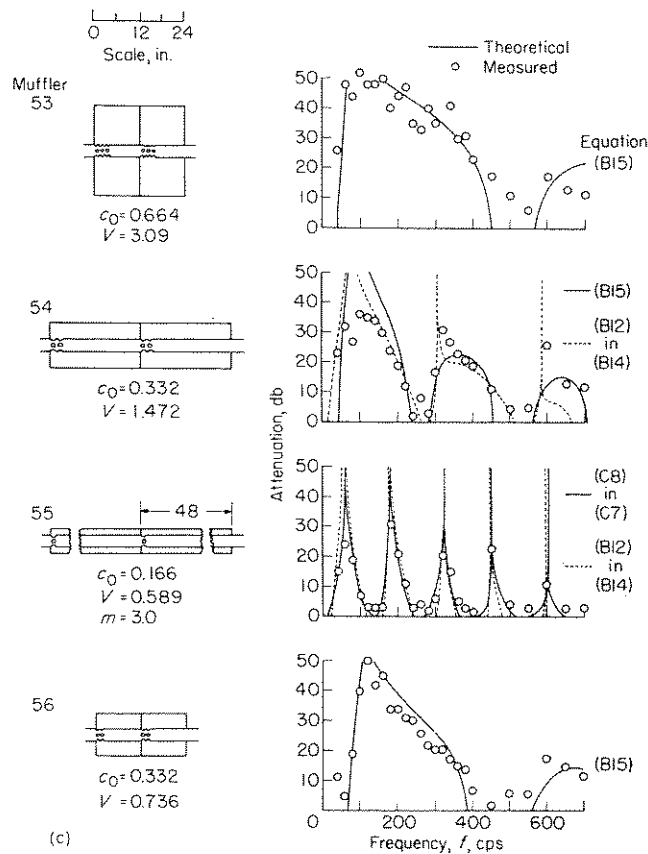
(c) Effect of length.
