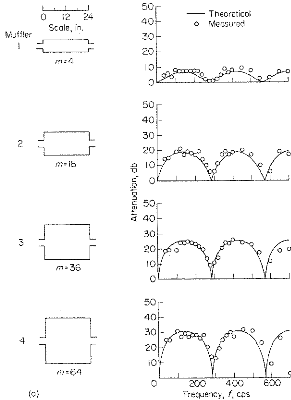
(a) Effect of expansion ratio m .
