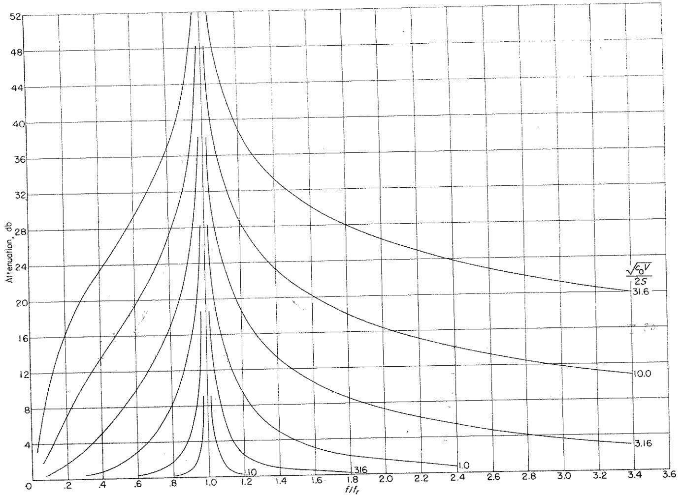
FIGURE 23.—Single-chamber-resonator design curves.
