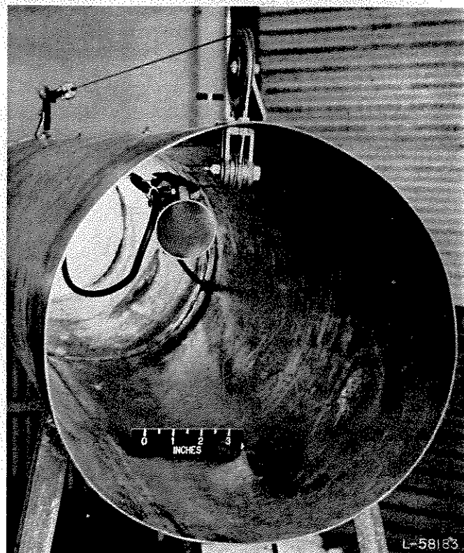
FIGURE 6.—Movable-microphone arrangement in the 12-inch tailpipe.
