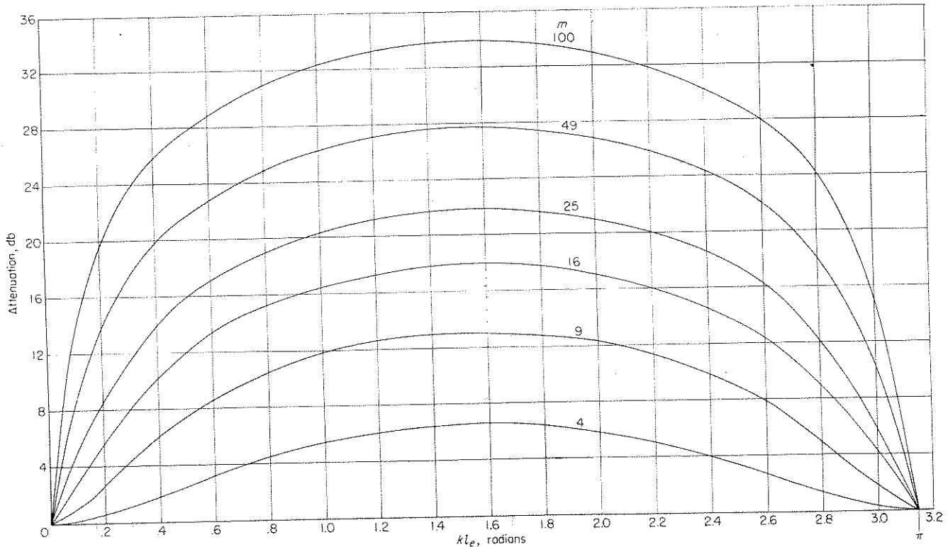
FIGURE 22.—Expansion-chamber design curves.
