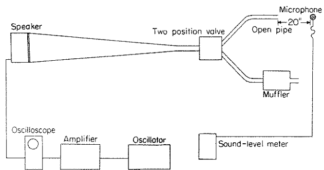
FIGURE 20.—Schematic diagram of the arrangement of apparatus for cold test of mufflers.
