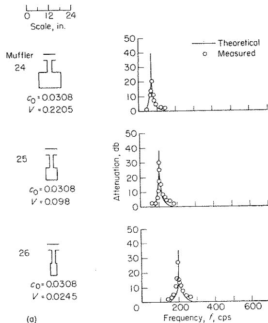
(a) Effect of volume V . Equation (B4).
