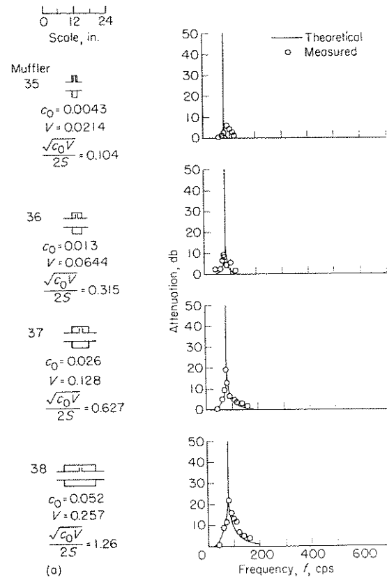
(a) Effect of varying the attenuation parameter \frac{\sqrt{c_0 V}}{2S} with the resonance parameter \sqrt{\frac{c_0 V}{V}} constant. Equation (B10).
