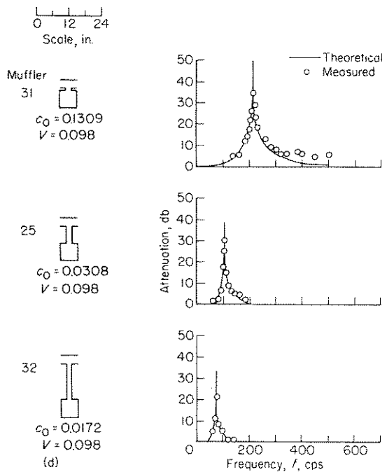
(d) Effect of length of connecting tube. Equation (B4).
