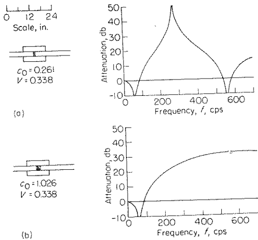
(a) Single-resonator muffler with tailpipe. k_r l_t = 0.48\pi . (See also table IV.) (b) Single-resonator muffler with tailpipe. k_r l_t = \pi .
