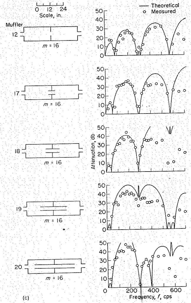
(c) Effect of connecting-tube length with an internal connecting tube. Equation (A17).
