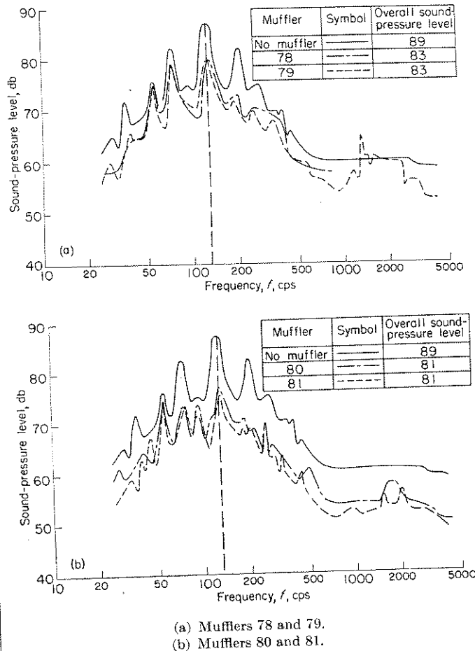
FIGURE 29.—Comparison of recorded frequency analyses of helicopter noise with and without mufflers.
