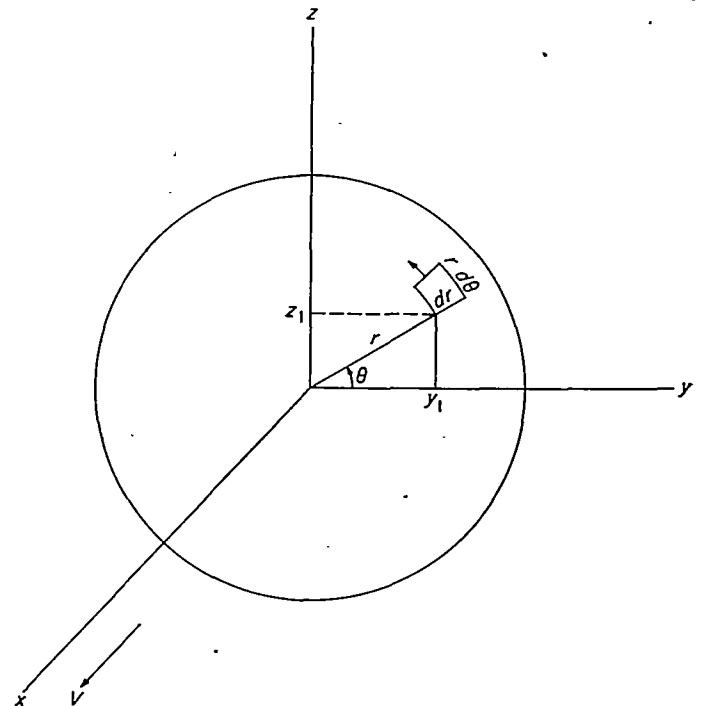
FIGURE 2.—Propeller disk and coordinate system.
