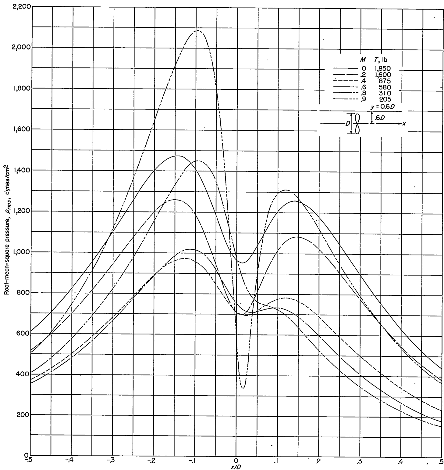
FIGURE 4.—Distribution of the root-mean-square pressures for the fundamental ( m=1 ) of a two-blade, 10-foot-diameter propeller at several forward-speed Mach numbers. C_P=0.10 ; k=0.29686 ; y=6 feet. (Operating conditions of propeller given in table I.)
