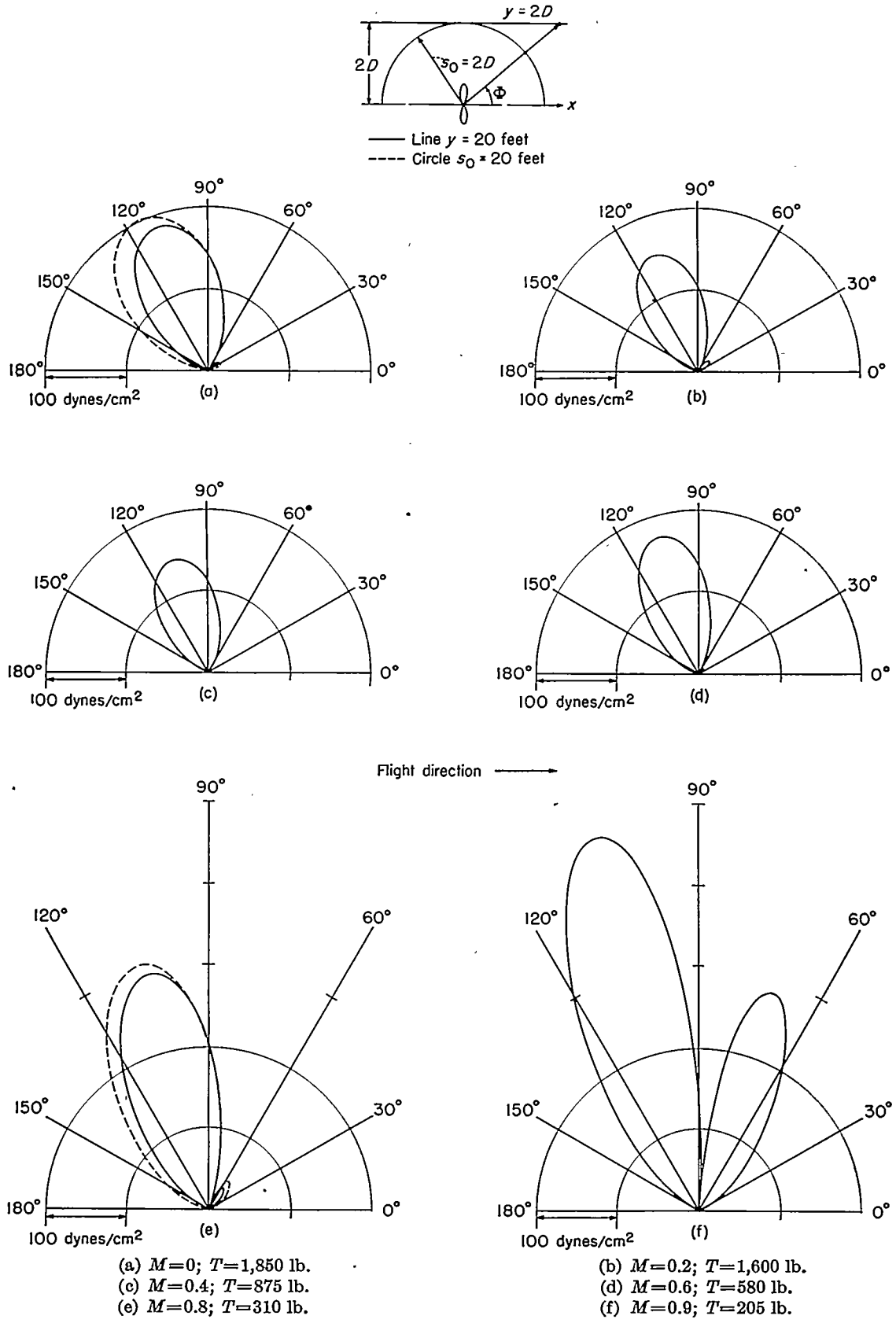
FIGURE 6.—Polar diagrams of the root-mean-square pressures calculated along a line y=20 feet and along a circle s_0=20 feet for a two-blade 10-foot-diameter propeller at several forward-speed Mach numbers. C_p=0.10 ; m=1 ; k=0.29686 . (Operating conditions of propeller given in table I.)
