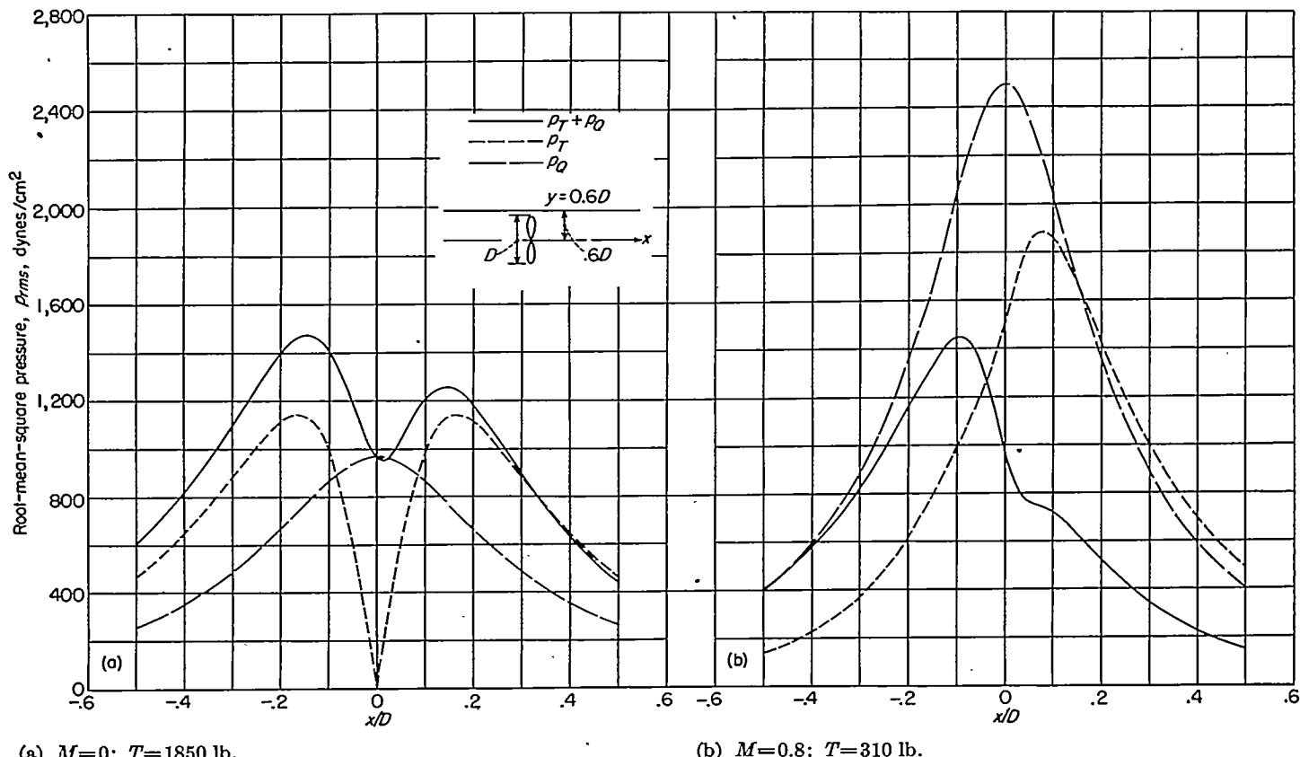
FIGURE 7.—Distribution of the root-mean-square total pressures and the root-mean-square pressures associated with thrust and torque for a two-blade, 10-foot-diameter propeller at forward-speed Mach numbers of 0 and 0.8. C_p=0.10 ; m=1 ; k=0.29886 ; y=6 feet. (Operating conditions of propeller given in table I.)
