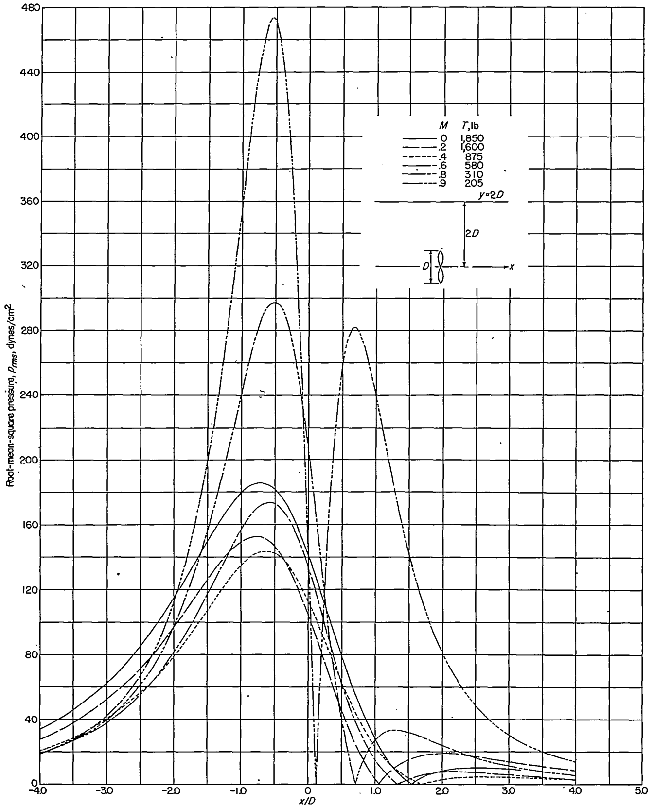
FIGURE 5.—Distribution of the root-mean-square pressures for the fundamental ( m=1 ) of a two-blade, 10-foot-diameter propeller at several forward-speed Mach numbers. C_P=0.10 ; k=0.29686 ; y=20 feet. (Operating conditions of propeller given in table I.)
