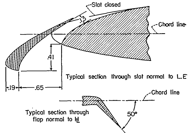
FIGURE 3.—Details of slats and plain flaps. All dimensions are in inches.
