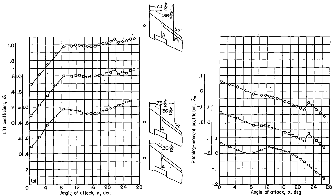
(b) Slats retracted and flaps and landing gear extended.
