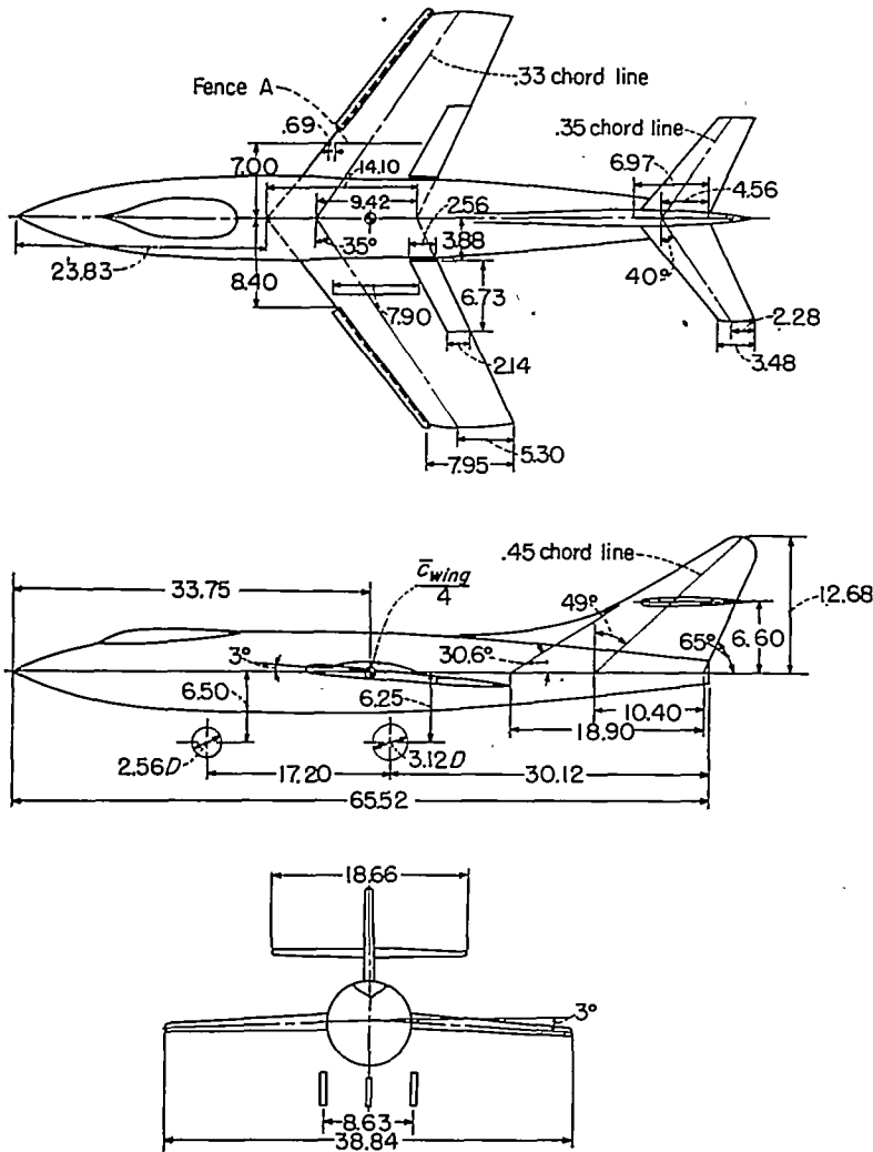
FIGURE 2.—Drawing of model used in the investigation. All dimensions are in inches.
