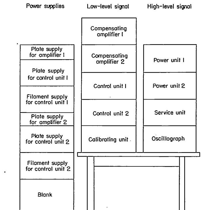
(b) FIGURE 10.—General disposition of equipment.
