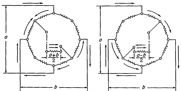
FIGURE 31.—Sum-difference circuit.
