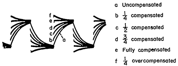
FIGURE 27.—Various degrees of compensation. Time constant, 0.4 millisecond; square-wave frequency, 500 cycles per second.
