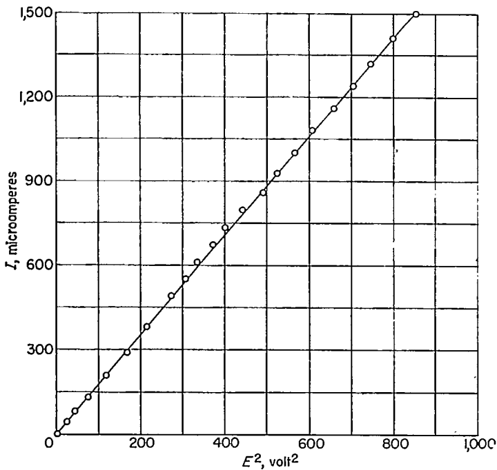
FIGURE 37.—Calibration of square-law circuit.
