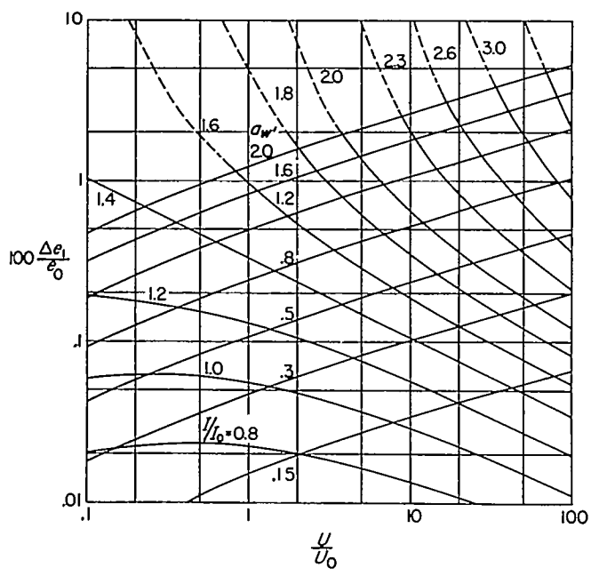
FIGURE 3.—Nondimensional hot-wire sensitivity in low-speed flow obtained in a thermal quasi equilibrium (eq. (3a) or (5)) and M is the time constant, depending on the operating conditions. The time constant is, in general,
