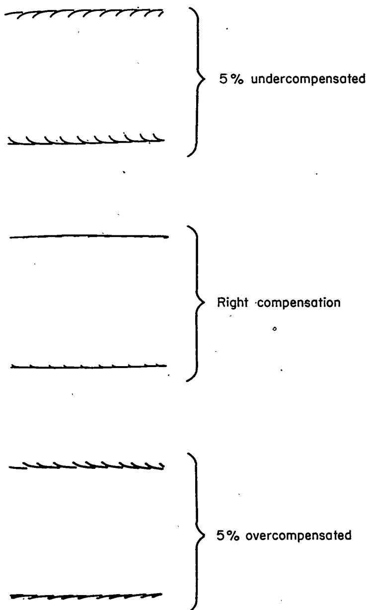
FIGURE 29.—Sensitivity of square-wave method.
