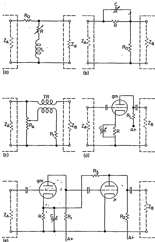
(a) Inductance resistance. (b) Capacitance resistance. (c) Transformer. (d) Negative-feedback resistance capacitance. (e) Improved form of system (d).
