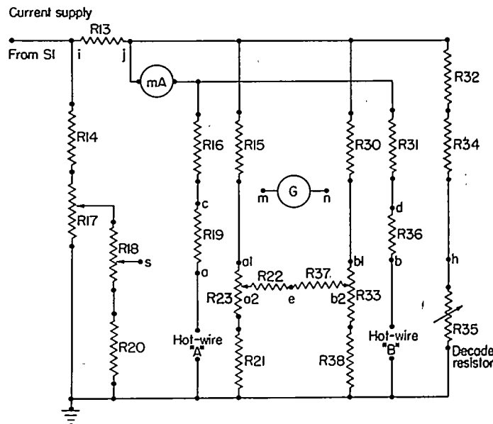
FIGURE 15.—Multiple bridge in control unit.
