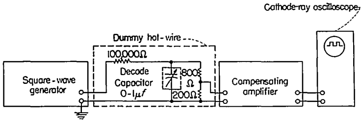
FIGURE 25.—Calibration of compensation performance by square waves.
