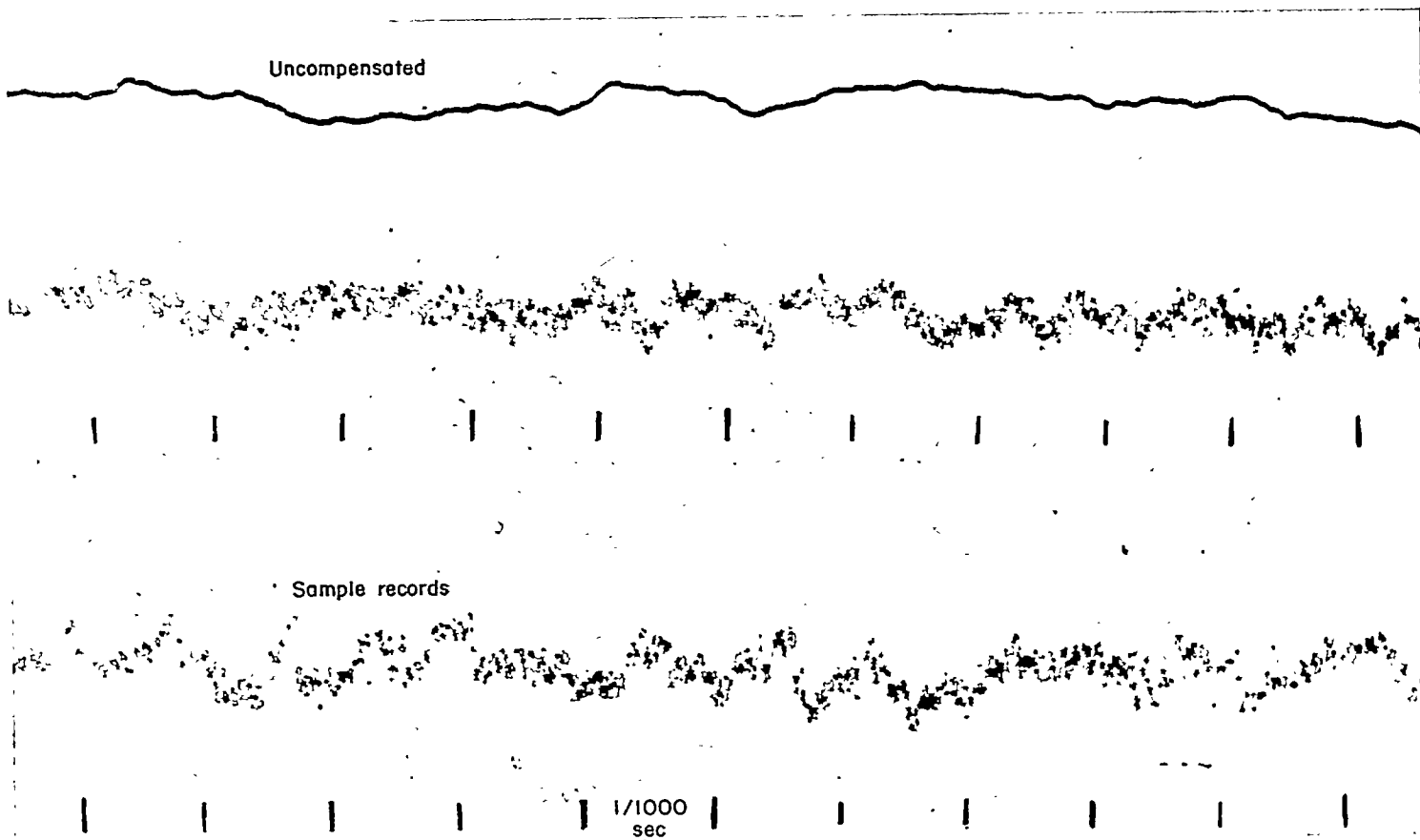
FIGURE 45.—Hot-wire record in supersonic wind tunnel. Tungsten wire, 0.00015-inch diameter, 0.08 inch long; pressure at stagnation temperature, 40 centimeters of mercury; T_o = 16^\circ \text{C} (289° K); Mach number, 1.73; current, 46.2 milliamperes; T_w = 101^\circ \text{C} (374° K); R_w = 13.4 ohms; time constant M = 0.45 millisecond.
