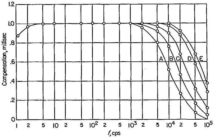
FIGURE 24.—Frequency response of compensating amplifier.
