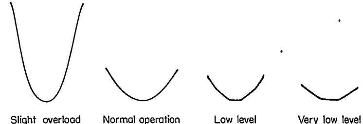
FIGURE 35.—Amplitude response of square-law circuit. Amplification readjusted for each oscillograph. Frequency, 100 cycles per second.
