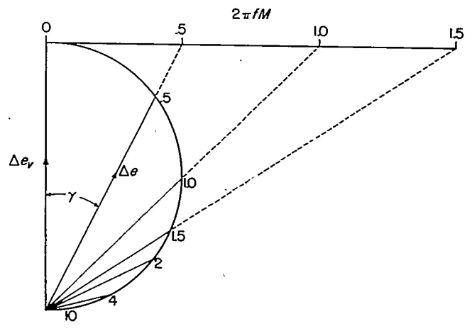
FIGURE 4.—Vector diagram of hot-wire thermal lag. \left|\frac{\Delta e}{\Delta e_0}\right| = \frac{1}{\sqrt{1 + (2\pi f M)^2}} ; \gamma = \tan^{-1} 2\pi f M .
