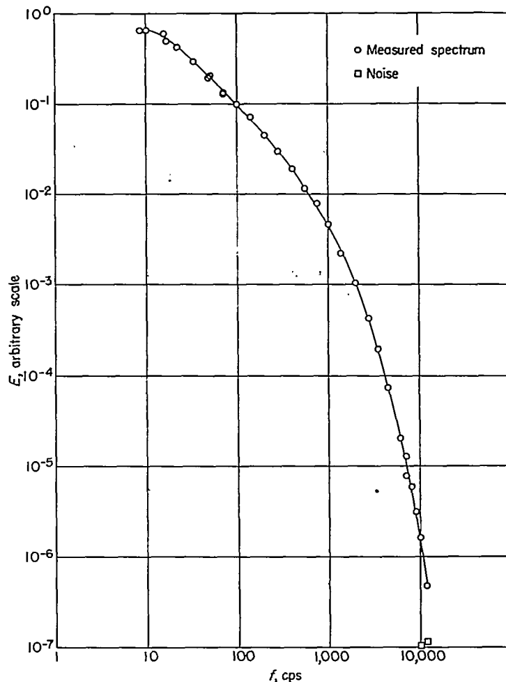
FIGURE 47.—Energy spectrum of turbulent velocity fluctuations in low-speed boundary layer. Free-stream velocity U_0=50 feet per second; boundary-layer thickness, 3 inches; distance of probe from surface, 0.15 inch; local mean velocity U/U_0=0.63 ; turbulence level in terms of free-stream velocity U'/U_0, 0.078 .
