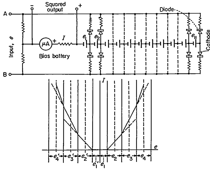
FIGURE 34.—Biased-diode square-law detector.
