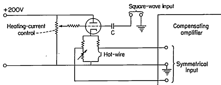
FIGURE 14.—Heating-current control and square-wave feeding system.
