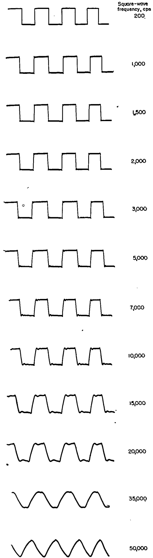
FIGURE 28.—Square-wave response of compensation.
