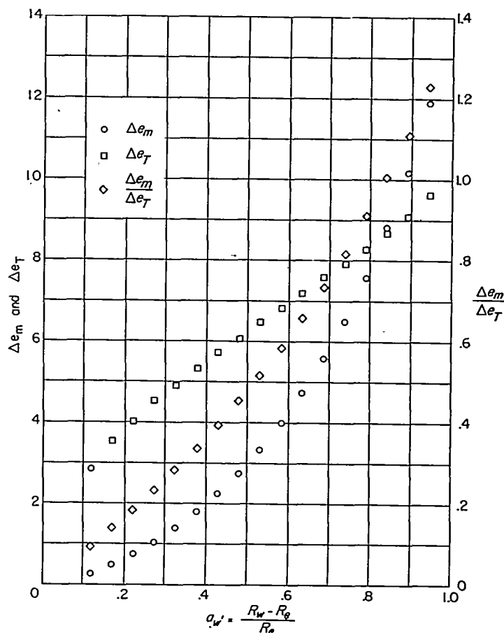
FIGURE 8.—Variation of fluctuation sensitivities with wire temperature in supersonic flow. Tungsten wire with 0.0015-inch diameter was used. Flow conditions: M=1.73 , T_0=293^\circ K, and pressure at stagnation temperature was 40 centimeters of mercury.
