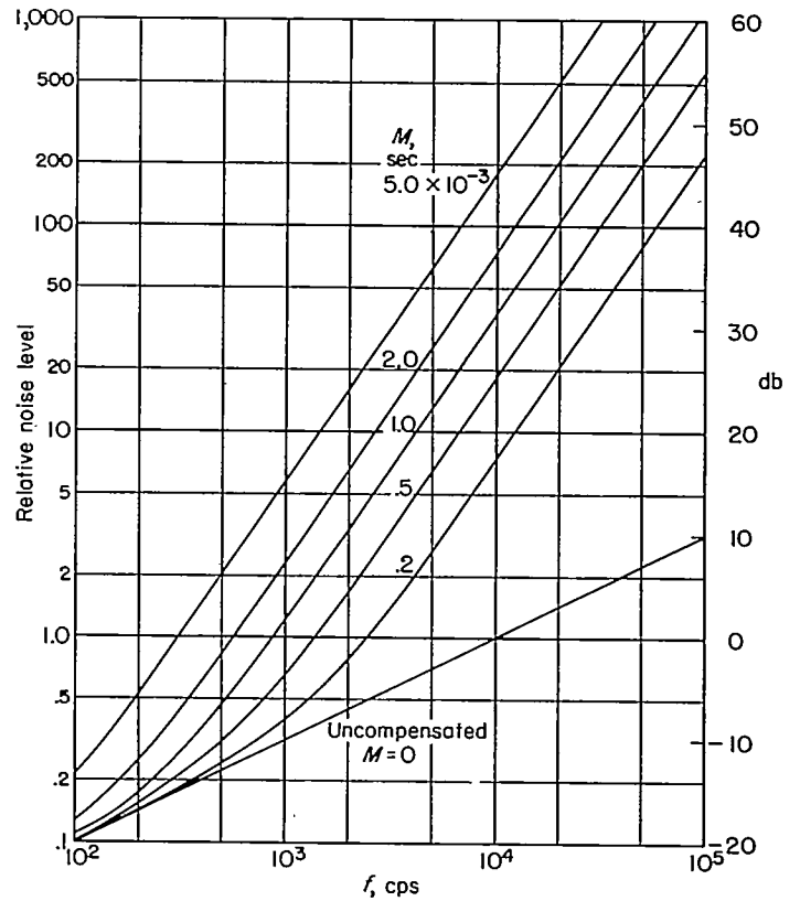
FIGURE 20.—Theoretical noise level of compensating amplifiers as compared with 10-kilocycle band-width amplifier.
