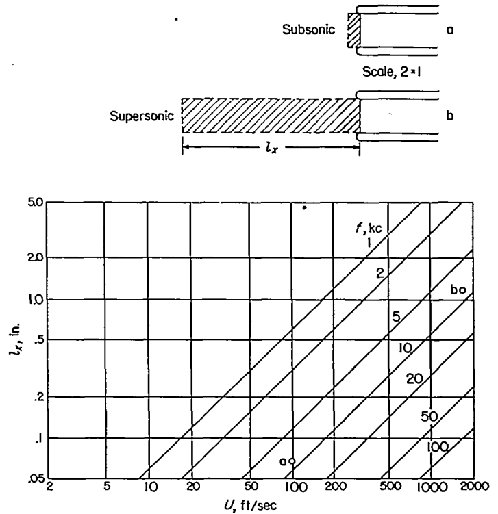
FIGURE 1.—Resolution length of hot-wire anemometer at various speeds.
