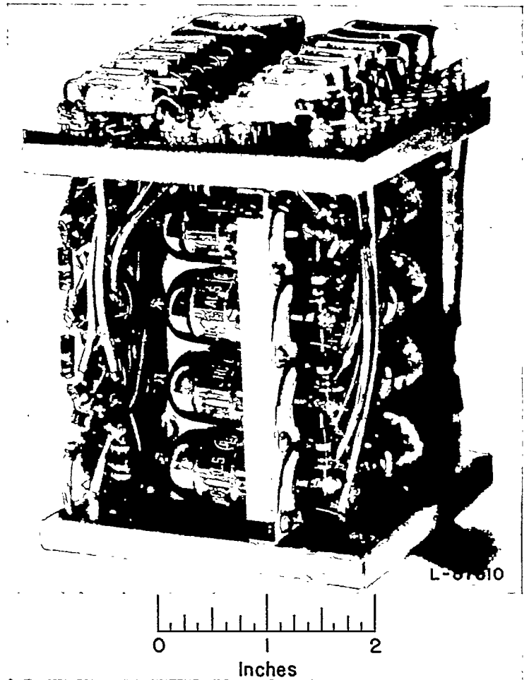
FIGURE 39.—Biased-diode square-law detector in power unit.
