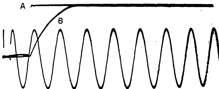
FIGURE 42.—Hot-wire response to traveling shock wave. Compensated A and uncompensated B record from shock wave. Wollaston wire, diameter, 0.0001 inch; heating current, 21.42 milliamperes; \alpha_s' = 0.47 ; time constant M = 0.225 millisecond; calibrating sine wave, 5-kilocycle, 75-millivolt root-mean-square value.
