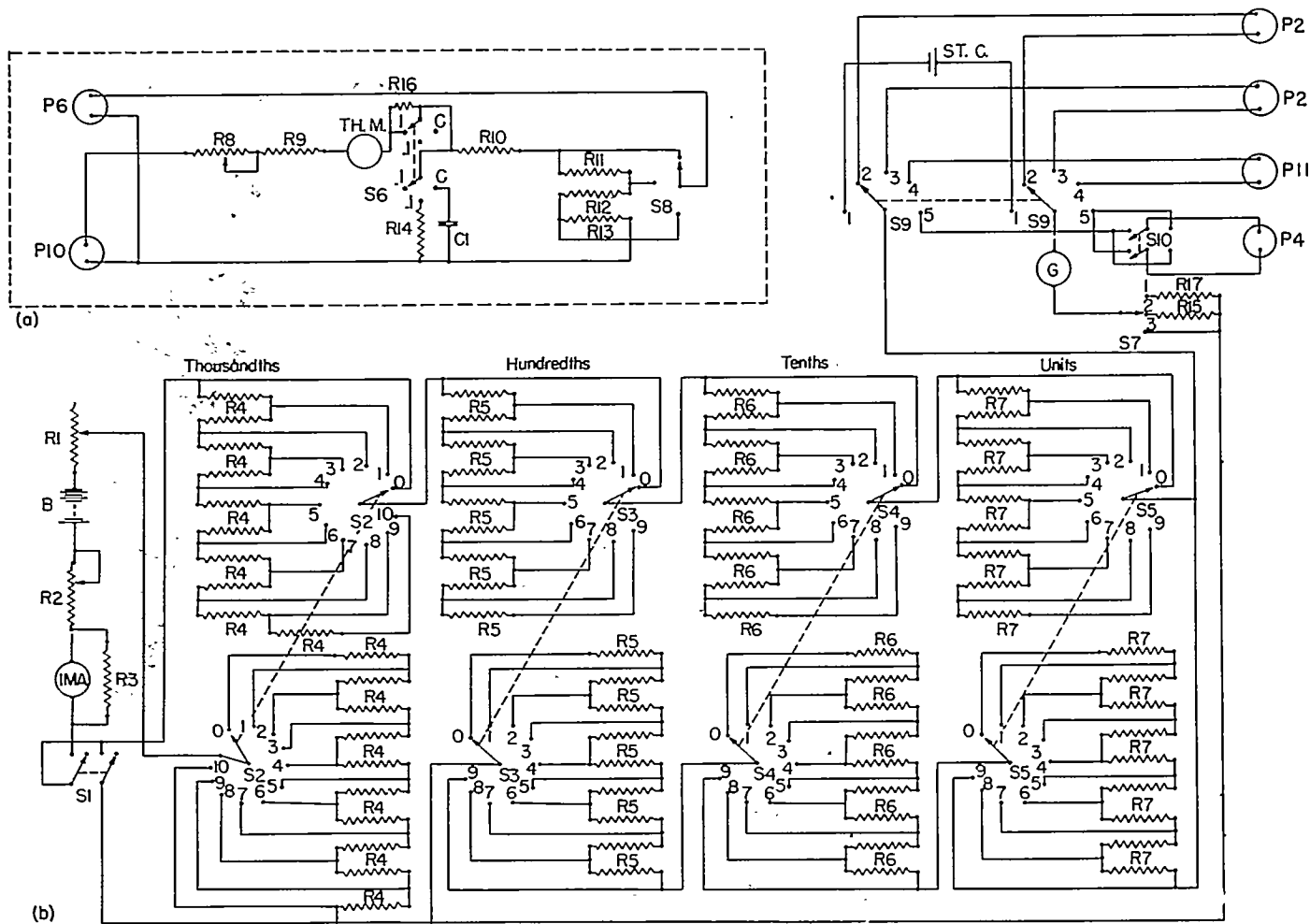
(a) Test-signal calibration. (b) Direct-current potentiometer.
