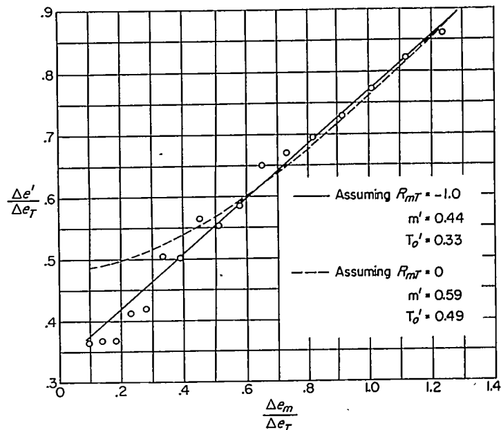
FIGURE 44.—Graphical separation of mass-flow and temperature fluctuations.
