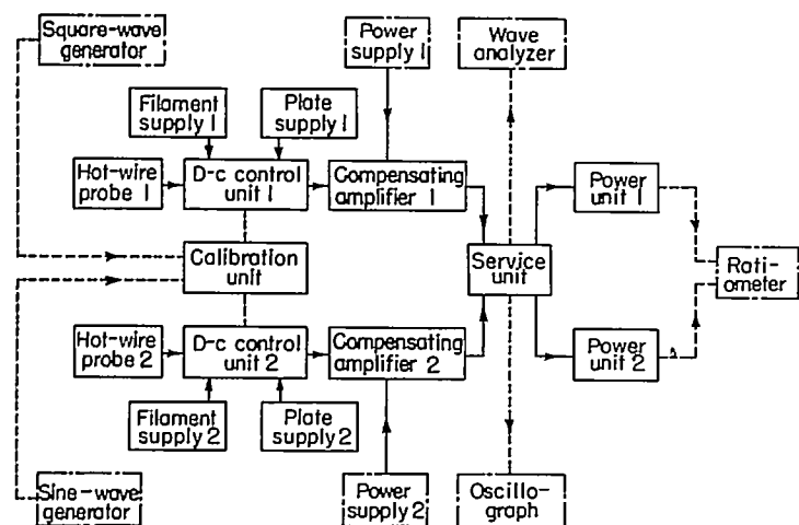
FIGURE 9.—Block diagram of turbulence-measuring equipment.
