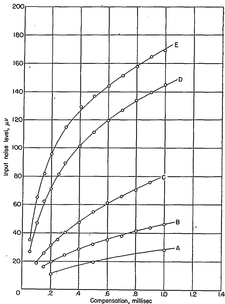
FIGURE 23.—Noise level of compensating amplifier (equivalent input with compensation off).
