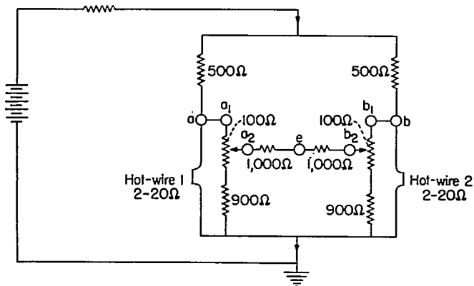
FIGURE 16.—Matching circuit.
