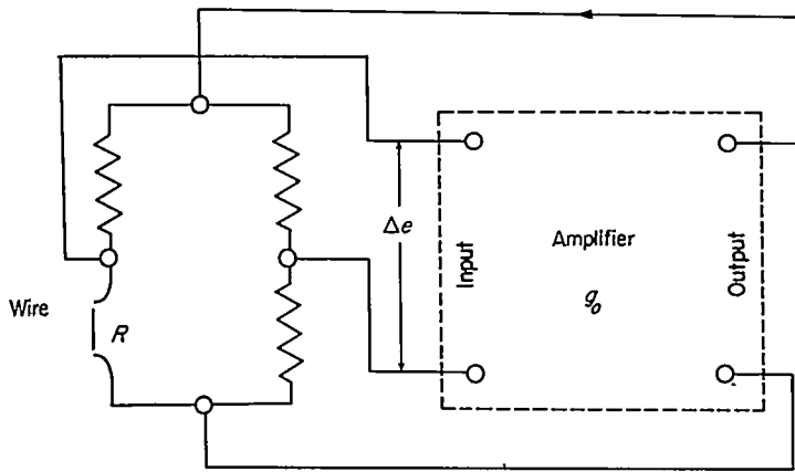
FIGURE 18.—Constant-temperature feedback system.
