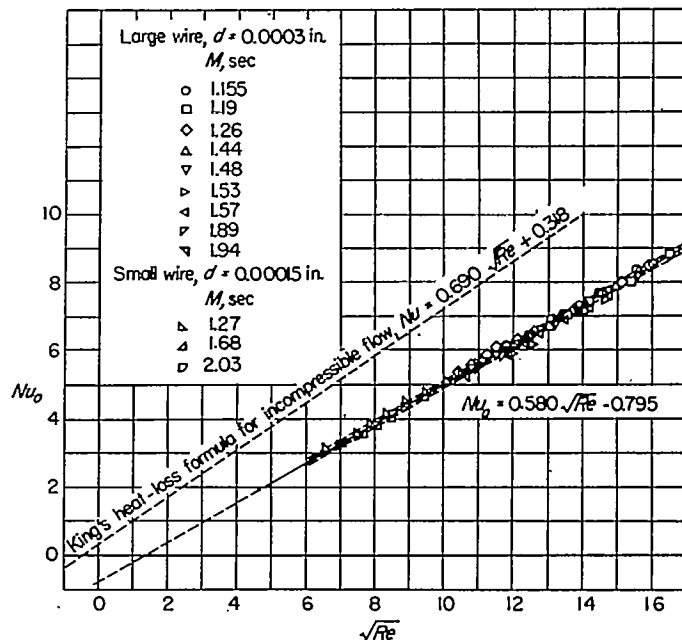
FIGURE 7.—Heat loss of wire at supersonic speeds. Re = \frac{\rho u d}{\mu_o} ; Nu_o = \frac{H}{\pi l \Delta T k_o} ; standard deviation of Nu_o is 0.098.
