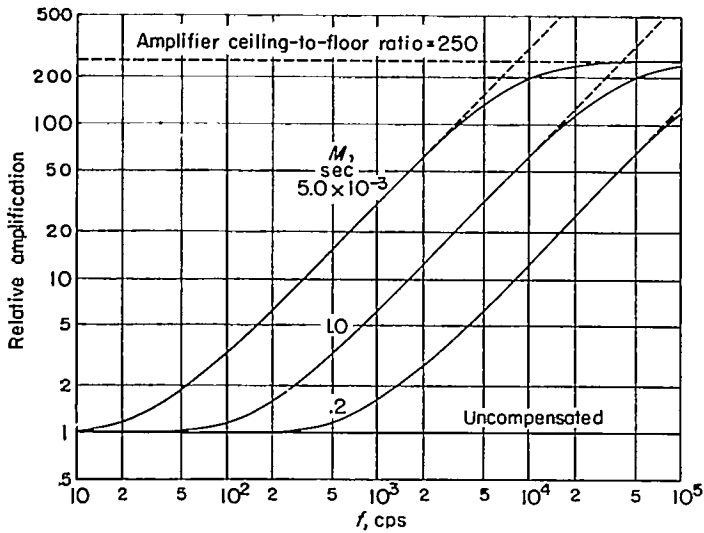
FIGURE 19.—Range of compensation.
