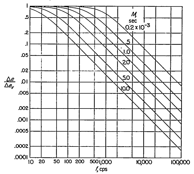
FIGURE 5.—Frequency response of uncompensated hot-wire.
