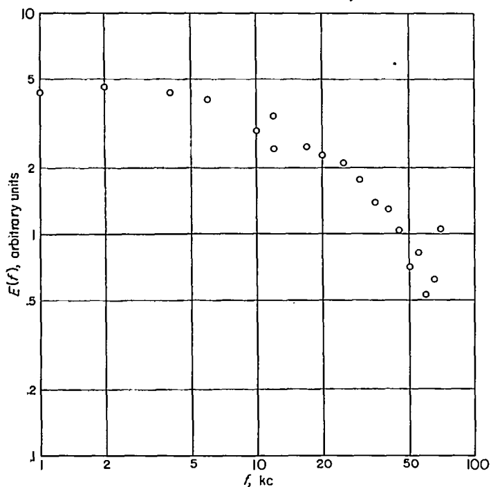
FIGURE 46.—Power spectrum of turbulent fluctuations in supersonic boundary layer. Free-stream Mach number, 1.75; atmospheric pressure; stagnation temperature T_0=20^\circ\text{C} ( 293^\circ\text{K} ); boundary-layer thickness, 0.500 inch; probe location y=0.250 inch.
