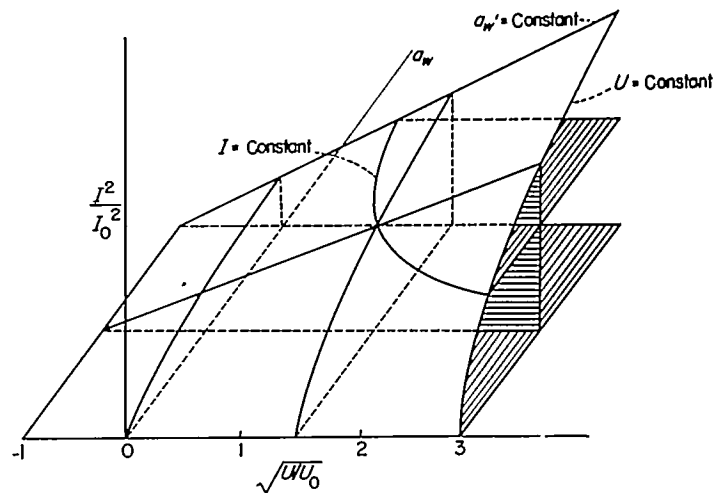
FIGURE 2.—Hot-wire in thermal equilibrium. a_w' = \frac{R_w - R_e}{R_e} .
