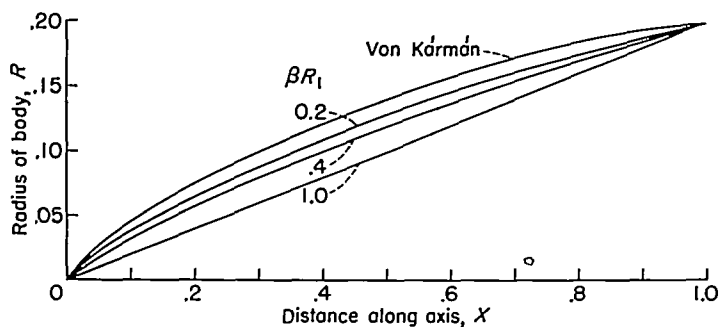
FIGURE 4.—Minimum-drag projectile-tip shapes. Von K6rm6n projectile tip is shown for comparison.
