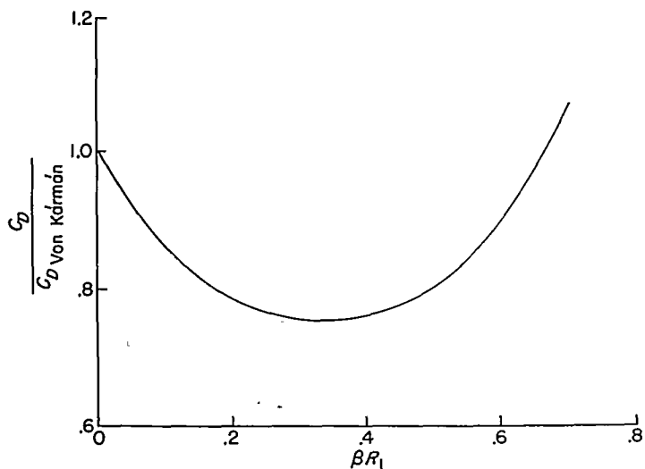
Figure 5.—Ratio of minimum-wave-drag coefficient to Von K6rm6n drag coefficient as a function of \beta R_1 .
