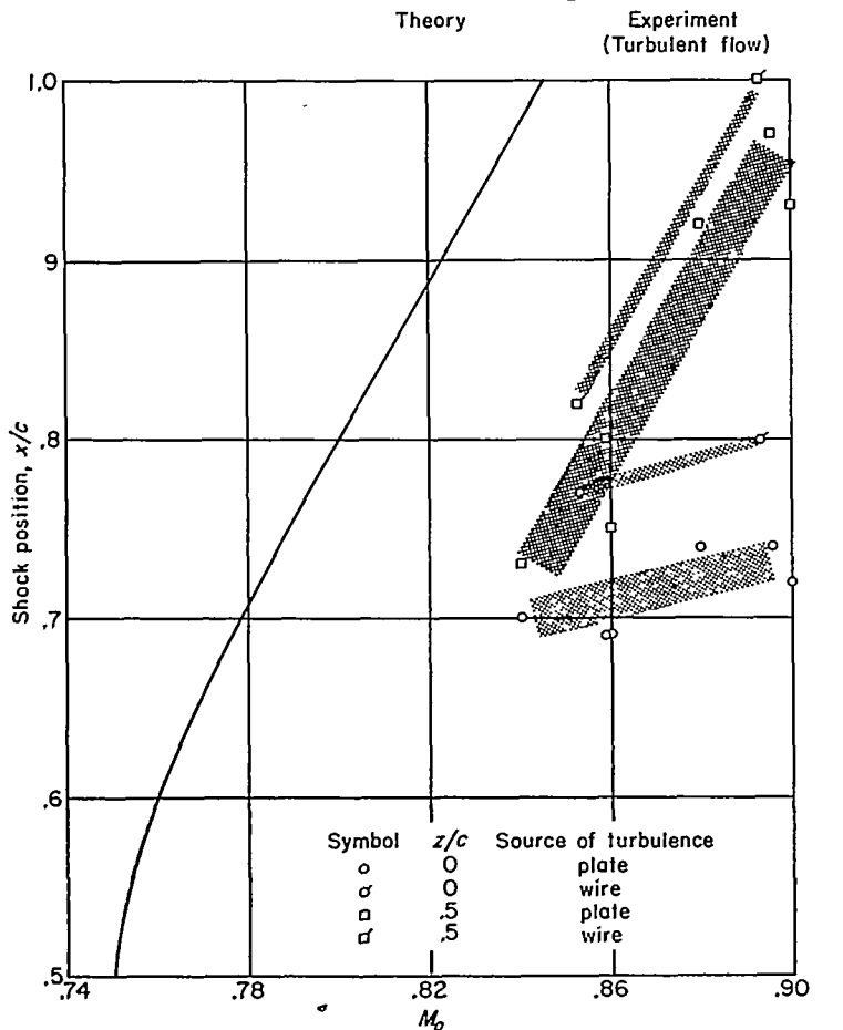
FIGURE 42.—Variation of shock position with Mach number for 12-percent-thick circular-arc airfoil.
