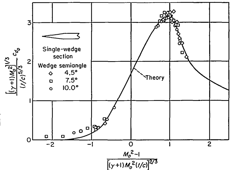
FIGURE 6.—Theoretical and experimental drag results for a single wedge section, k = \frac{M_0^2(\gamma+1)}{U_0} .
