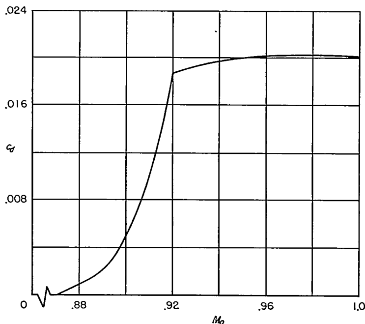
FIGURE 39.—Variation of c_d with M_o , 4-percent-thick circular-arc airfoil.
