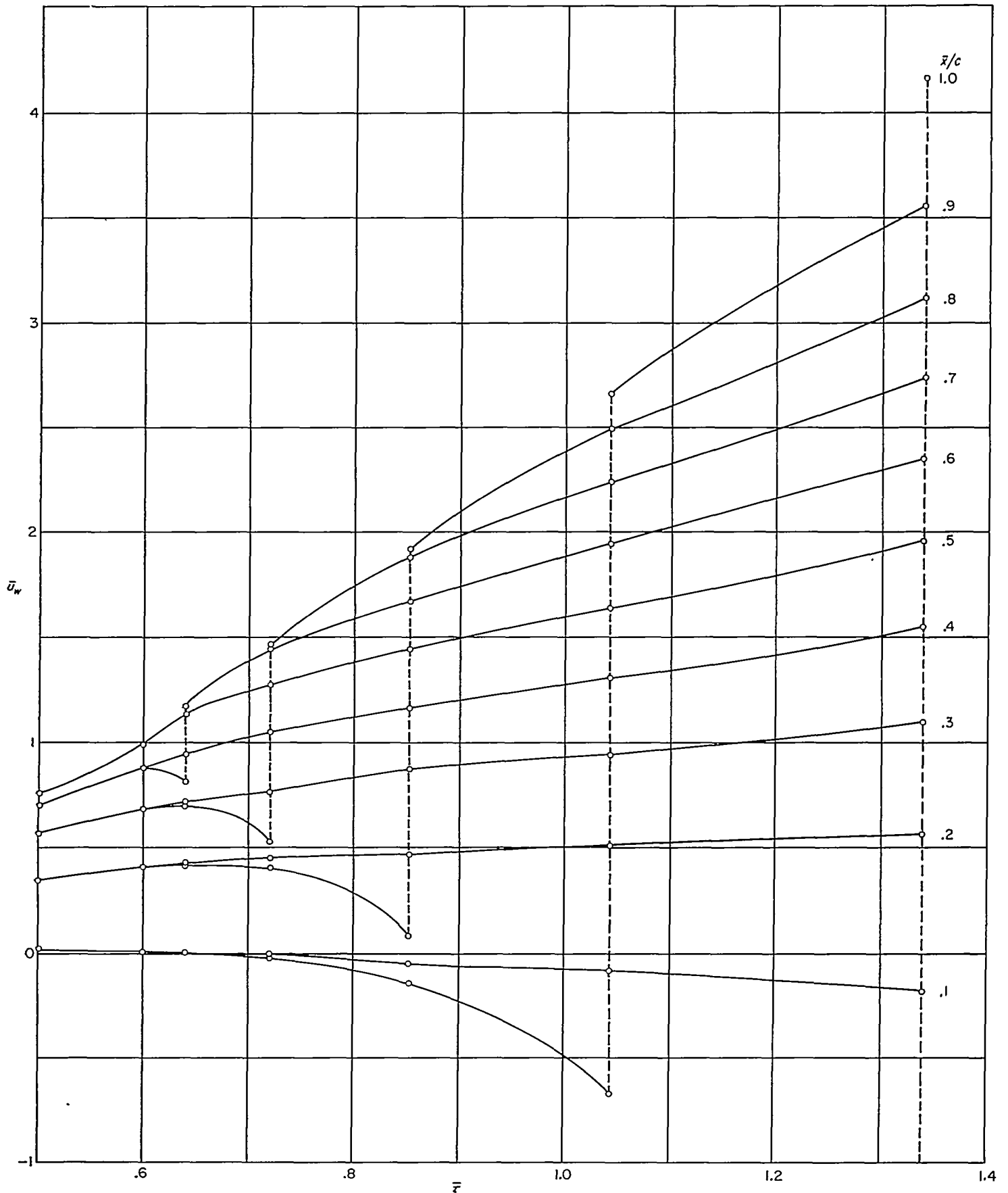
FIGURE 27.—Variation of u_w with \bar{r} for various values of x/c , shock wave forward of trailing edge.
