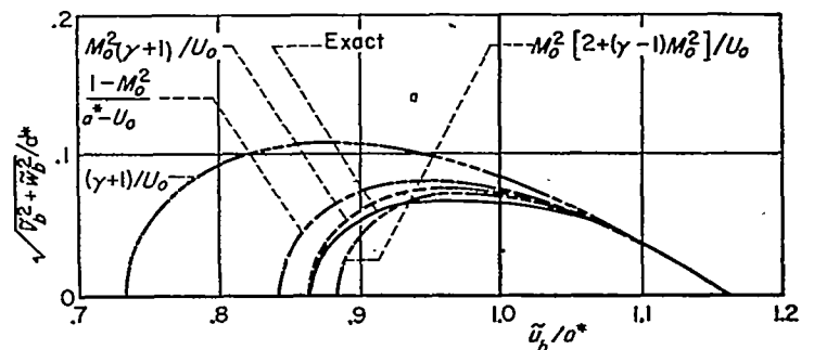
FIGURE 4.—Approximate and exact shock polar diagram, M_o = 1.2 .
