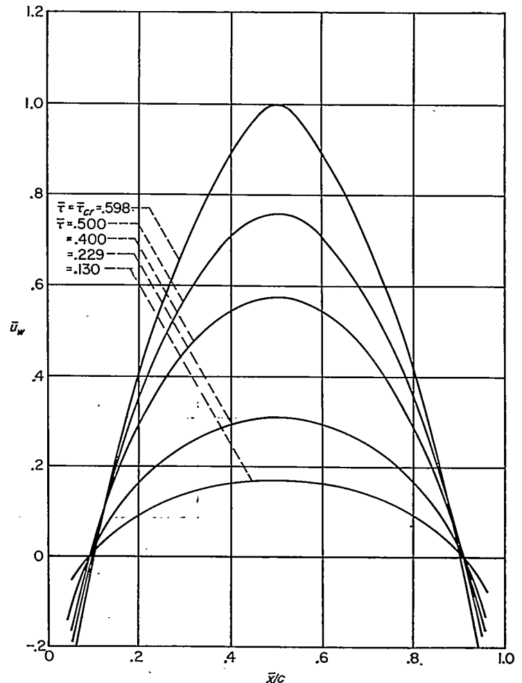
FIGURE 22.—Chordwise variation of \bar{u}_W for various \bar{\tau} in the subcritical range.
