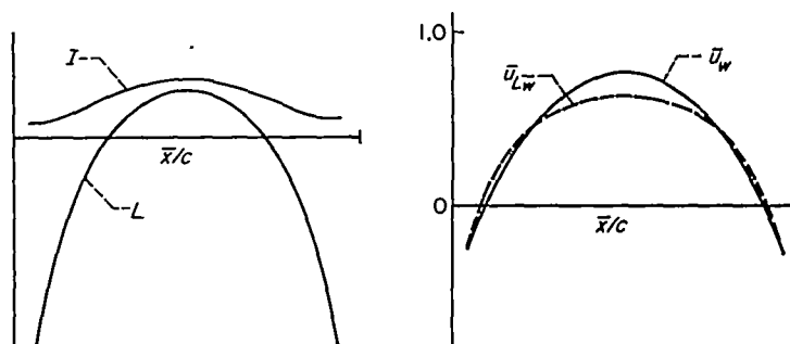
FIGURE 8.—Typical curves of I , L , \bar{u} , and \bar{u}_L in the subcritical range
