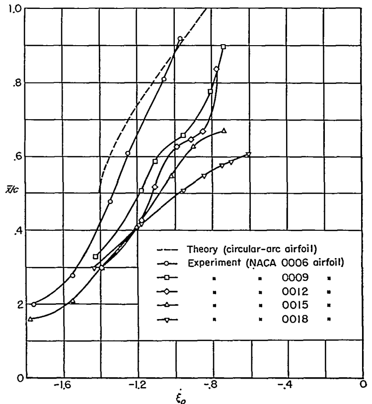
FIGURE 43.—Effect of thickness on shock position.
