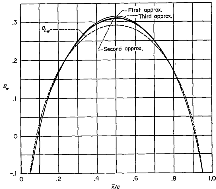
FIGURE 21.—Results of iteration calculations in the subcritical range, \bar{\tau} = 0.229 .
