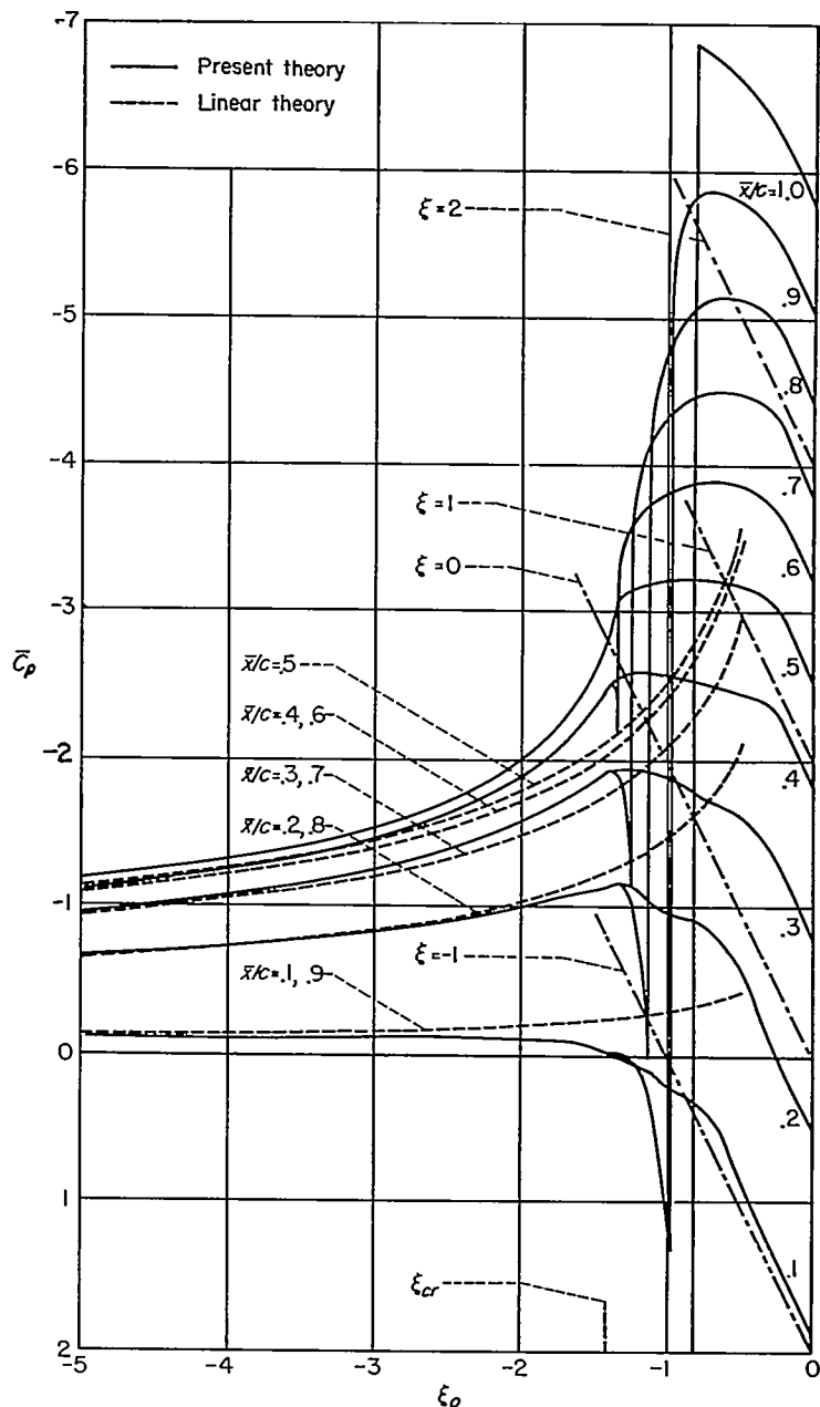
FIGURE 34.—Variation of \bar{C}_p with \xi_0 for various \bar{x}/c .
