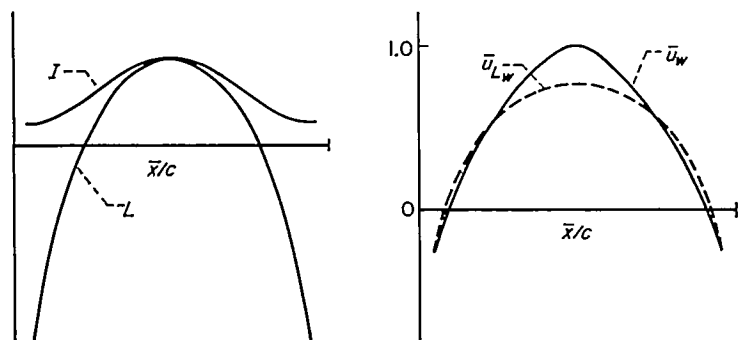
FIGURE 9.—Typical curves of I , L , \bar{u} , and \bar{u}_L at the critical Mach number.
