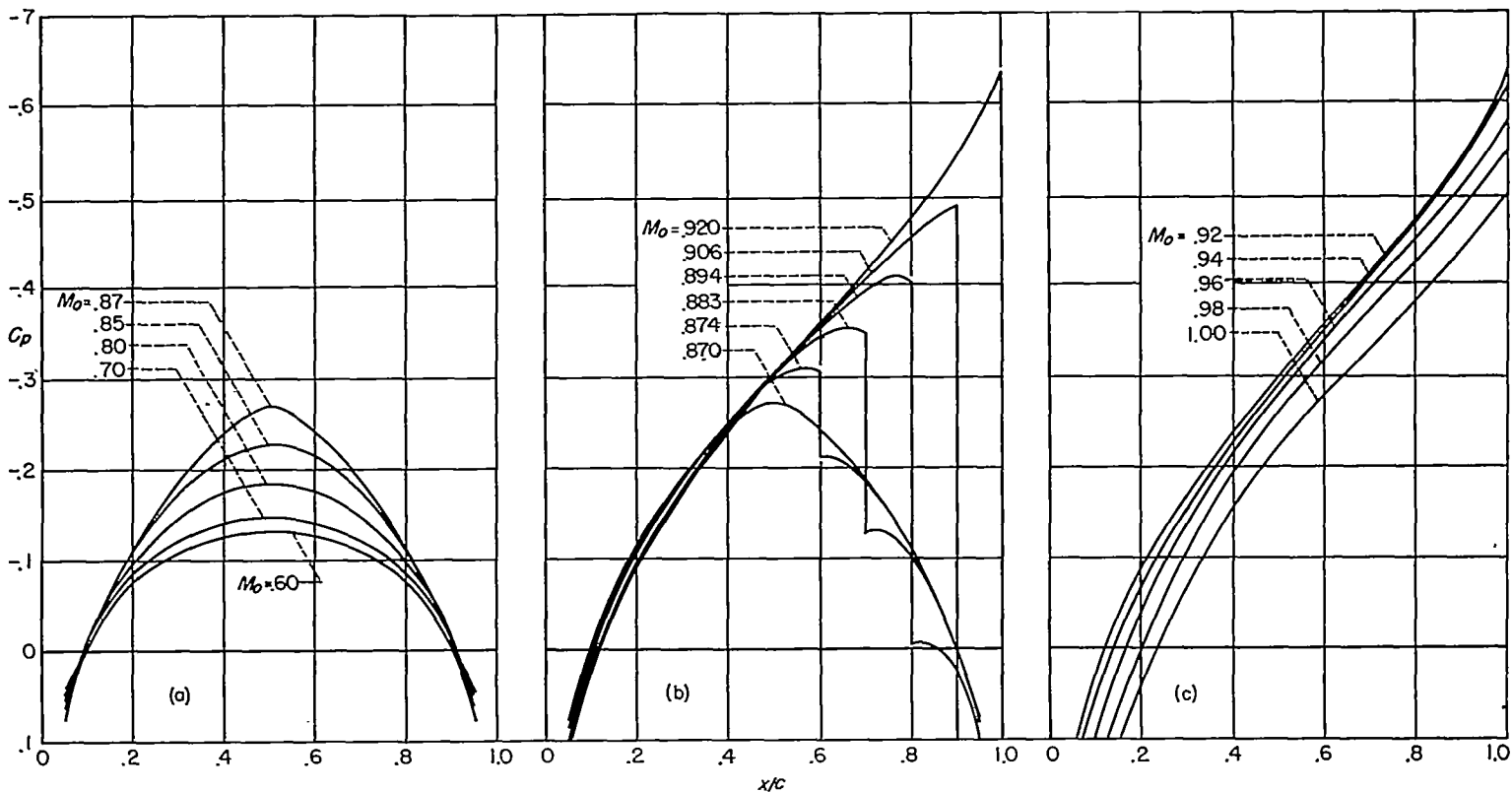
(a) Subcritical. (b) Shock wave forward of trailing edge. (c) Shock wave at trailing edge. FIGURE 37.—Chordwise variation of C_p for various free-stream Mach numbers, 4-percent-thick circular-arc airfoil.
