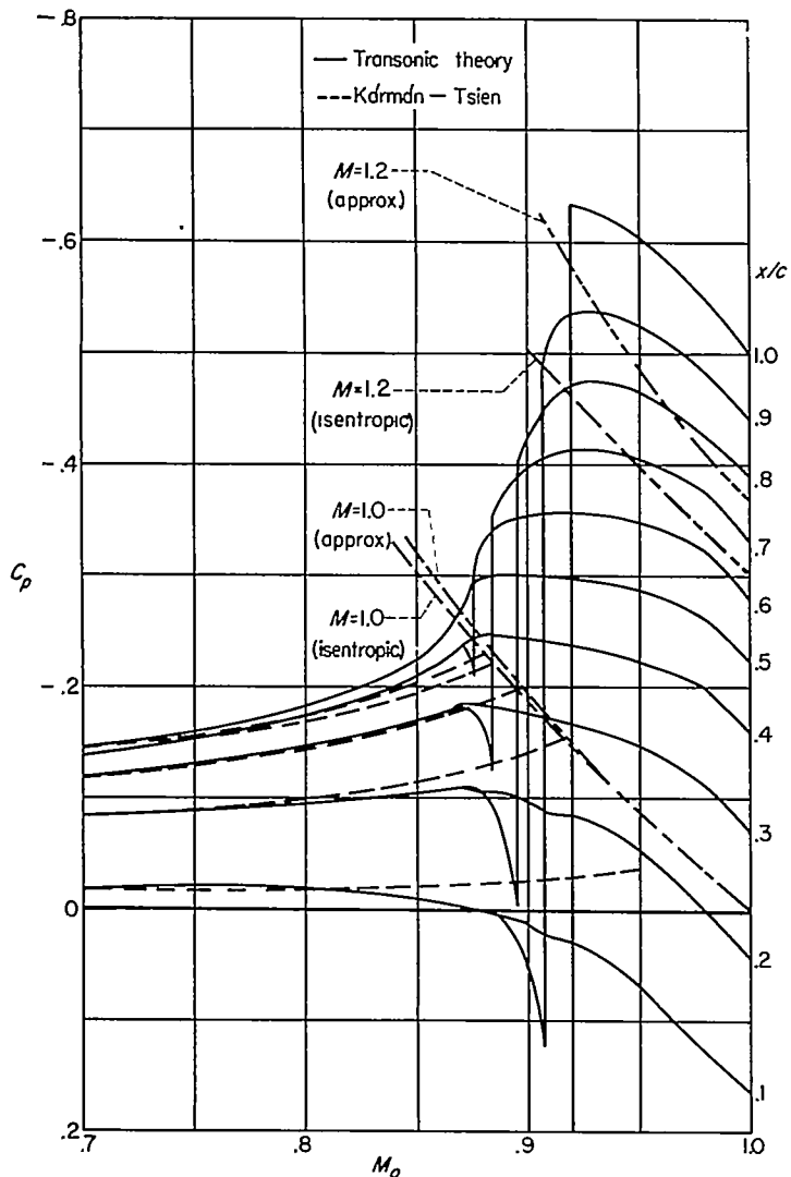
FIGURE 38.—Variation of C_p with M_o for various values of x/c , 4-percent thick circular-arc airfoil.
