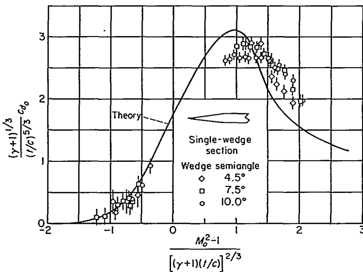
FIGURE 5.—Theoretical and experimental drag results for a single wedge section, k = \frac{\gamma+1}{U_0} .
