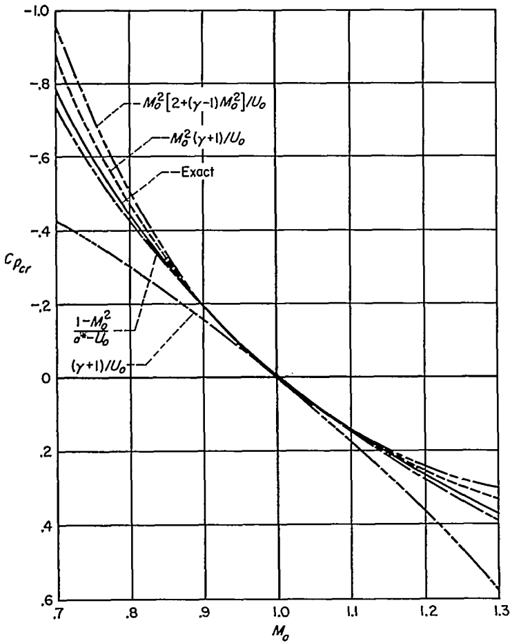
FIGURE 2.—Variation, approximate and exact, of critical pressure coefficient with free-stream Mach number.
