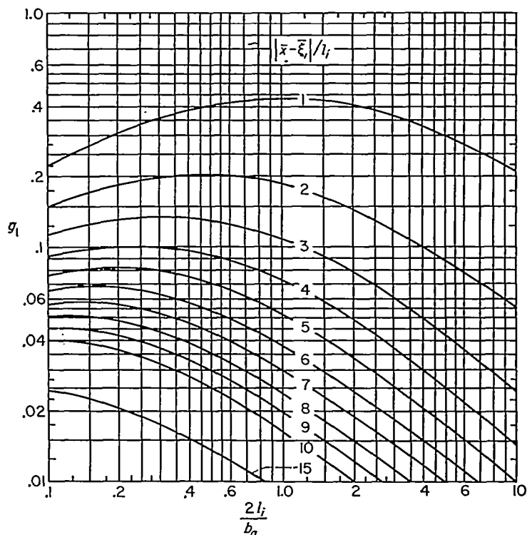
FIGURE 20.—Variation of influence function g_1 \left[ \left( \frac{\bar{x} - \bar{\xi}_i}{l_i}, \left( \frac{2l_i}{b_i} \right) \right] with \frac{2l_i}{b_i} for various values of \frac{\bar{x} - \bar{\xi}_i}{l_i} . Computed from equation (77).
