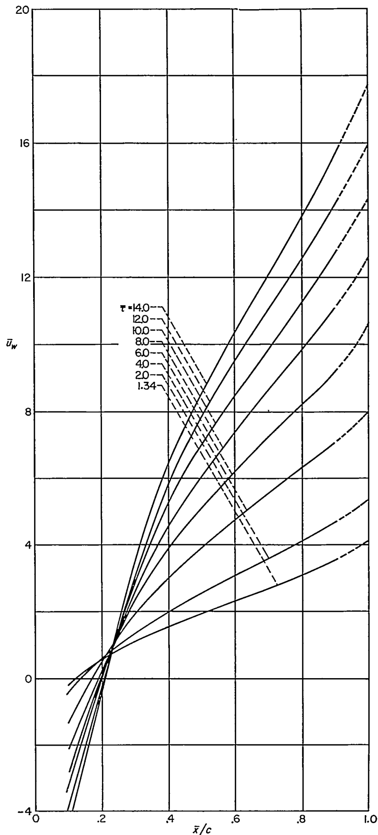
FIGURE 31.—Chordwise variation of \bar{u}_w for various \bar{\tau} , shock wave at trailing edge.
