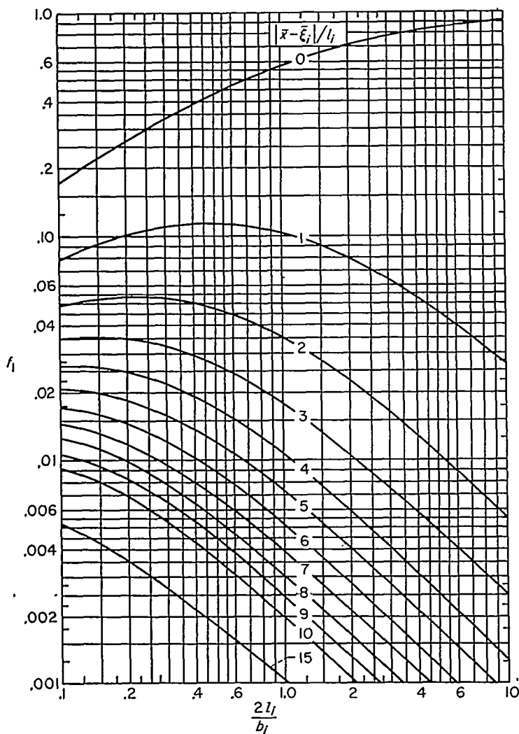
FIGURE 19.—Variation of influence function f_1 \left[ \left( \frac{\bar{x} - \bar{\xi}_i}{l_i}, \left( \frac{2l_i}{b_i} \right) \right] with \frac{2l_i}{b_i} for various values of \frac{\bar{x} - \bar{\xi}_i}{l_i} . Computed from equation (73).
