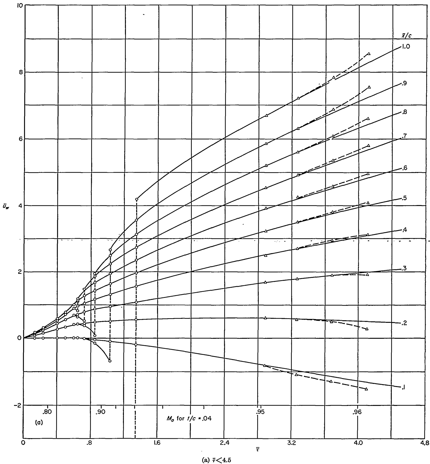
FIGURE 32.—Variation of \bar{u}_w with \bar{r} for various values of \bar{x}/c , shock wave at trailing edge.
