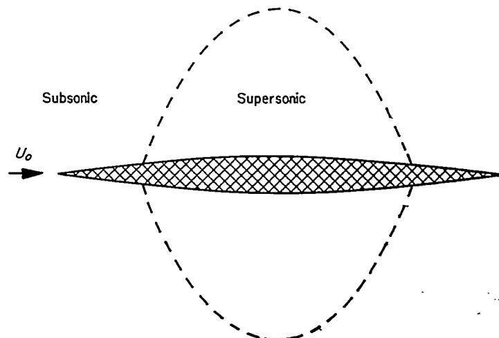
FIGURE 11.—Shock-free transonic flow.
