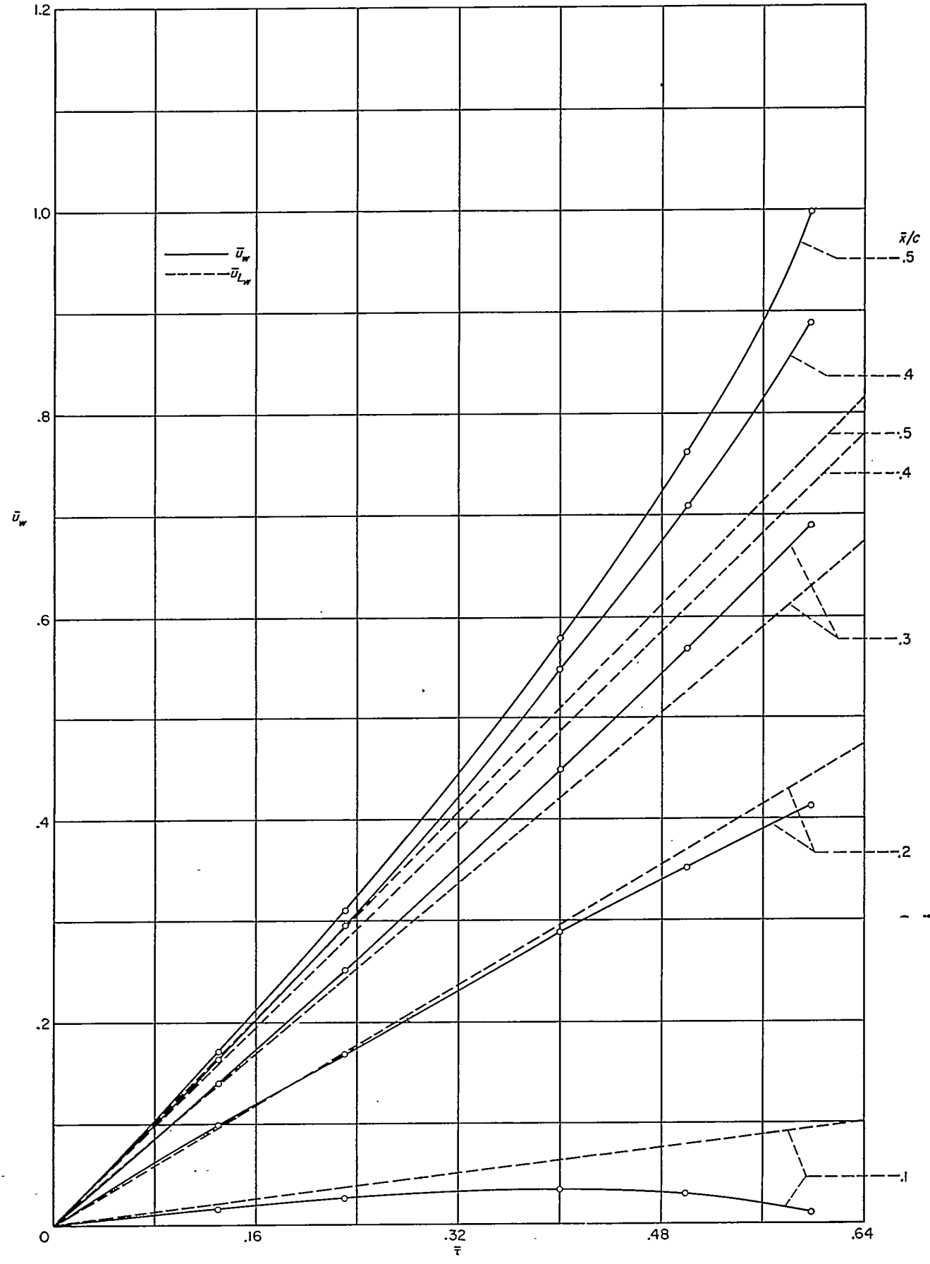
FIGURE 23.—Variation of \bar{u}_w and \bar{u}_{Lw} with \bar{r} for various values of x/c . Subcritical range.
