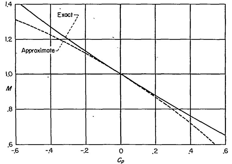
FIGURE 3.—Variation, approximate and exact, of local Mach number with pressure coefficient, M_o = 1 .
