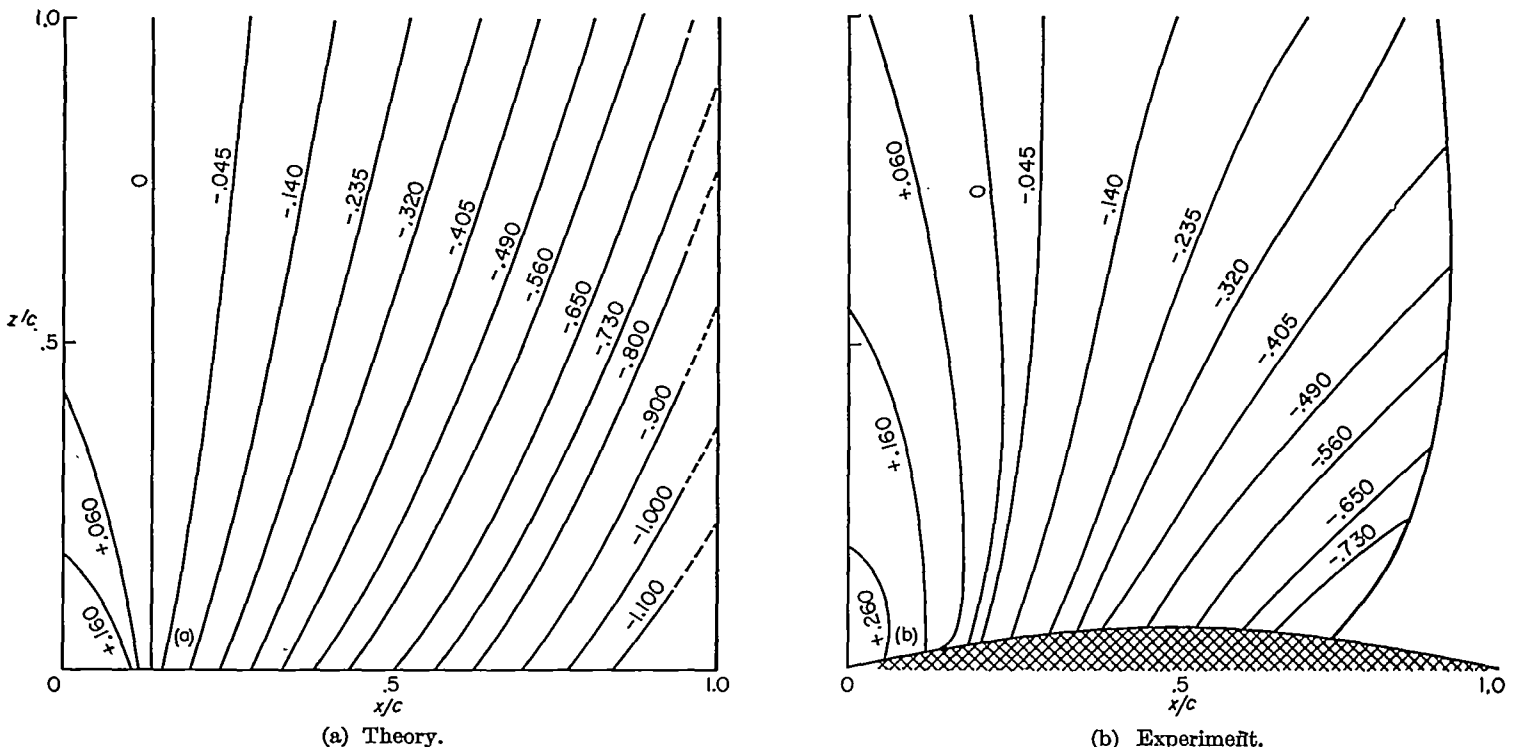
FIGURE 45.—Comparison of theoretical and experimental lines of constant C_p around a 12-percent-thick circular-arc airfoil at a Mach number of 0.88. Experimental data from reference 35 for Reynolds number of 600,000. Turbulent boundary layer.
