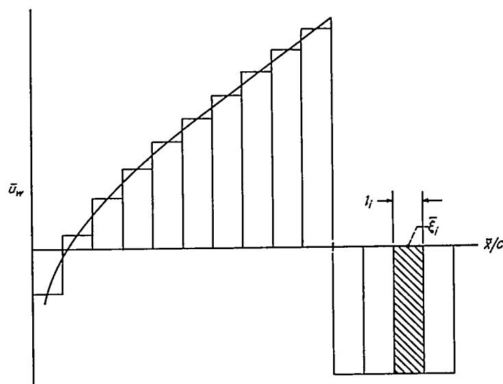
FIGURE 18.—Stepwise approximation used in evaluation of integral when shock wave is at trailing edge.
