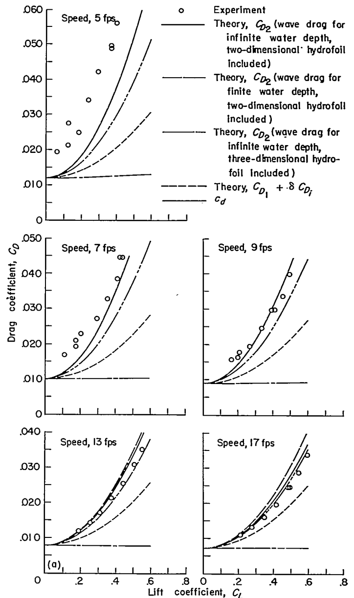
FIGURE 21.—Comparison of experimental and theoretical drag coefficients for aspect-ratio-10 hydrofoil. Water depth, 10.64 feet (tank no. 1).
