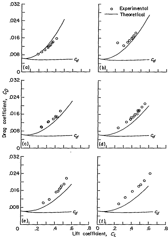
(a) Depth of submergence, 0.53 chord. (b) Depth of submergence, 0.84 chord. (c) Depth of submergence, 1.59 chords. (d) Depth of submergence, 2.34 chords. (e) Depth of submergence, 3.09 chords. (f) Depth of submergence, 3.84 chords.
