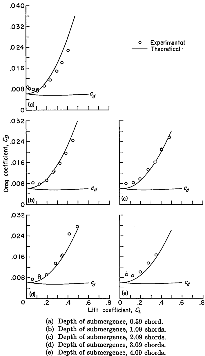
FIGURE 20.—Comparison of experimental and theoretical drag coefficients for aspect-ratio-4 hydrofoil. Speed, 25 fps.
