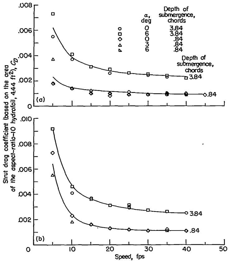
(a) Tank no. 1. (b) Tank no. 2.
