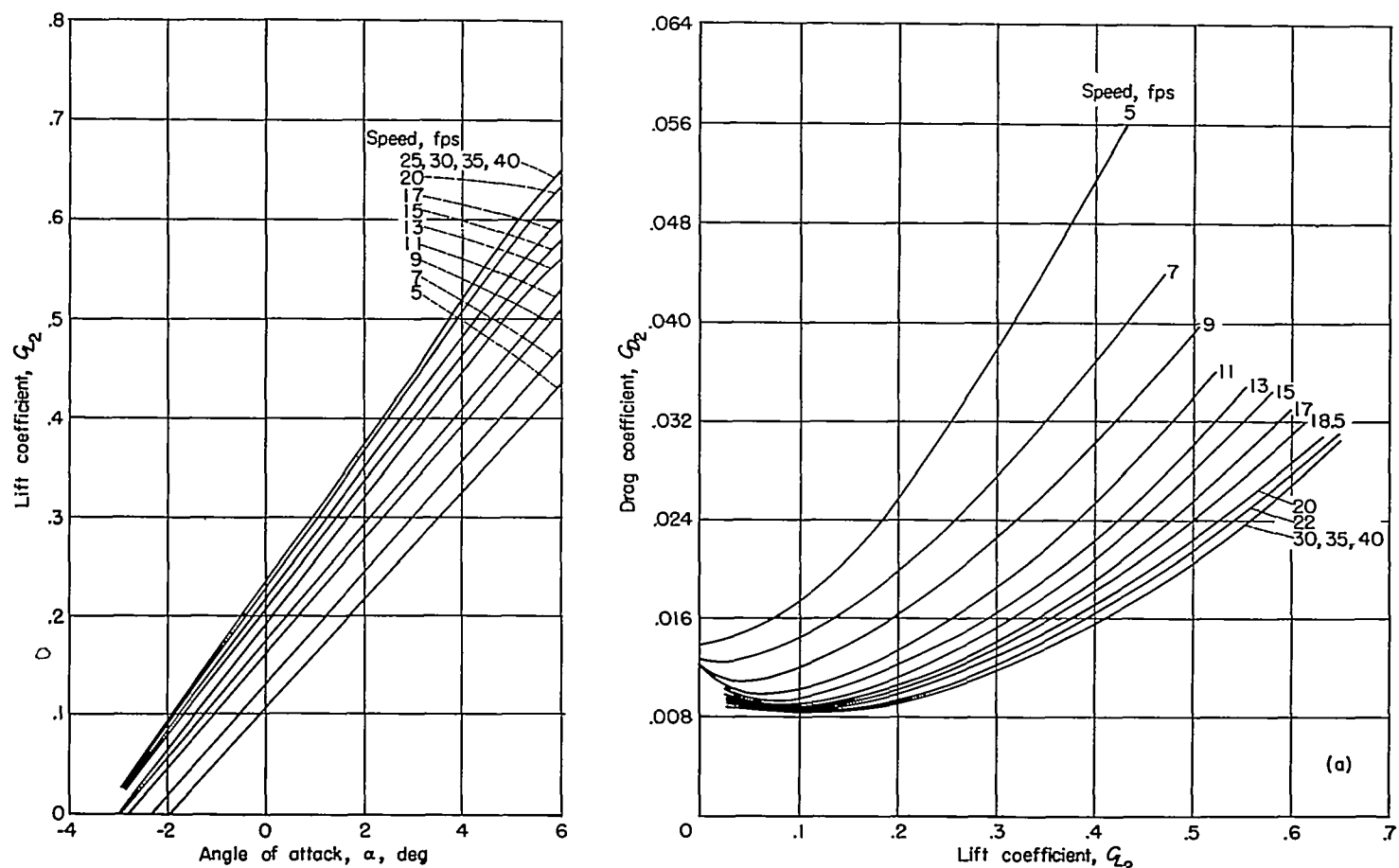
(a) Water depth, 10.64 feet (15.98 chords); depth of submergence, 0.84 chord.
