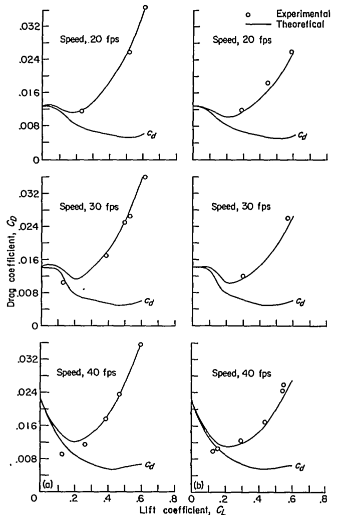
(a) Depth of submergence, 1.0 chord. (b) Depth of submergence, 5.0 chords.
