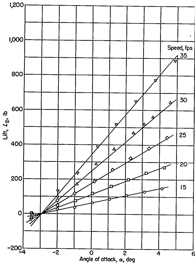
(a) Depth of submergence, 0.59 chord.
