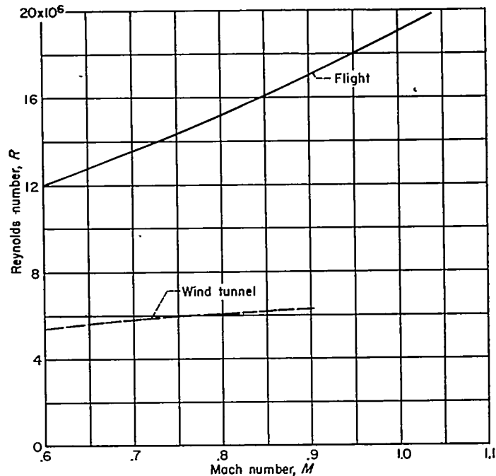
FIGURE 16.—Variation of average Reynolds number with Mach number.
