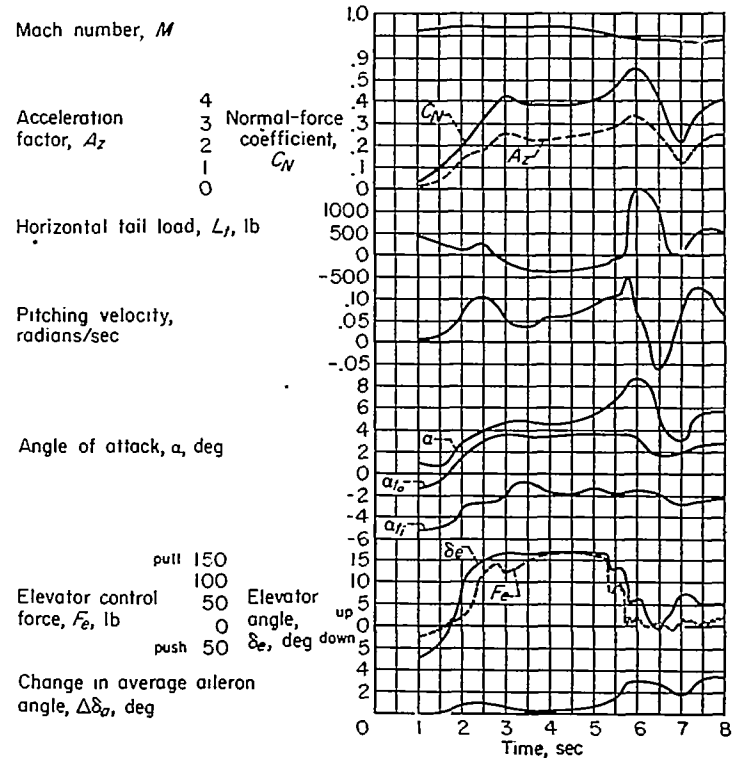
FIGURE 12.—Time-history plot of a pull-out in which a pitch-up occurred as the Mach number decreased.
