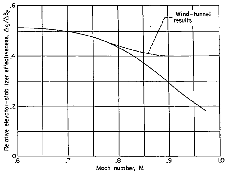
FIGURE 19.—Variation with Mach number of relative elevator-stabilizer effectiveness parameter.
