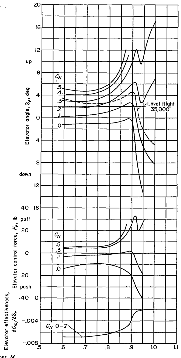
FIGURE 13.—Variation of the longitudinal-control characteristics with Mach number.
