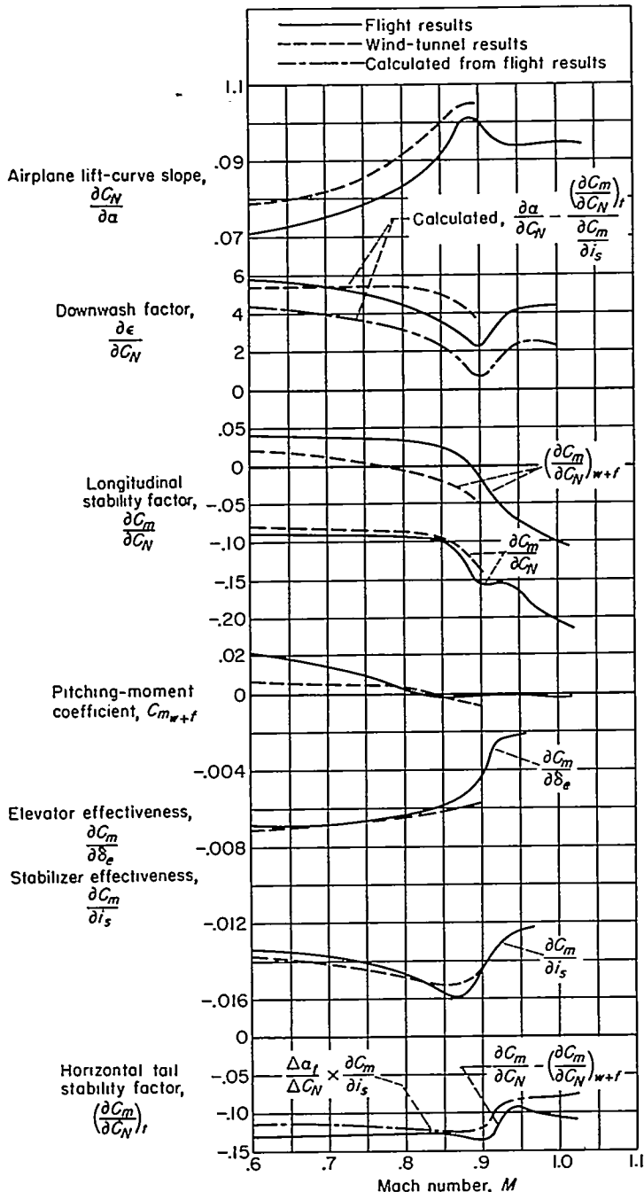
FIGURE 15.—Variation with Mach number of a number of aerodynamic parameters and a comparison with wind tunnel results; steady level flight.
