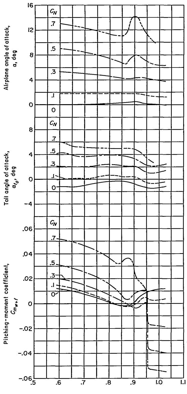
FIGURE 13.—Variation of the longitudinal-control characteristics with Mach number.
