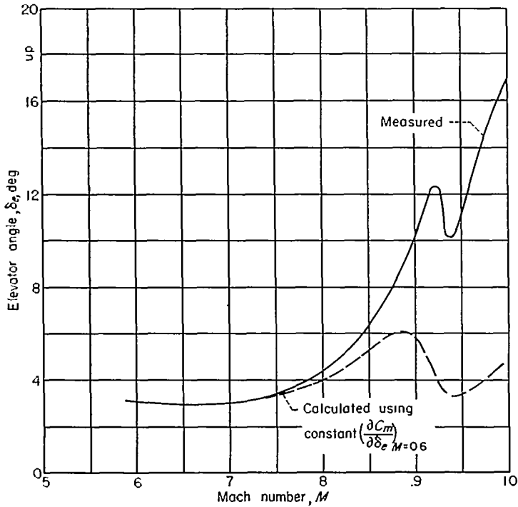
FIGURE 14.—Variation with Mach number of elevator angle required for balance at C_N=0.3 .
