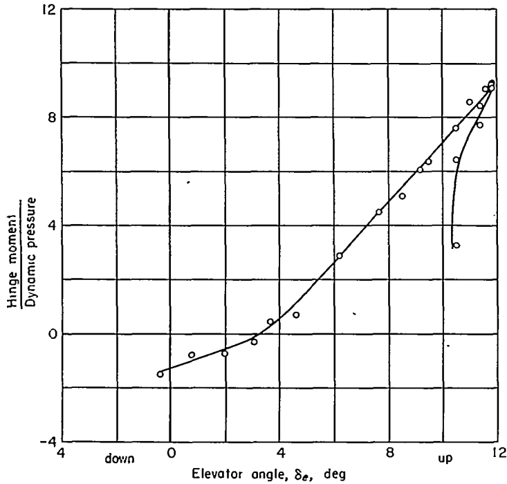
FIGURE 11.—Variation of elevator hinge moment with deflection for wind-up turn; Mach number=0.87.
