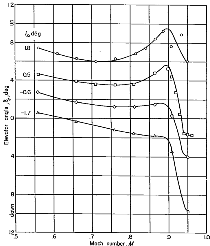
FIGURE 18.—Variation with Mach number of elevator angle required for steady level flight for various stabilizer settings.
