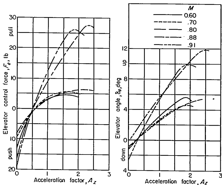
FIGURE 3.—Variation of elevator angle and force with normal acceleration for several Mach numbers.
