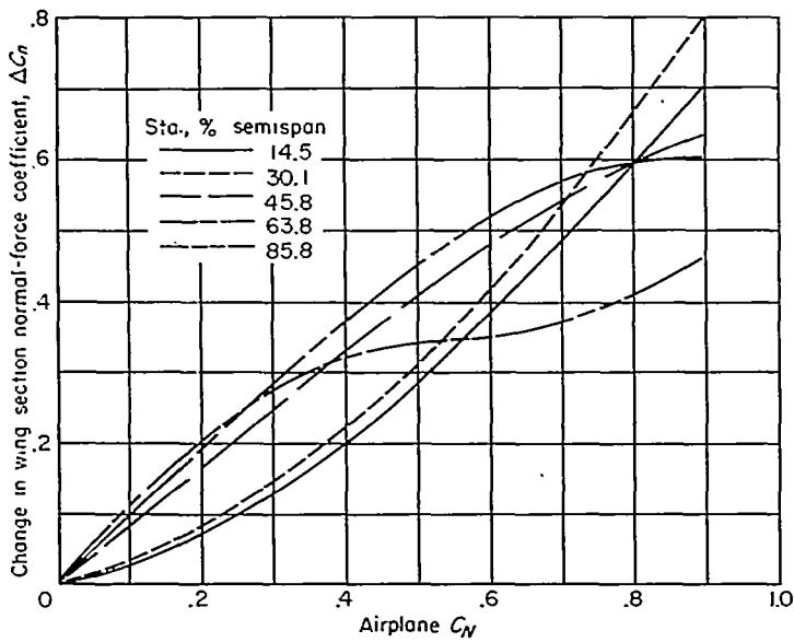
FIGURE 9.—Variation of \Delta c_n with airplane C_N for various spanwise stations; Mach number=0.87.
