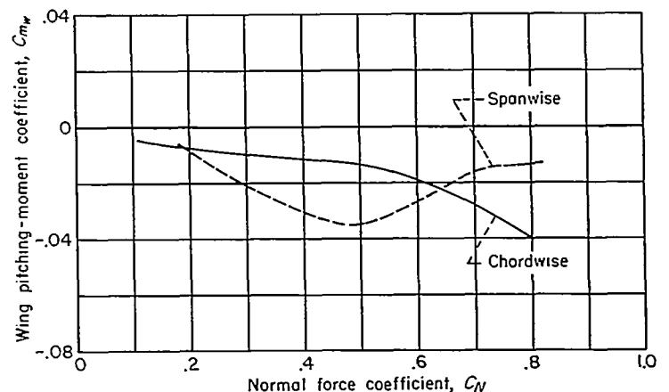
FIGURE 8.—Variation of wing pitching-moment coefficient with airplane normal-force coefficient due to changes in chordwise and spanwise loadings; Mach number=0.87.
