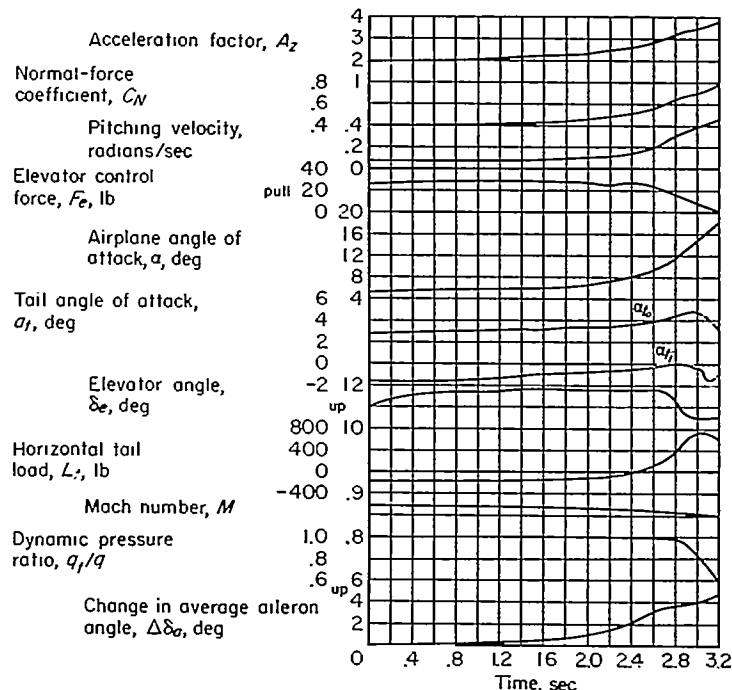
FIGURE 4.—Time-history plot of a pitch-up encountered in a wind-up turn.
