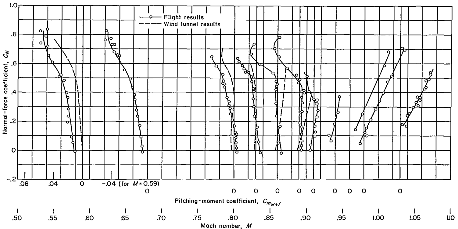
FIGURE 10.—Variation of the wing-fuselage pitching moment with C_N for various Mach numbers.
