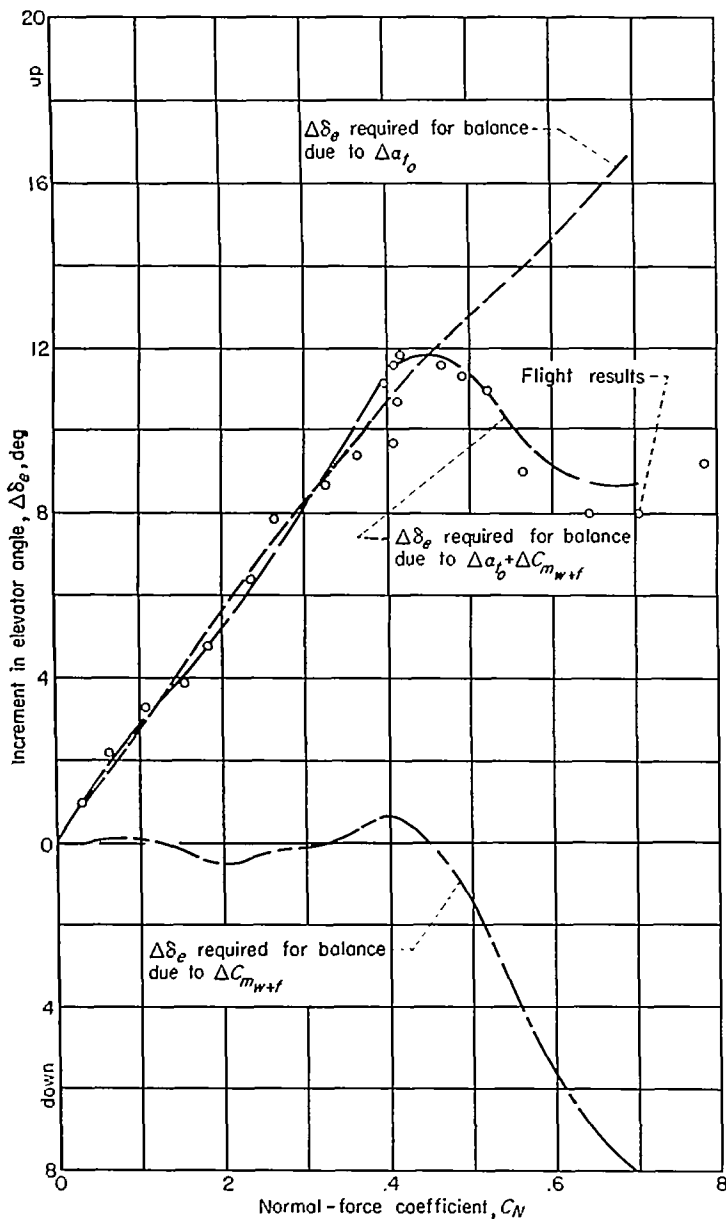
FIGURE 6.—Variation with C_N of elevator angle required for balance; Mach number=0.87.
