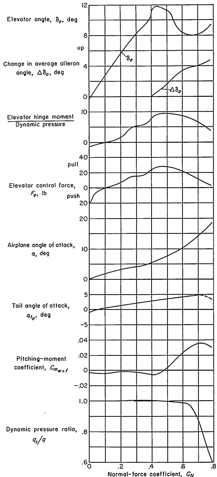
FIGURE 5.—Variation of the longitudinal control characteristics with normal-force coefficient; Mach number=0.87.
