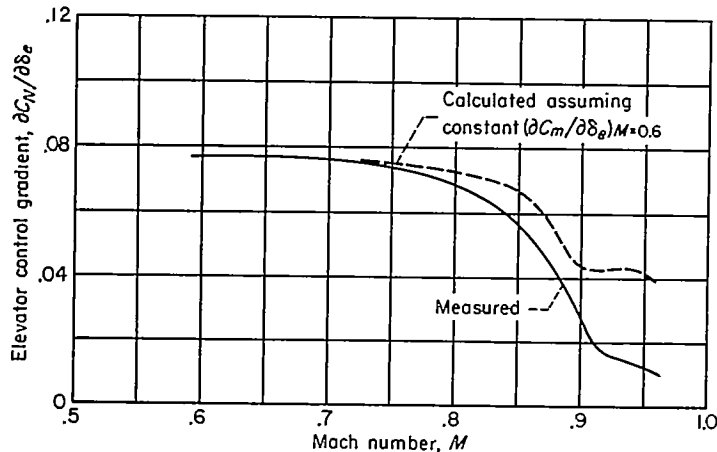
FIGURE 17.—Variation with Mach number of the elevator control gradient.
