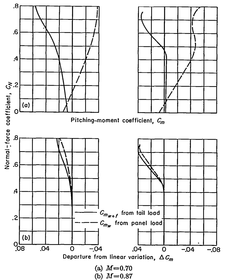
FIGURE 7.—Variation of C_m with C_N as obtained from tail load measurements and wing panel load measurements.
