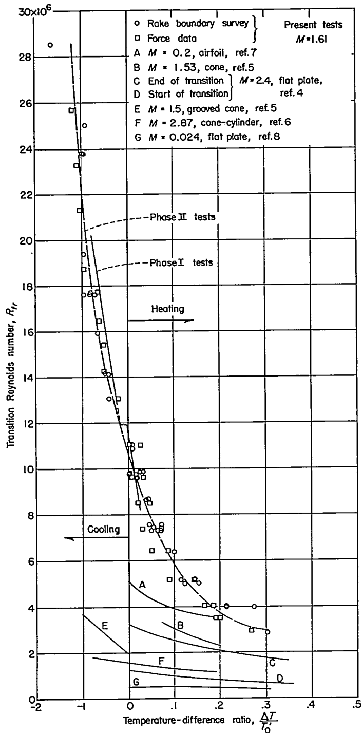
FIGURE 12.—Effect of heating and cooling on boundary-layer transition for present tests and comparison with results from other sources.
