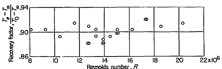
FIGURE 11.—Variation of average model temperature recovery factor with Reynolds number. M=1.61 ; T_0=109^\circ F .
