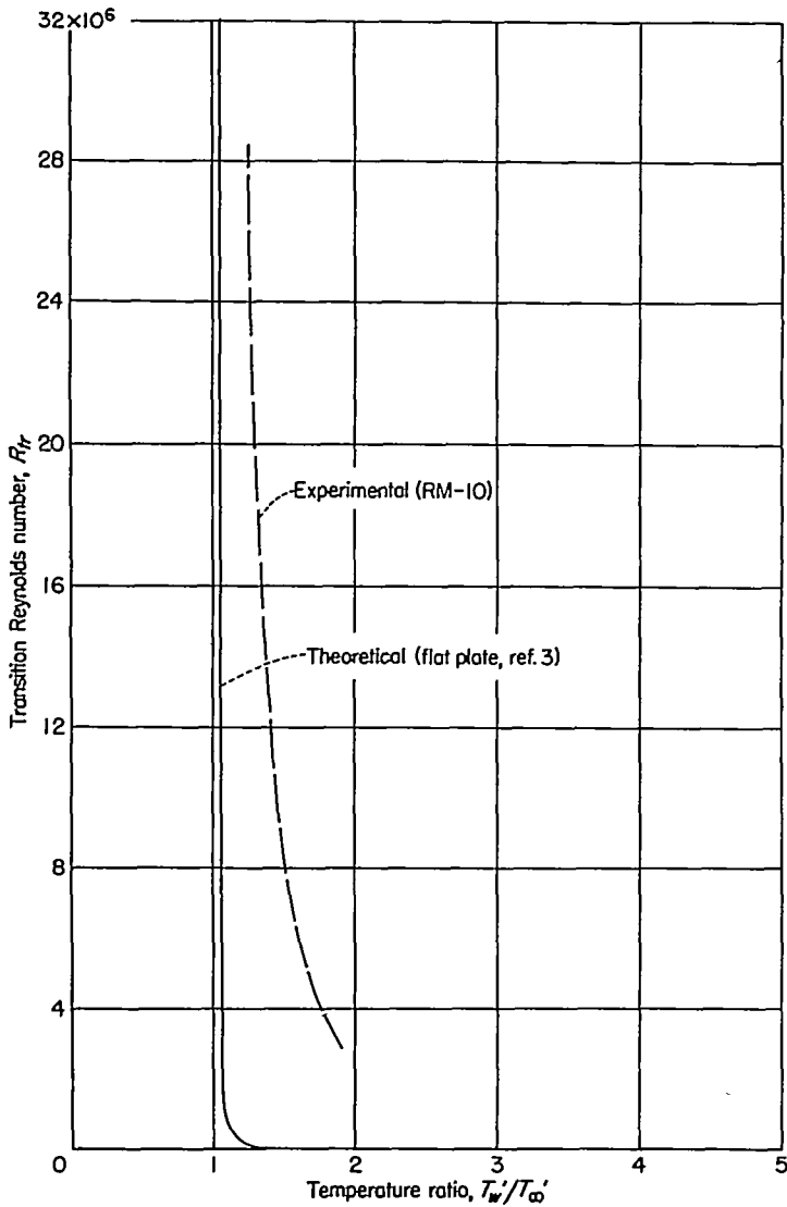
FIGURE 13.—Comparison of experimental transition Reynolds number for NACA RM-10 model and theoretical calculations of boundary-layer stability for flat plate (ref. 3).
