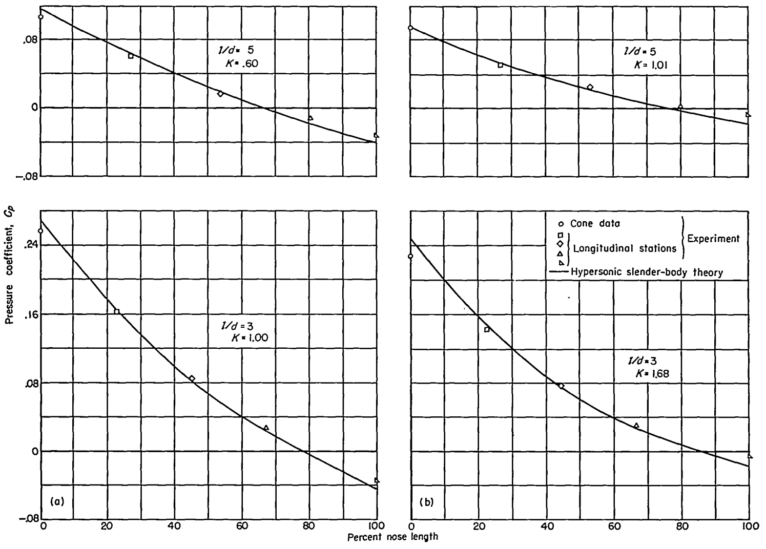
FIGURE 19.—Pressure distributions predicted by hypersonic slender-body theory for ogives at \alpha = 0^\circ .
