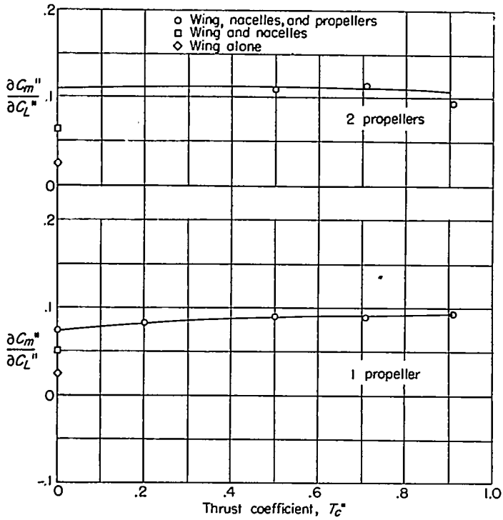
FIGURE 21.—Variation with thrust coefficient of longitudinal stability parameter \partial C_m''/\partial C_L'' near \alpha=0^\circ .
