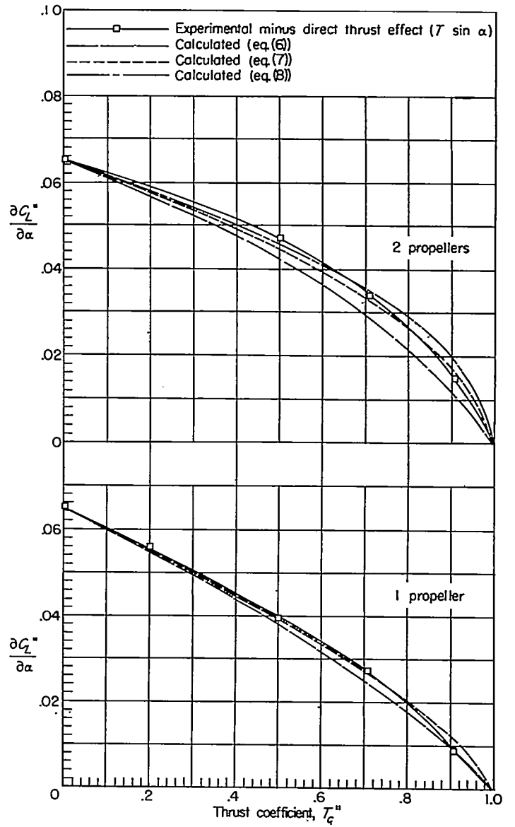
FIGURE 22.—Variation of \partial C_L''/\partial \alpha with thrust coefficient near \alpha=0^\circ .
