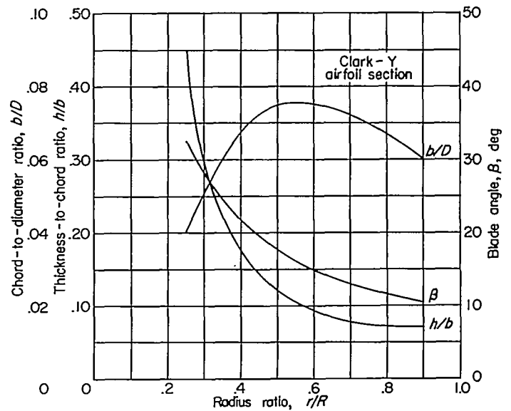
FIGURE 4.—Propeller-blade geometric characteristics.
