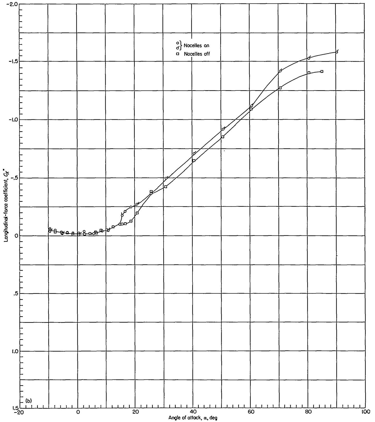
(b) Longitudinal-force coefficient. FIGURE 20.—Continued.
