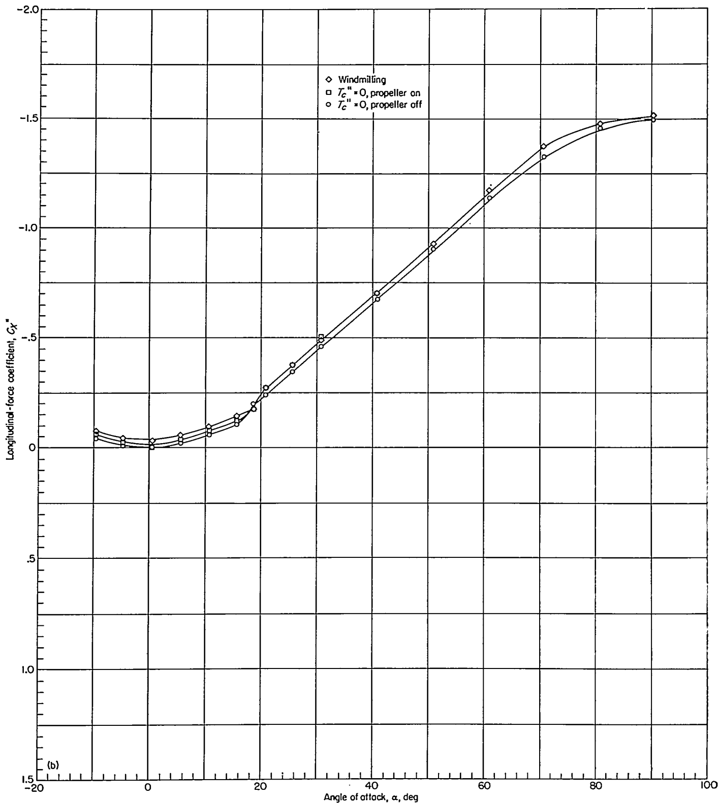
(b) Longitudinal-force coefficient. FIGURE 19.—Continued.
