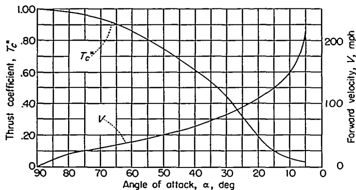
FIGURE 23.—Variation with angle of attack of thrust coefficient required and velocity attained in level flight by assumed airplane. W/S=40 pounds per square foot.
