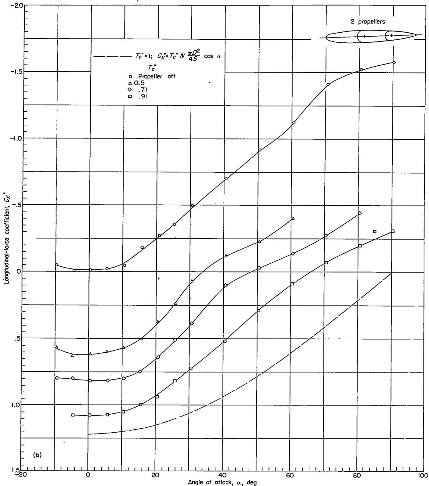
(b) Longitudinal-force coefficient. FIGURE 17.—Continued.
