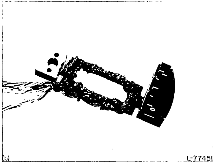
(b) Strain-gage beam used in measuring forces on propeller.
