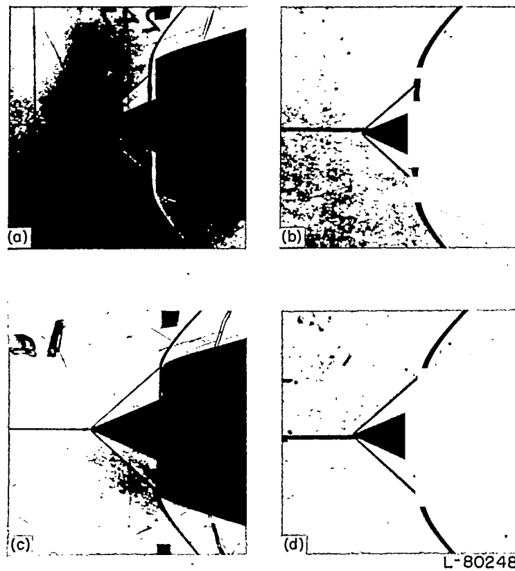
(a) Configuration 4.026-29.82-48.1°; \alpha=0.5^\circ . (b) Configuration 1.278-29.82-48.1°; \alpha=0.5^\circ . (c) Configuration 4.026-29.82-44.2°; \alpha=0.5^\circ . (d) Configuration 1.278-29.82-44.2°; \alpha=0.5^\circ .
