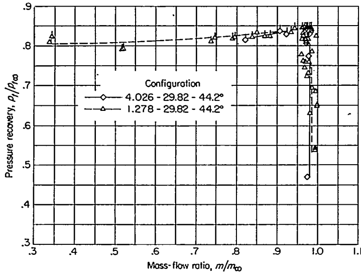
FIGURE 7.—Curves of pressure recovery plotted against mass-flow ratio for configurations 29.82–44.2°. Flagged symbols denote unsteady flow.
