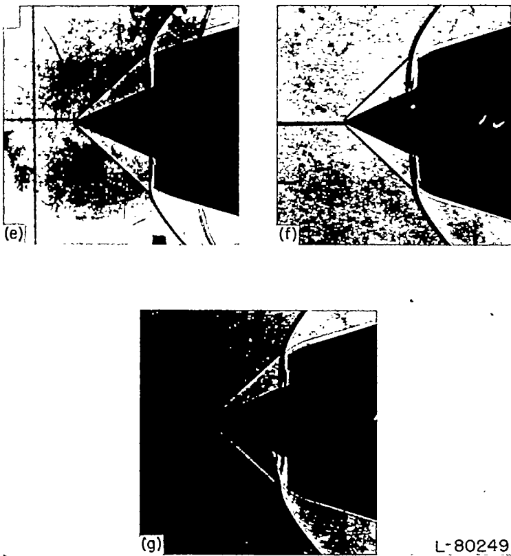
(e) Configuration 4.026-29.82-40.1°; \alpha=0.5^\circ . (f) Configuration 1.278-29.82-40.1°; \alpha=0.5^\circ . (g) Configuration 1.278-14.91-40.1°; \alpha=-0.5^\circ .
