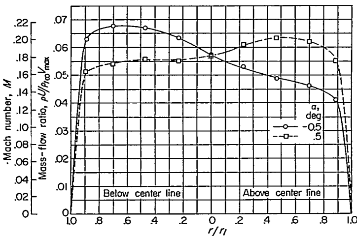
FIGURE 17.—Mass-flow and Mach number profiles at rake survey station for configuration 1.278-14.91-40.1° at angles of attack of ±0.5°.
