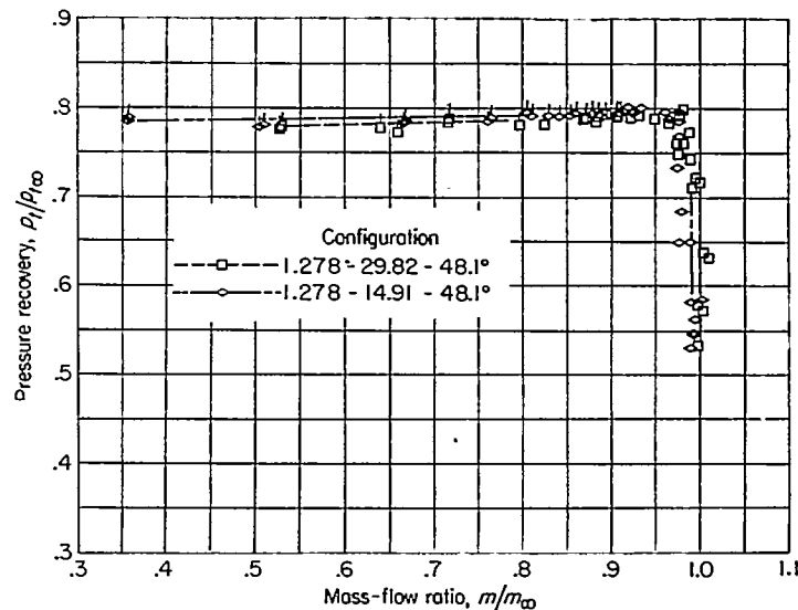
FIGURE 6.—Curves of pressure recovery plotted against mass-flow ratio for configurations 1.278–48.1°. Flagged symbols denote unsteady flow.
