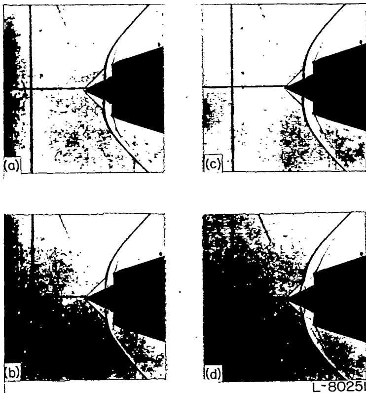
FIGURE 22.—Instantaneous shadowgraphs taken during buzzing of configuration 1.278-14.91-40.1° to show variation in flow pattern at foot of shock when outer part of shock is at same position.
