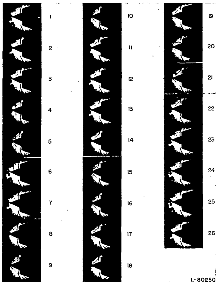
FIGURE 21.—High-speed motion-picture shadowgraphs of isolated spasmodic pulse in buzzing of configuration 1.278-14.91-40.1°.
