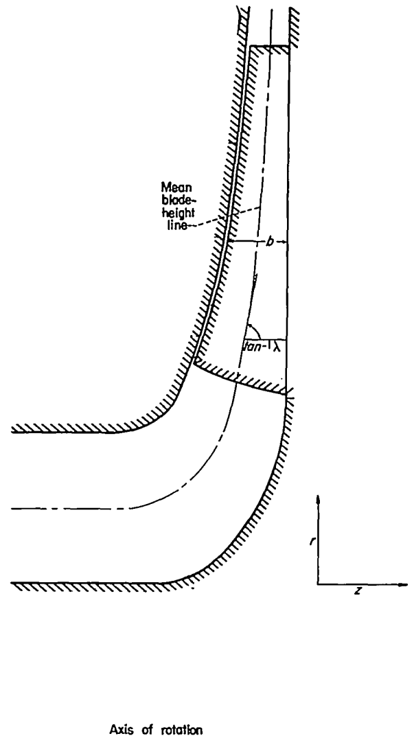
FIGURE 2.—Axial-radial plane view of 48-inch-diameter centrifugal impeller.
