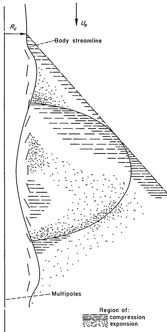
FIGURE 39.—Regions of expansion and compression on wing with fuselage distortion shown.
