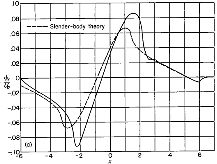
(a) Radial velocities induced by sources. FIGURE 25.—Velocities induced by the elliptic-wing cancellation multipoles at the control surface where \beta R/L_e = 0.148 .
