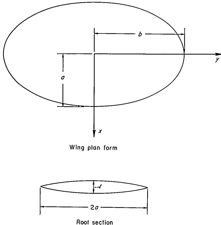
FIGURE 18.—Definition of parameters used to study elliptic wing. 435875-57-47
