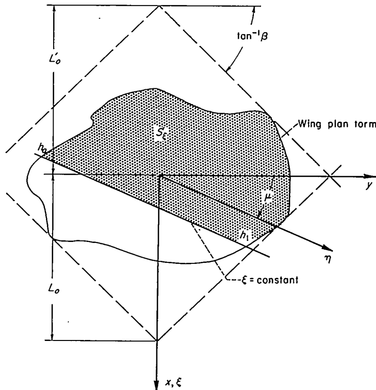
FIGURE 10.—Symbols used in study of multipole properties.
