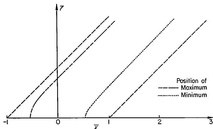
FIGURE 12.—Effective length of multipole distribution.
