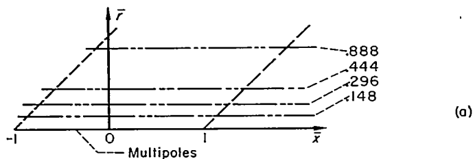
FIGURE 11.—Radial and tangential velocities induced by three different multipole distributions at four radii.
