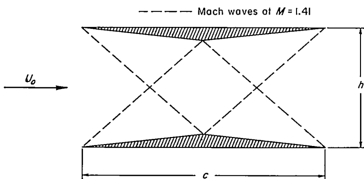
FIGURE 3.—Busemann biplane.
