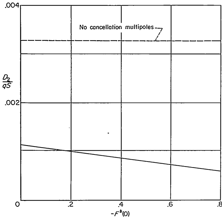
FIGURE 35.—Reduction in drag caused by second-order multipoles.
