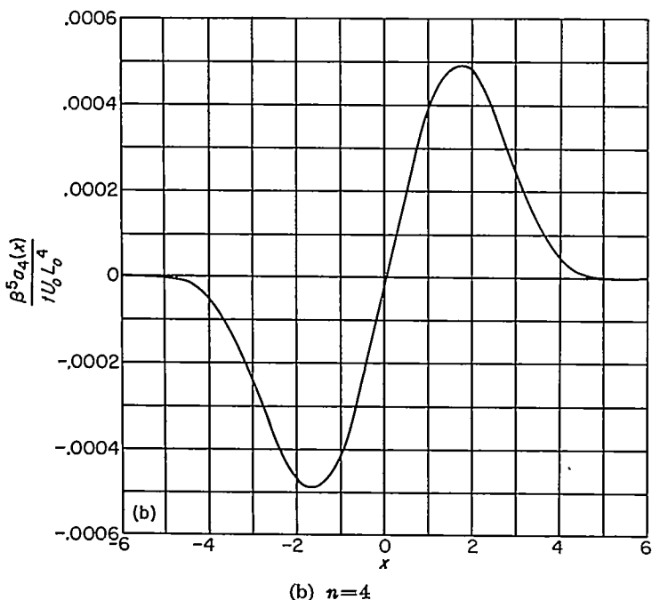
FIGURE 22.—Variation of n th-order cancellation multipoles for elliptic wing.
