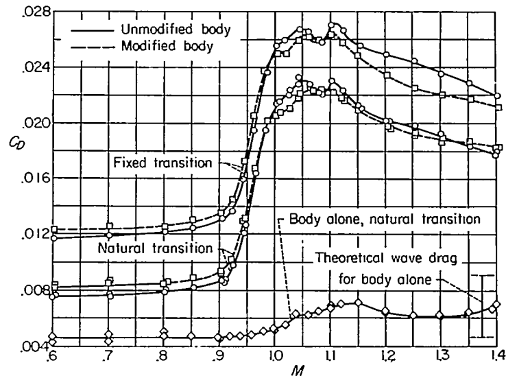
FIGURE 42.—Experimental values for drag coefficient.
