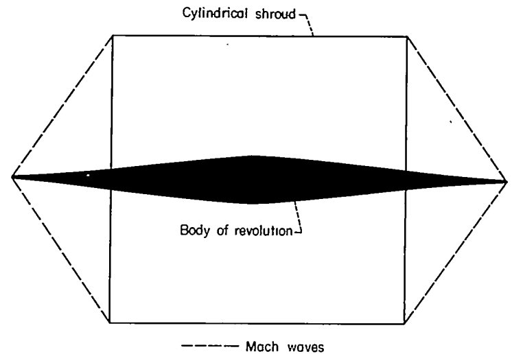
FIGURE 2.—Body and shroud with zero wave drag.
