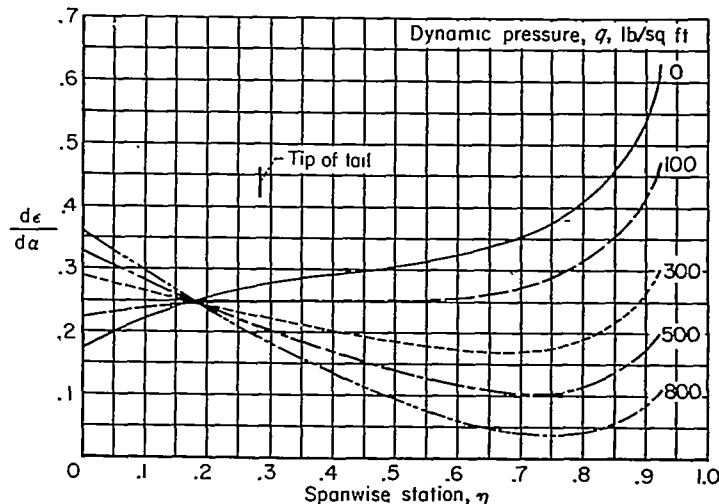
FIGURE 6.—Variation along the swept-tail span of the rate of change of downwash in the plane of the vortex sheet for several values of dynamic pressure for the example airplane as affected by aerodynamic loads only.
