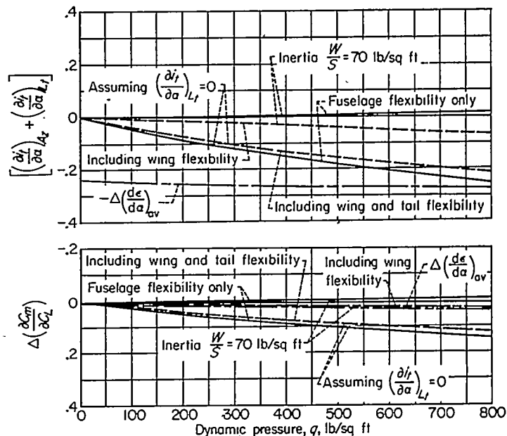
FIGURE 9.—Variation with dynamic pressure, q , lb/sq ft of the factors associated with fuselage flexibility and the stability change due to these factors for the example airplane.
