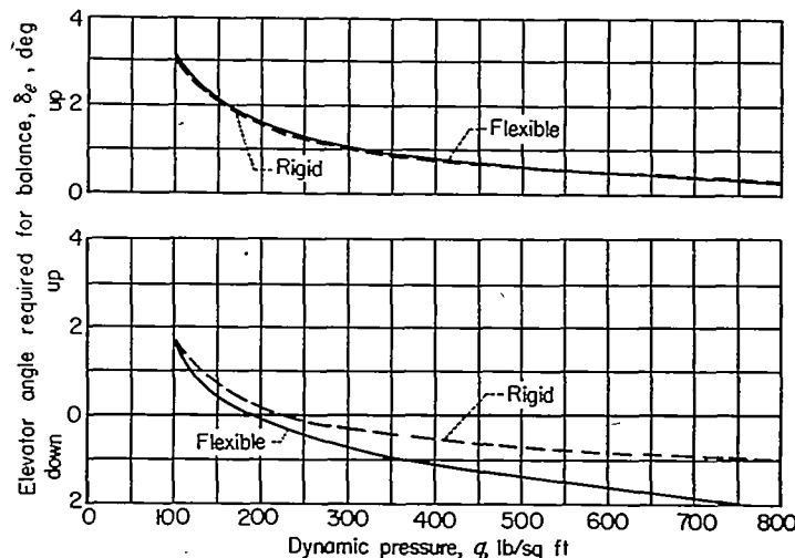
(a) With only up-elevator angle required ( C_{m_0} = 0 ).
