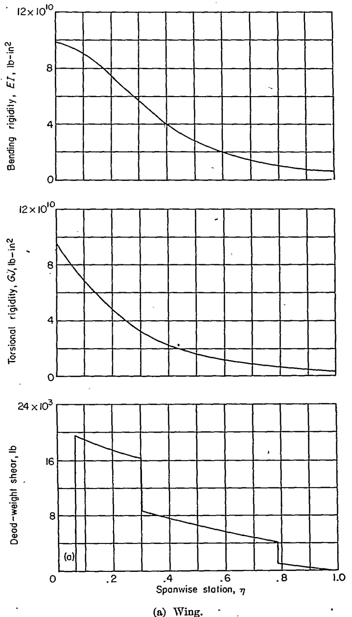
FIGURE 3.—Variation in pertinent structural characteristics across the semispan for the wing and horizontal tail of the example airplane.
