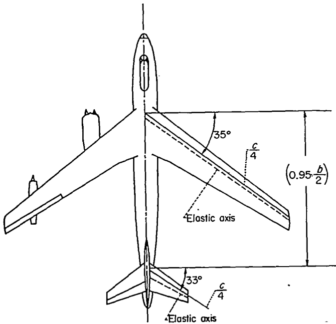
FIGURE 2.—Geometric characteristics of example airplane.
