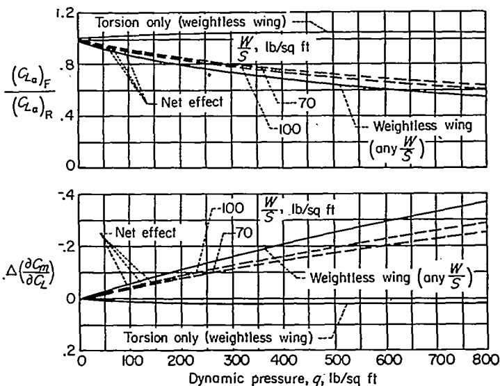
FIGURE 5.—Variation of the ratio of flexible to rigid wing lift-curve slope with dynamic pressure for the example airplane.
