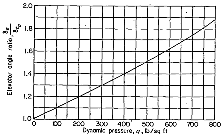
FIGURE 14.—Variation of the elevator angle ratio \delta_e/\delta_0 with dynamic pressure for the example airplane.
