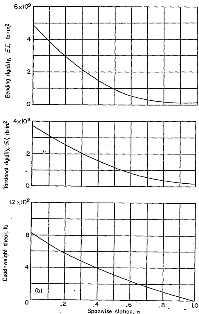
(b) Horizontal tail.
