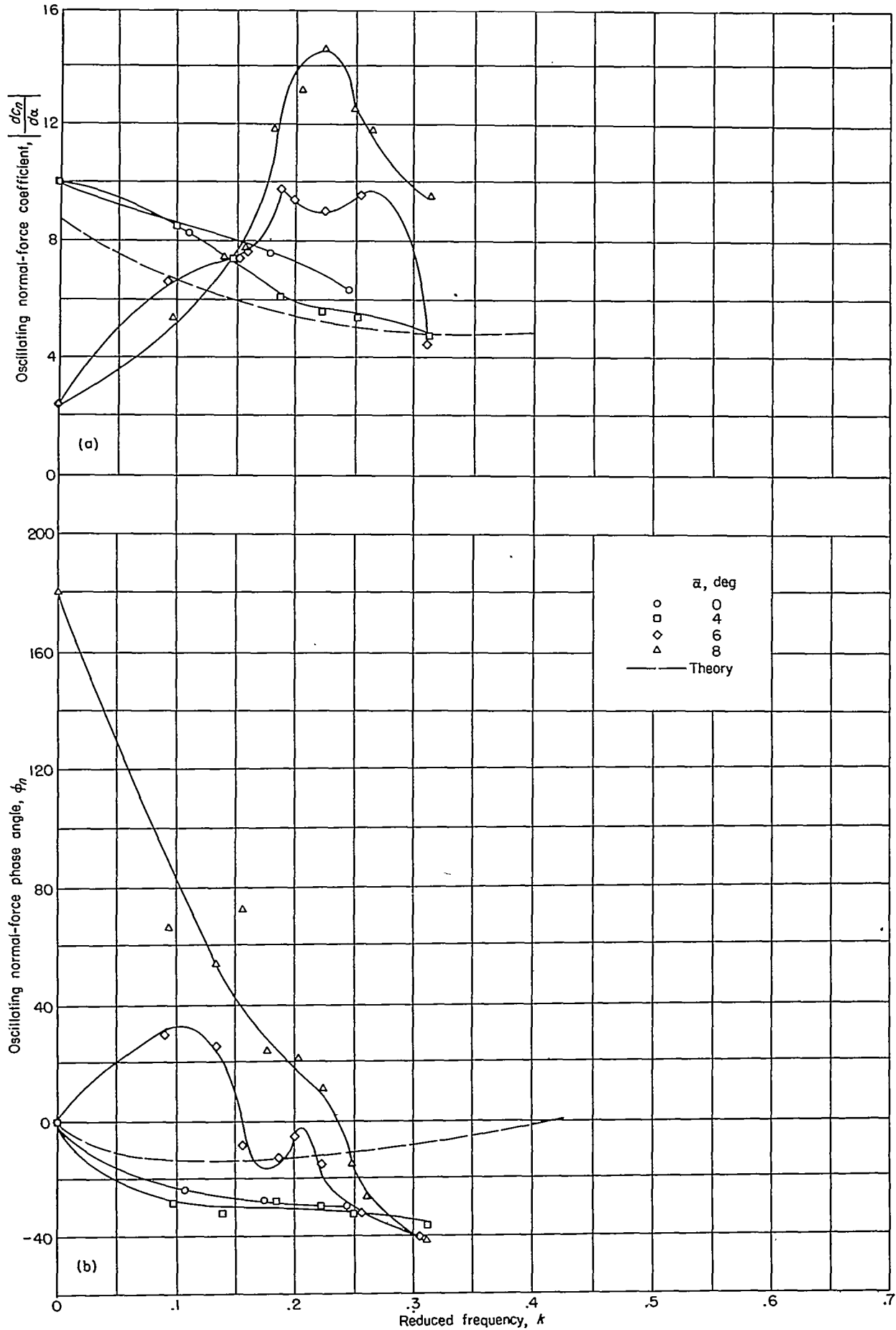
FIGURE 11.—Variation of normal-force coefficient with reduced frequency for two-dimensional 65A010 airfoil oscillating in pitch about the midchord at Mach number of 0.7.
