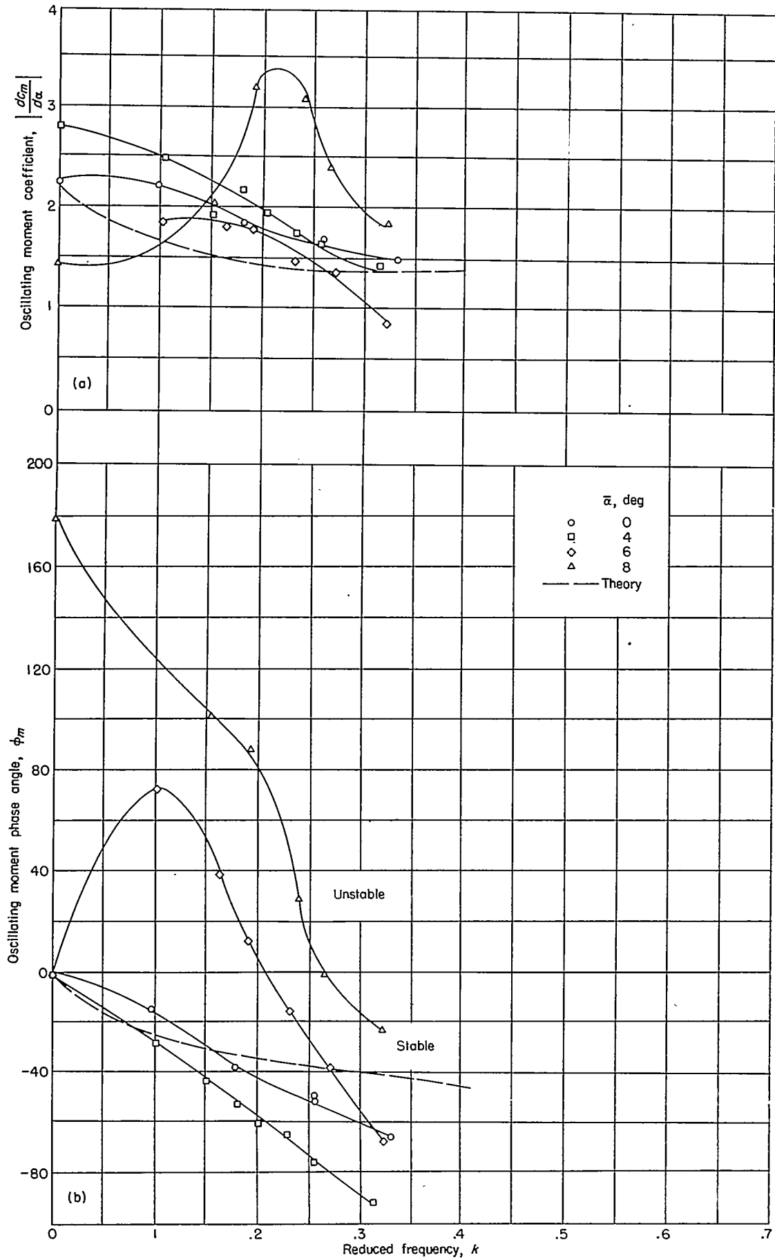
FIGURE 12.—Variation of pitching-moment coefficient with reduced frequency for two-dimensional 65A010 airfoil oscillating in pitch about the midchord at Mach number of 0.7.
