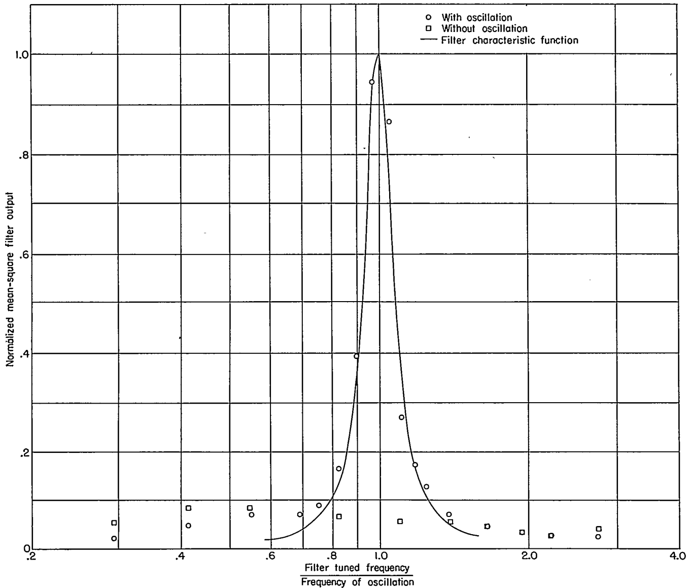
FIGURE 6.—Comparison of normal-force filter output with and without oscillation with filter characteristic function. \alpha=12^\circ ; f=35 ops; and Mach number of 0.35.
