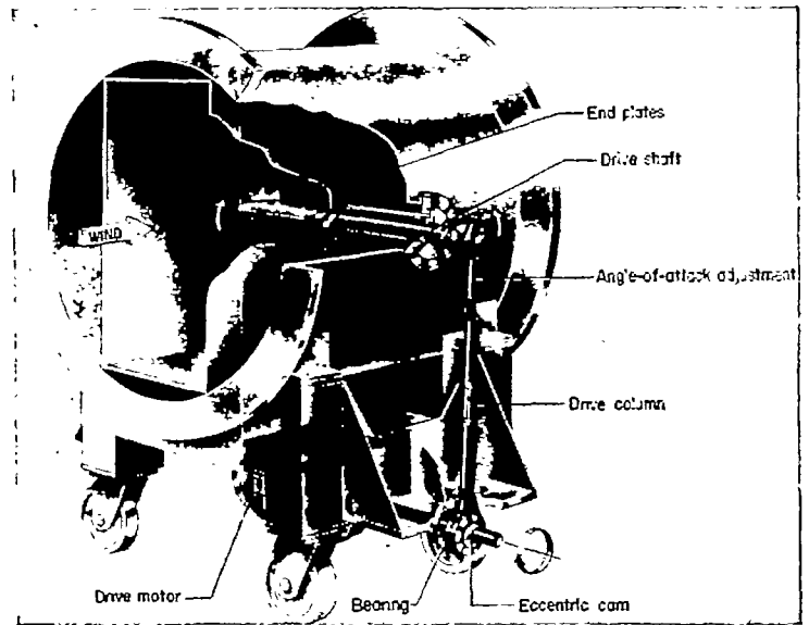
FIGURE 2.—Schematic drawing of model and oscillating mechanism.
