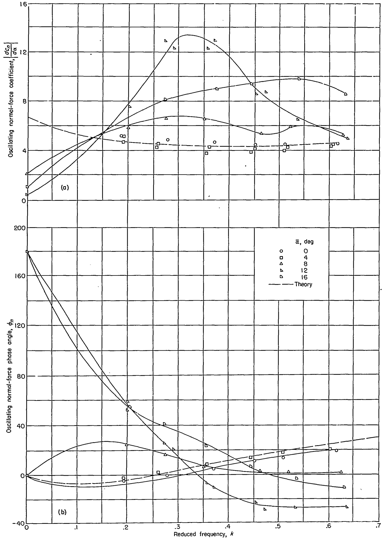
(a) Magnitude. (b) Phase angle. FIGURE 9. —Variation of normal-force coefficient with reduced frequency for two-dimensional 65A010 airfoil oscillating in pitch about the midchord at Mach number of 0.35.
