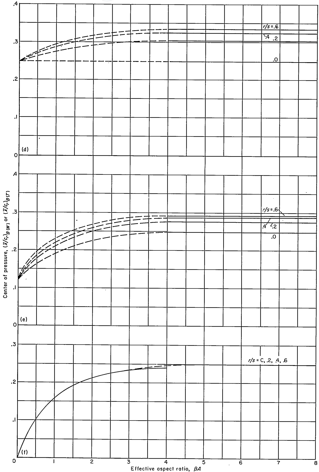
(e) No midchord sweep, \lambda=1/2 .
