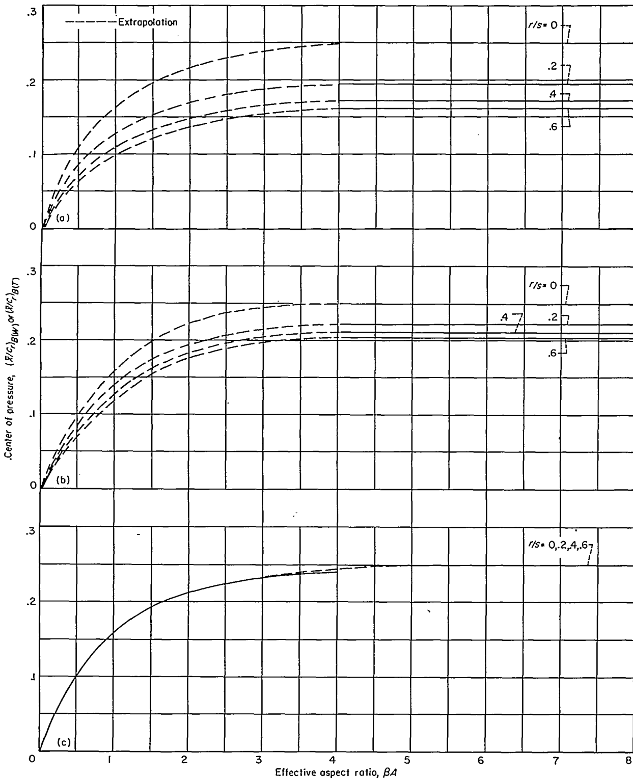
(a) No leading-edge sweep, \lambda=0 .
