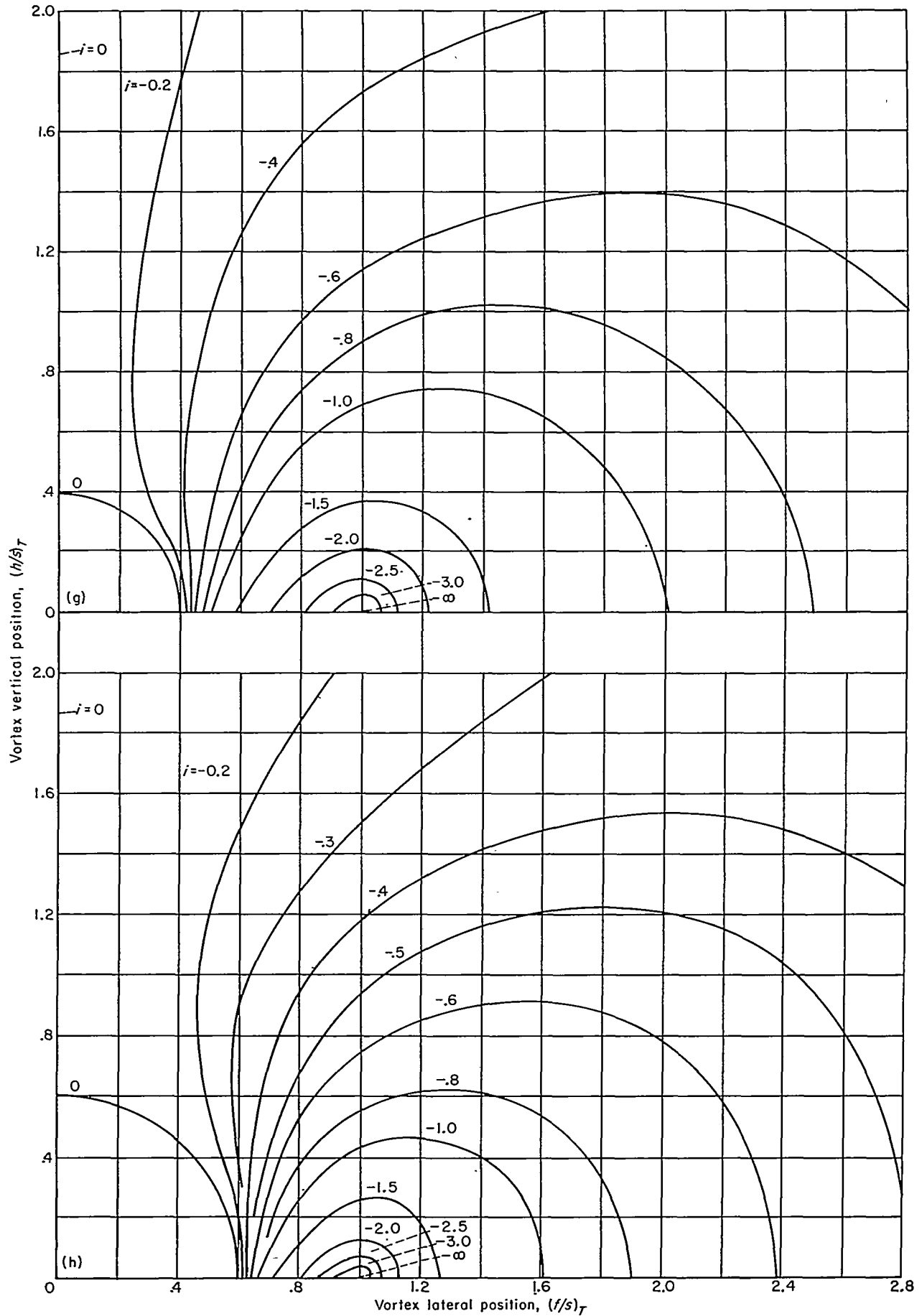
(g) \lambda_T = 1/2, (r/s)_T = 0.4
