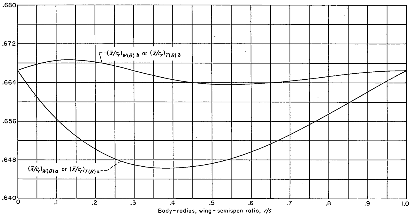
CHART 13.—Center of pressure of lift acting on triangular wing (or tail) panel in combination with a body, from slender-body theory ( \Delta_{TE}=0 ).
