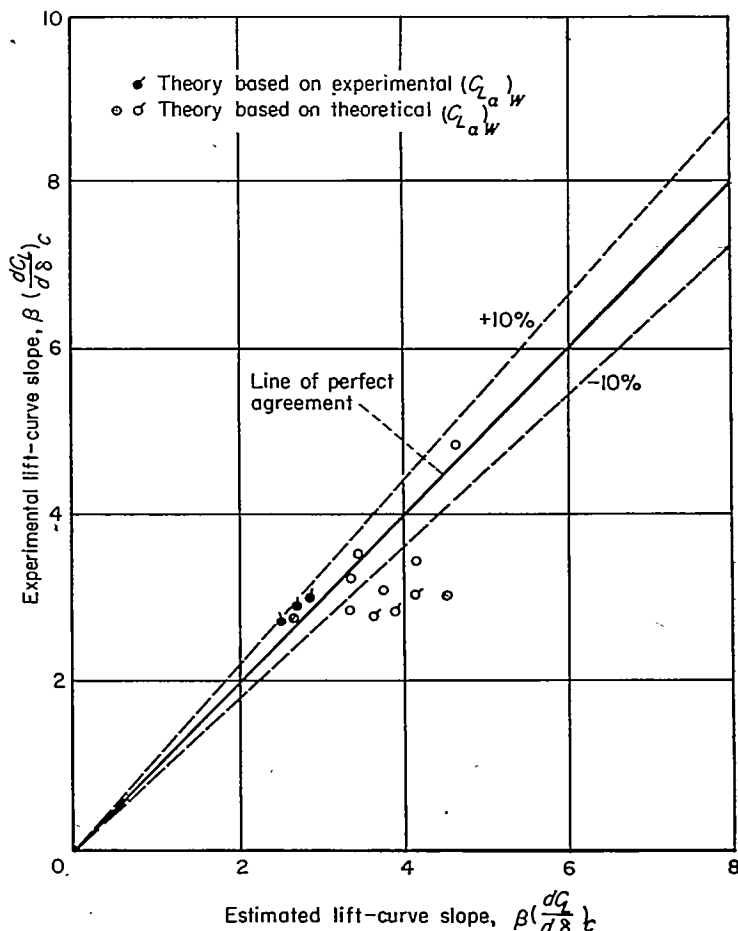
FIGURE 21.—Comparison of experimental and estimated lift-curve slopes for wing-body combinations at \delta=0 .
