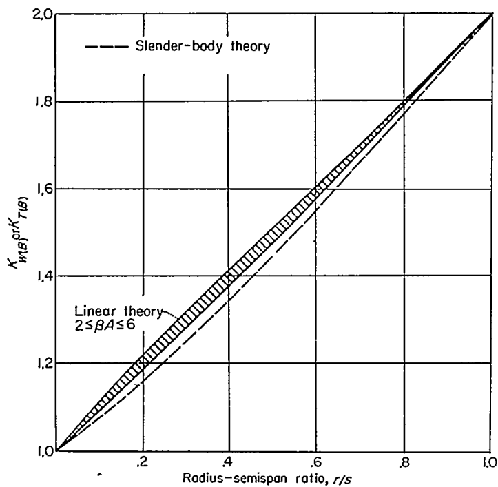
CHART 2.—Values of K_{W(B)} or K_{T(B)} for rectangular wing and body combinations.
