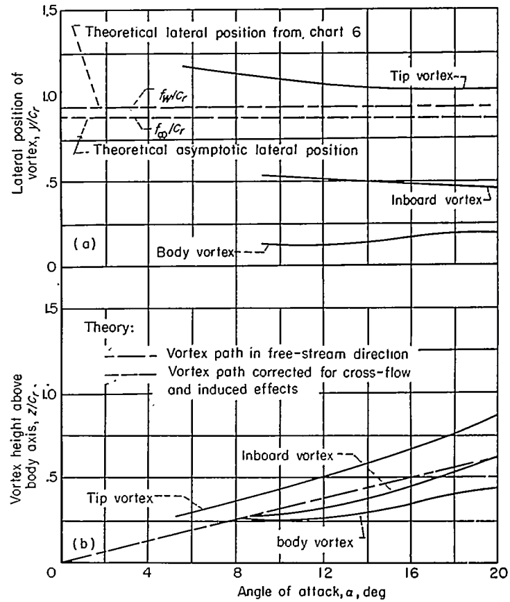
(a) Lateral position of vortex. (b) Vertical position of vortex.
