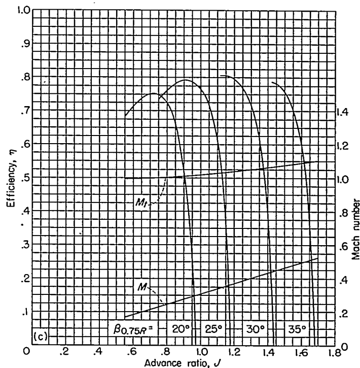
(c) Efficiency.
