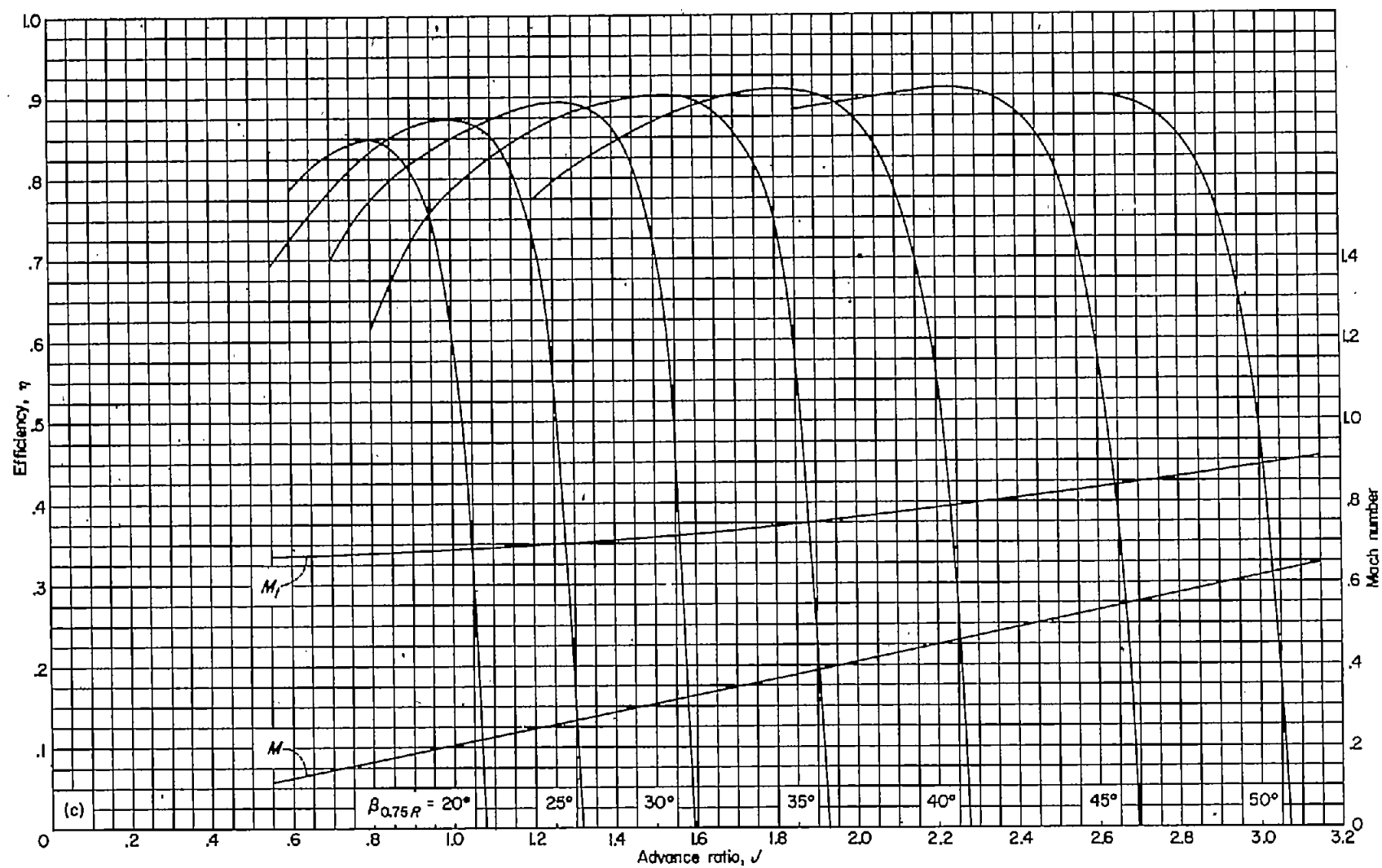
(c) Efficiency.
