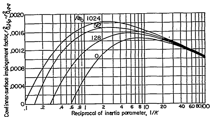
FIGURE 24.—Cowl inner-surface impingement factor. Inlet velocity ratio, 0.7.
