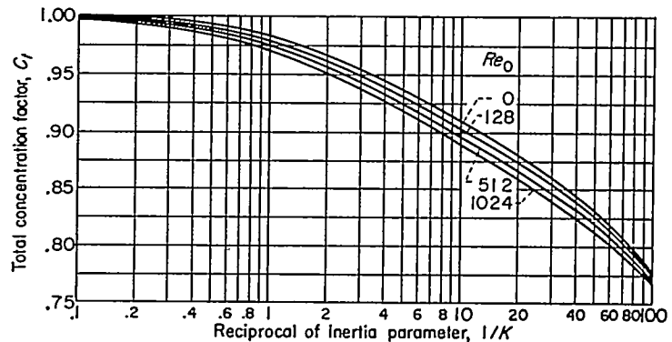
FIGURE 20.—Total concentration factor as function of free-stream Reynolds number and reciprocal of inertia parameter. Inlet velocity ratio, 0.7.
