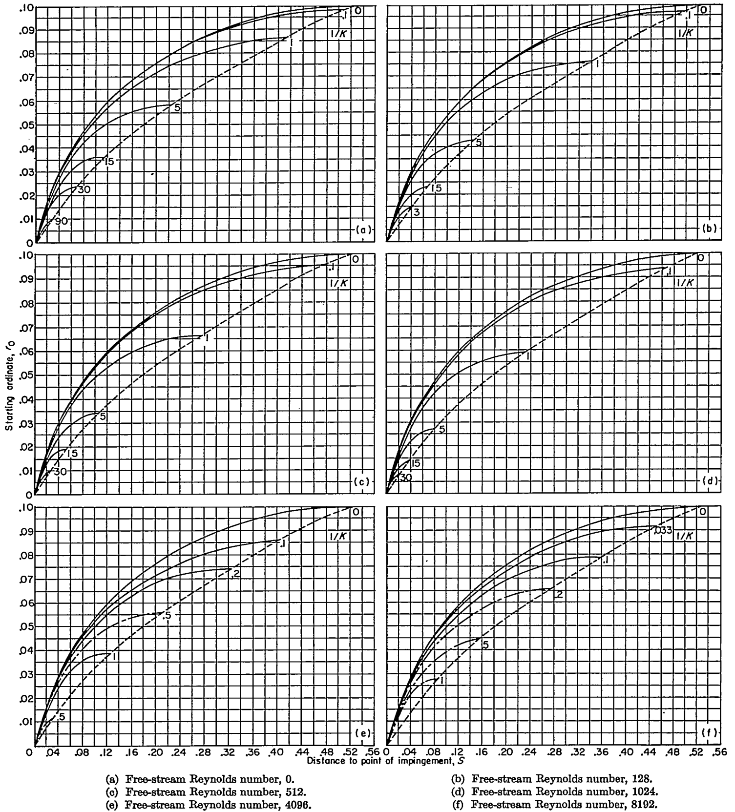
FIGURE 16.—Starting ordinate as function of distance along surface to point of impingement. Basic ellipsoid, 20 percent thick; inlet velocity ratio, 1.0.
