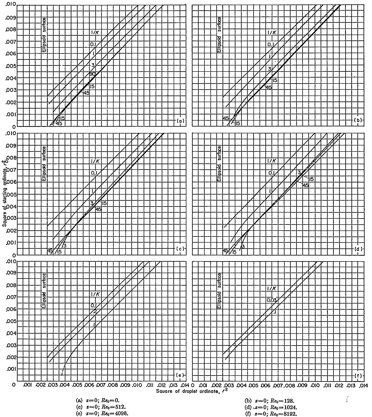
FIGURE 7.—Square of starting ordinate as function of square of droplet ordinate at constant axial position. Basic ellipsoid, 10 percent thick; inlet velocity ratio, 1.0.
