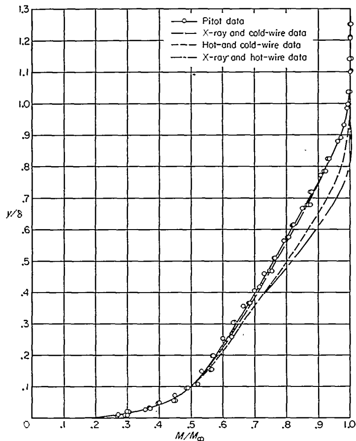
FIGURE 11.—Mach number distributions through the turbulent boundary layer from pitot, X-ray, cold-wire, and hot-wire data.
