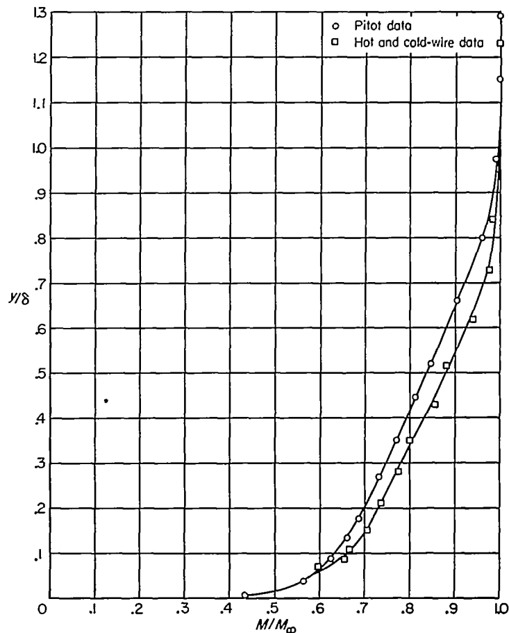
FIGURE 12.—Mach number distributions through the turbulent boundary layer on the side wall of the Ames 1-by 3-foot supersonic wind tunnel from pitot, cold-wire, and hot-wire data; M_\infty = 1.95 , \delta = 2.84 inches.
