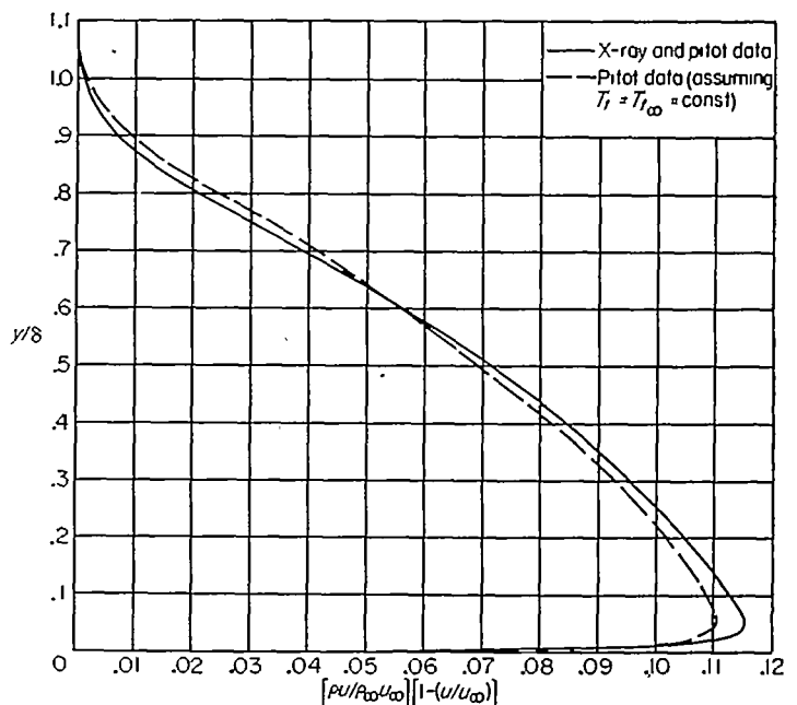
FIGURE 16.—Momentum-loss distributions through the turbulent boundary layer.
