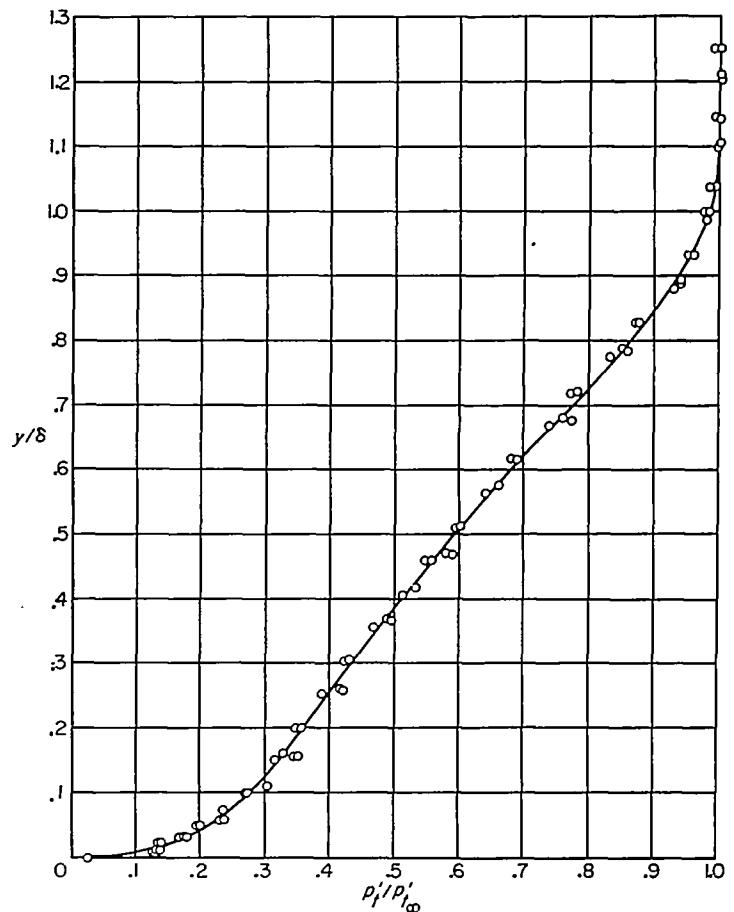
FIGURE 7.—Pitot-pressure distribution through the turbulent boundary layer from pitot-probe measurements.
