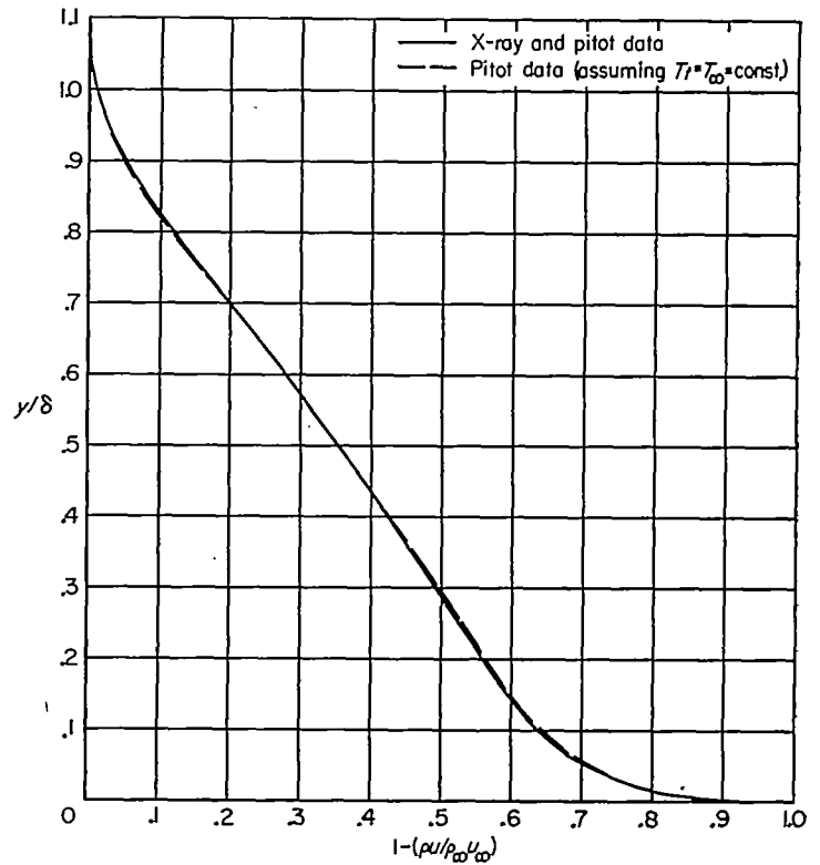
FIGURE 15.—Mass-flow-defect distributions through the turbulent boundary layer.
