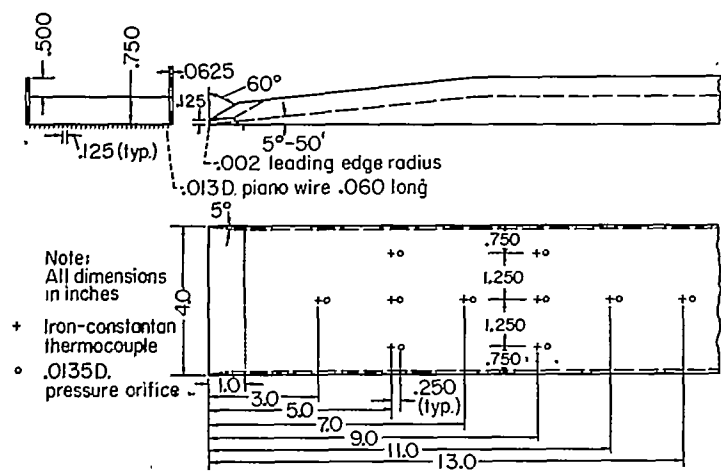
FIGURE 3.—Sketch of flat plate.
