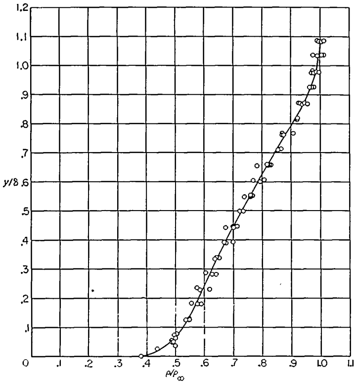
FIGURE 8.—Density distribution through the turbulent boundary layer from X-ray densitometer measurements.
