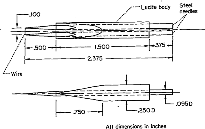
FIGURE 4.—Wire probe.
