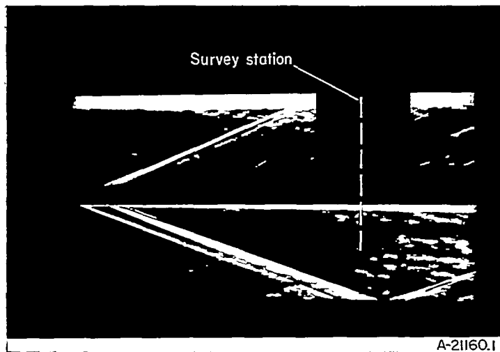
FIGURE 6.—Schlieren photograph of turbulent boundary layer on the flat plate.
