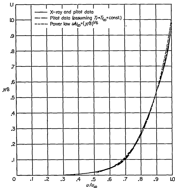
FIGURE 17.—Velocity distributions through the turbulent boundary layer.
