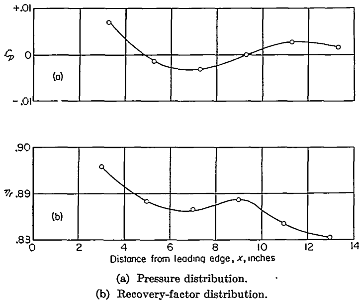
FIGURE 5.—Surface-pressure and recovery-factor distributions along the center line of the flat plate.
