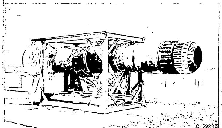
FIGURE 5.—Thrust stand with engine B installed.
