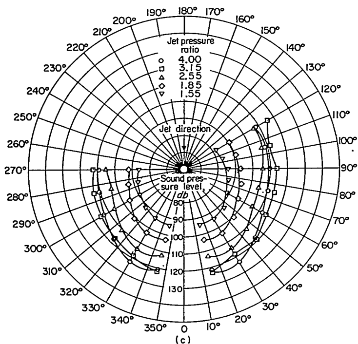
(a) Conical plug; design pressure ratio, 4.0. (c) Isentropic plug; design pressure ratio, 4.0.
