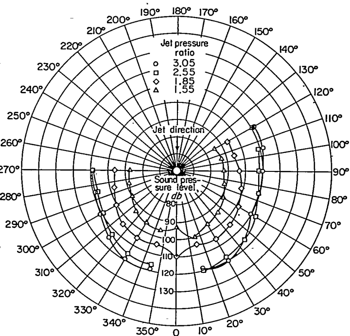
FIGURE 31.—Sound polar diagram of 4-inch-diameter convergent-divergent nozzle for range of pressure ratios. Distance from jet exit, 50 feet.
