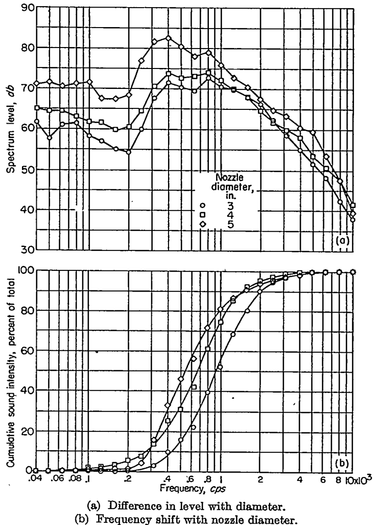
FIGURE 15.—Effect of convergent nozzle diameter on sound spectra. Jet pressure ratio, 1.85; azimuth, 30°.
