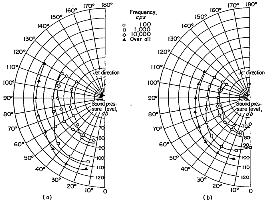
FIGURE 27.—Directional distribution of noise from 4-inch-diameter air jet. Distance from jet exit, 50 feet.
