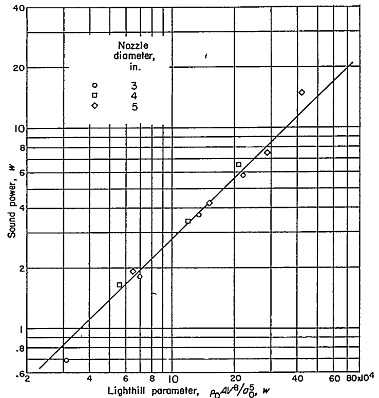
FIGURE 9.—Sound power as function of Lighthill parameter (ref. 3) for three circular convergent nozzles. Pressure ratio, less than 1.89.
