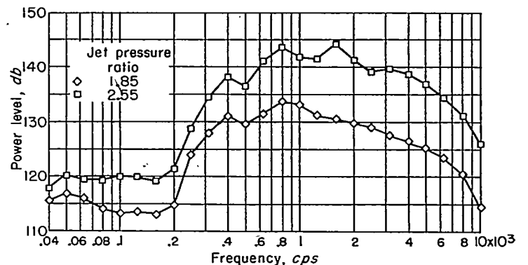
FIGURE 16.—Sound-power spectra of jet discharging from 4-inch-diameter circular convergent nozzle at several pressure ratios.
