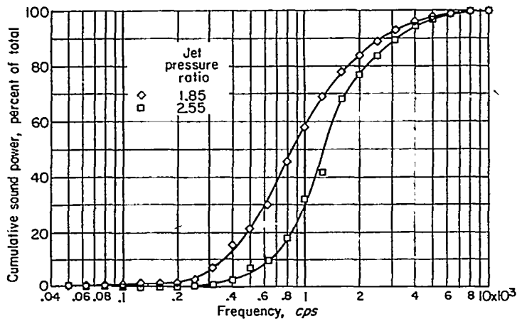
FIGURE 17.—Cumulative sound power of jet discharging from 4-inch-diameter circular convergent nozzle at several pressure ratios.
