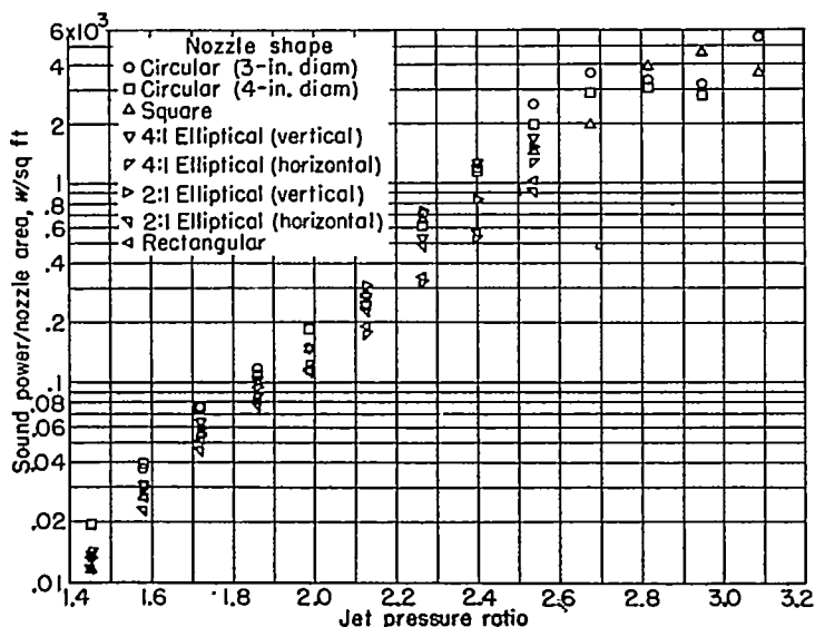
FIGURE 11.—Effect of nozzle shape on sound-power generation.
