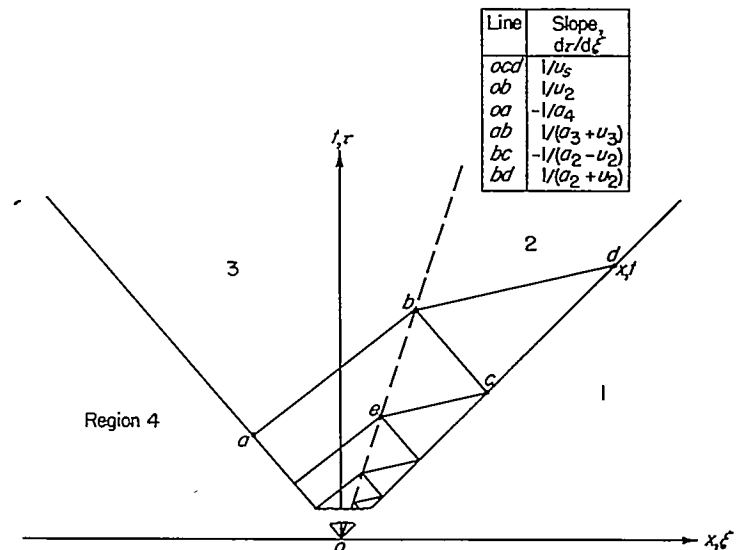
FIGURE 2.—Characteristic lines appropriate for study of attenuation in shock tube.
