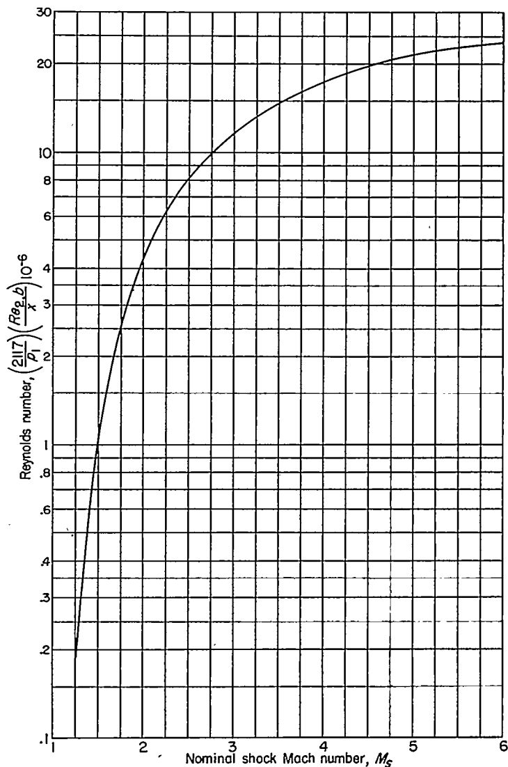
FIGURE 3.—Reynolds number at point b for air in region 1 at 520° R. Re_{2,b} = v_{22} Re_{2,b} (appendix H).
