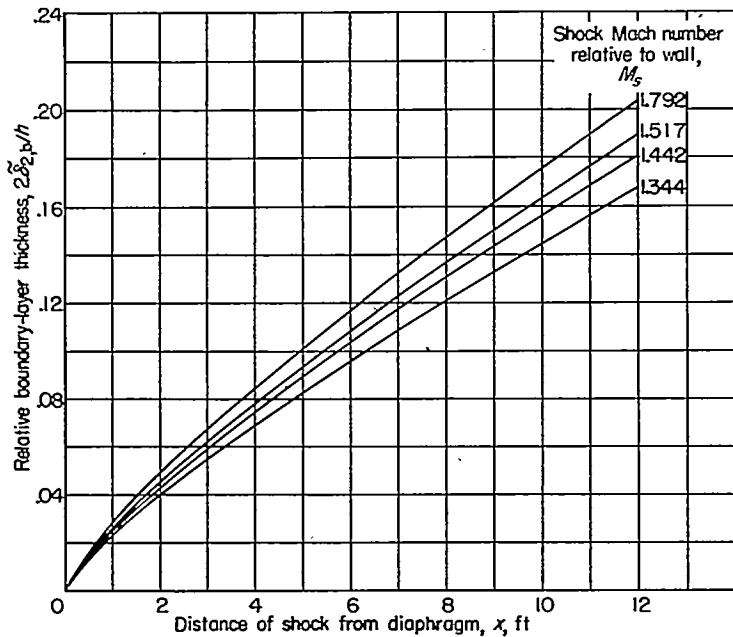
FIGURE 8.—Relative boundary-layer thickness at point b of region 2 for experimental conditions of reference 6 (air in region 1; turbulent boundary layer; T_1 = T_{2,\infty} = 520^\circ \text{R} ; h , 1/8 ft).
