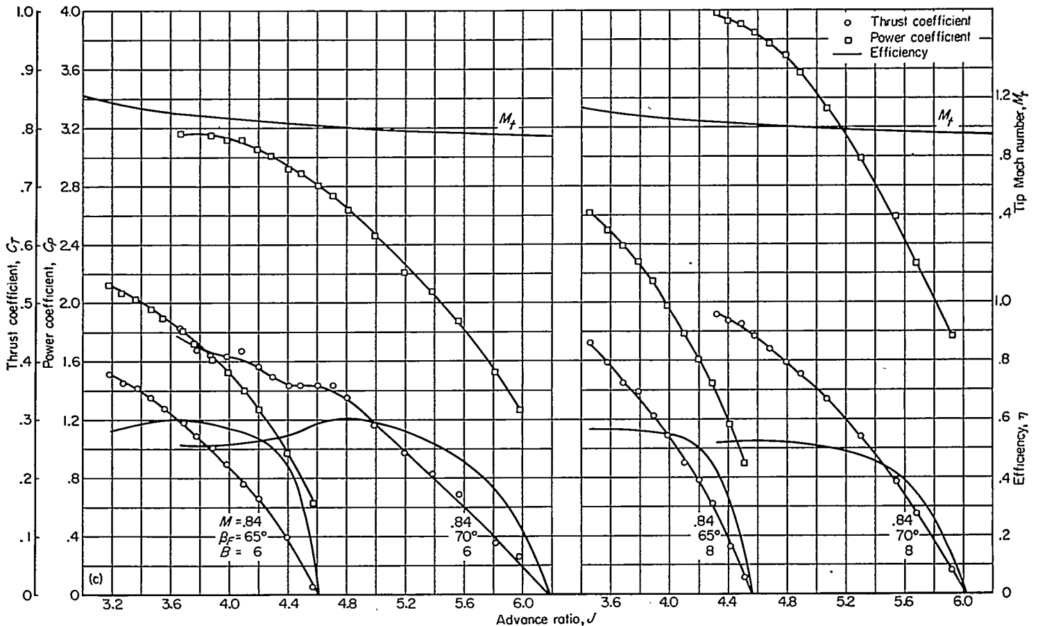
(c) M=0.84 FIGURE 13.—Concluded.
