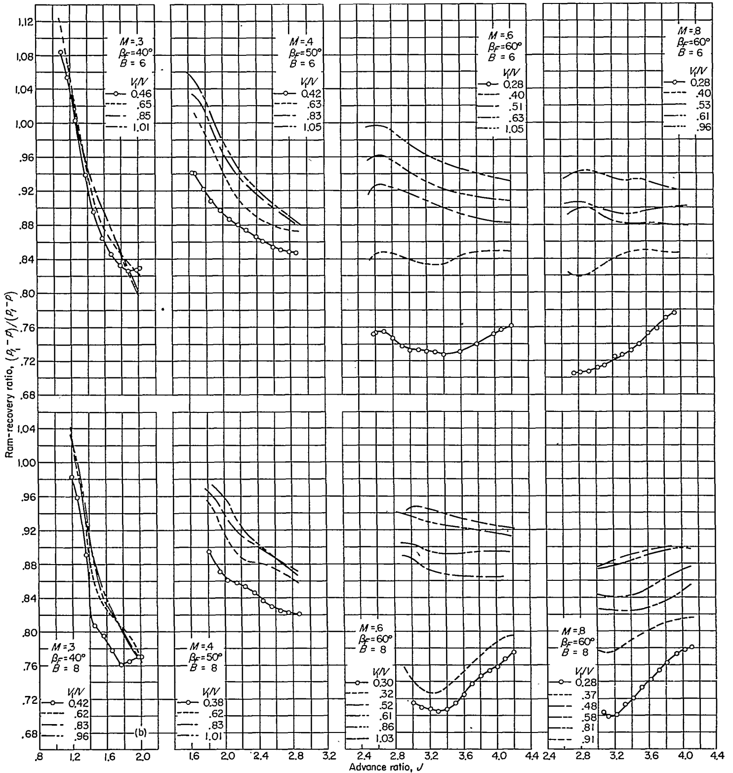
(b) Dual-rotation propeller-spinner-cowling combinations. FIGURE 24.— Concluded.
