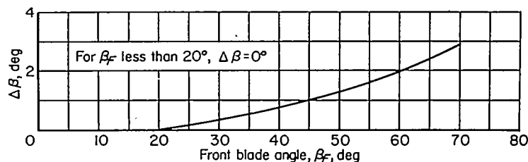
FIGURE 5.—The difference between the front and rear blade angles used for the optimum setting of the dual-rotation propellers.
