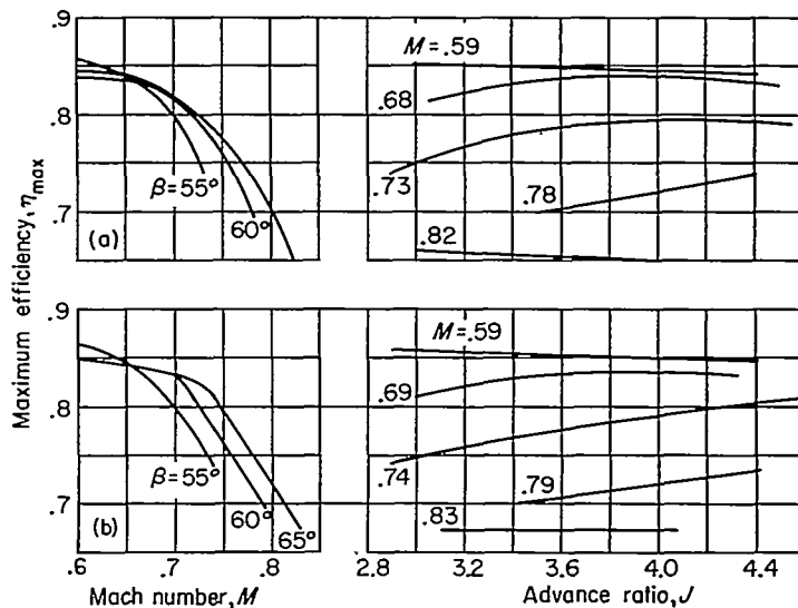
(a) Propeller with 7.2-inch-diameter spinner. (b) Propeller with 12.0-inch-diameter spinner. FIGURE 11. —The effect of Mach number and advance ratio on the maximum efficiency of the NACA 4-(5)(05)-041 four-blade, single-rotation propeller with extended cylindrical spinners.
