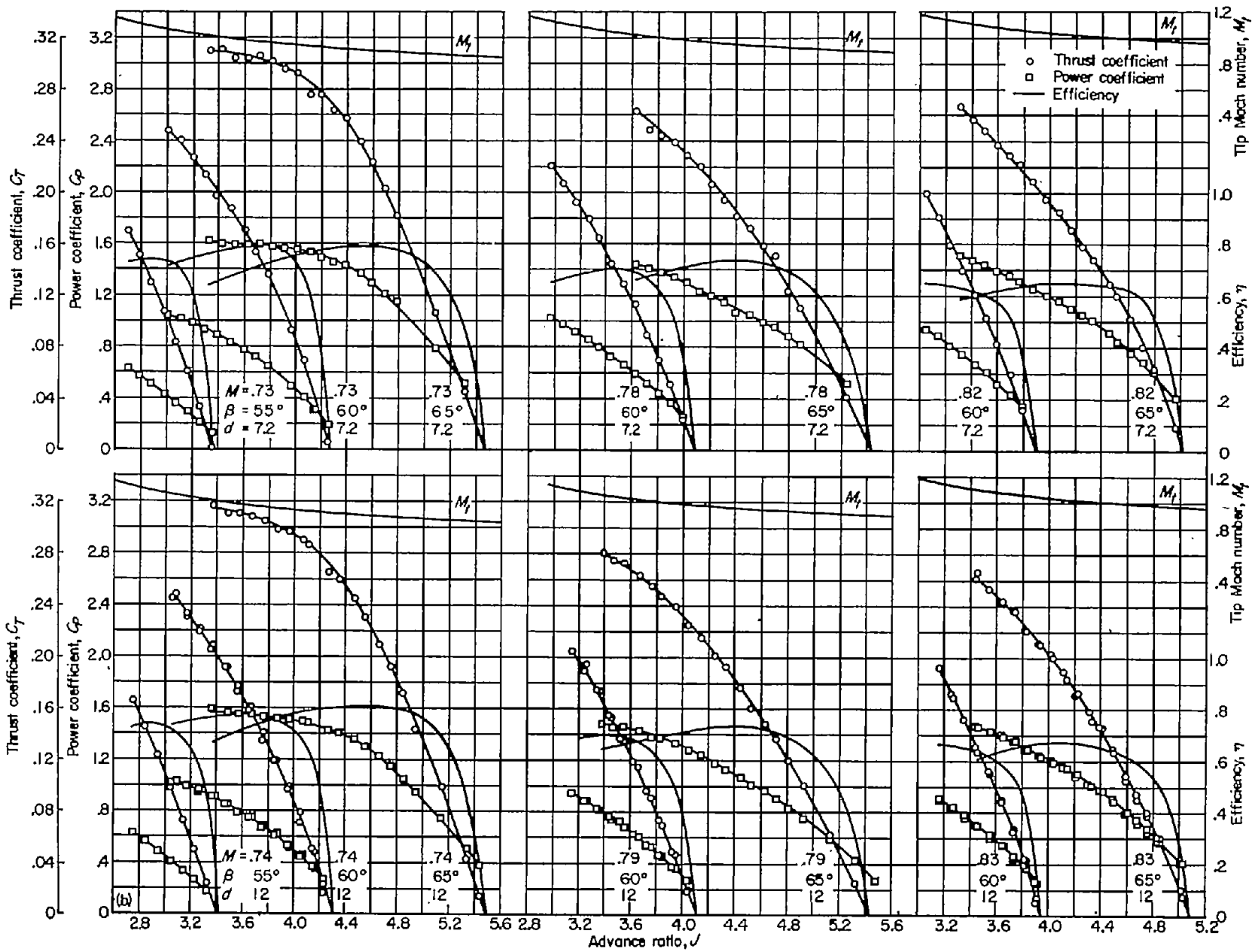
(b) M \approx 0.74, 0.70, and 0.88 FIGURE 8.—Concluded.
