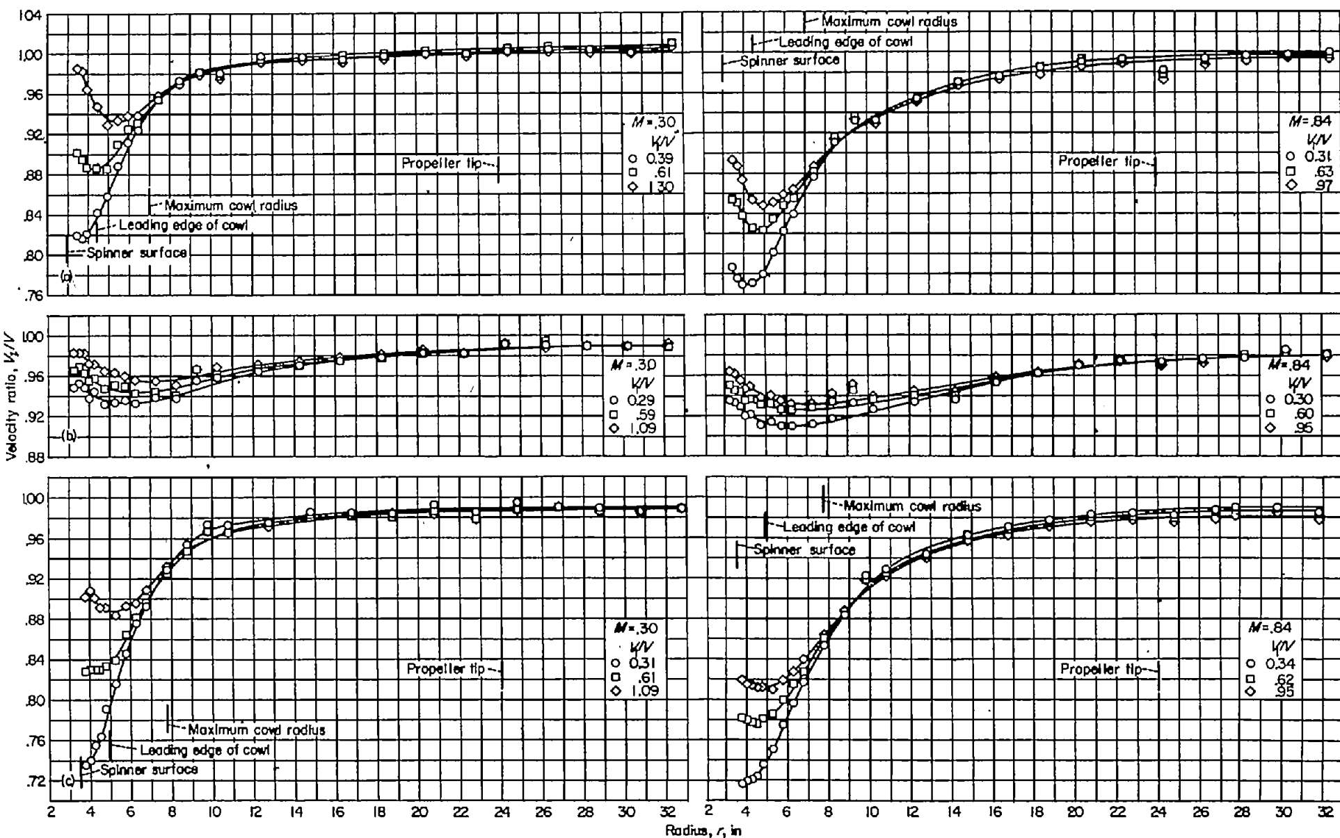
(a) NACA 1-46.5-047 spinner with NACA 1-62.8-070 cowling. (b) NACA 1-46.5-085 spinner with NACA 1-62.8-070 cowling, front plane of rotation. (c) NACA 1-46.5-085 spinner with NACA 1-62.8-070 cowling, rear plane of rotation.
