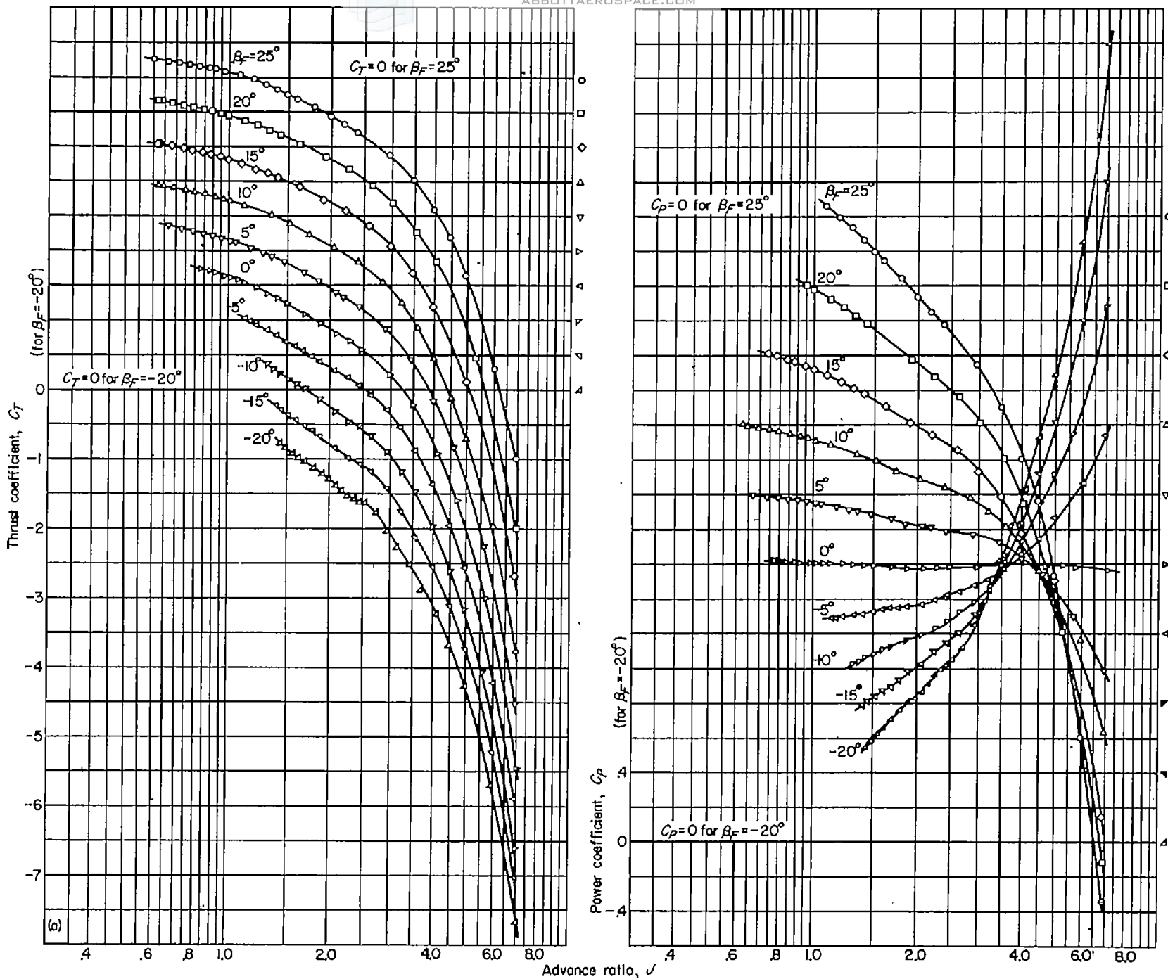
FIGURE 10.—The negative-thrust characteristics of the NACA 4-(5)(05)-037 six-blade, dual-rotation propeller, with NACA 1-series spinner.
