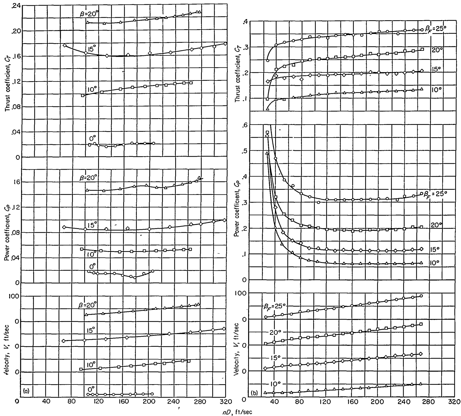
(a) NACA 4-(5)(05)-041 four-blade, single-rotation propeller.
