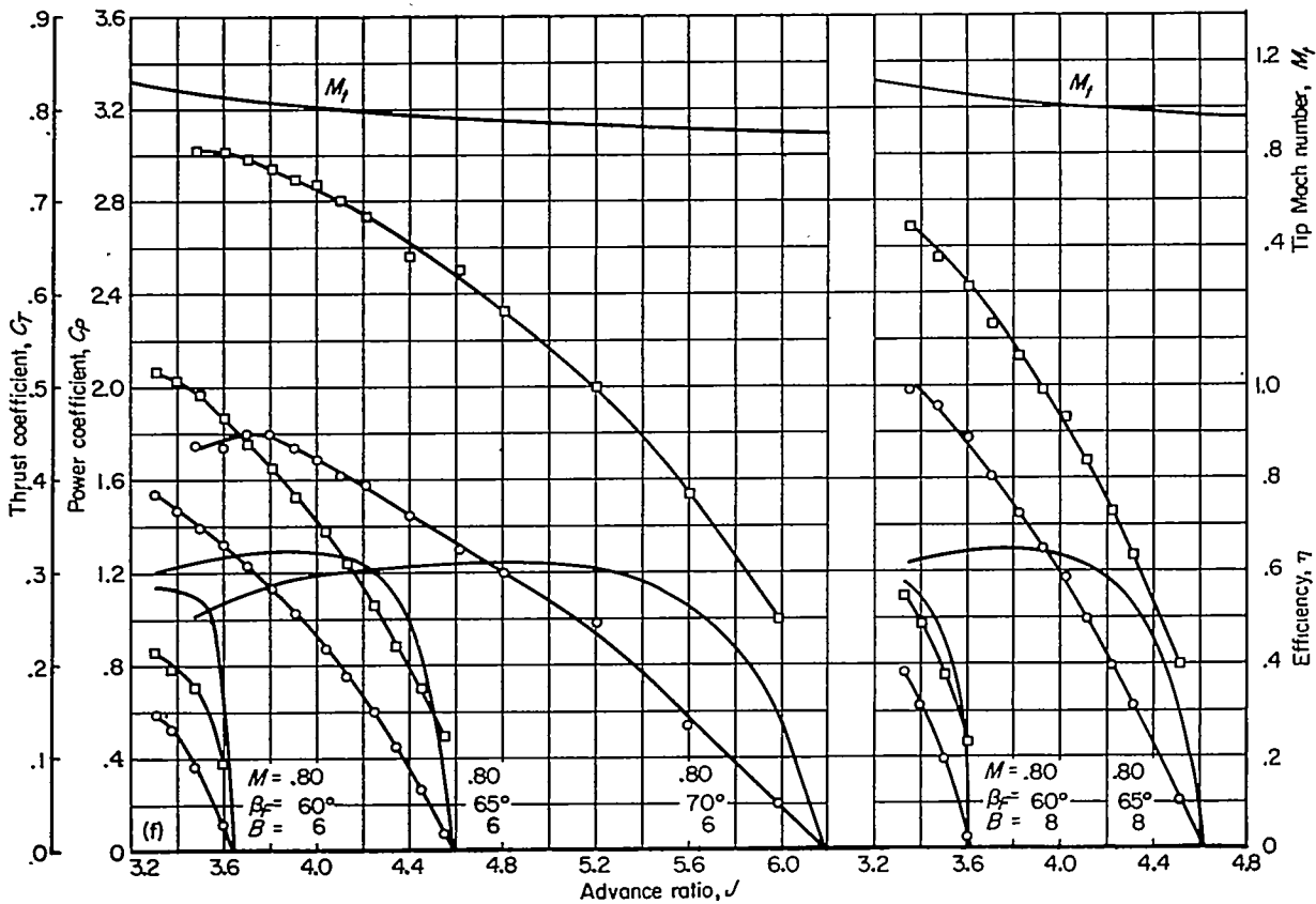
(f) M_t \approx 0.80 FIGURE 7.—Continued.
