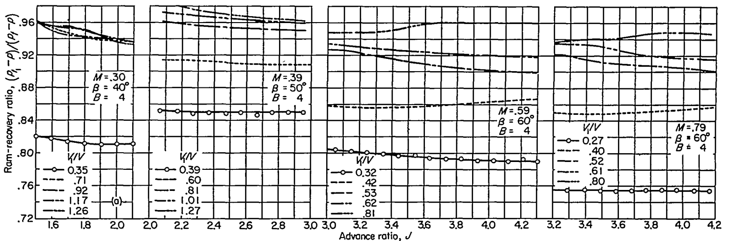
(a) Single-rotation propeller-spinner-cowling combination.
