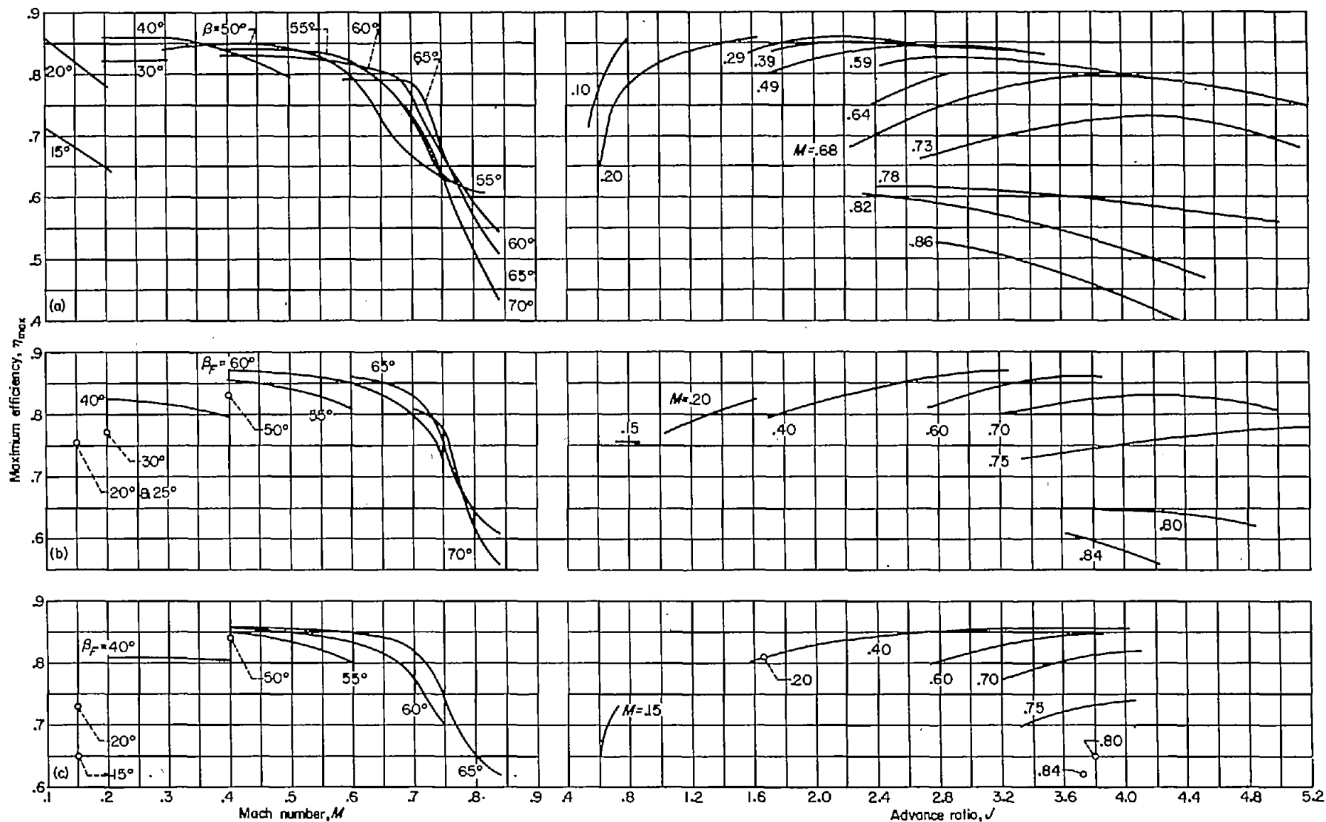
(a) NACA 4-(5)(05)-041 four-blade, single-rotation propeller. (b) NACA 4-(5)(05)-037 six-blade, dual-rotation propeller. (c) NACA 4-(5)(05)-037 eight-blade, dual-rotation propeller.
