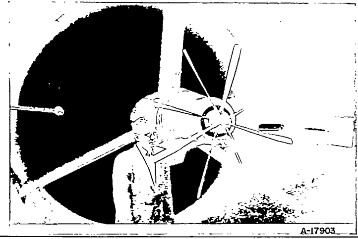
FIGURE 4.—Sketches, coordinates, and photographs of the single- and dual-rotation propeller-spinner-cowling combinations.
