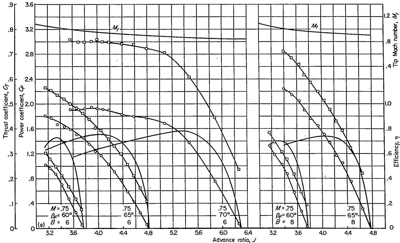
(e) M \approx 0.75 FIGURE 7.—Continued.
