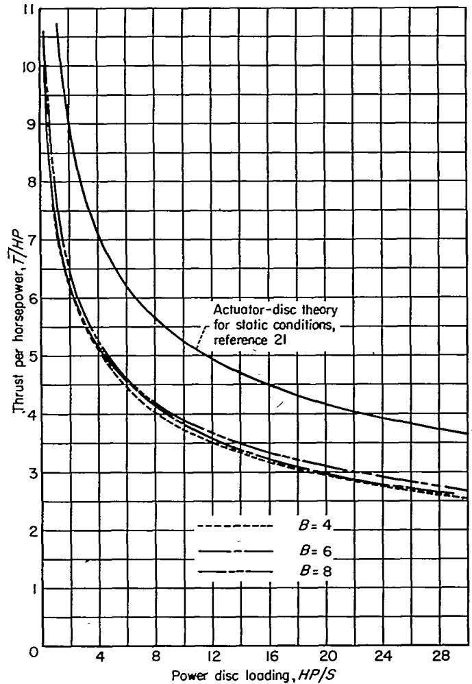
FIGURE 19.—Comparison with actuator-disc theory of the experimentally determined variation of thrust per horsepower with power disc loading for operation of the propellers at near static conditions.
