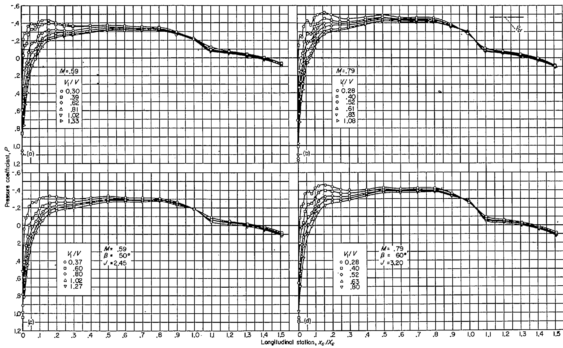
(a) M=0.59 , propeller removed.
