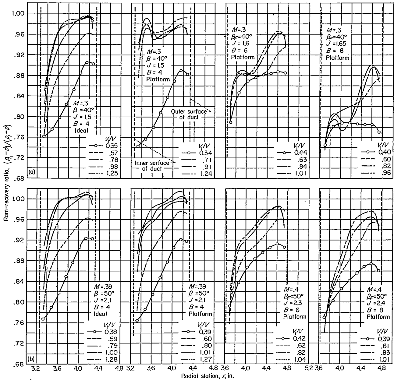
(a) Propeller-spinner-cowling combinations, with ideal and platform junctures, at M=0.30 .
