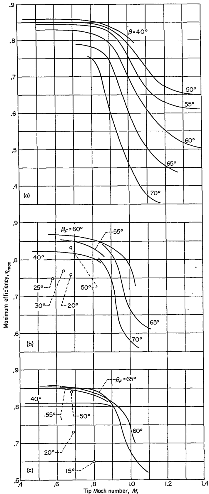
(a) NACA 4-(5)(05)-041 four-blade, single-rotation propeller. (b) NACA 4-(5)(05)-037 six-blade, dual-rotation propeller. (c) NACA 4-(5)(05)-037 eight-blade, dual-rotation propeller. FIGURE 10. —The effect of tip Mach number on the maximum efficiency of the propellers with NACA 1-series spinners.
