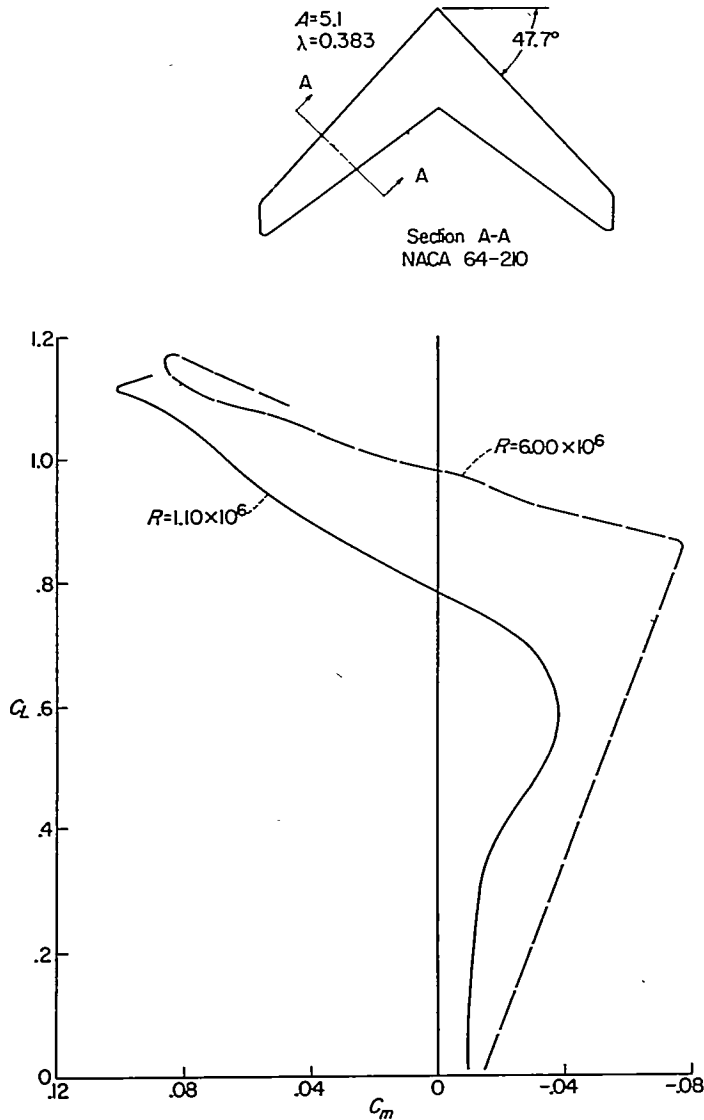
FIGURE 10.—An example of the effect of mixed-flow separation resulting from an increase in Reynolds number from 1.10 \times 10^6 to 6.00 \times 10^6 on the pitching-moment characteristics. (Data obtained from ref. 73.)
