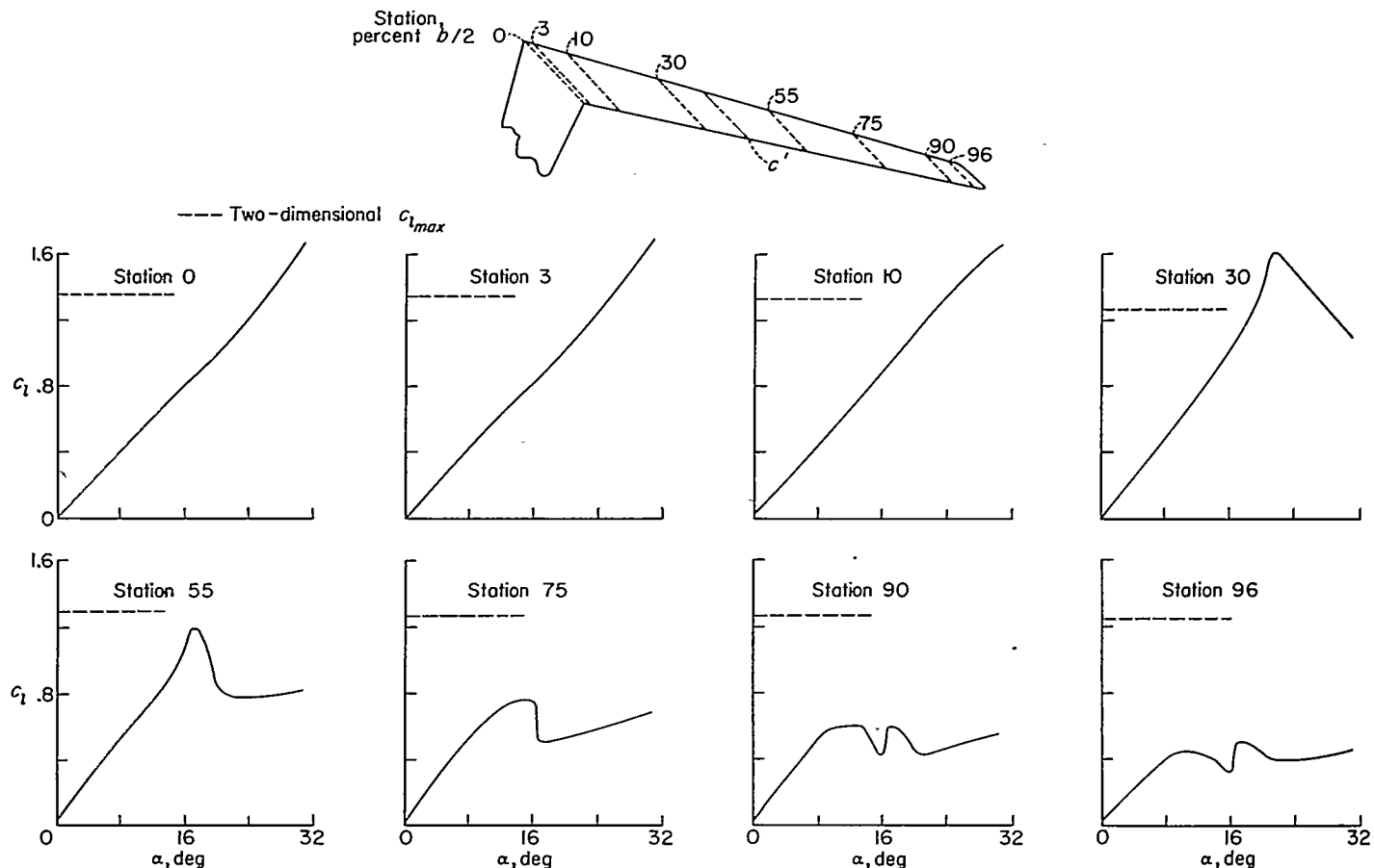
FIGURE 2.—Stall progression on a sweptback wing ( \Lambda_{e/t}=45^\circ ) having an aspect ratio of 8.02, a taper ratio of 0.45, and NACA 63A012 airfoil sections as indicated by the section lift characteristics. (Data obtained from ref. 70.)
