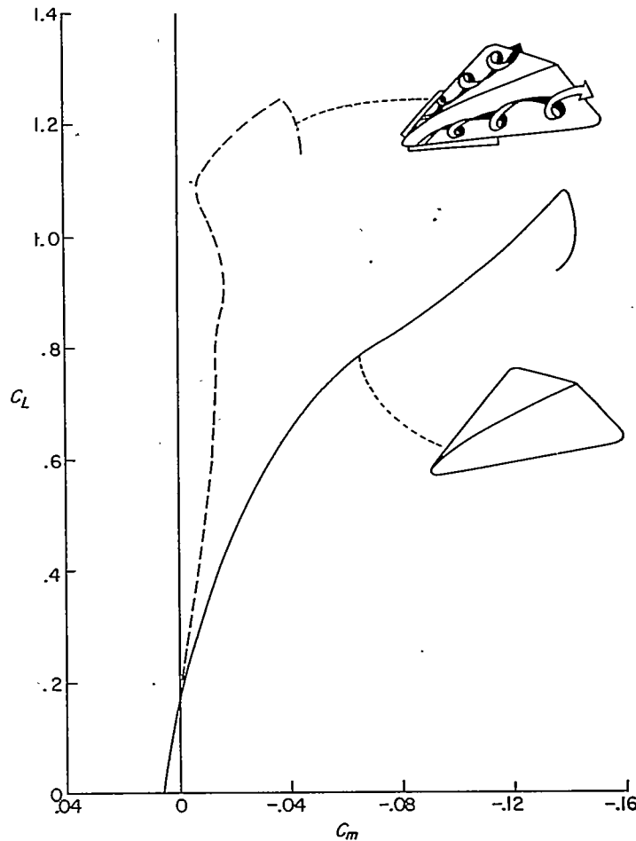
FIGURE 9.—An example of the reduction of the longitudinal stability and out-of-trim pitching moment of a delta wing ( \Delta_{LE}=60^\circ ) by the leading-edge vortex flow resulting from leading-edge separation. (Data obtained from ref. 56.)
