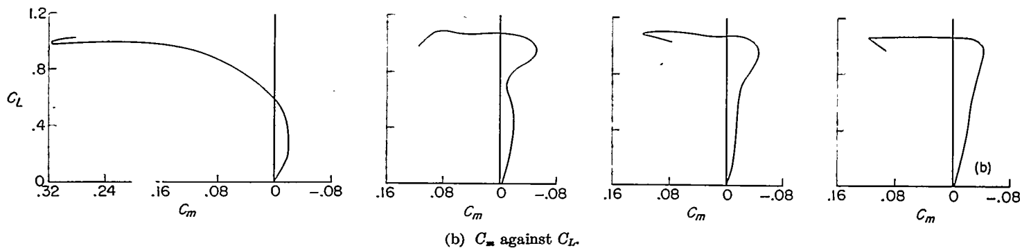
FIGURE 14.—Effect of fences on the section lift and wing pitching-moment characteristics of a sweptback wing ( \Delta_c A = 45^\circ ) having an aspect ratio of 8.02, a taper ratio of 0.45, and NACA 63 1 A012 airfoil section. (Data obtained from ref. 70.)
