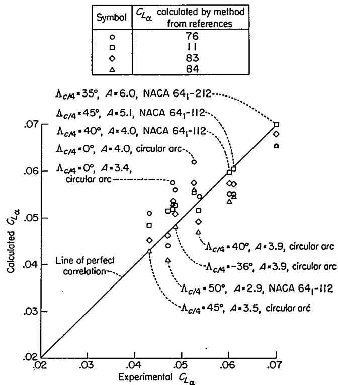
FIGURE 30.—Comparisons of the experimental lift-curve slopes for several wings with those calculated by several methods available for rapidly making such estimates.
