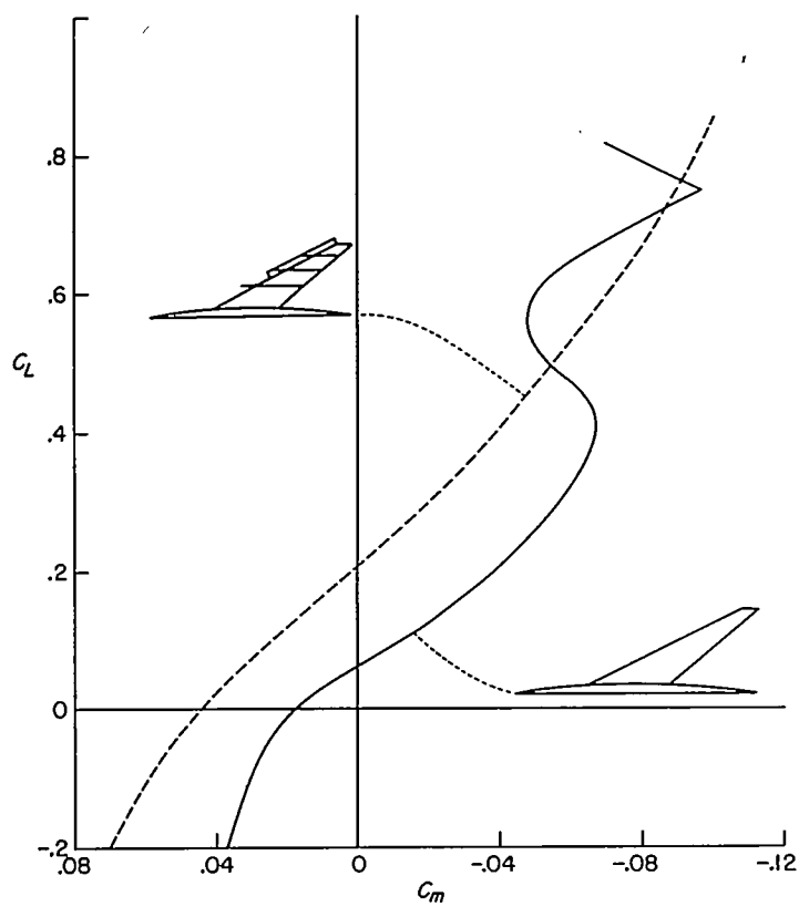
FIGURE 25.—The effect of extensible leading-edge flaps and fences on the pitching-moment characteristics of a twisted and cambered sweptback wing ( \Lambda_{c/4}=60.8^\circ ) having an aspect ratio of 3.5, and a taper ratio of 0.25. (Data obtained from reference 80.)
