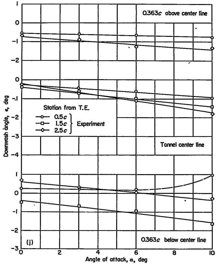
(j) Spanwise station, 1.571 \frac{b}{2}
