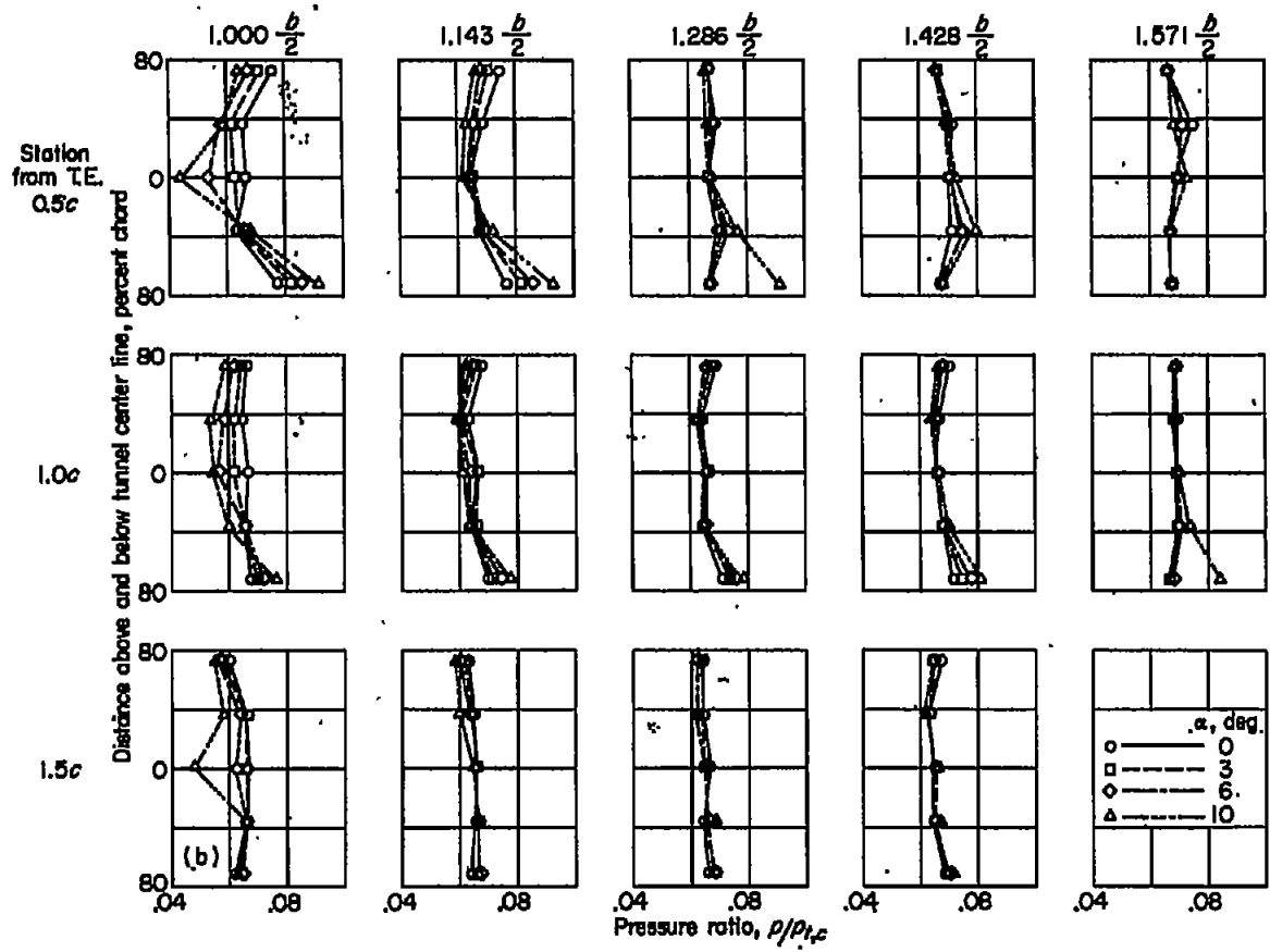
(b) Survey stations 0.5, 1.0, and 1.5 chords behind wing trailing edges. Outboard of tip. FIGURE 8.—Continued.
