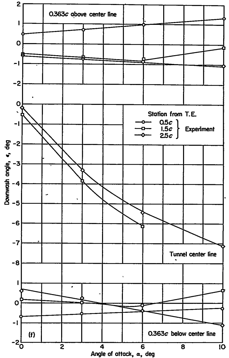
(f) Spanwise station, 1.000\frac{b}{2}
