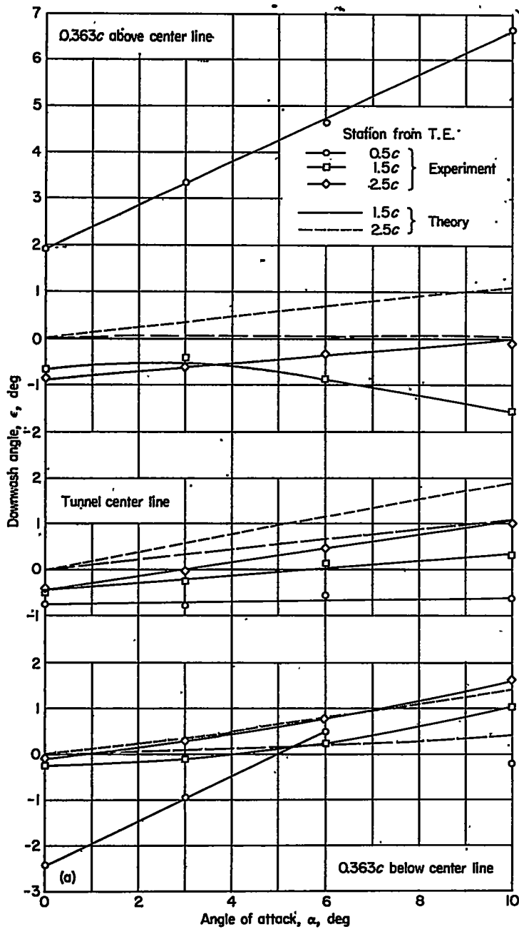
(a) Spanwise station, 0.280\frac{b}{2} (Slight curvature of theoretical curves is due to trailing-edge displacement relative to fixed test-point locations.)
