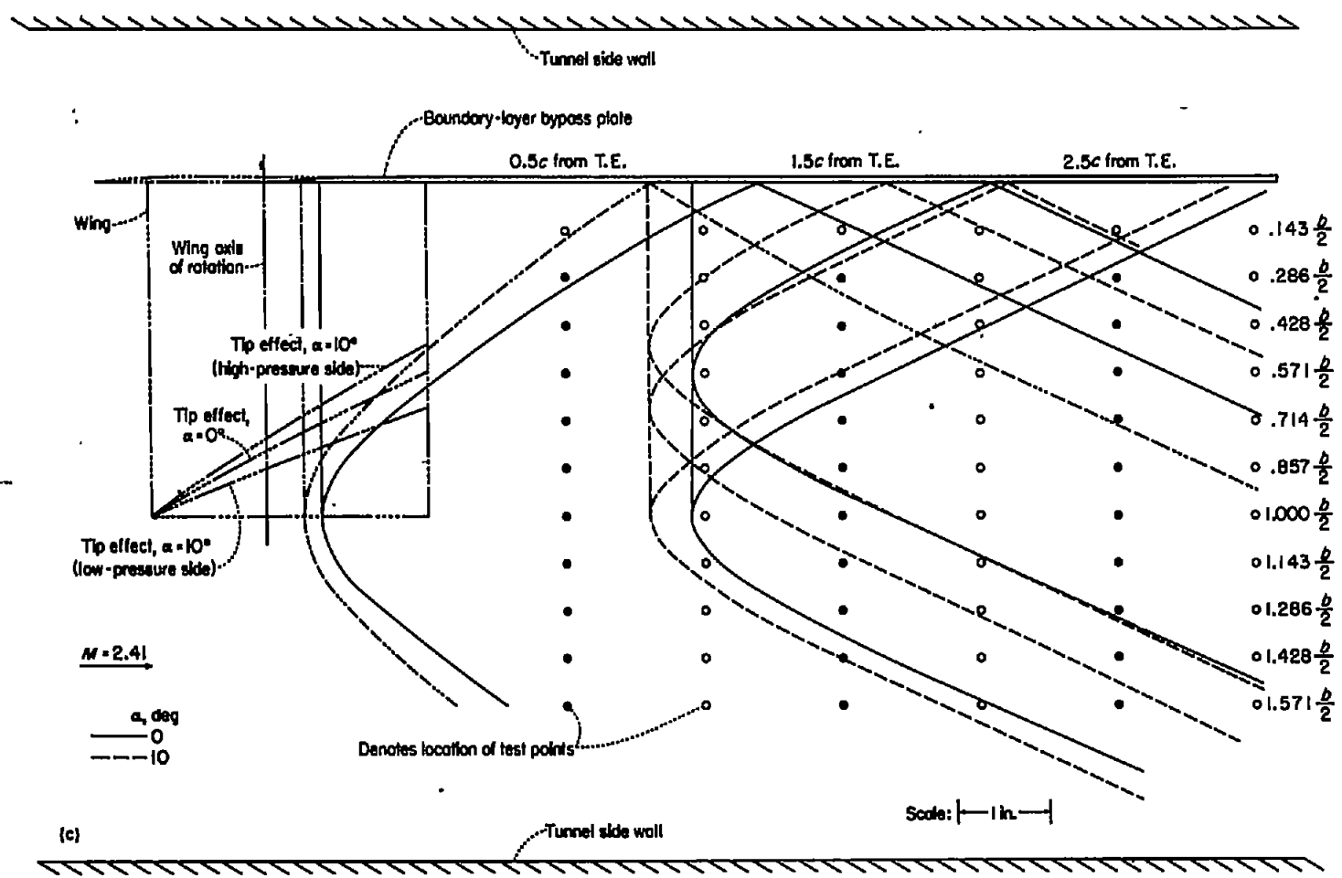
(c) Horizontal plane 0.363 chord below tunnel center line. FIGURE 7.—Concluded.
