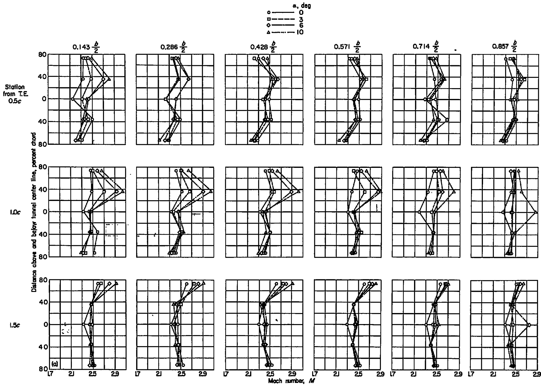
(a) Survey stations 0.5, 1.0, and 1.5 chords behind wing trailing edge. Inboard of tip. FIGURE 9.—Mach number distribution behind rectangular wing. Undisturbed stream Mach number, 2.41.
