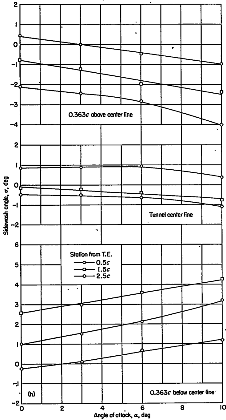
(h) Spanwise station, 1.286 \frac{b}{2}
