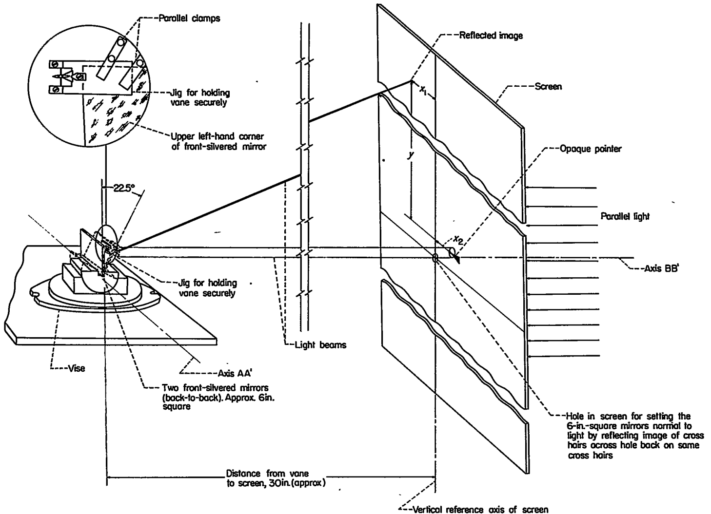
FIGURE 25.—Sketch of setup used for measuring the angles between vane axis and normals to each mirror-polished surface of vane.
