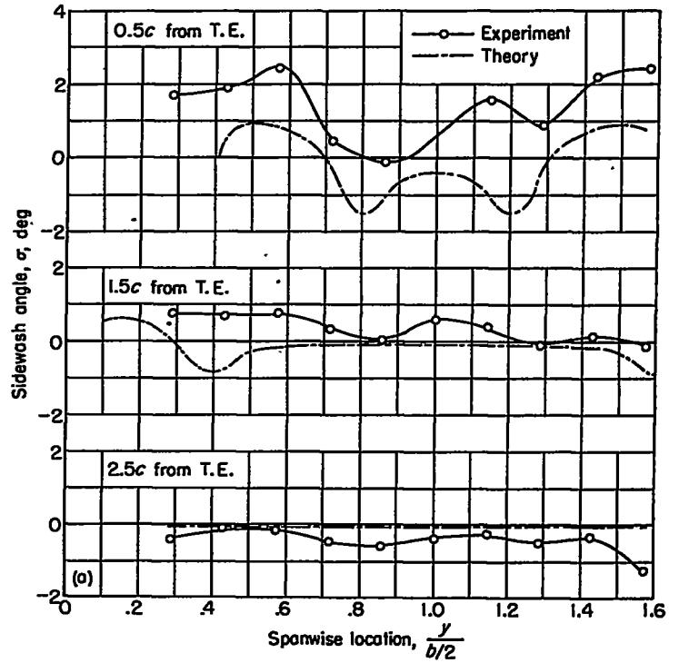
(a) On tunnel center line.
