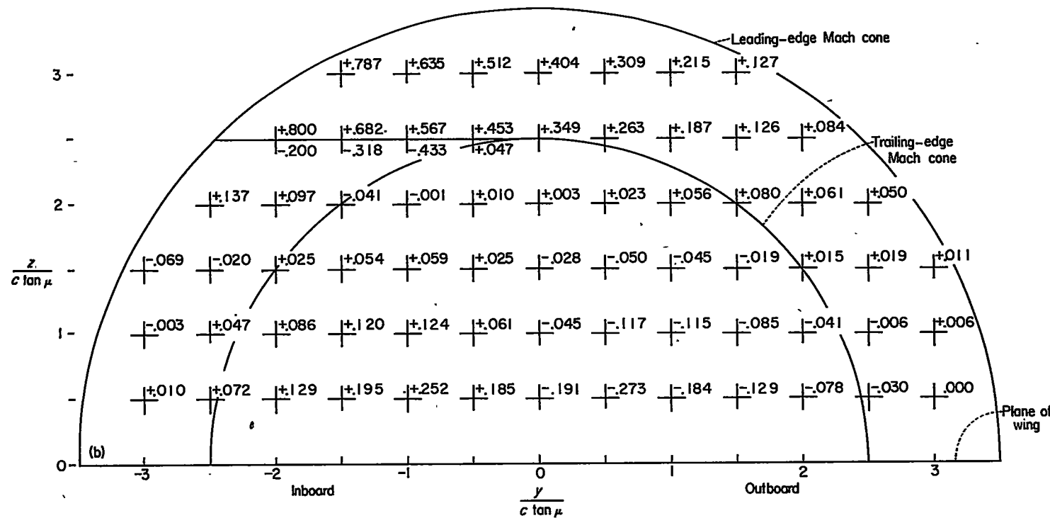
(a) Sidewash, d\sigma/d\alpha . (Signs reversed below plane of wing.) (b) Downwash, d\epsilon/d\alpha . (Signs same below plane of wing.)
