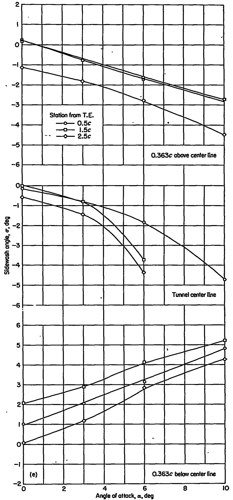
(e) Spanwise station, 0.857 \frac{b}{2}
