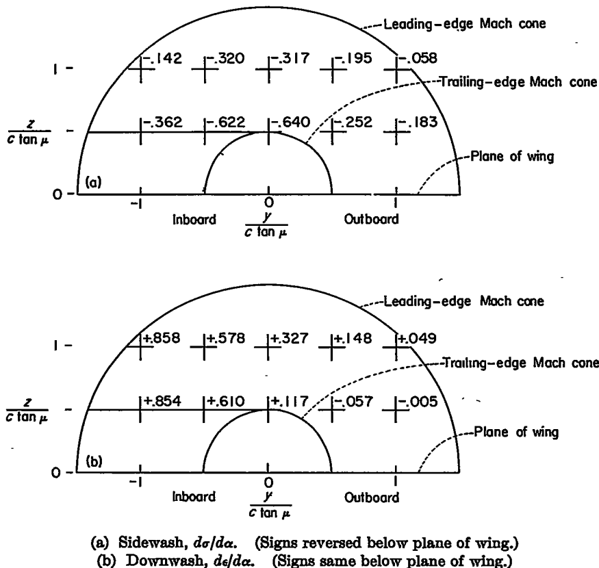
FIGURE 14.—Theoretical values of ds/d\alpha and de/d\alpha in a vertical plane 0.5 chord behind the trailing edge of a semi-infinite rectangular wing of zero thickness
