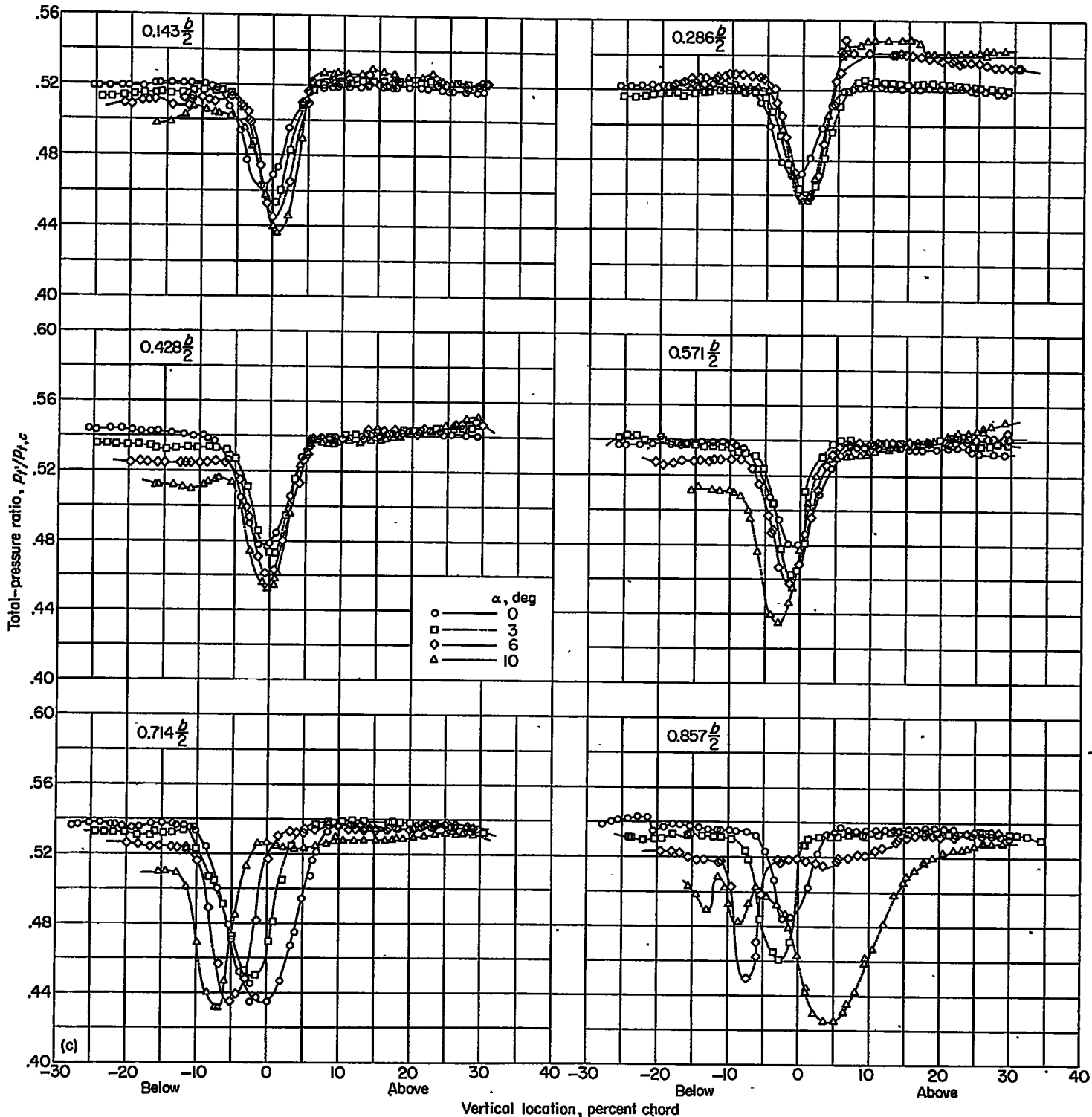
(c) Station 1.5 chords behind wing trailing edge. Spanwise stations 0.143 \frac{b}{2} through 0.857 \frac{b}{2}
