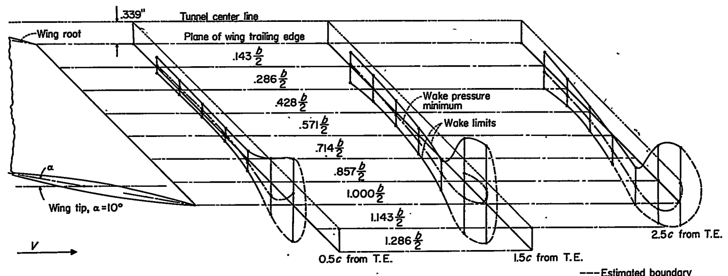
(c) \alpha = 6^\circ .
