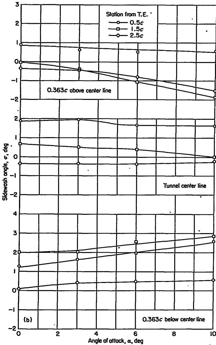
(b) Spanwise station, 0.428 \frac{b}{2}
