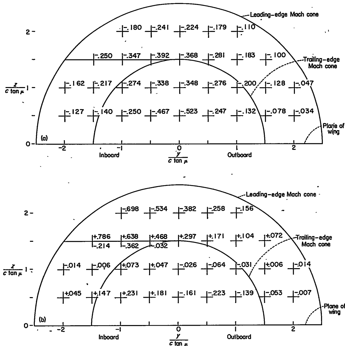
(a) Sidewash, d\sigma/d\alpha . (Signs reversed below plane of wing.) (b) Downwash, d\epsilon/d\alpha . (Signs same below plane of wing.)
