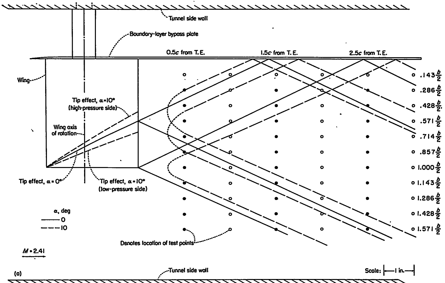
(a) Horizontal plane of tunnel center line.
