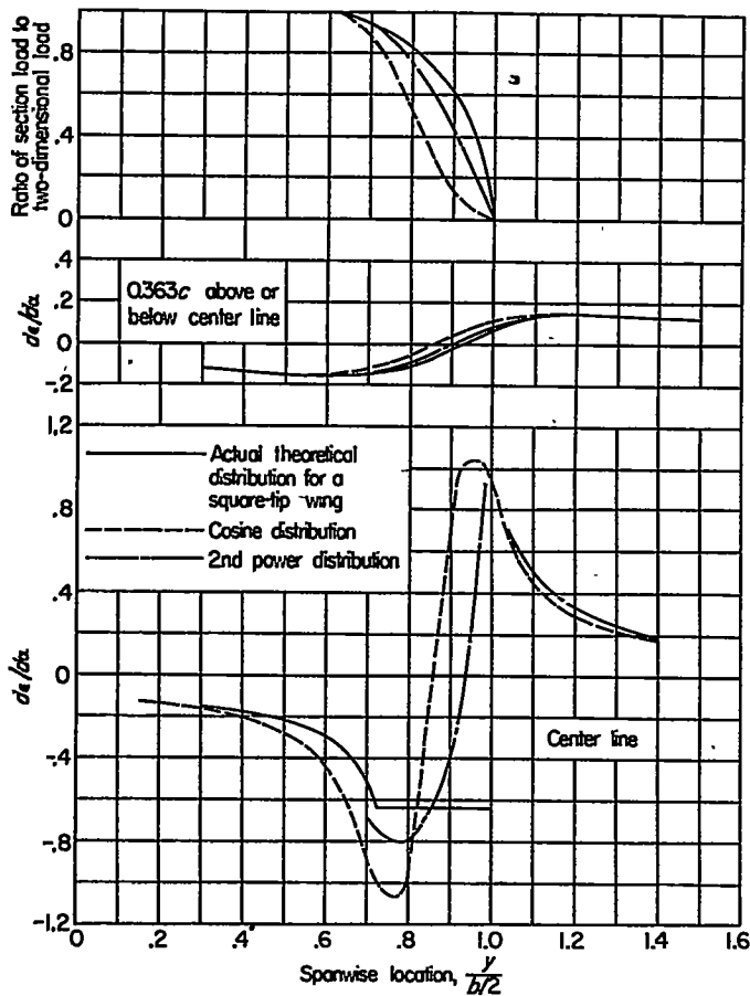
FIGURE 20.—Theoretical curves of ds/d\alpha against span in the Trefftz plane behind a rectangular wing, showing effect of spanwise load distribution on downwash values.
