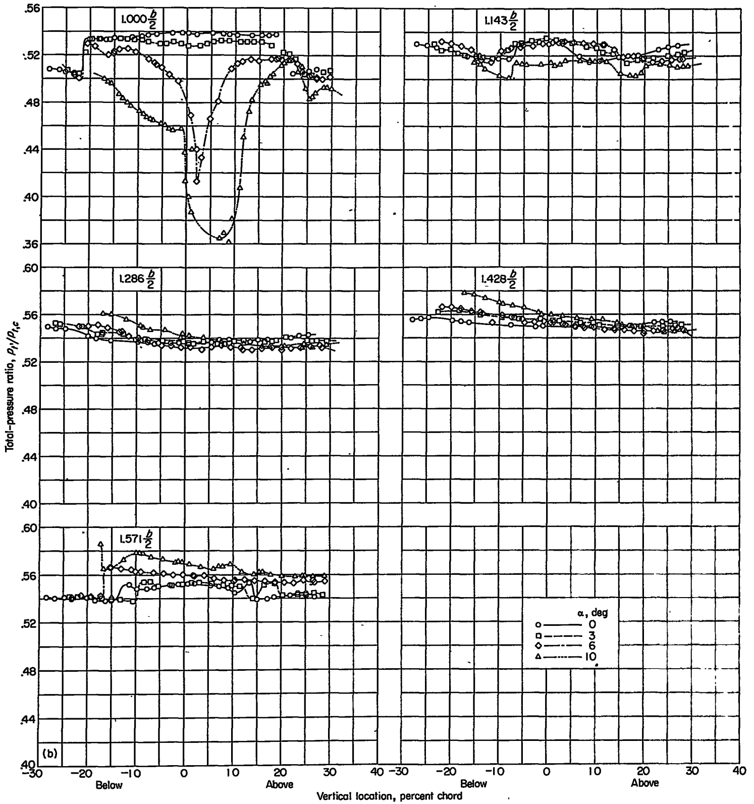
(b) Station 0.5 chord behind wing trailing edge. Spanwise stations 1.000 \frac{b}{2} through 1.571 \frac{b}{2} .
