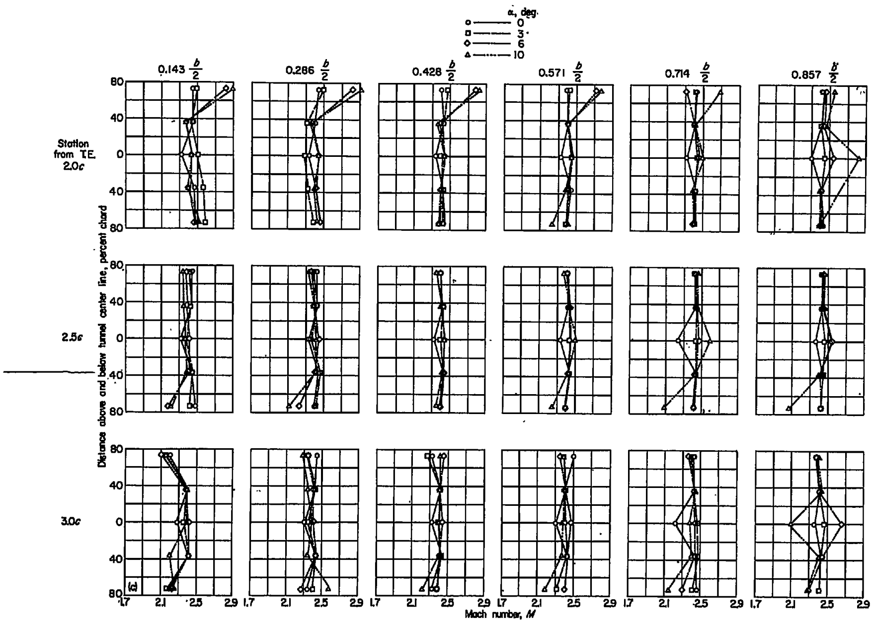
(c) Survey stations 2.0, 2.5, and 3.0 chords behind wing trailing edge. Inboard of tip.
