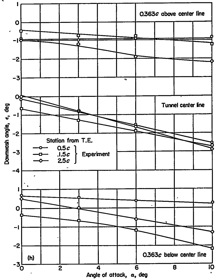
(h) Spanwise station, 1.286 \frac{b}{2}
