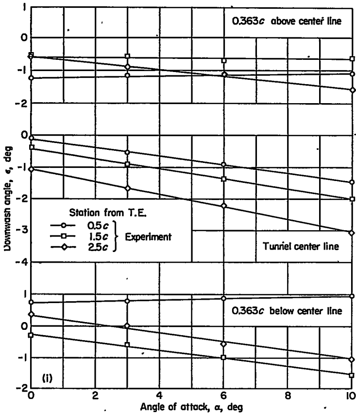
(i) Spanwise station, 1.428 \frac{b}{2}
