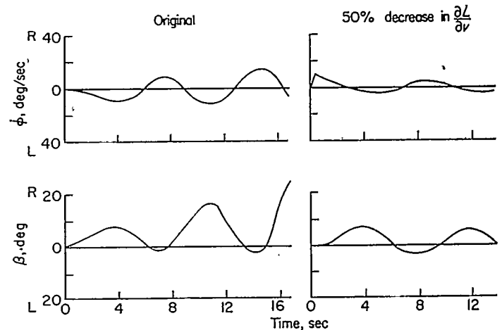
FIGURE 7.—Measured effect of reduction in effective dihedral on lateral oscillation.
