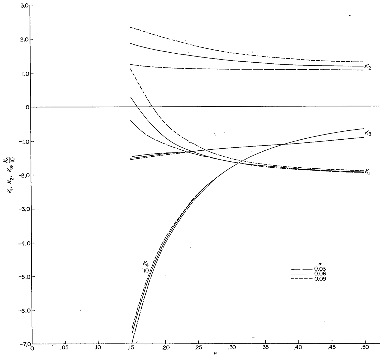
FIGURE 5.—Equation for speed stability of tandem-rotor helicopters.
