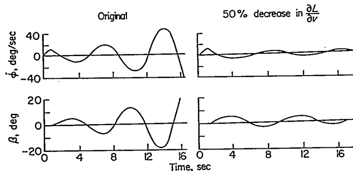
FIGURE 6.—Predicted effect of reduction in effective dihedral on lateral oscillation.
