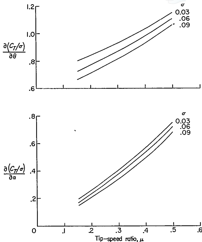
FIGURE 1.—Variation of C_T/\sigma derivatives with respect to \mu .
