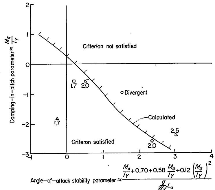
FIGURE 4.—Maneuver-stability chart for 2-second criterion.
