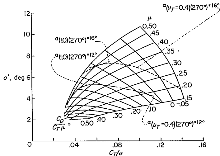
FIGURE 3.—Sample chart for determining derivatives of a' and C_Q/\sigma . \theta = 8^\circ .
