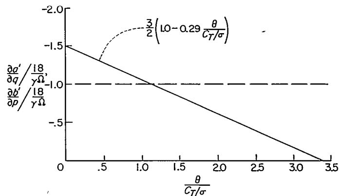
FIGURE 2.—Chart for determining rotor damping in pitch and roll.
