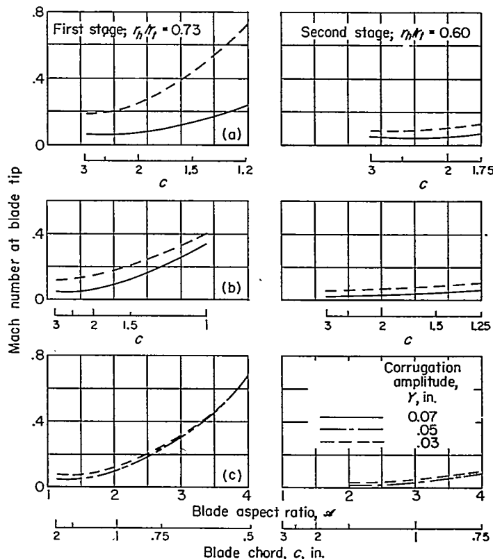
(a) Turbine diameter, 35 inches. (b) Turbine diameter, 25 inches. (c) Turbine diameter, 15 inches.
