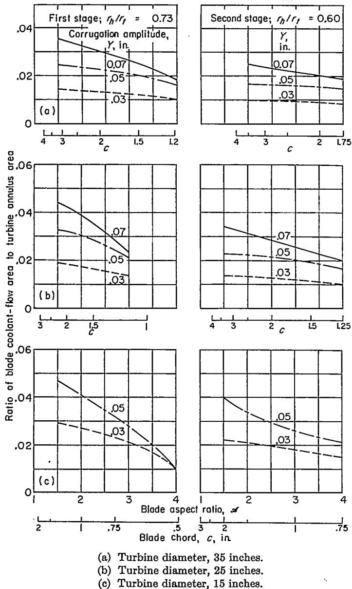
FIGURE 6.—Effect of turbine blade size on coolant-passage flow area.
