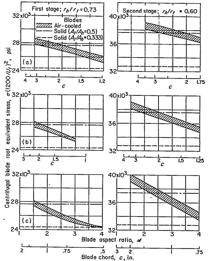
(a) Turbine diameter, 35 inches. (b) Turbine diameter, 25 inches. (c) Turbine diameter, 15 inches.
