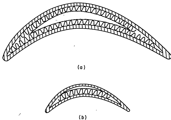
(a) Typical corrugated-insert blade. (b) Effect of placing chord on air-cooled blade inside heat-transfer surface area.
