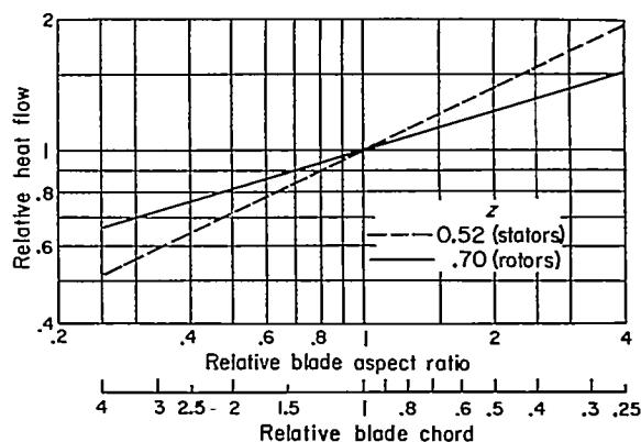
FIGURE 7.—Effect of turbine blade size on heat flow to blade.
