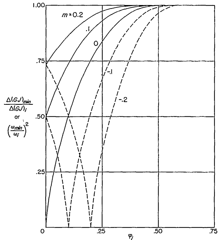
FIGURE 6.—Calculated ratio of minimum incremental stiffness to initial incremental stiffness as a function of initial twist for several values of applied moment.
