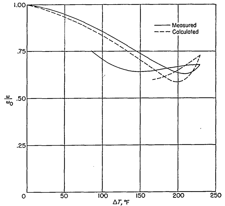
FIGURE 12.—Comparison of measured and calculated values of the frequency ratio as a function of temperature difference.
