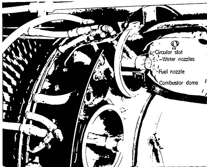
FIGURE 15.—Combustion-chamber water spray nozzle (J47 engine).
