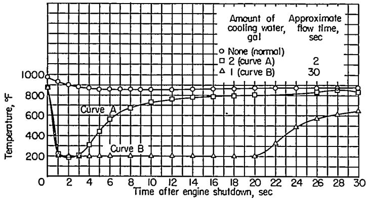
FIGURE 18.—Comparison of turbine-wheel cooling with short- and long-duration water sprays.
