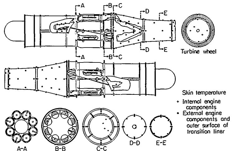
FIGURE 6.—Thermocouple locations on J47 engine.
