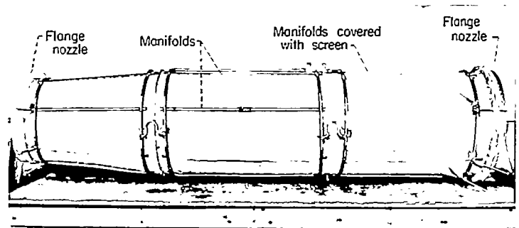
FIGURE 19.—Typical water distribution system for F-84 tailpipe.
