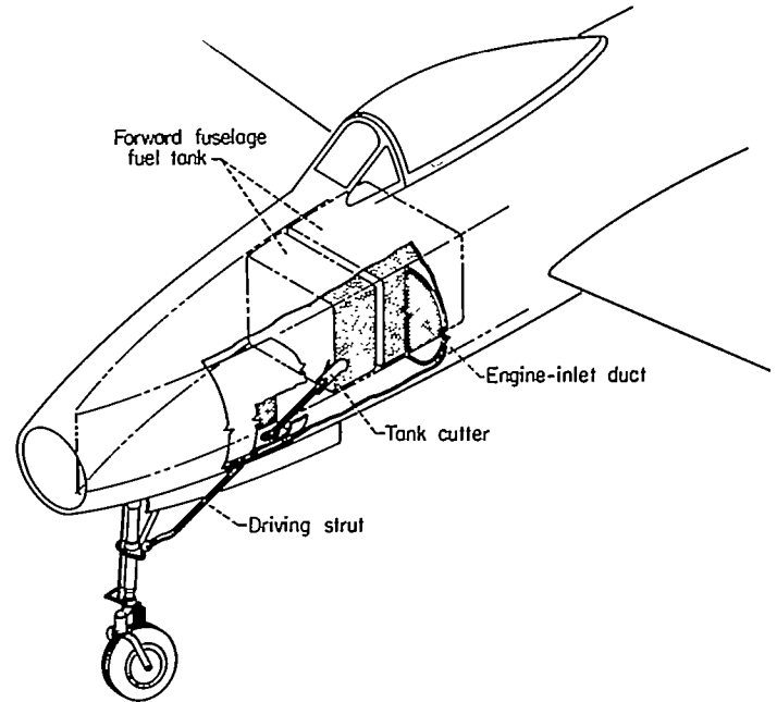
FIGURE 4.—Schematic diagram of F-84 tank-cutting mechanism.
