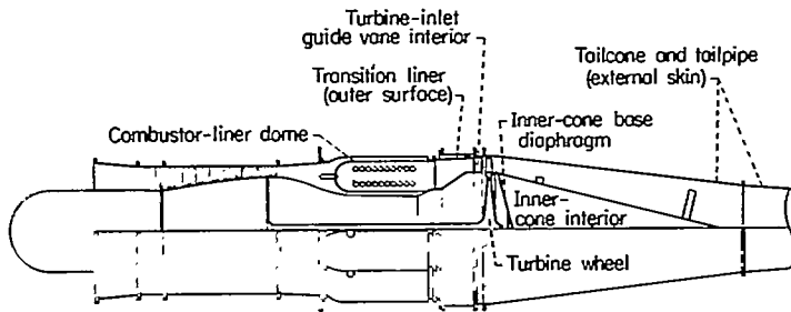
FIGURE 11.—Hot-metal ignition sources found in J35 engine.
