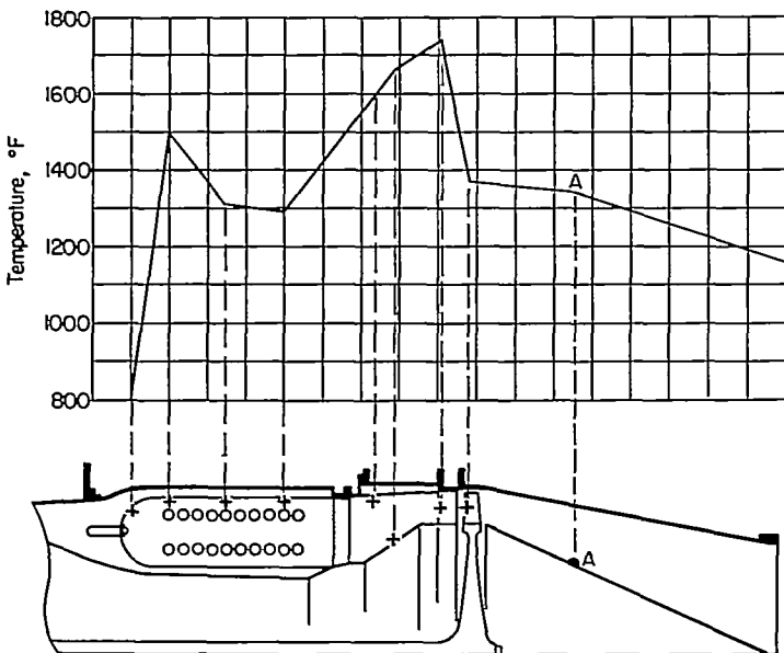
FIGURE 7.—Maximum temperatures of metal components in main gas stream of J47 and J35 engines.
