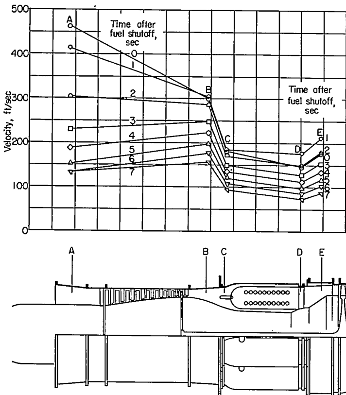
FIGURE 9.—Air velocity through J35 engine after combustor fuel shutoff.
