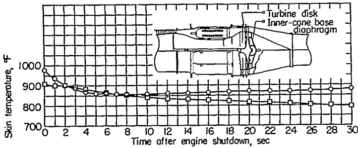
FIGURE 30.—History of maximum skin temperatures on turbine disk and inner-cone base diaphragm.
