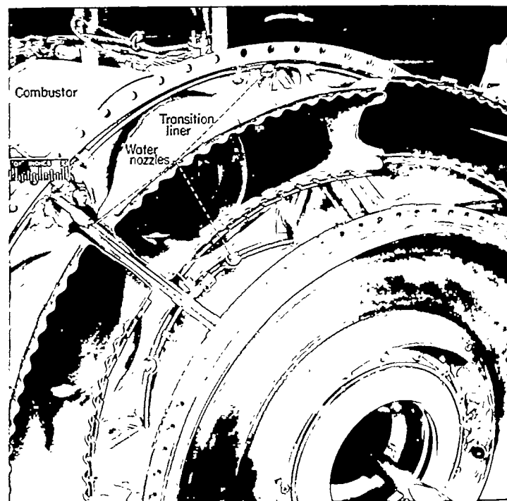
FIGURE 16.—Transition-liner water spray system (J35 and J47 engines).
