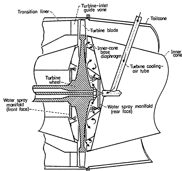
FIGURE 17.—Schematic diagram of turbine-cooling system.
