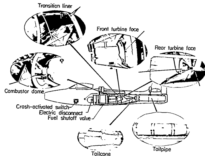
FIGURE 20.—Complete inerting system installed in F-84 airplane.
