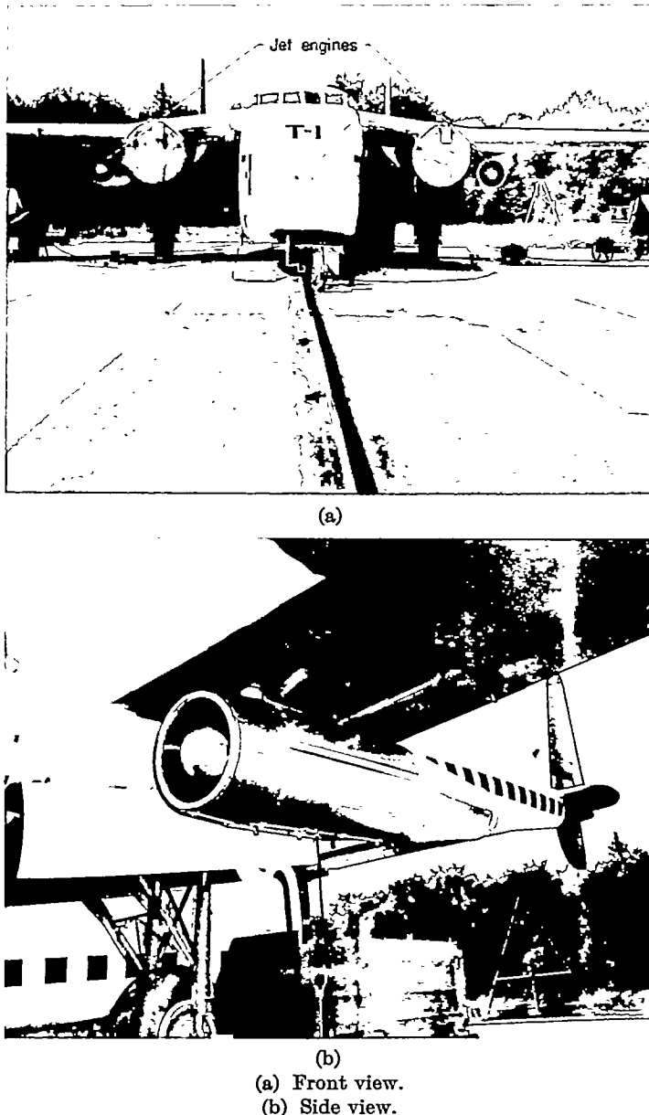
FIGURE 1.—Jet engines pylon-mounted to wing of cargo airplane.
