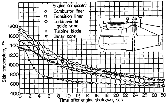
FIGURE 29.—History of maximum skin temperatures on engine components in main gas streams.
