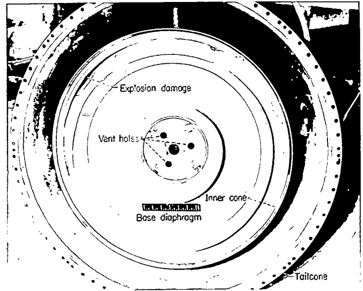
FIGURE 12.—J35 Inner-cone base diaphragm.
