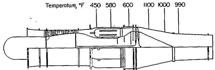
FIGURE 32.—Maximum external skin temperatures on J47 engine.
