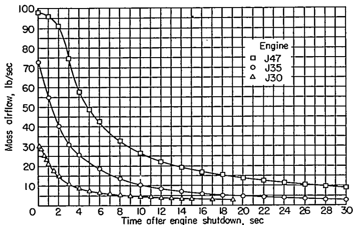
FIGURE 33.—Mass airflow after combustor fuel has been stopped.
