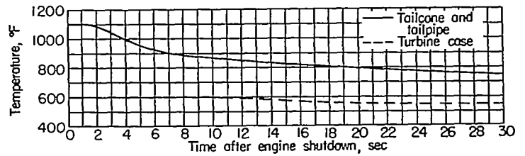
FIGURE 31.—History of maximum external skin temperatures on J47 turbine case and tailcone and tailpipe.
