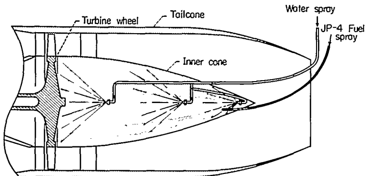
FIGURE 34.—Typical equipment used to study ignition hazard (J30 inner tailcone).
