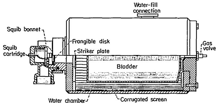
FIGURE 23.—Bladder-type water reservoir.
