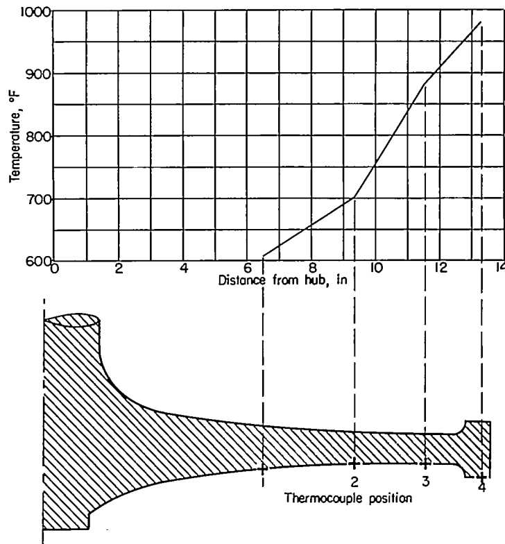
FIGURE 28.—Maximum temperatures recorded on J47-engine turbine wheel.
