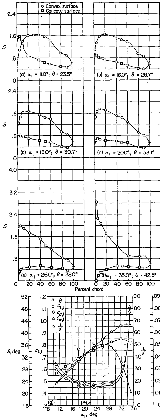
(g) Section characteristics; flagged symbol indicates leading-edge roughness.
