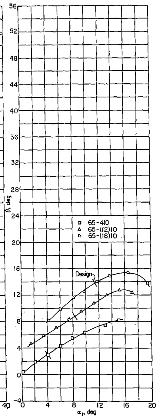
FIGURE 99.—Summary of relationship between turning angle \theta and angle of attack \alpha_1 for the blade sections tested at \beta_1=80^\circ , \sigma=0.50 .
