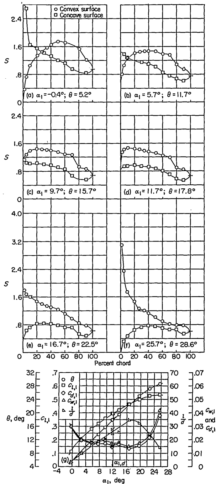
FIGURE 41.—Blade-surface pressure distributions and blade section characteristics for the cascade combination, \beta_1 = 45^\circ , \sigma = 1.50 , and blade section, NACA 65-810.
