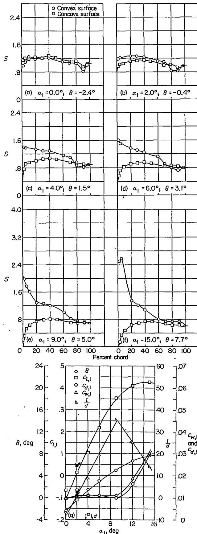
FIGURE 71.—Blade-surface pressure distributions and blade section characteristics for the cascade combination, \beta_1=70^\circ , \sigma=1.00 , and blade section, NACA 65-010.
