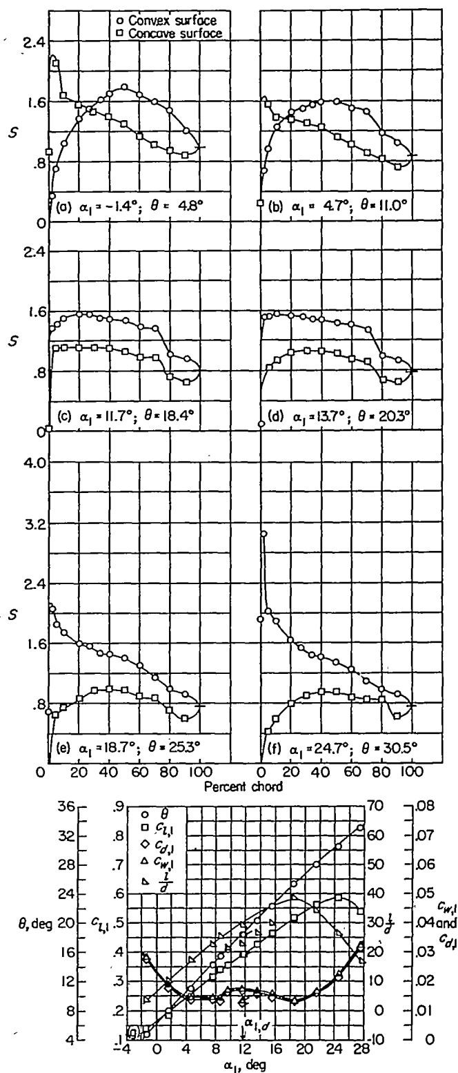
FIGURE 17.—Blade-surface pressure distributions and blade section characteristics for the cascade combination, \beta_1 = 30^\circ , \sigma = 1.50 , and blade section, NACA 65-810.
