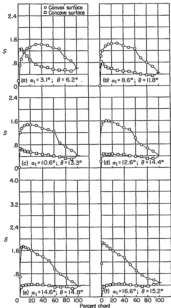
(g) Section characteristics; flagged symbol indicates leading-edge roughness.
