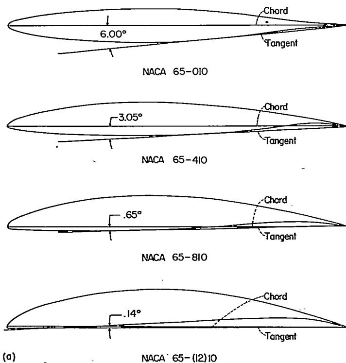
FIGURE 4.—Blade sections tested in this investigation.
