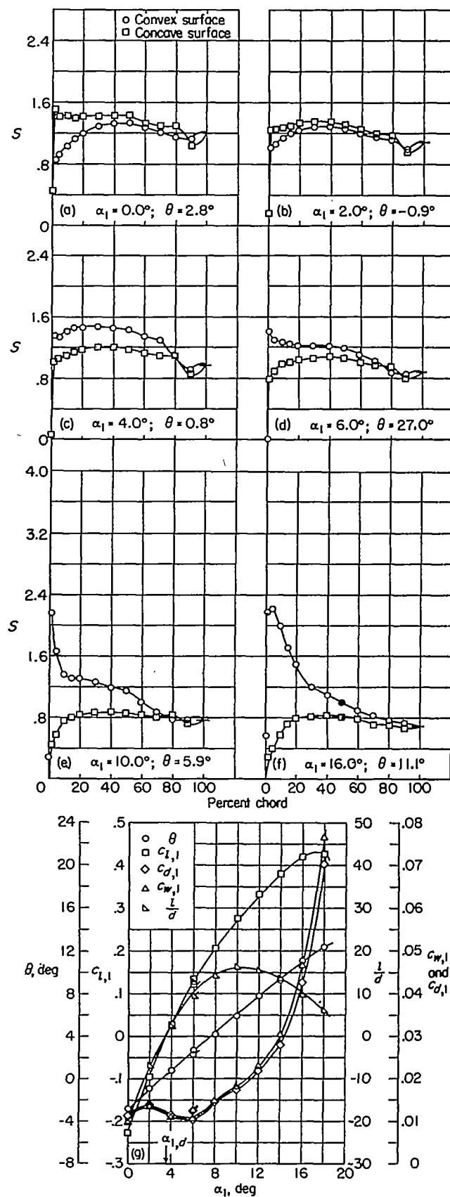
(g) Section characteristics; flagged symbol indicates leading-edge roughness.
