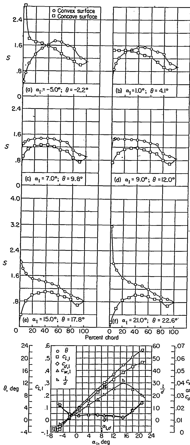
FIGURE 16.—Blade-surface pressure distributions and blade section characteristics for the cascade combination, \beta_1 = 30^\circ , \sigma = 1.50 , and blade section, NACA 65-410.
