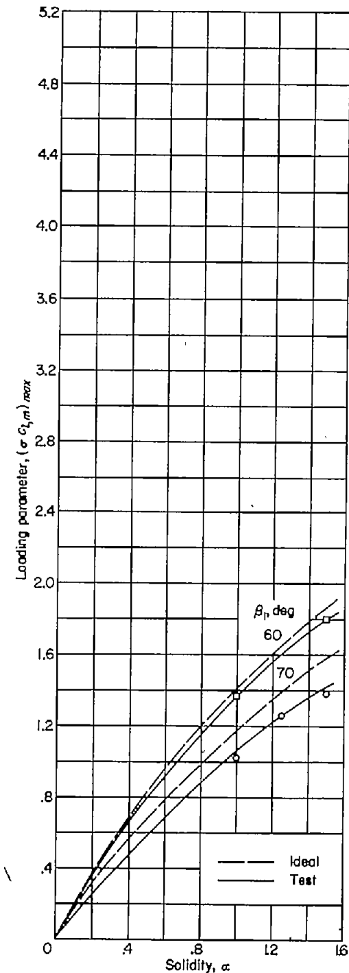
FIGURE 89.—Variation of the limit loading parameter, (\sigma c_{l,m})_{max} with solidity for inlet angles of 60° and 70°.
