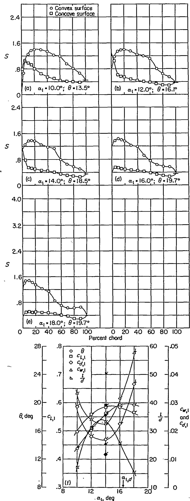
FIGURE 79.—Blade-surface pressure distributions and blade section characteristics for the cascade combination, \beta_1=70^\circ , \sigma=1.25 , and blade section, NACA 65-(15)10.
