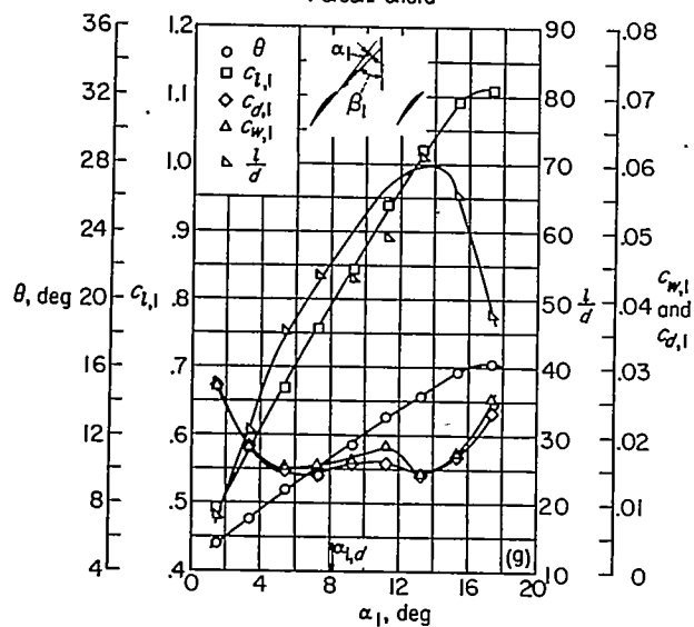
(g) Section characteristics.
