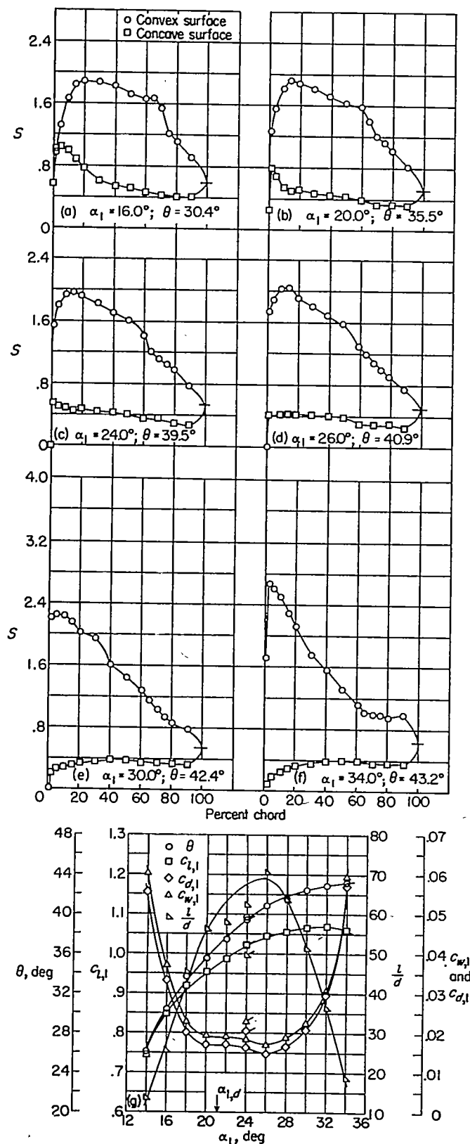
(g) Section characteristics; flagged symbol indicates leading-edge roughness. FIGURE 34.—Blade-surface pressure distributions and blade section characteristics for the cascade combination, \beta_1=45^\circ , \sigma=1.00 , and blade section, NACA 65-(24)10.
