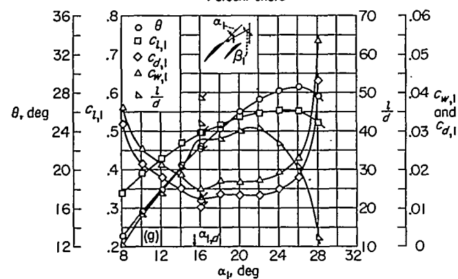
FIGURE 66.—Blade-surface pressure distributions and blade section characteristics for the cascade combination, \beta_1 = 60^\circ , \sigma = 1.50 , and blade section, NACA 65-(12)10.
