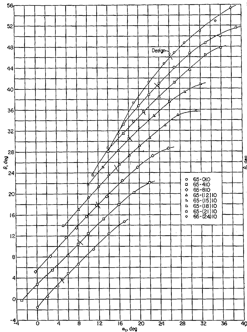
FIGURE 98.—Summary of relationship between turning angle \theta and angle of attack \alpha_1 for the blade sections tested at \beta_1=46^\circ , \sigma=1.50 .
