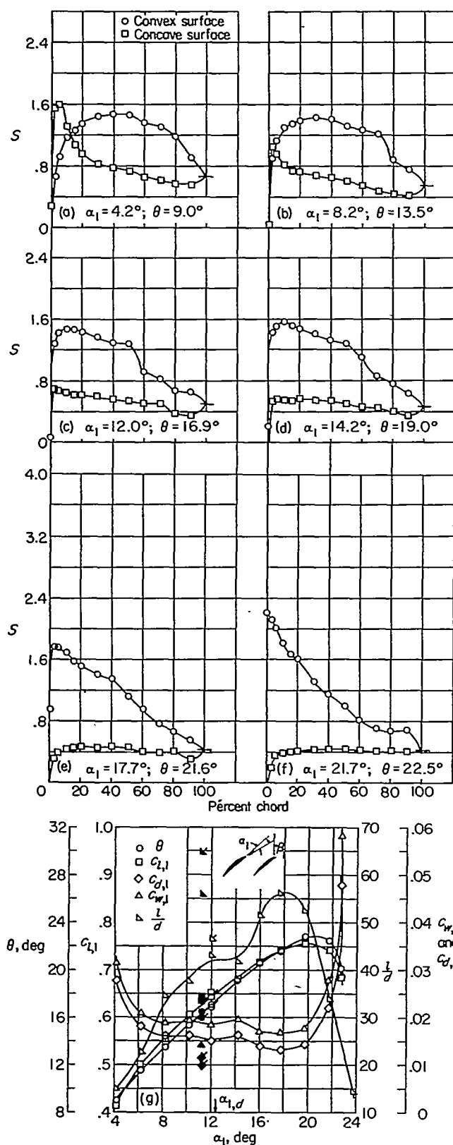
(g) Section characteristics; flagged symbol indicates leading-edge roughness; solid symbol indicates high Reynolds number.
