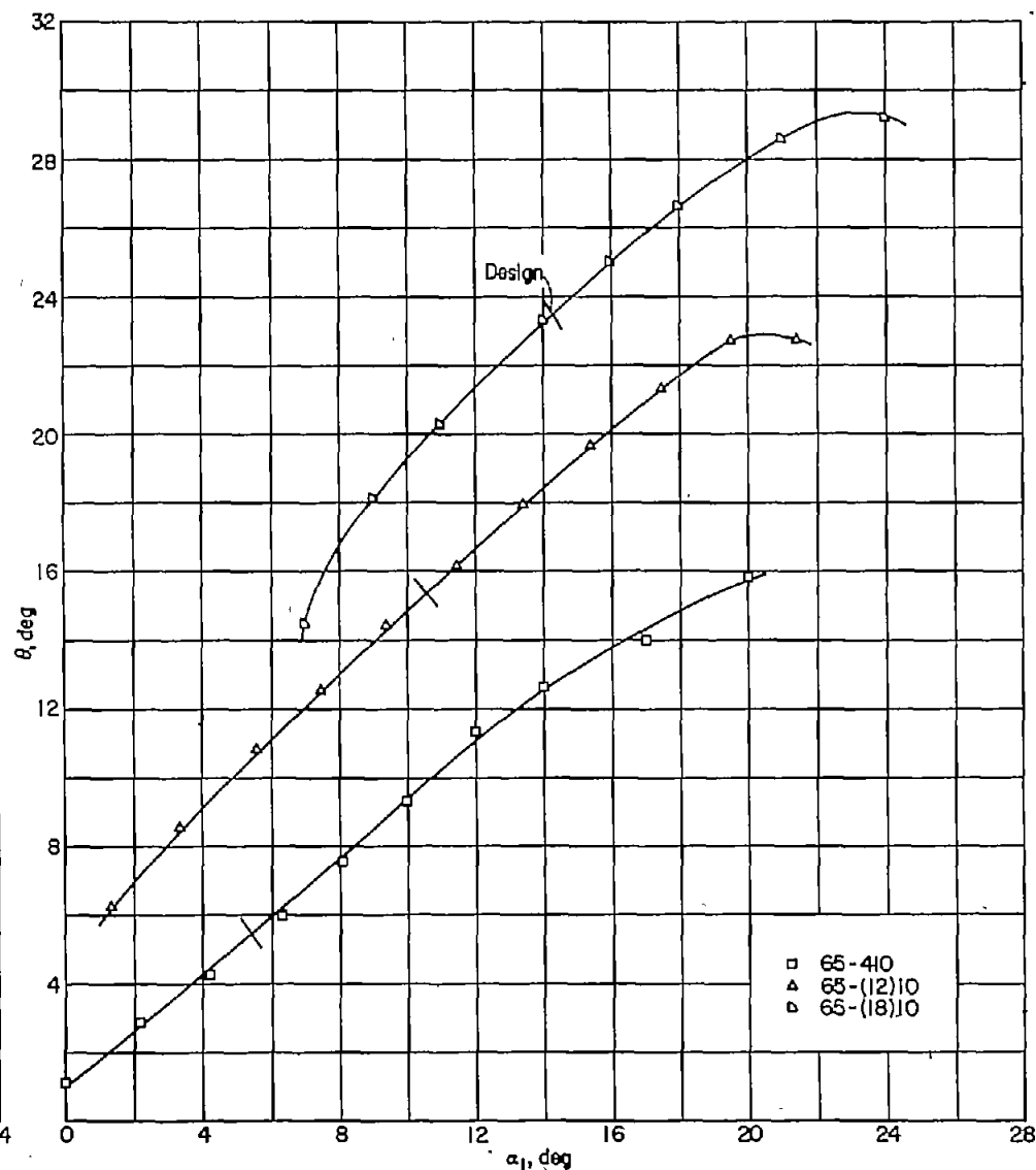
FIGURE 95.—Summary of relationship between turning angle \theta and angle of attack \alpha_1 for the blade sections tested at \beta_1=45^\circ , \sigma=0.75 .
