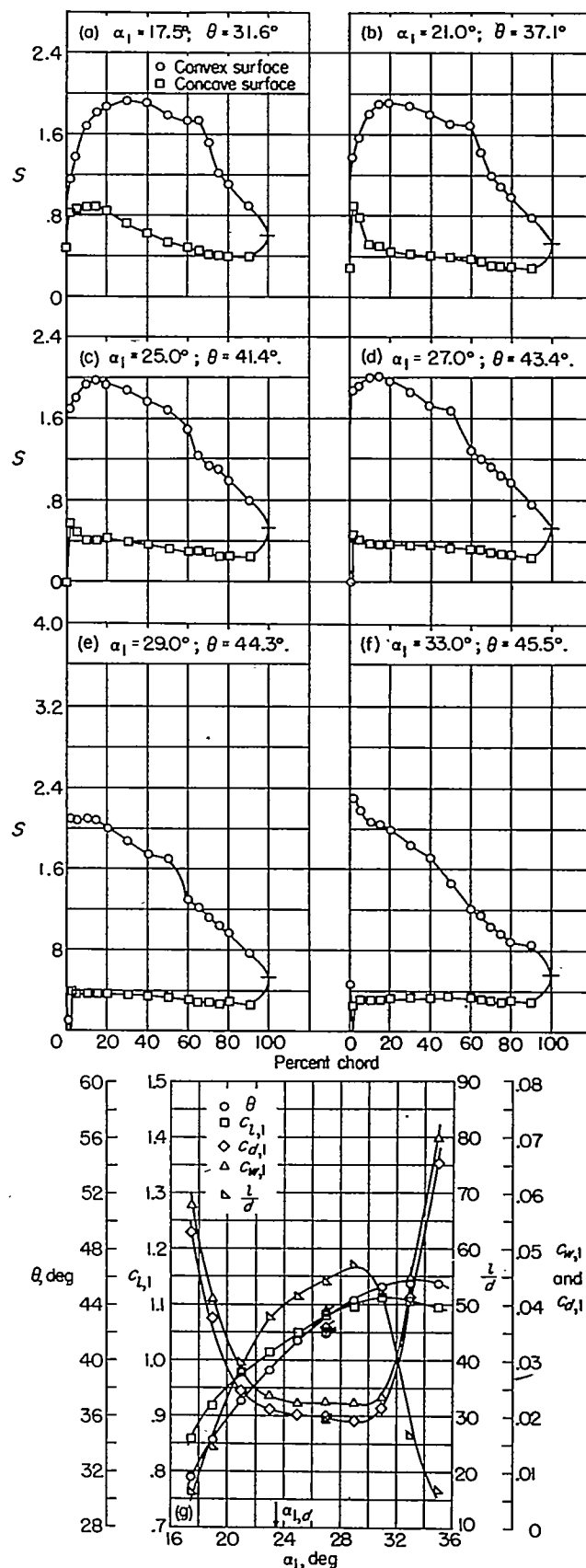
(g) Section characteristics; flagged symbol indicates leading-edge roughness. FIGURE 35.—Blade-surface pressure distributions and blade section characteristics for the cascade combination, \beta_1=45^\circ , \sigma=1.00 , and blade section, NACA 65-(27)10.
