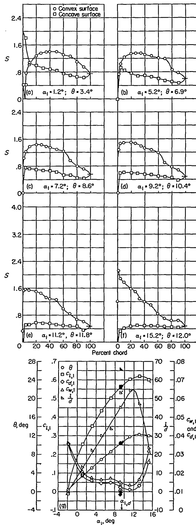
(g) Section characteristics; flagged symbol indicates leading-edge roughness; solid symbol indicates high Reynolds number.
