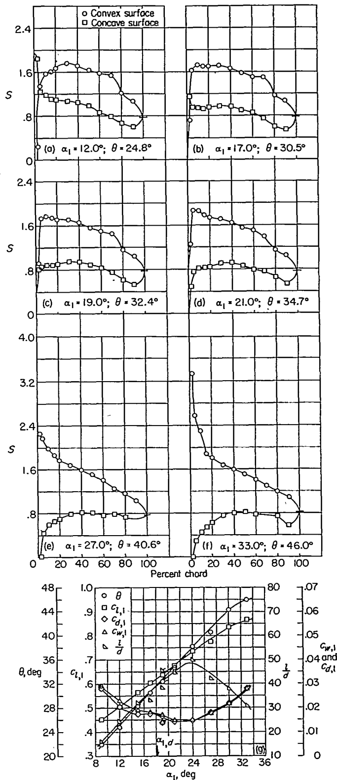
FIGURE 19.—Blade-surface pressure distributions and blade section characteristics for the cascade combination, \beta_1=30^\circ , \sigma=1.50 , and blade section, NACA 65-(15)10.
