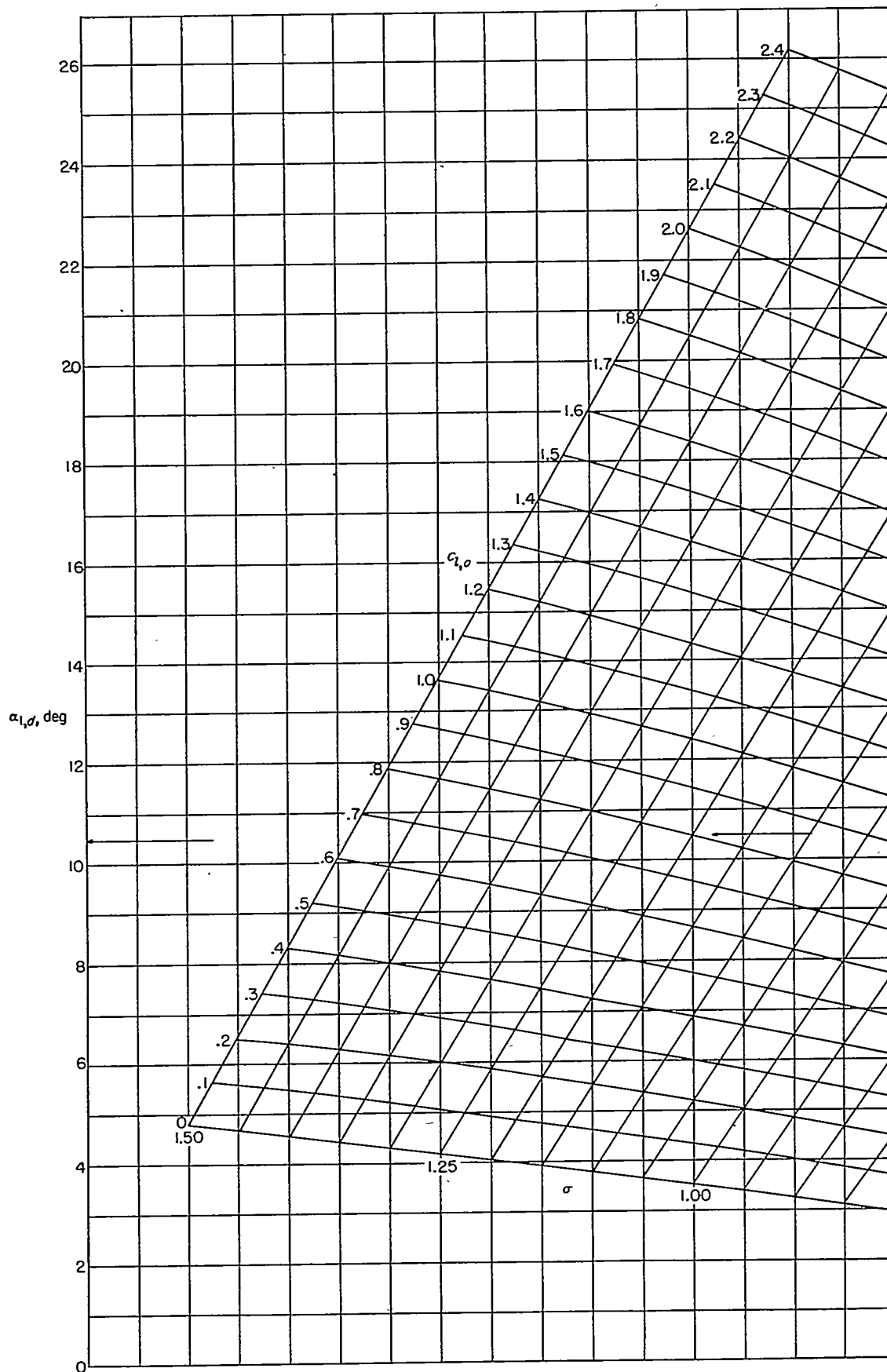
FIGURE 113.—Design angle-of-attack chart for NACA 65-( c_{l,o} )10 sections.
