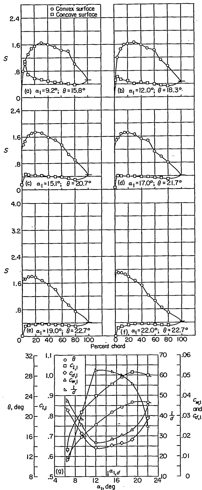
(g) Section characteristics.
