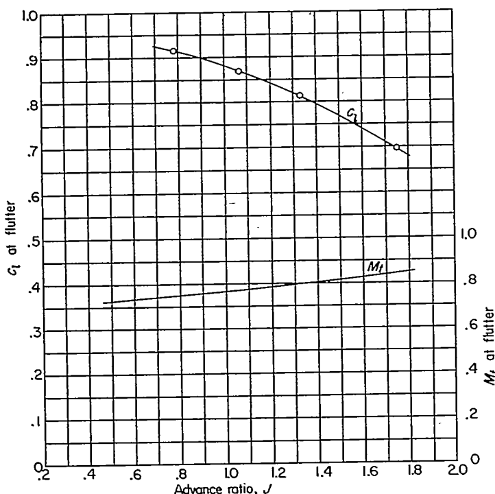
FIGURE 20.—Variation with advance ratio of lift coefficient and tip Mach number at flutter. \alpha=0.60 ; rotational speed, 1600 rpm.
