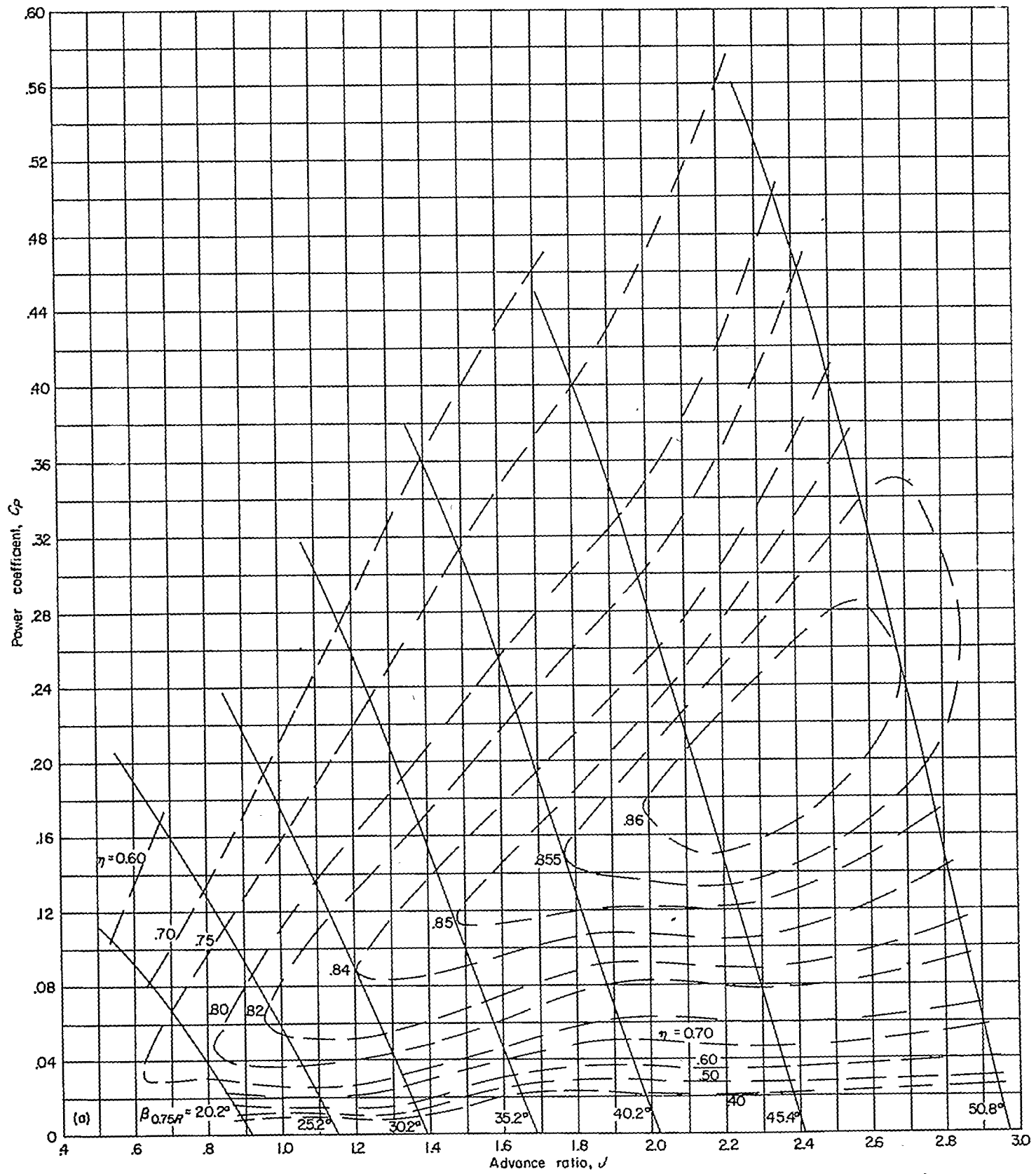
FIGURE 19.—Operating charts for three-blade propeller.
