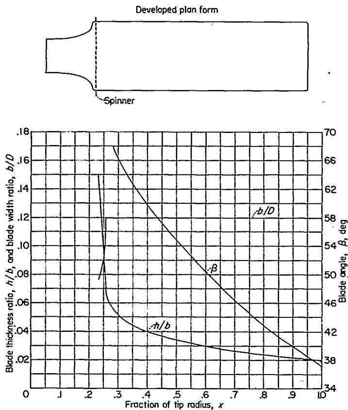
FIGURE 3.—Blade-form characteristics.
