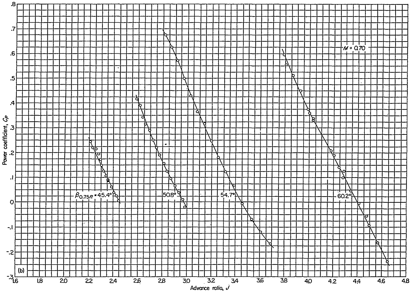
(b) Power coefficient. FIGURE 8.—Continued.
