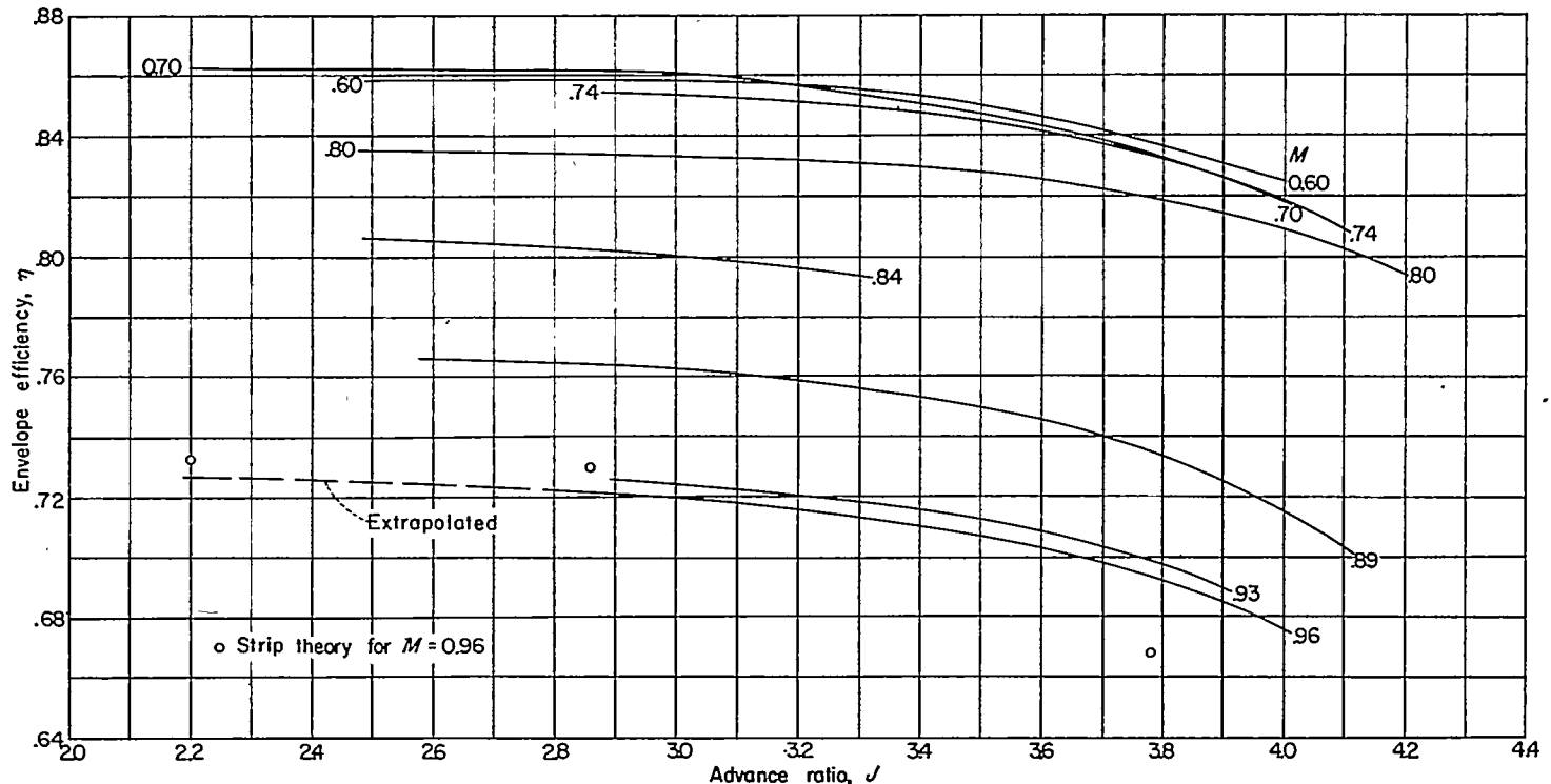
FIGURE 15.—Variation of envelope efficiency with advance ratio for various forward Mach numbers.
