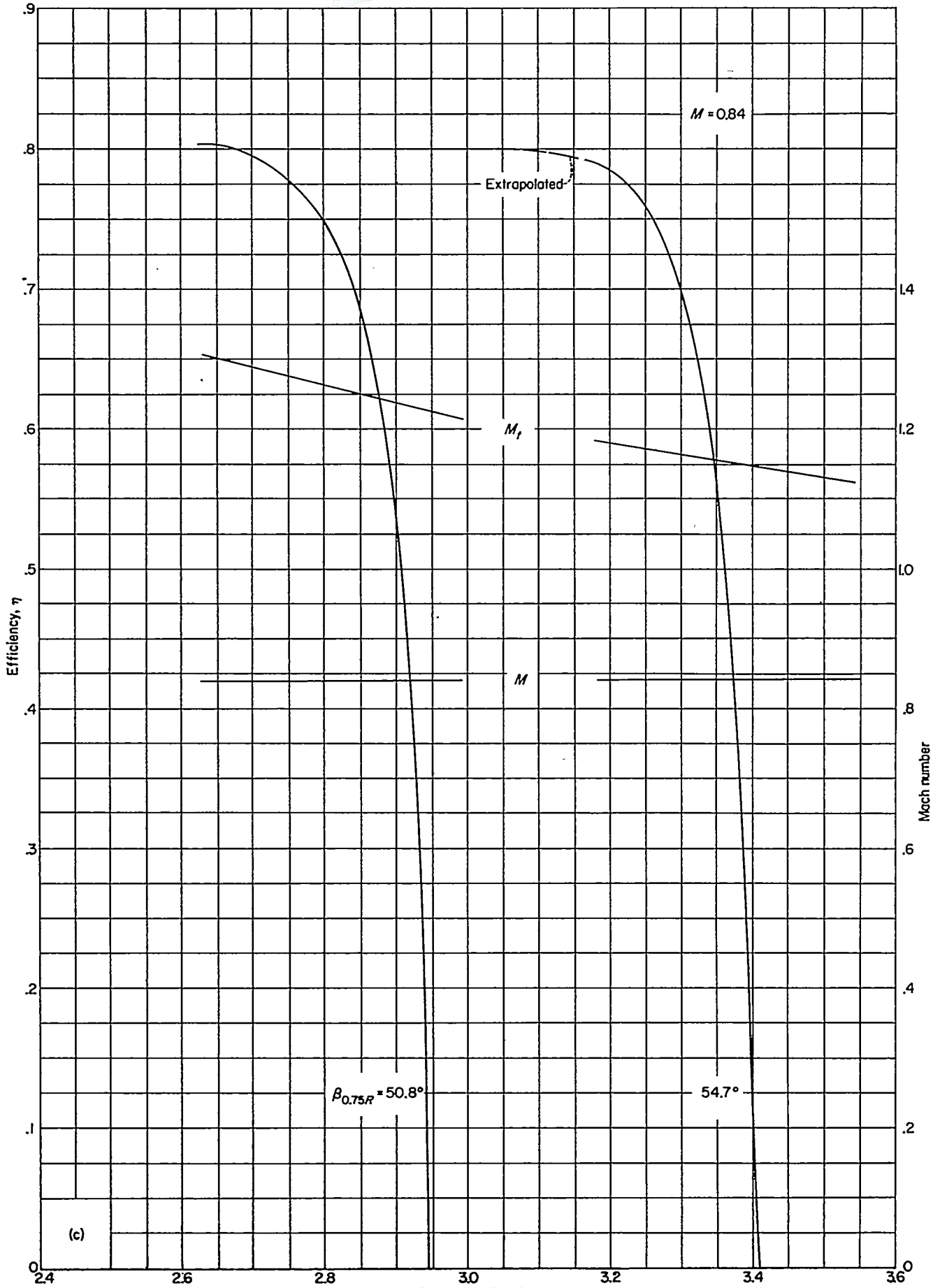
(c) Efficiency. FIGURE 11.—Concluded.
