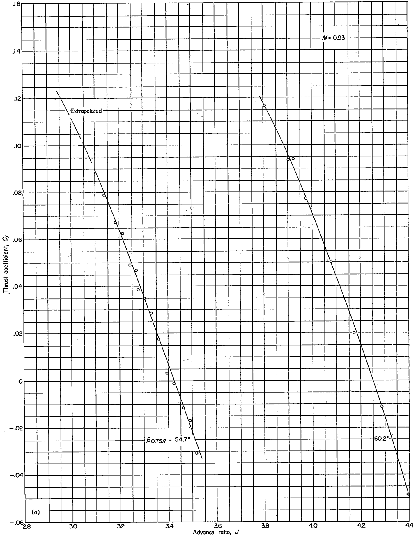
(a) Thrust coefficient. FIGURE 13.—Characteristics of propeller. Forward Mach number 0.93.
