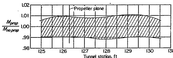
FIGURE 5.—Effect of propeller operation on the tunnel-wall measurements for the range of Mach numbers and thrust coefficients obtained in the tests.
