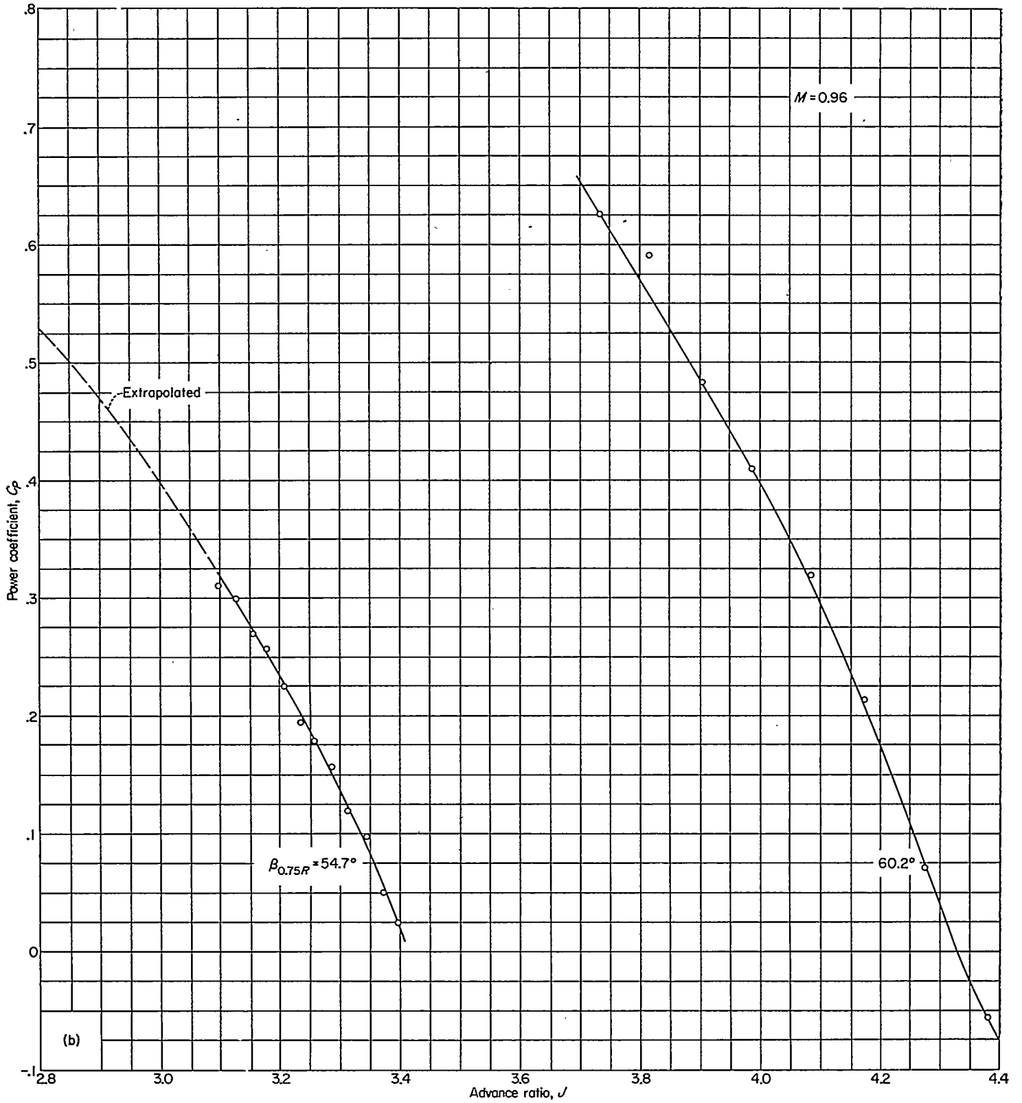
(b) Power coefficient. FIGURE 14.—Continued.
