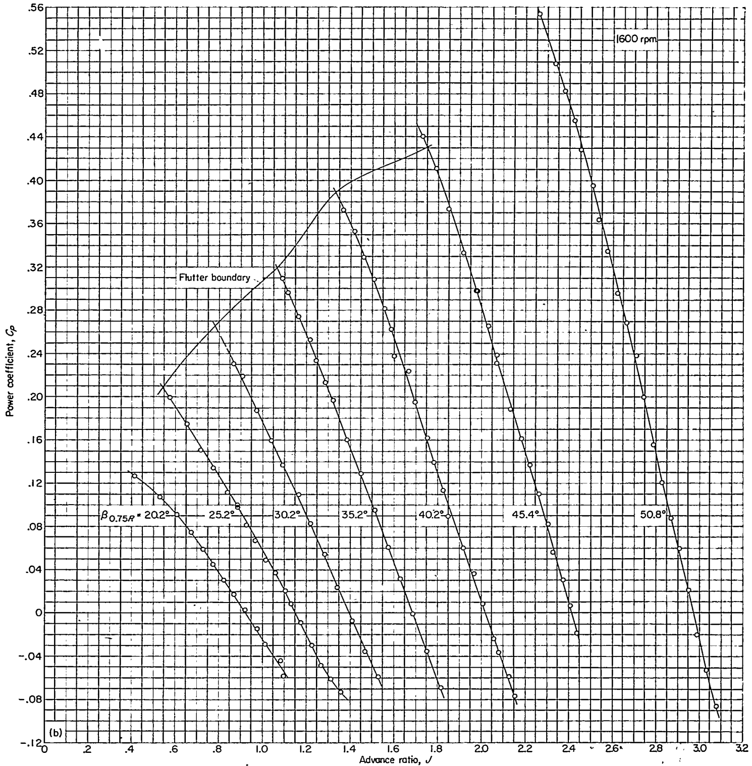
(b) Power coefficient. FIGURE 6.—Continued.
