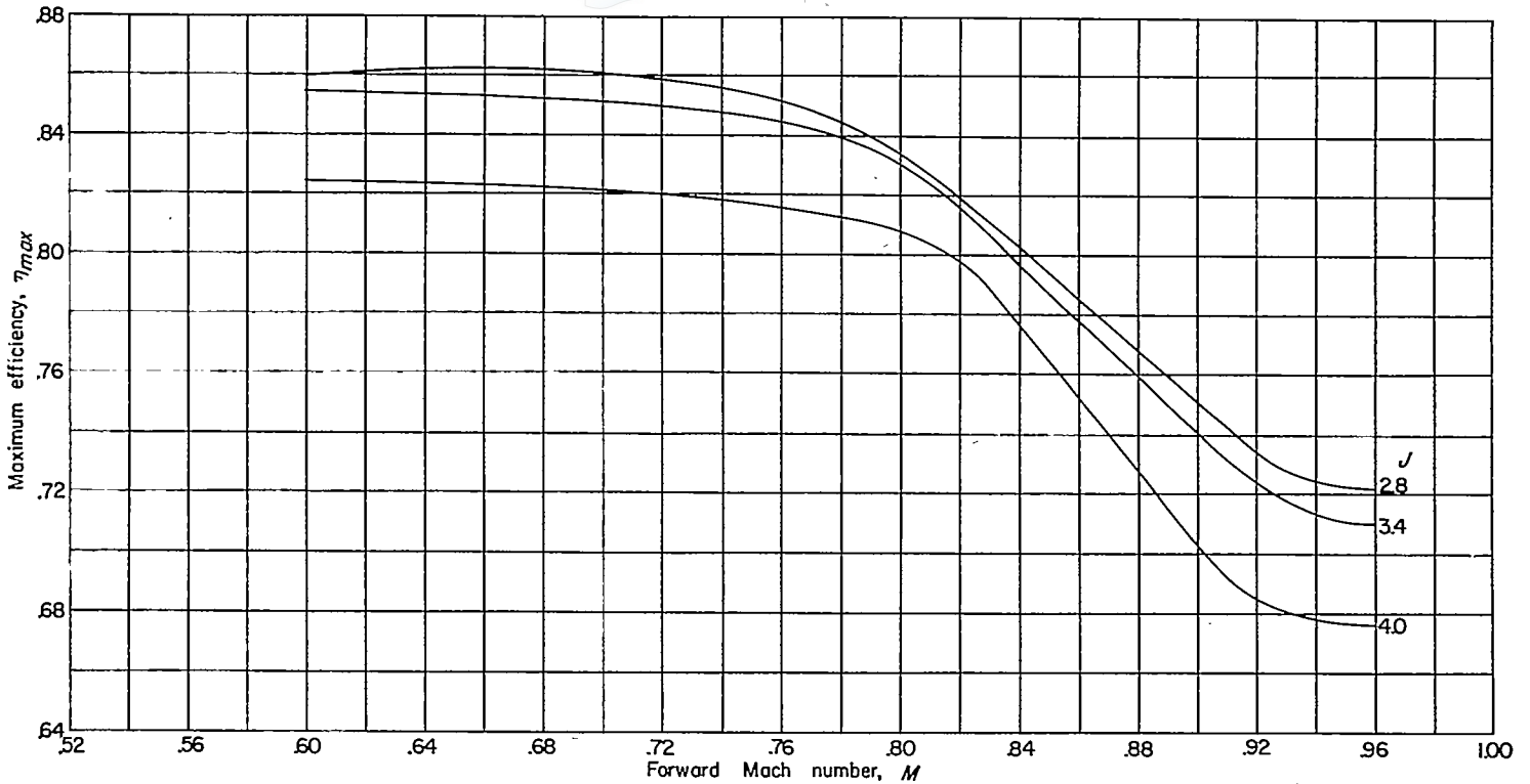
FIGURE 16.—Variation of maximum propeller efficiency with forward Mach number for several values of advance ratio.
