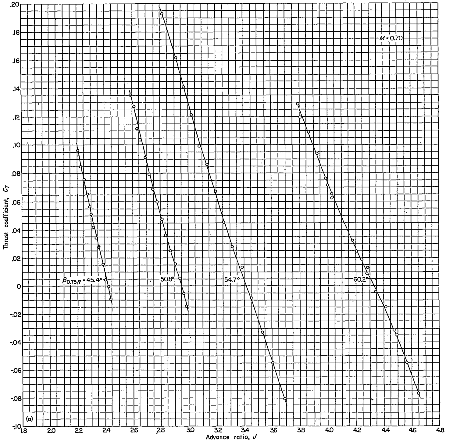
FIGURE 8.—Characteristics of propeller. Forward Mach number 0.70.
