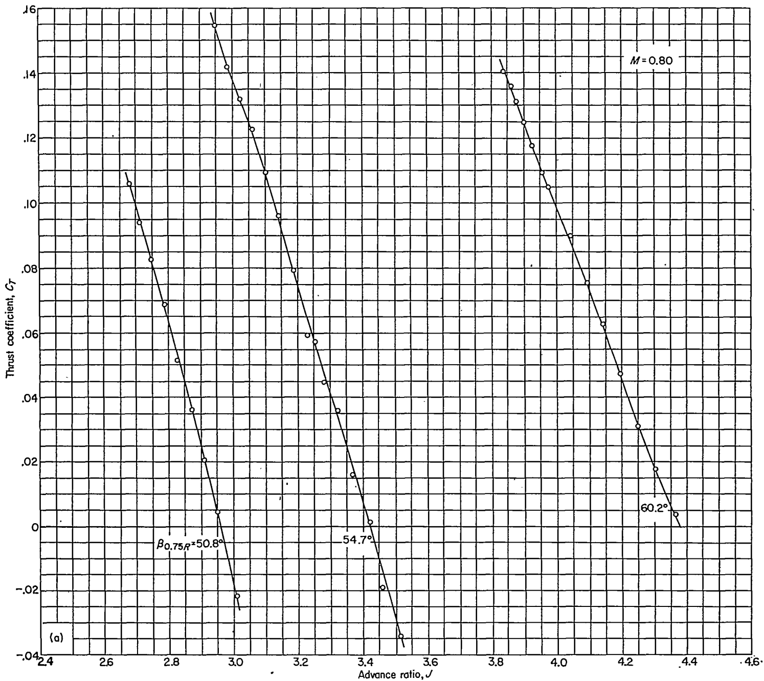
(a) Thrust coefficient. FIGURE 10.—Characteristics of propeller. Forward Mach number 0.80.
