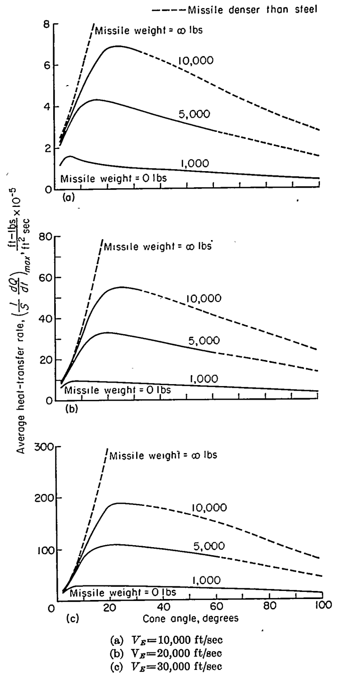
FIGURE 7.—Maximum average rate of convective heat transfer to conical missiles of the same base area entering the earth's atmosphere at an angle of 30° to the horizontal and velocities of 10,000, 20,000, and 30,000 ft/sec (base area=10 sq ft).
