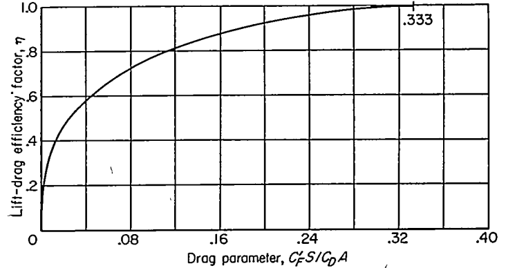
FIGURE 16.—Variation of lift-drag efficiency factor with drag parameter for cones.
