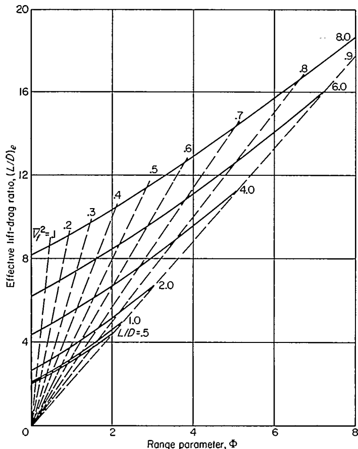
FIGURE 5.—Variation of effective lift-drag ratio with range for various values of aerodynamic lift-drag ratio of skip vehicle.
