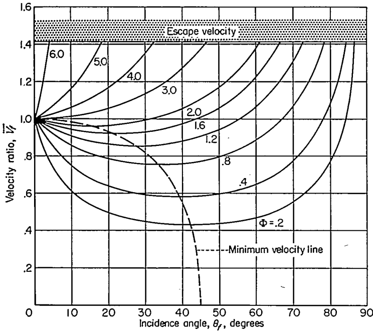
FIGURE 1.—Variation of velocity with incidence angle for various values of range of ballistic vehicle.
