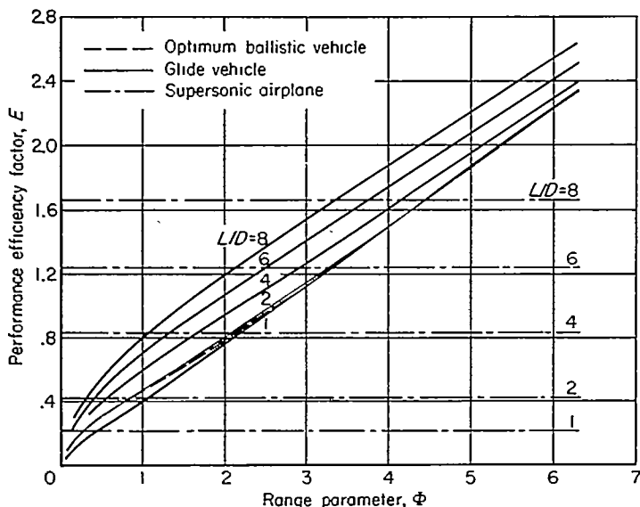
FIGURE 10.—Variation of performance efficiency factor with total range for ballistic and glide vehicles and the supersonic airplane.
