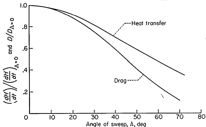
FIGURE 12.—Effect of sweep on drag and heat transfer to circular cylinders.
