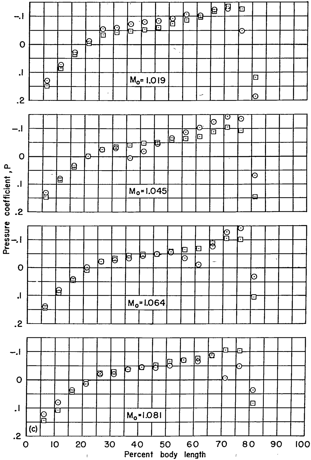
(c) Supersonic speeds ( M_o from 1.019 to 1.081).
