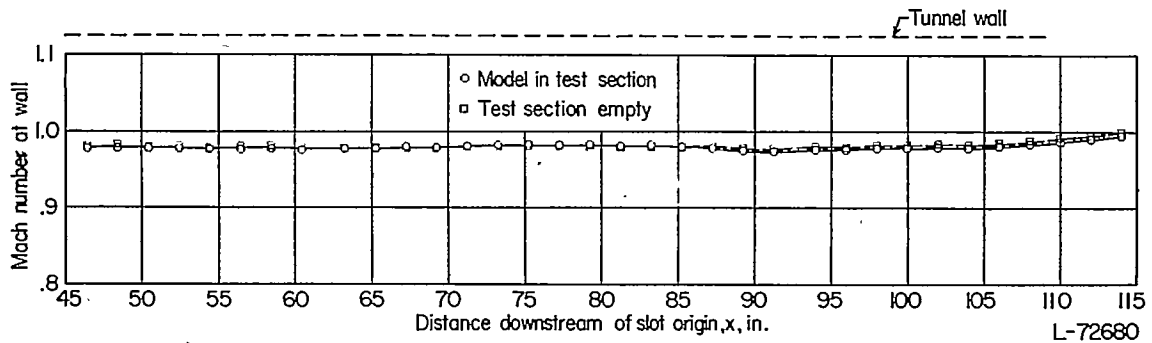
(b) M_0 = 0.980 .
