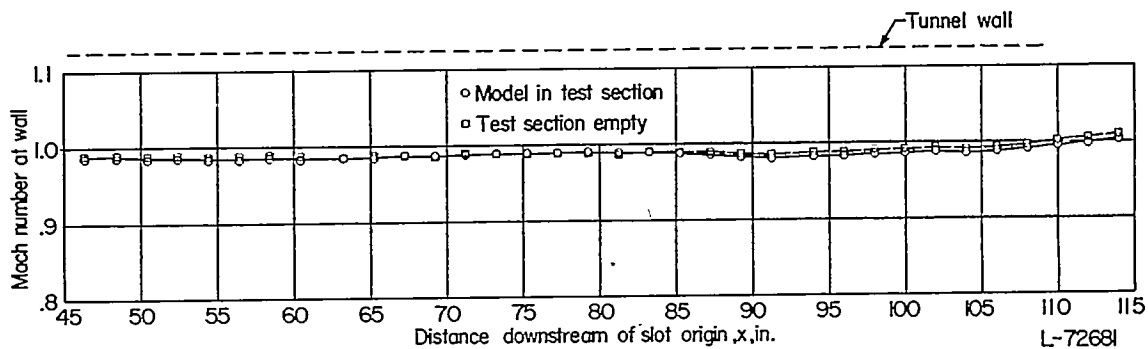
(c) M_0 = 0.990 .
