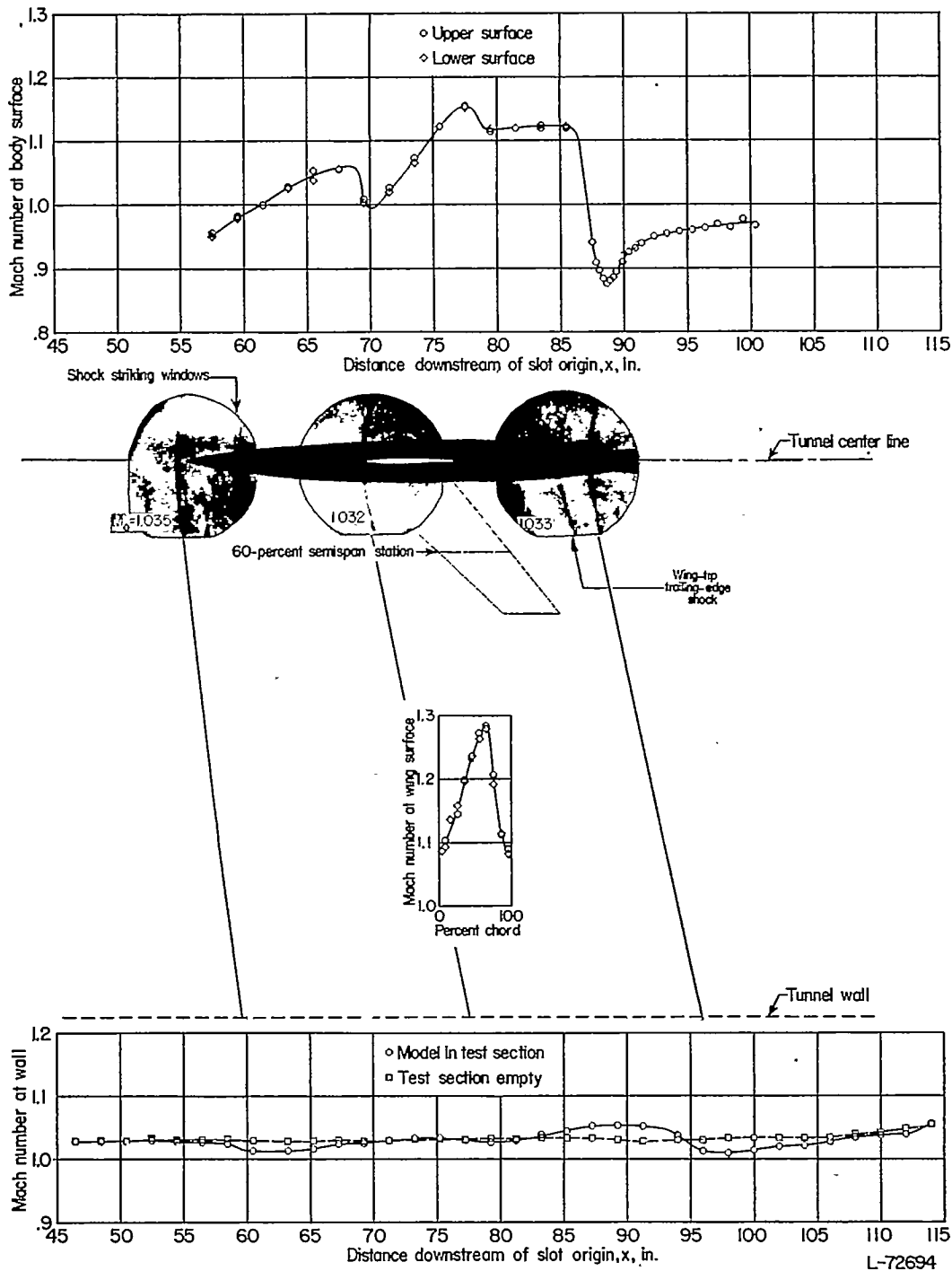
(b) M_0 = 1.034 . FIGURE 32.—Continued.
