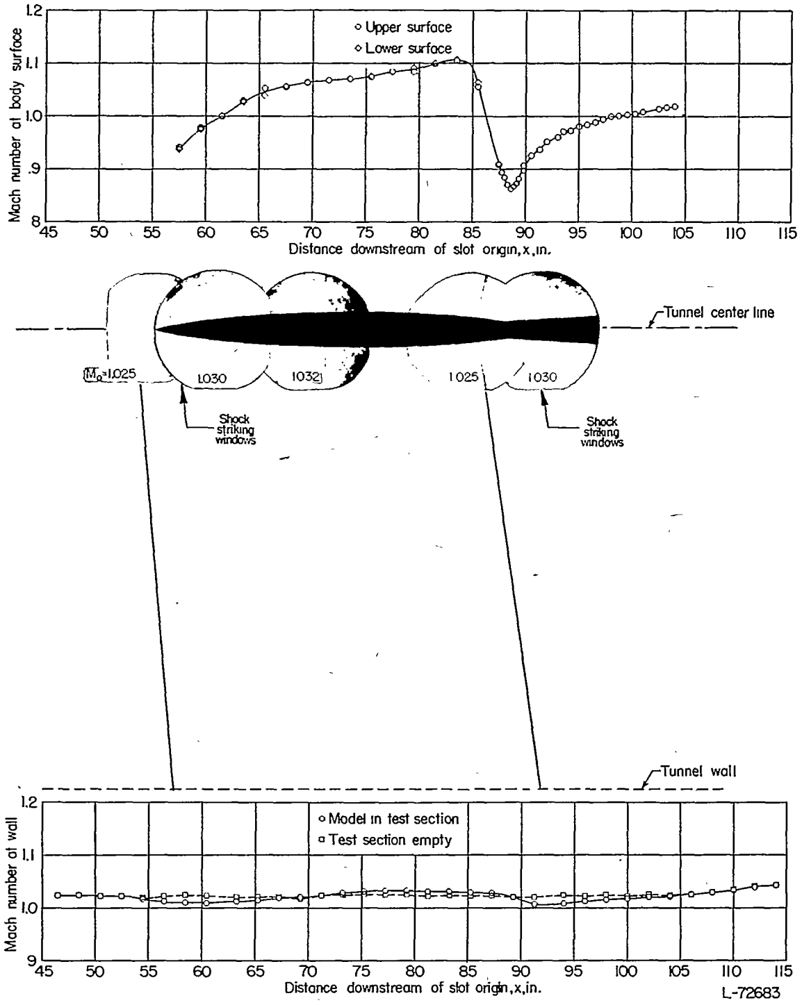
(e) M_o = 1.025 .
