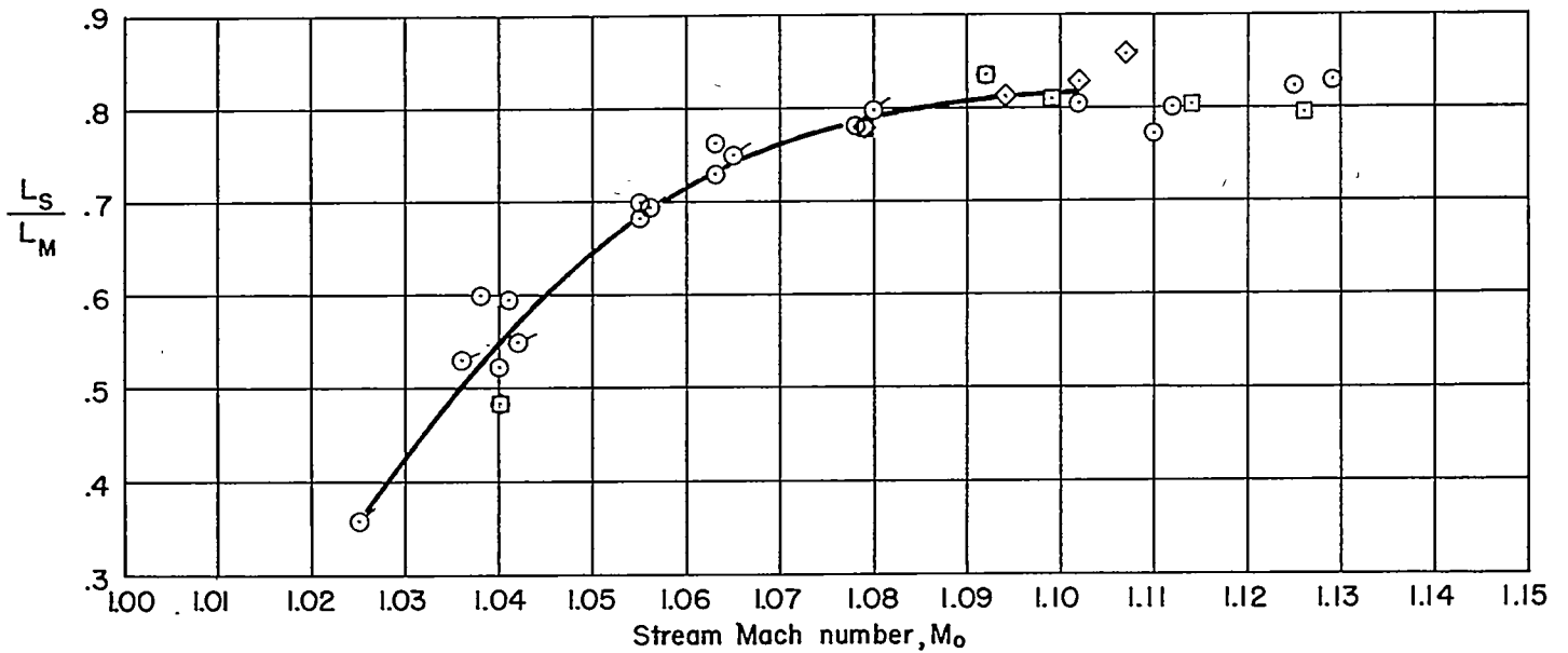
FIGURE 39.—Axial distance required for model bow wave to reflect from test-section wall and strike surface of model near center line. \alpha=0^\circ
