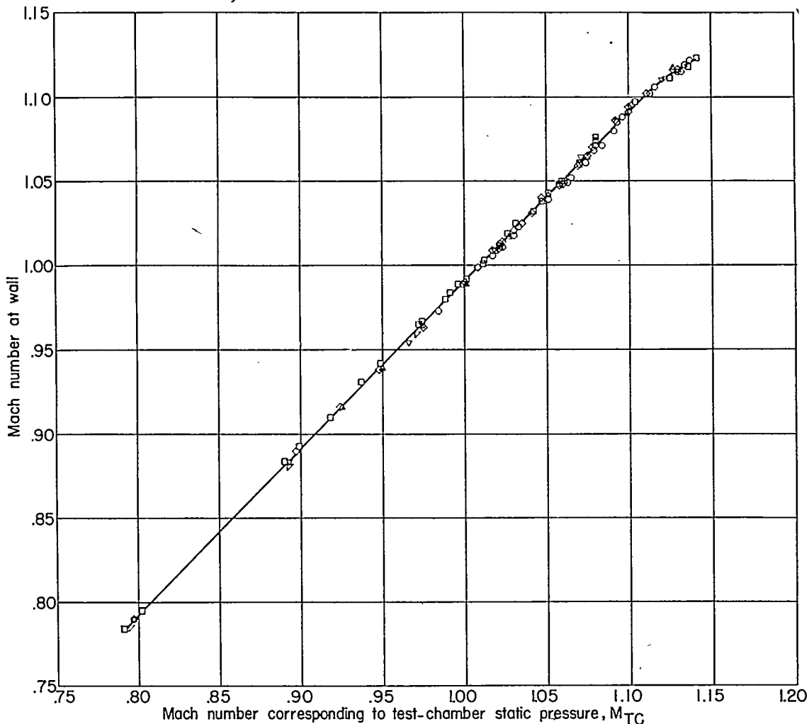
FIGURE 29.—Variation with test-chamber Mach number of Mach numbers measured on tunnel wall approximately 10 inches upstream of model nose (model at different angles of attack) and Mach numbers measured at the same axial station with model removed. Slot shape 11.
