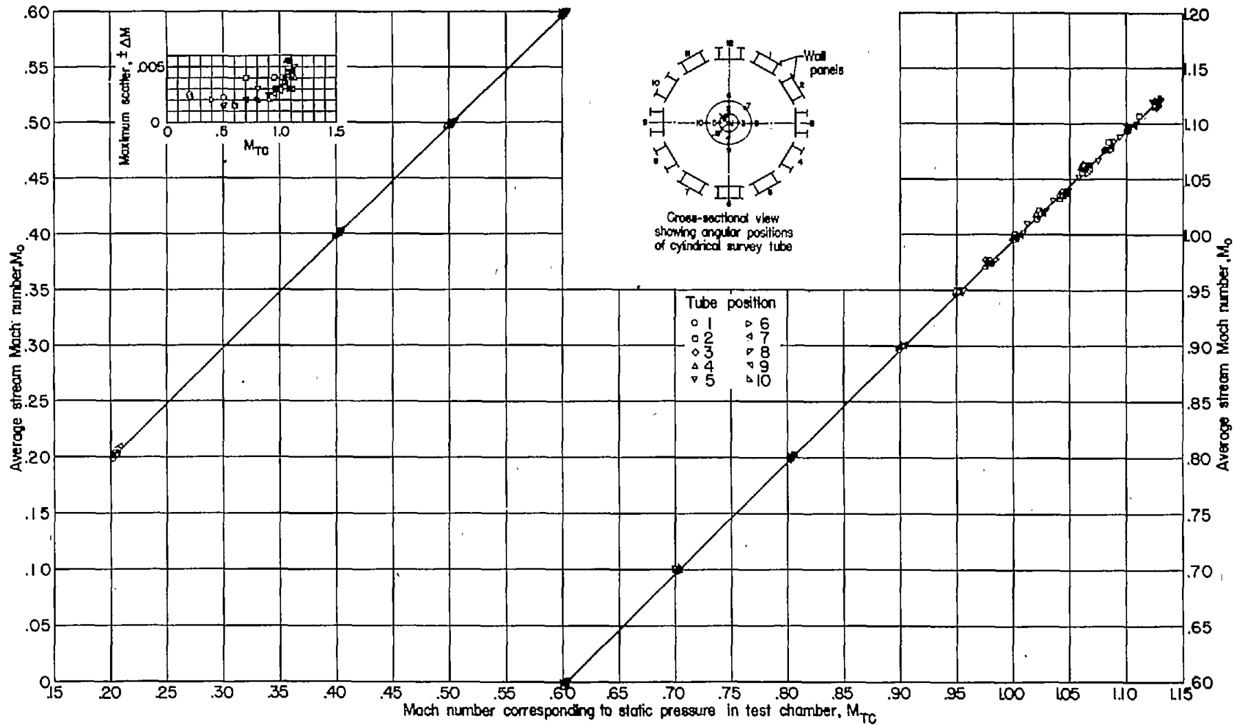
FIGURE 26.—Typical calibration curve showing the variation with test-chamber Mach number of the average Mach number over a test region 86 inches long and 30 inches in diameter near the center line of the slotted test section with diffuser-entrance nose A. Model removed; slot shape 11.
