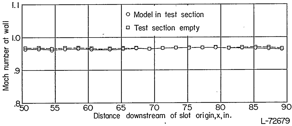
(a) M_o = 0.970 .
