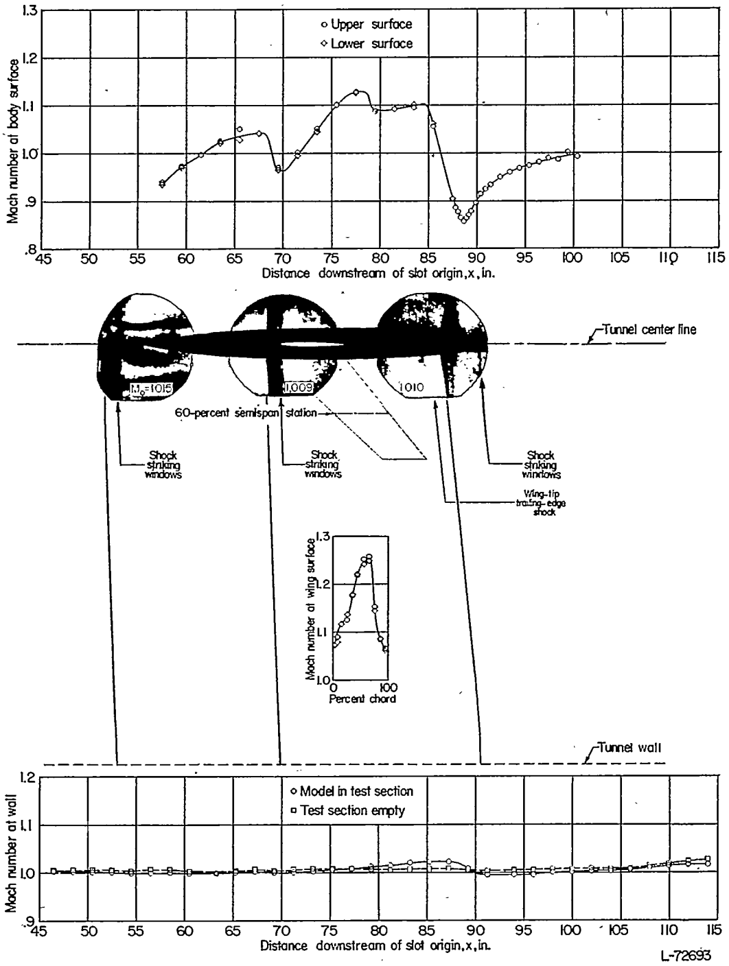
(a) M_0 = 1.009 .
