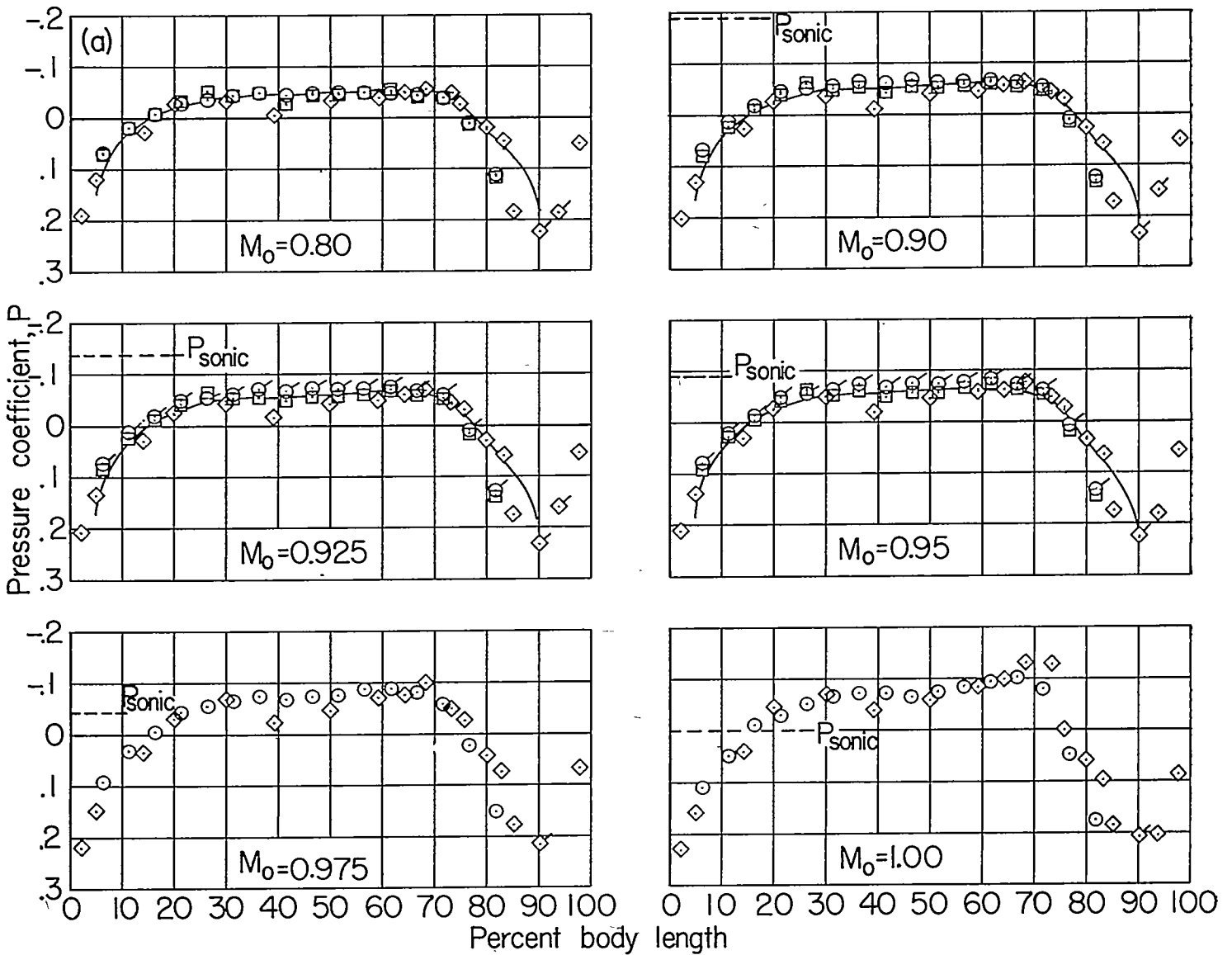
FIGURE 33.—Comparison of body-surface pressure distributions obtained from tests of a body of revolution in the slotted test section with those from closed-test-section tests, free-fall tests, and theory. Flagged symbols indicate data obtained from faired curves.
