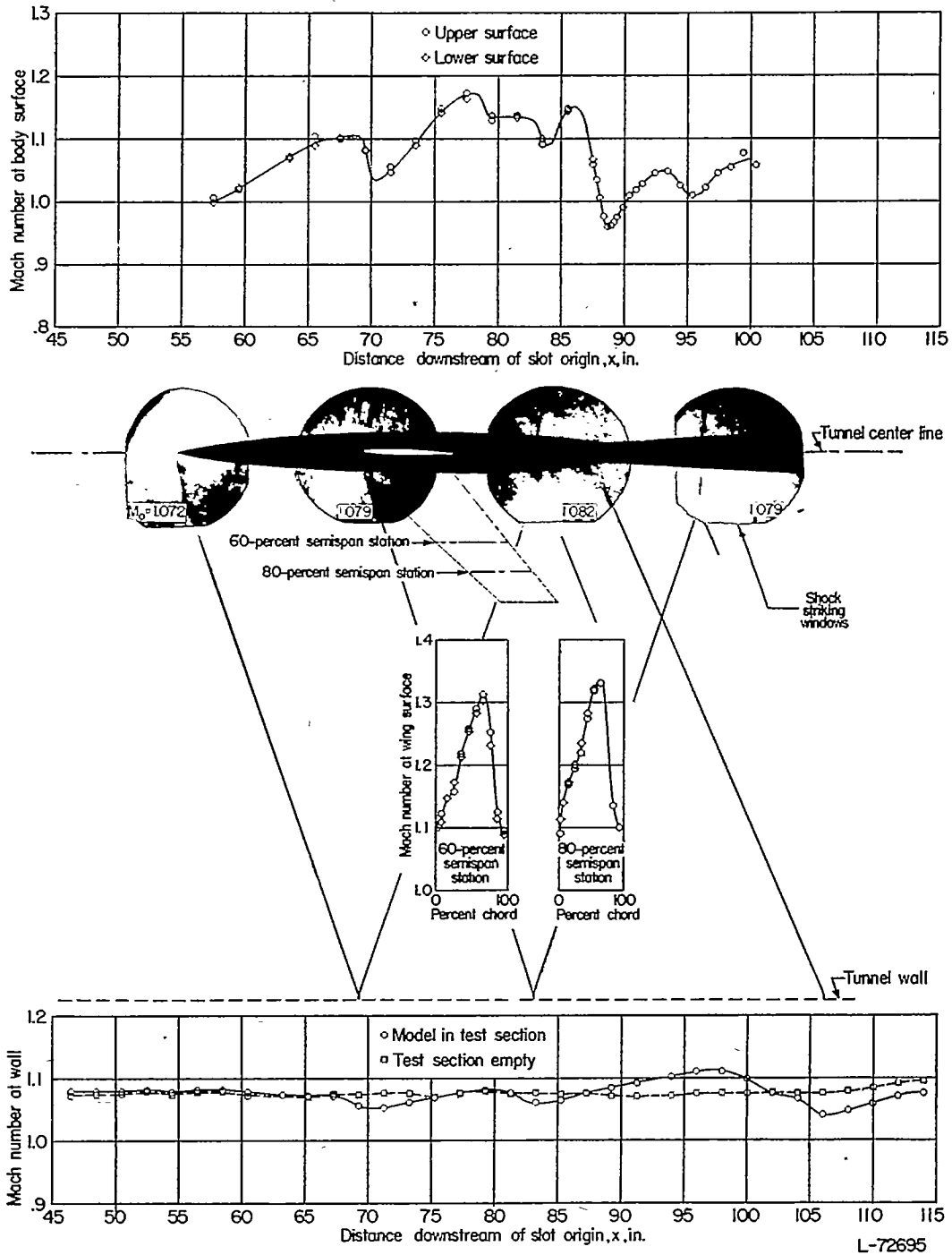
(c) M_o=1.079 .
