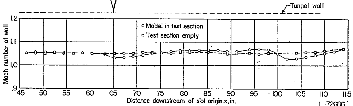
(h) M_0 = 1.056 .
