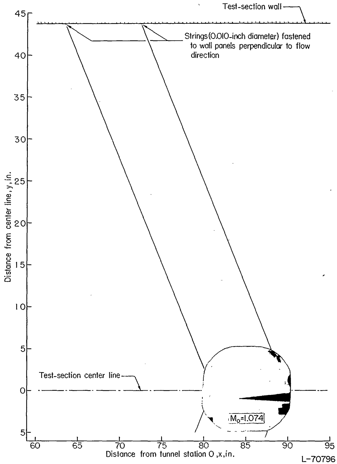
FIGURE 24.—Schlieren picture illustrating the propagation of weak disturbances in supersonic flow in the slotted test section. M_o=1.074 .
