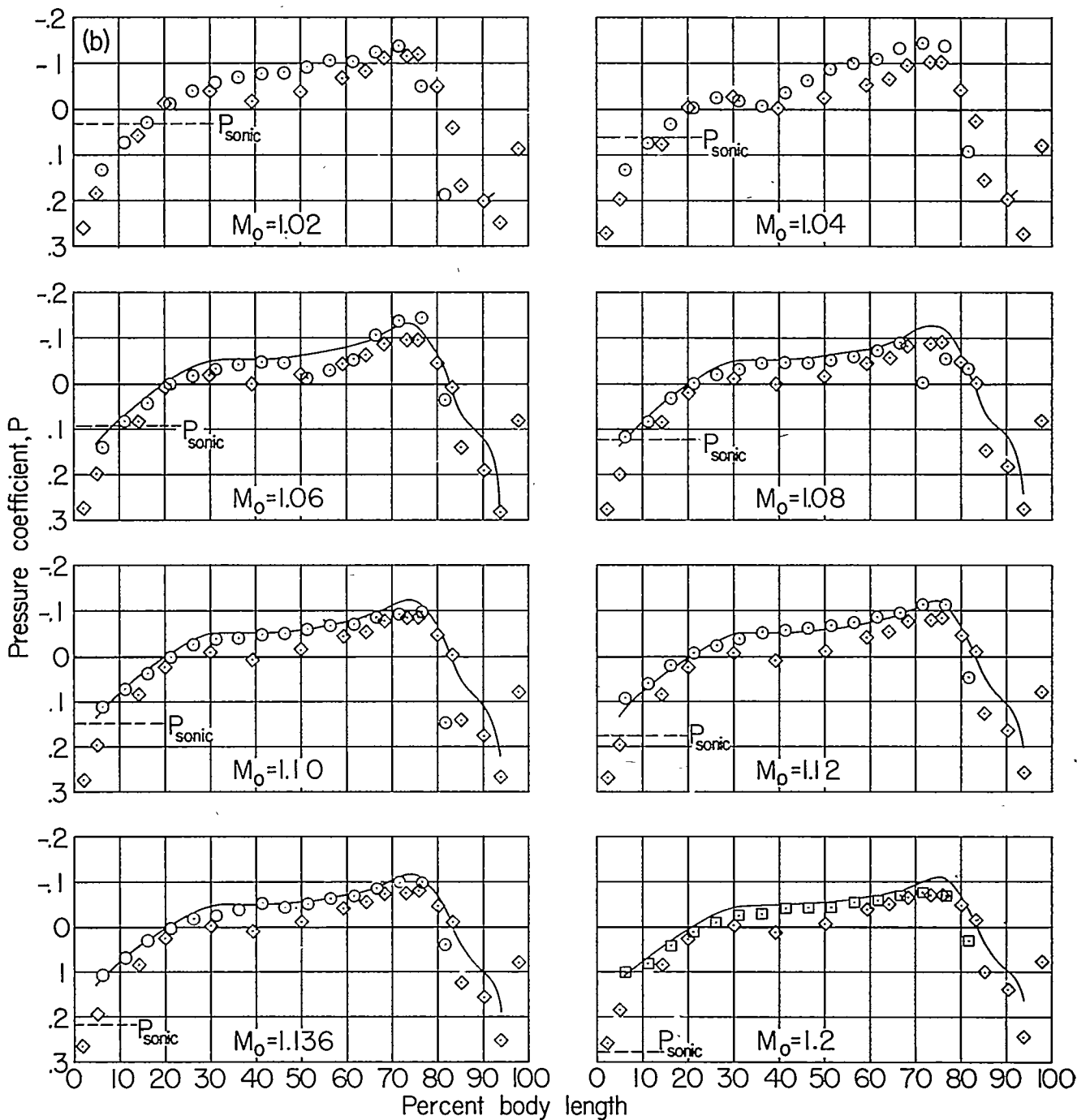
(b) Supersonic speeds.
