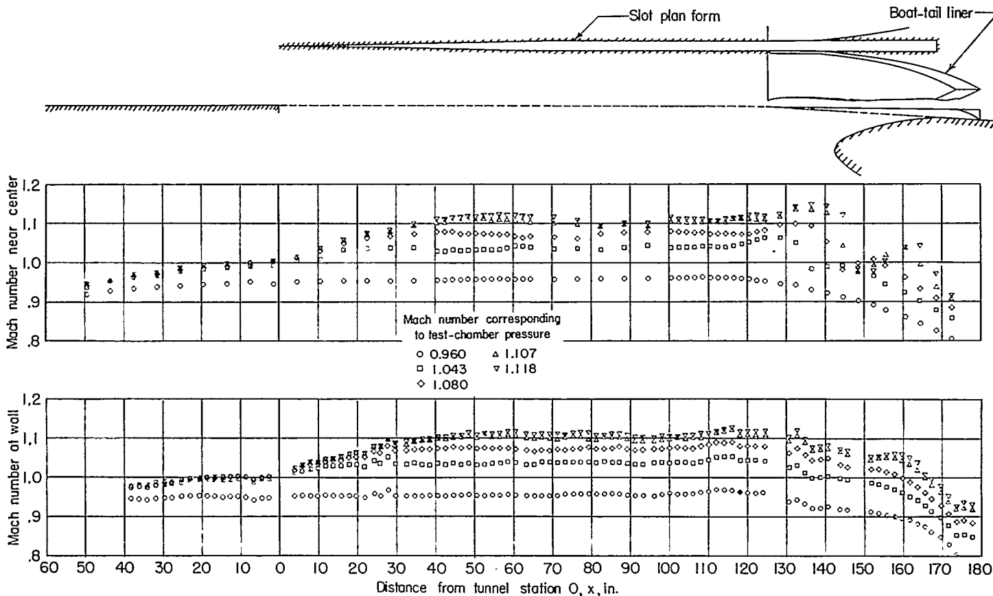
FIGURE 18.—Mach number distributions axially along center line and wall of the slotted throat with 5-minute divergence of test-section wall panels. Slot shape 7.
