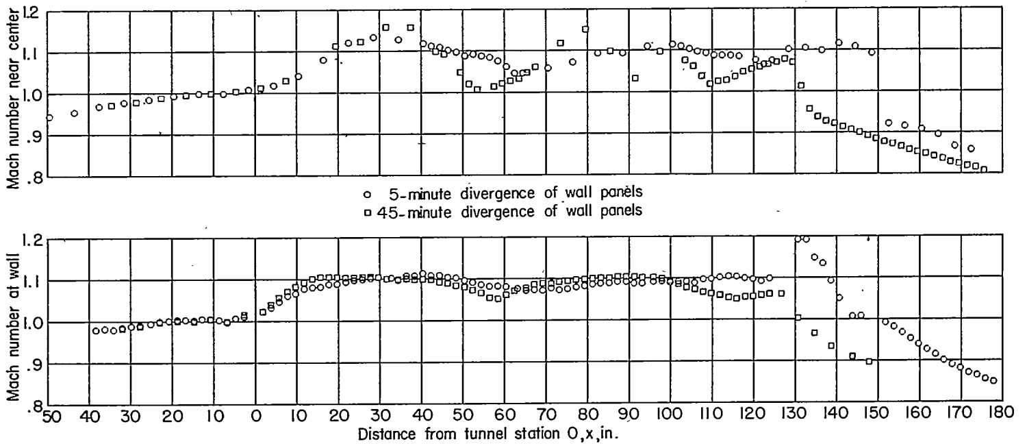
FIGURE 12.—Comparison of Mach number distributions axially along center line and wall of the slotted throat with 5-minute and 45-minute divergence of test-section wall panels. Slot shape 10; M_{TC}=1.093 .
