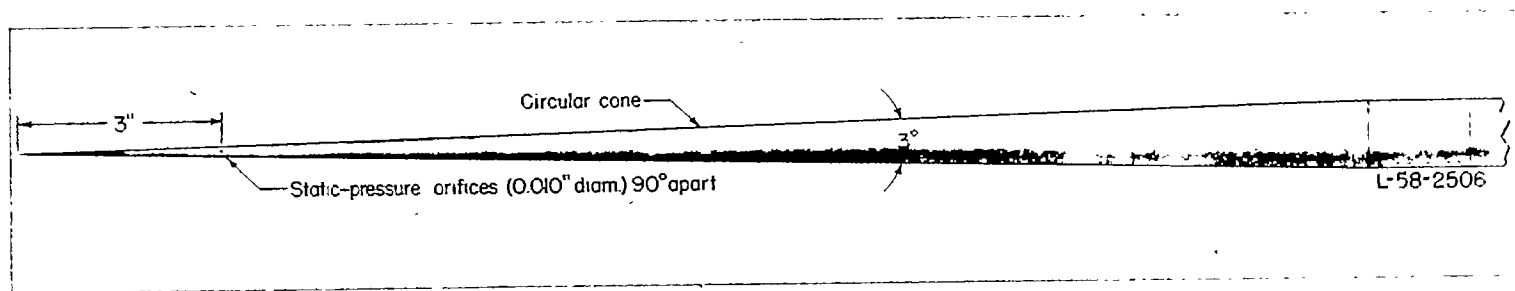
FIGURE 8.—Null-pressure-type instrument (3° cone) used for measuring angularity of flow in slotted test section.
