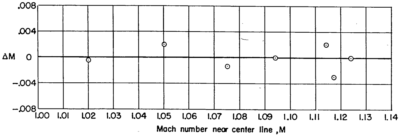
FIGURE 11.—Agreement of flow Mach numbers obtained from pressure measurements at test-section center line with those indicated by measured angularity of weak shocks produced by 0.010-inch-diameter strings fastened to wall panels. \Delta M is the Mach number from pressure measurements minus the Mach number indicated by shock angles.
