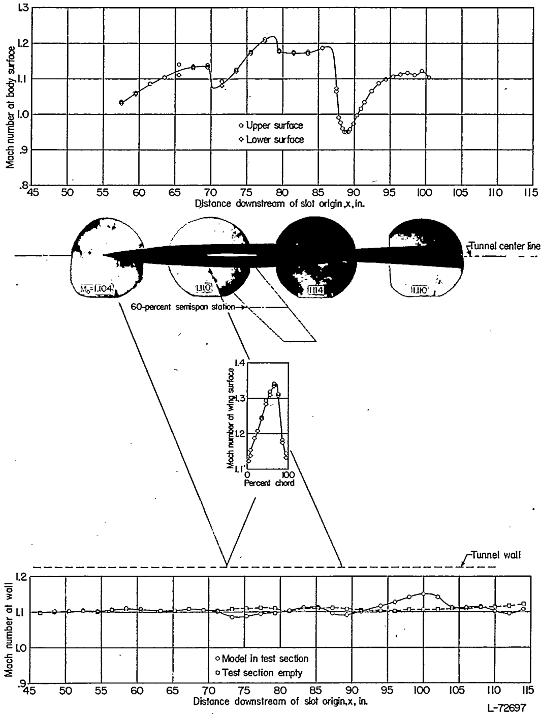
(e) M_o = 1.110 .
