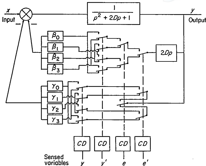
FIGURE 5.—Block diagram showing complete physical interpretation of equation (8). CD, zero-coincidence detectors.
