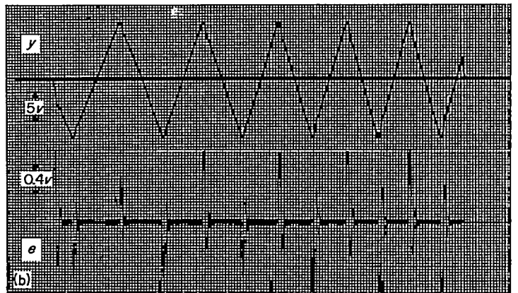
FIGURE 17.—Nonlinear system responses to 20-volt peak-to-peak triangular-wave input with period T varied. D=0.1 ; \beta_3=-\beta_0=12 ; \beta_2=-\beta_1=3 ; \gamma_3=-\gamma_0=2 ; \gamma_2=-\gamma_1=0.5 ; 2.5 small divisions on time scale=1 normalized time unit; tick marks at bottom of figures indicate when period was varied
