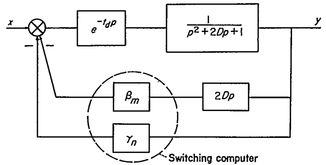
FIGURE 28.—Insertion of time-delay circuit for study of transport delays.
