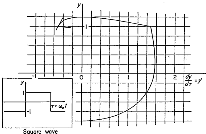
FIGURE 21.—Portion of output phase diagram for square-wave input. \beta_3 = -\beta_0 = 2 ; \beta_2 = -\beta_1 = 0.5 ; \gamma_3 = -\gamma_0 = 2 ; \gamma_2 = -\gamma_1 = 0.5 ; D = 0.6 ; \omega_r = 1 .
