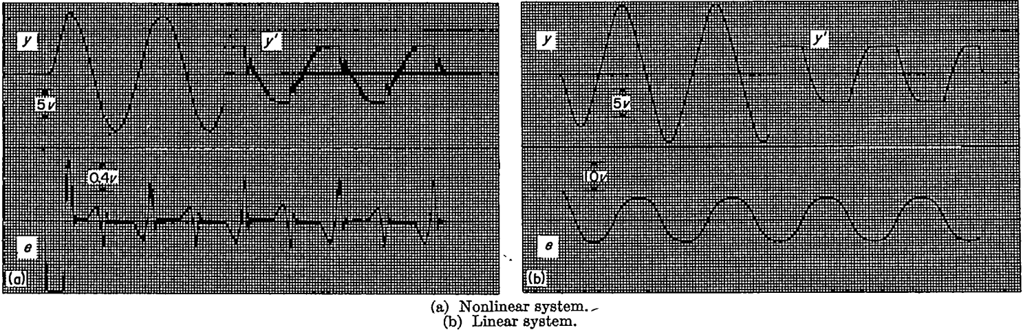
FIGURE 15.—Linear and nonlinear system responses to 20-volt peak-to-peak sinusoidal input with \pm 4\frac{1}{2} -volt velocity limit. D=0.6 ; \Omega=2\pi/T=0.5 ; 2.5 small divisions on time scale=1 normalized time unit.
