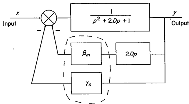
FIGURE 3.—Block diagram of equation (8) assuming that \beta_m and \gamma_n are constant (denoted by encircling dotted line).
