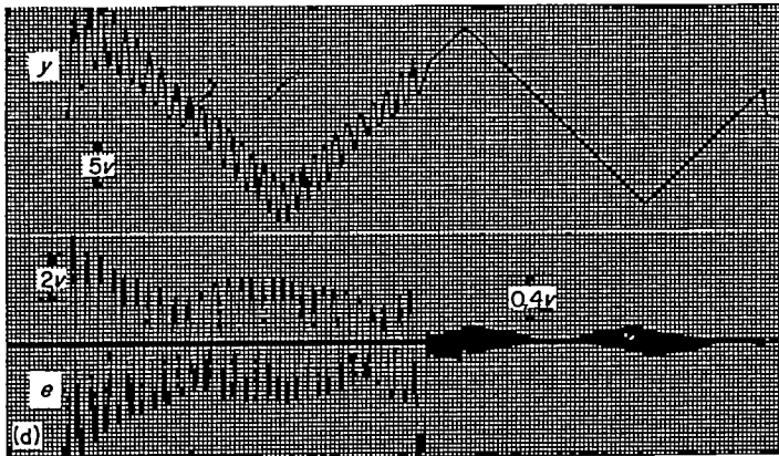
FIGURE 16.—Responses of nonlinear system with four different parameter sets to a 20-volt peak-to-peak triangular-wave input with fixed period T=10\pi . D=0.8 ; 2.5 small divisions on time scale=1 normalized time unit; tick marks at bottom of figures indicate demarcation between systems. For systems' numbering see table 3
