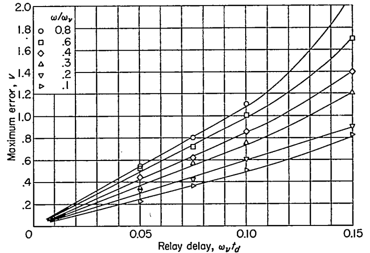
FIGURE 33.—Maximum error occurring during each input cycle plotted against switching delay with input frequency as a parameter (same data as for fig. 32).
