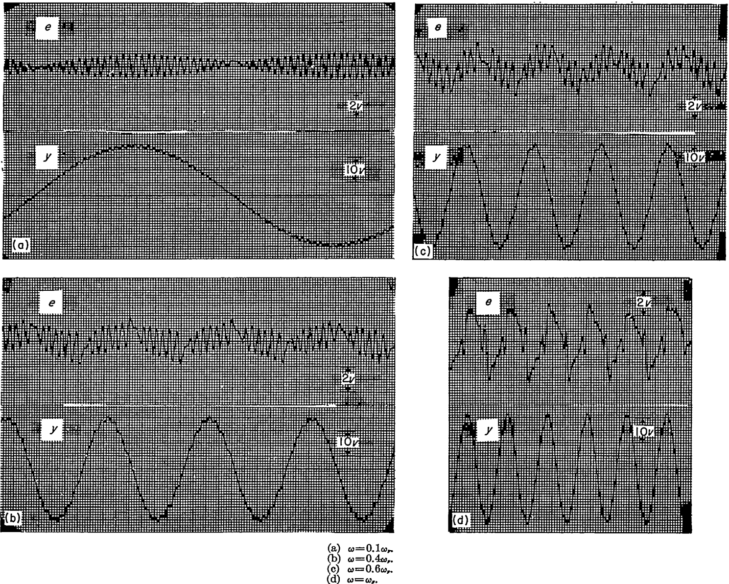
FIGURE 31.—Responses for inputs of various frequencies with relay delays of \omega_r t_d = 0.10 .
