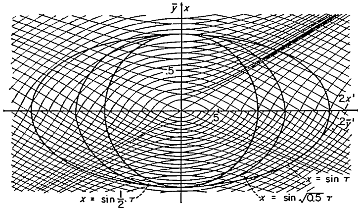
FIGURE 20.—Superposed input and output phase planes showing available angular sectors for sinusoidal inputs. {}_1\beta=1.5 ; {}_1\gamma=0.45 ; {}_2\beta=0.5 ; {}_2\gamma=0.05 ; 2D=0.25 ; \omega_r=2 ; |\beta|_{max}=2 ; |\gamma|_{max}=0.5 ; |\beta|_{min}=1 ; |\gamma|_{min}=0.4 .
