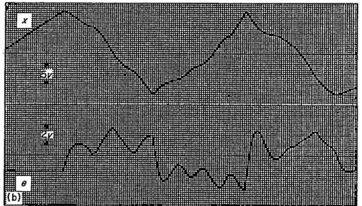
(a) Nonlinear system. \beta_3 = -\beta_0 = 2; \beta_2 = -\beta_1 = 0.1; \gamma_3 = -\gamma_0 = 2; \gamma_2 = -\gamma_1 = -0.5 . (b) Linear system.
