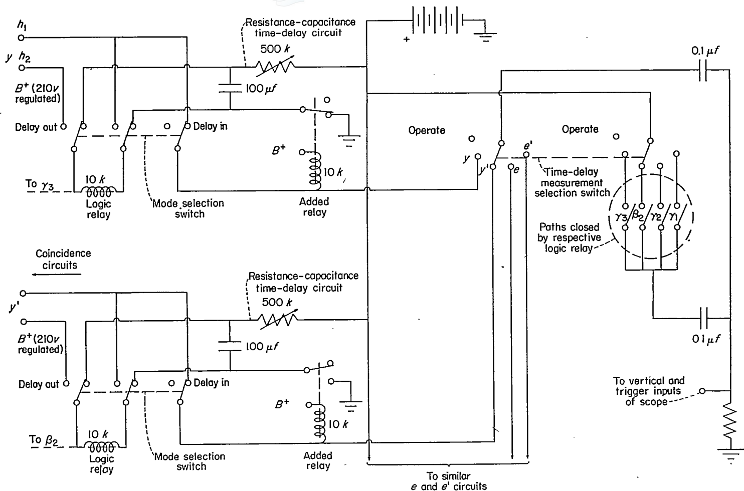
FIGURE 25.—Schematic diagram of electromechanical switching-delay simulation.
