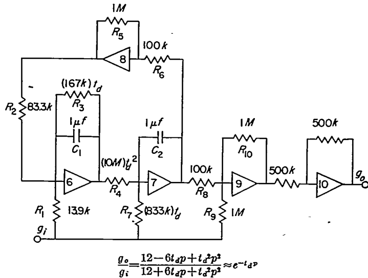
FIGURE 26.—Analog-computer circuit for Padé second-order approximation for e^{-t_d p} .
