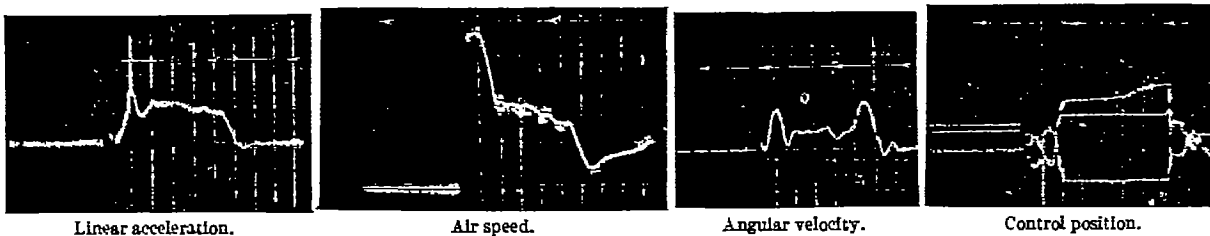
Fig. 5.—A set of records obtained with N. A. C. A. instruments. (Tall spin.)
